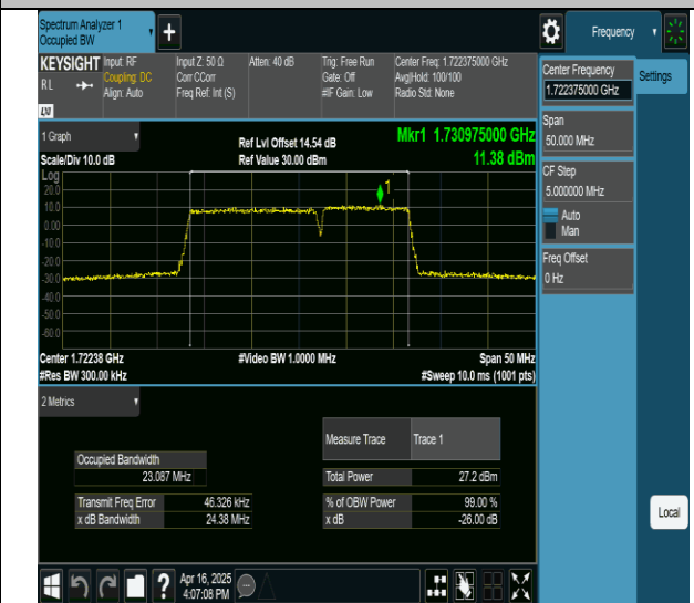
66-66-15MHz-10MHz-256QAM-256QAM-132047-132167-75RB#0-50RB#0-PASS
