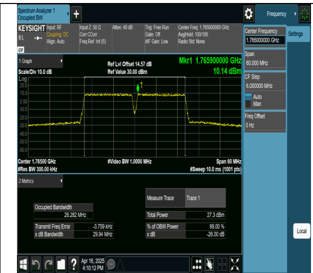
66-66-15MHz-15MHz-256QAM-256QAM-132447-132597- 75RB#0-75RB#0-PASS
