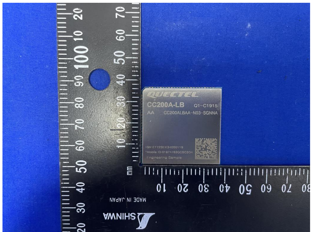
(1) EUT Photo
