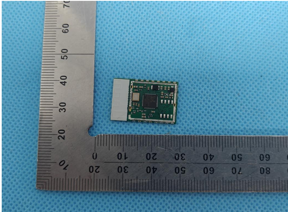
INTERNAL VIEW OF EUT (FIGURE 2)
