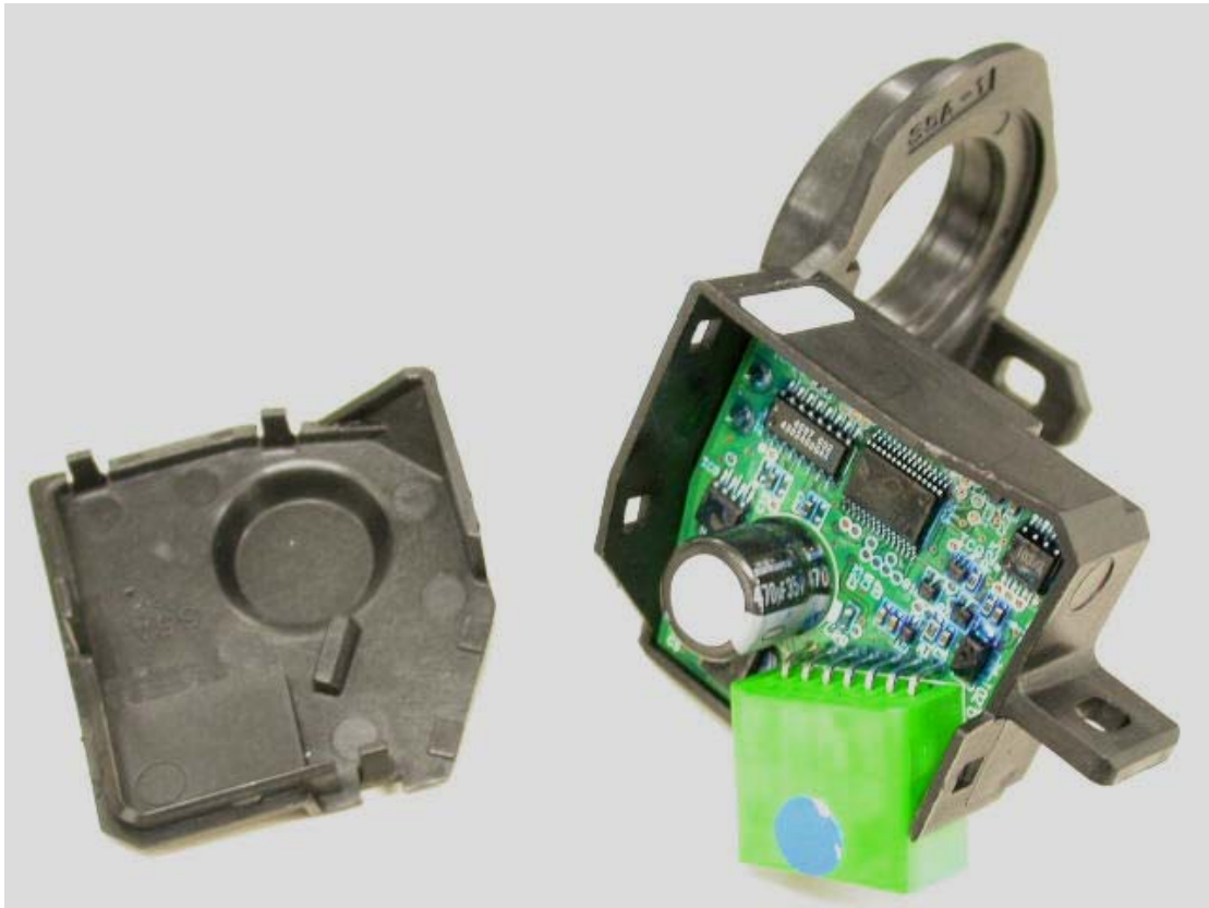
Internal side with cover of Immobiliser unit
