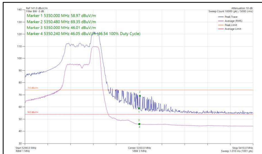
Figure 64 - 802.11ax, HE40, RU 52-44, SISO, Core 1 - 5310 MHz, Band Edge Frequency 5350 MHz
