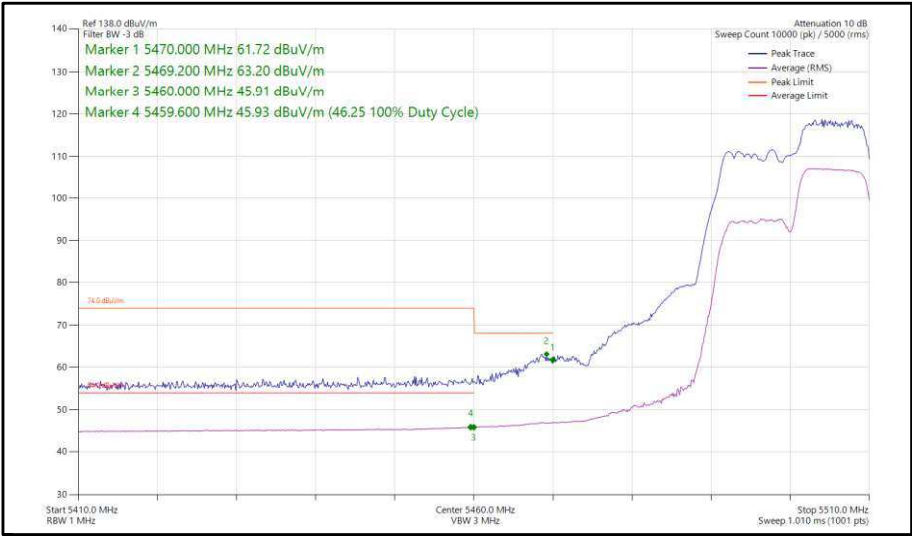
Figure 12 - 802.11ax, HE20, RU 106-54, SISO, Core 0 - 5500 MHz, Band Edge Frequency 5460 MHz
