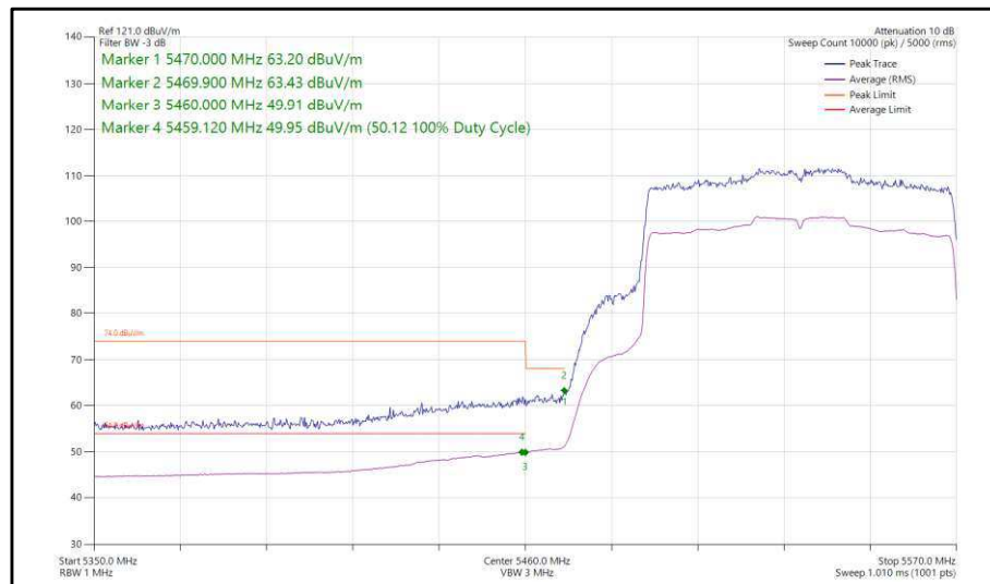
Figure 109 - 802.11ax, HE80, SU, SISO, Core 1 - 5530 MHz, Band Edge Frequency 5460 MHz
