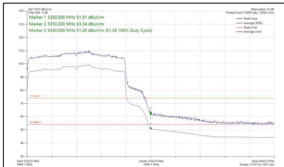
Figure 106 - 802.11ax, HE80, SU, SISO, Core 1 - 5290 MHz, Band Edge Frequency 5350 MHz
