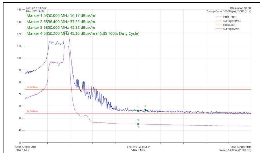
Figure 51 - 802.11ax, HE40, RU 52-44, SISO, Core 0 - 5270 MHz, Band Edge Frequency 5350 MHz
