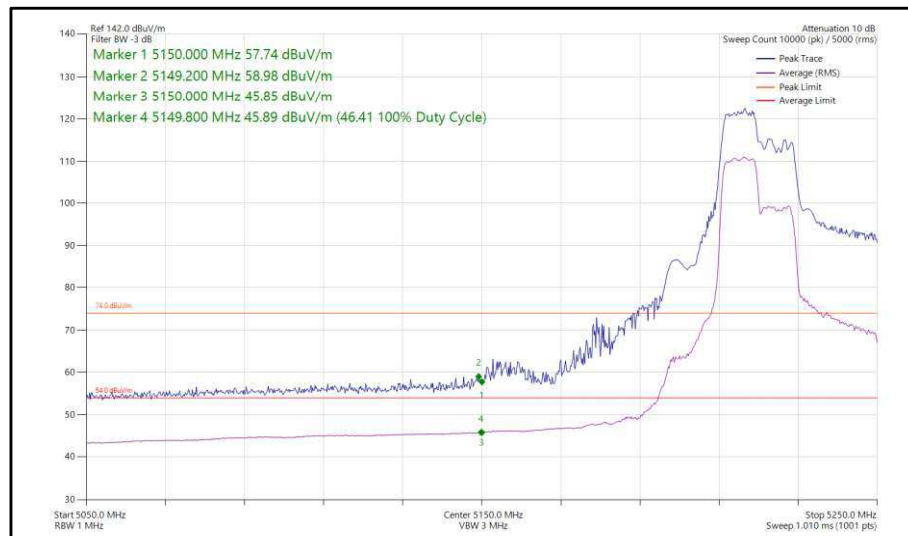
Figure 71 - 802.11ax, HE40, RU 106-53, CDD, Core 0-1 - 5230 MHz, Band Edge Frequency 5150 MHz
