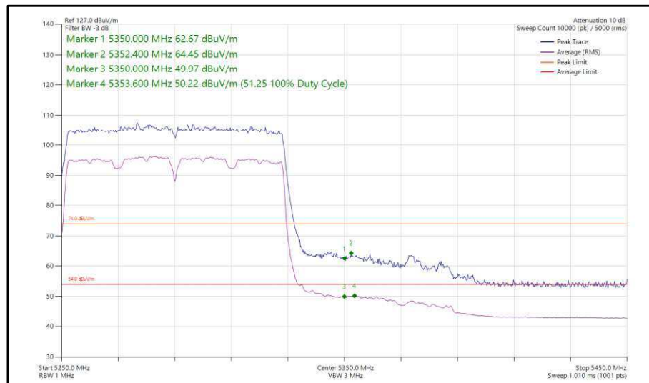
Figure 96 - 802.11ac, VHT80, SISO, Core 0 - 5290 MHz, Band Edge Frequency 5350 MHz
