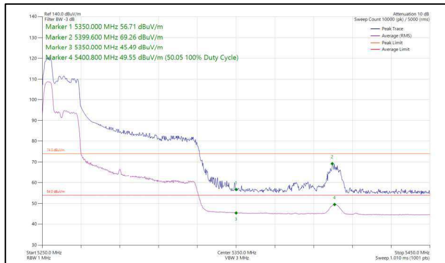
Figure 107 - 802.11ax, HE80, RU 52-37, SISO, Core 1 - 5290 MHz, Band Edge Frequency 5350 MHz
