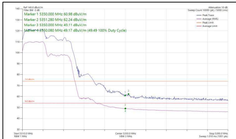
Figure 30 - 802.11ax, HE20, RU 106-53, CDD, Core 0-1 - 5320 MHz, Band Edge Frequency 5350 MHz
