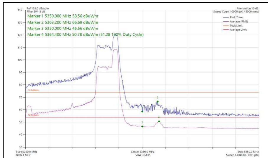
Figure 116 - 802.11ax, HE80, RU 52-52, CDD, Core 0-1 - 5290 MHz, Band Edge Frequency 5350 MHz
