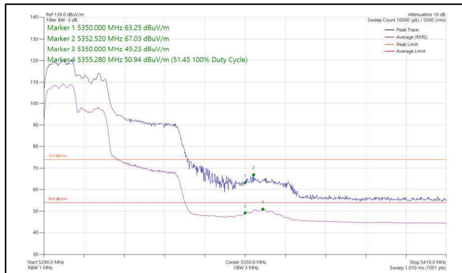
Figure 86 - 802.11ax, HE40, RU 106-53, SDM, Core 0-1 - 5310 MHz, Band Edge Frequency 5350 MHz
