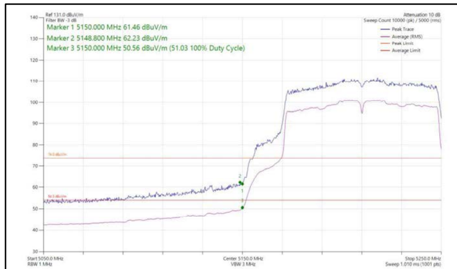
Figure 93 - 802.11ac, VHT80, SISO, Core 0 - 5210 MHz, Band Edge Frequency 5150 MHz
