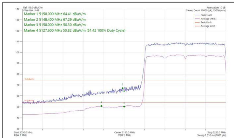
Figure 103 - 802.11ax, HE80, SU, SISO, Core 1 - 5210 MHz, Band Edge Frequency 5150 MHz
