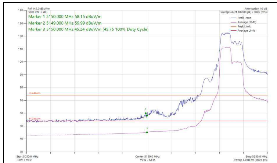
Figure 49 - 802.11ax, HE40, RU 106-53, SISO, Core 0 - 5230 MHz, Band Edge Frequency 5150 MHz
