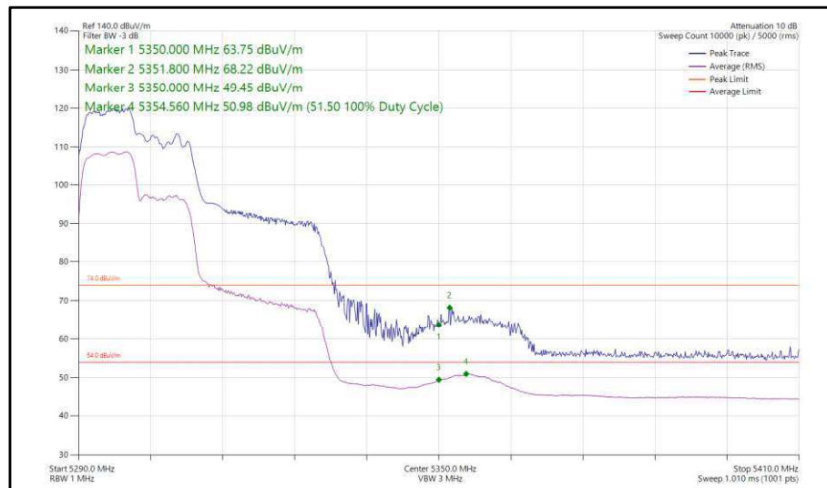
Figure 75 - 802.11ax, HE40, RU 106-53, CDD, Core 0-1 - 5310 MHz, Band Edge Frequency 5350 MHz
