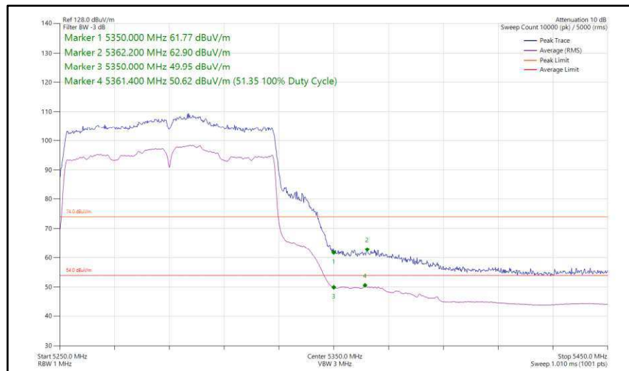
Figure 105 - 802.11ac, VHT80, SISO, Core 1 - 5290 MHz, Band Edge Frequency 5350 MHz
