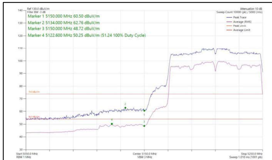
Figure 120 - 802.11ac, VHT80, SDM, Core 0-1 - 5210 MHz, Band Edge Frequency 5150 MHz
