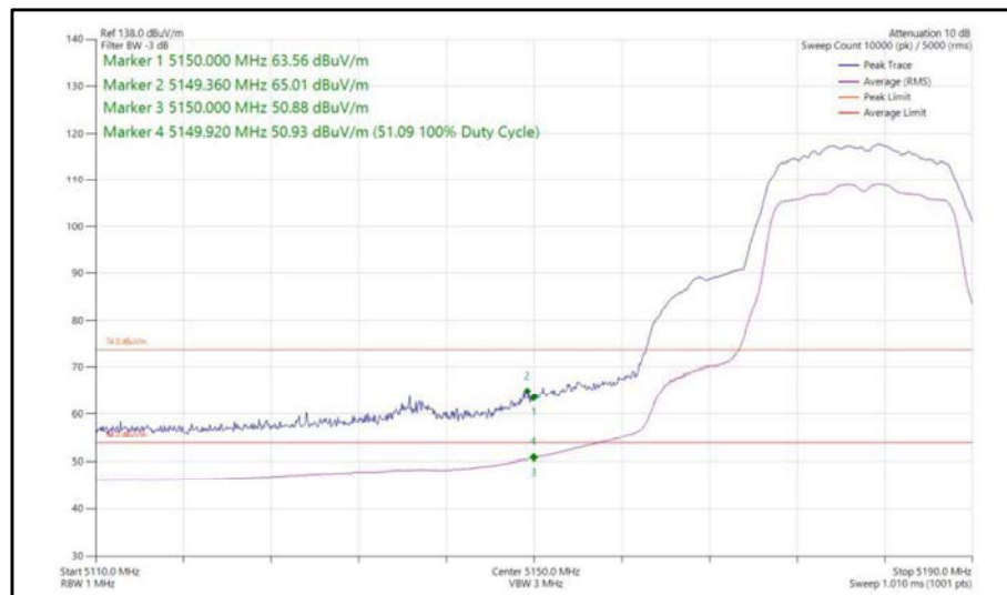
Figure 13 - 802.11a, SISO, Core 1 - 5180 MHz, Band Edge Frequency 5150 MHz
