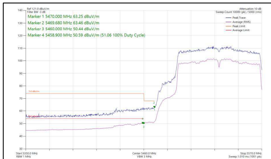
Figure 117 - 802.11ac, VHT80, CDD, Core 0-1 - 5530 MHz, Band Edge Frequency 5460 MHz
