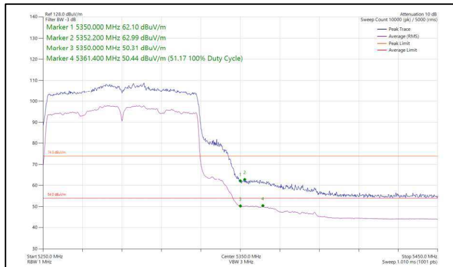
Figure 114 - 802.11ac, VHT80, CDD, Core 0-1 - 5290 MHz, Band Edge Frequency 5350 MHz
