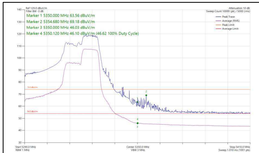
Figure 53 - 802.11ax, HE40, RU 106-56, SISO, Core 0 - 5310 MHz, Band Edge Frequency 5350 MHz
