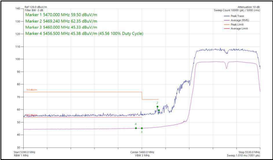
Figure 92 - 802.11ac, VHT40, TxBF, Core 0-1 - 5510 MHz, Band Edge Frequency 5460 MHz
