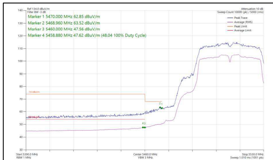
Figure 87 - 802.11n, HT40, SDM, Core 0-1 - 5510 MHz, Band Edge Frequency 5460 MHz
