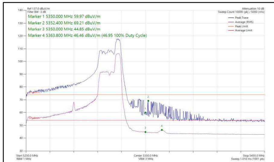
Figure 98 - 802.11ax, HE80, RU 52-52, SISO, Core 0 - 5290 MHz, Band Edge Frequency 5350 MHz
