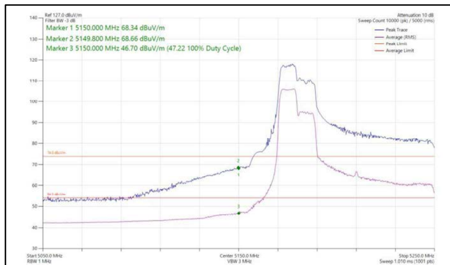
Figure 95 - 802.11ax, HE80, RU 106-53, SISO, Core 0 - 5210 MHz, Band Edge Frequency 5150 MHz
