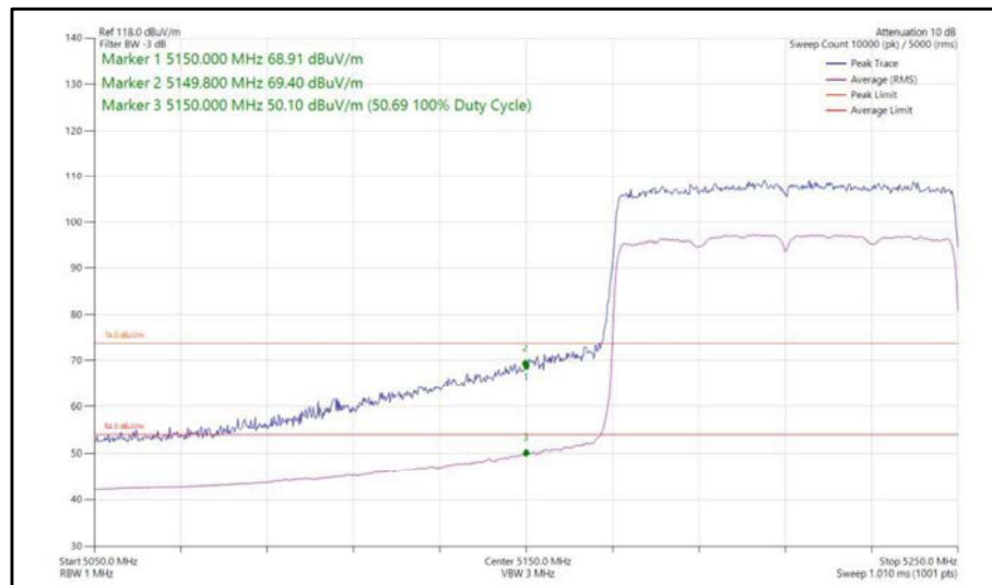
Figure 94 - 802.11ax, HE80, SU, SISO, Core 0 - 5210 MHz, Band Edge Frequency 5150 MHz
