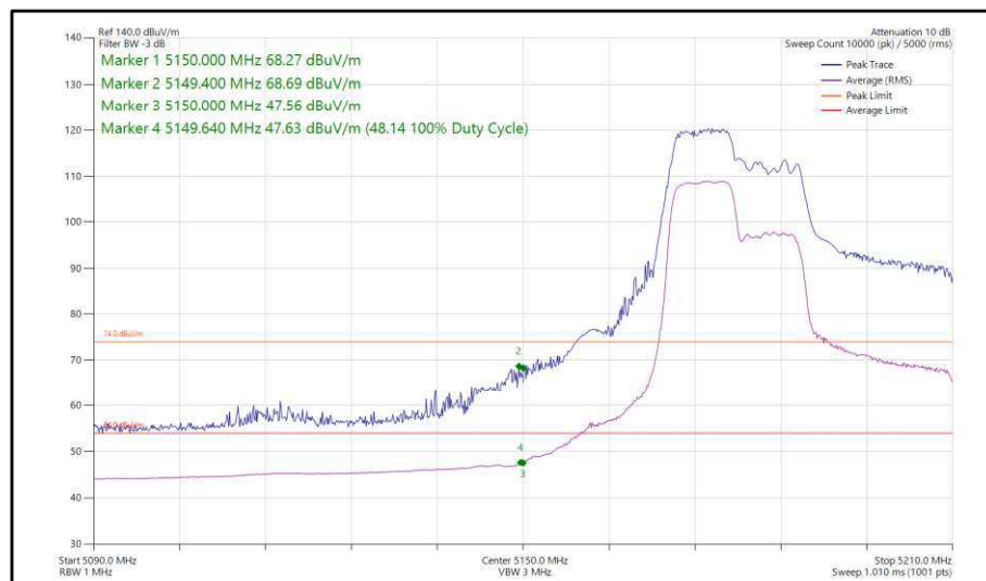
Figure 70 - 802.11ax, HE40, RU 106-53, CDD, Core 0-1 - 5190 MHz, Band Edge Frequency 5150 MHz
