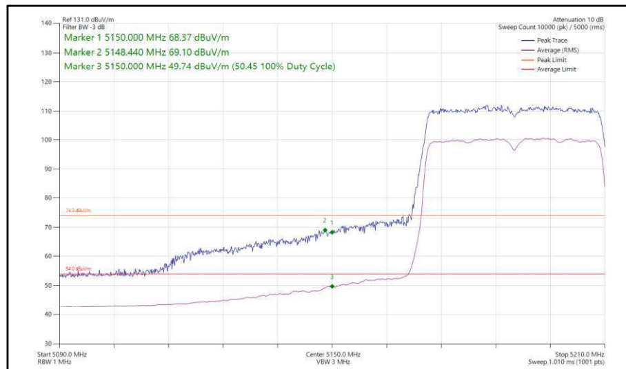
Figure 80 - 802.11ax, HE40, SU, SDM, Core 0-1 - 5190 MHz, Band Edge Frequency 5150 MHz
