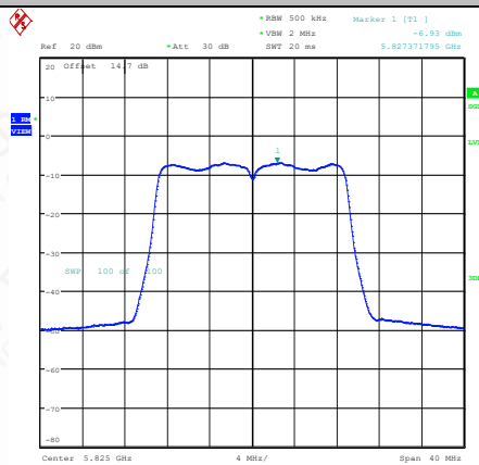
11N20MIMO-Ant1-5825-PASS
