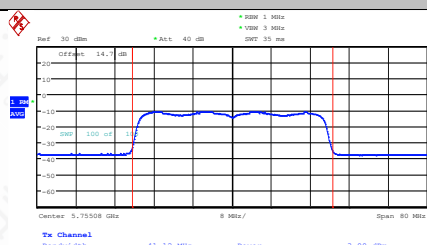
11AX40SISO-Ant1-5755-PASS
