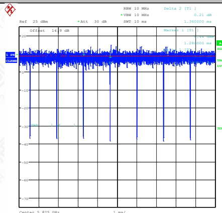
NTNV-11AC20SISO-Ant2-5825
