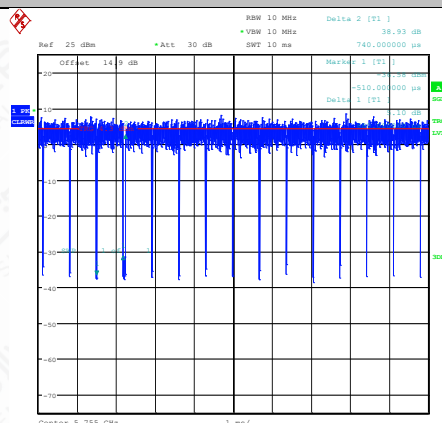
NTNV-11AC40SISO-Ant2-5755
