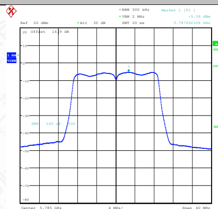
11N20SISO-Ant2-5785-PASS
