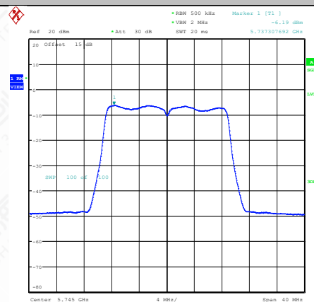
11N20SISO-Ant2-5745-PASS
