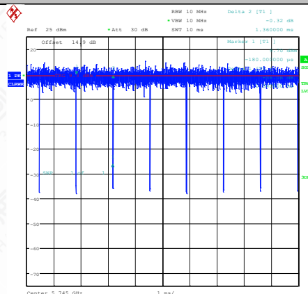
NTNV-11N20SISO-Ant2-5745
