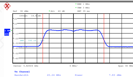
11N20MIMO-Ant2-5825-PASS
