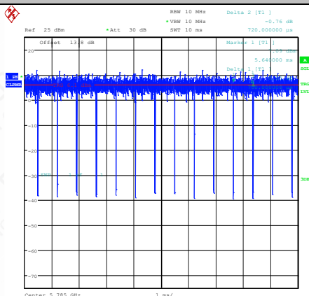
NTNV-11AC20MIMO-Ant1-5785
