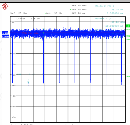
NTNV-11N20SISO-Ant1-5825
