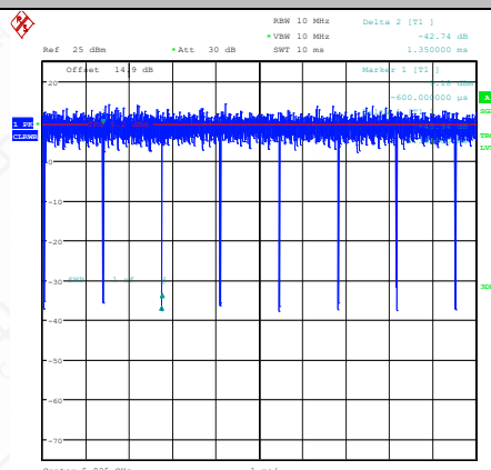
NTNV-11N20SISO-Ant2-5825
