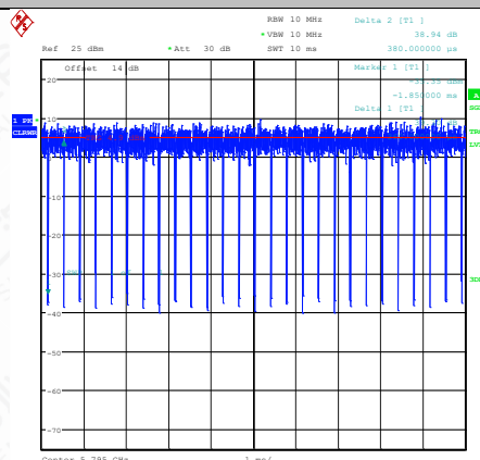
NTNV-11AC40MIMO-Ant2-5795
