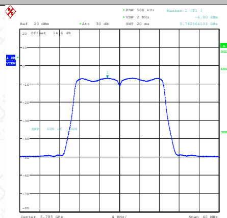
11N20SISO-Ant1-5785-PASS
