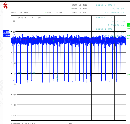
NTNV-11AX40MIMO-Ant2-5755
