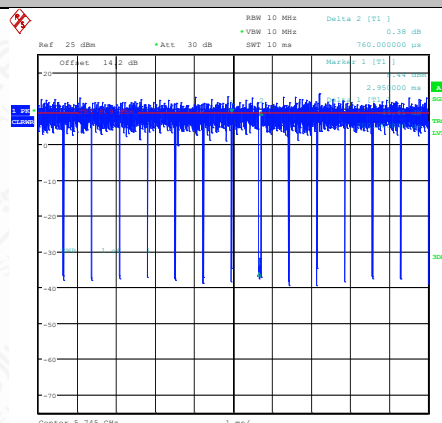
NTNV-11AC20MIMO-Ant2-5745
