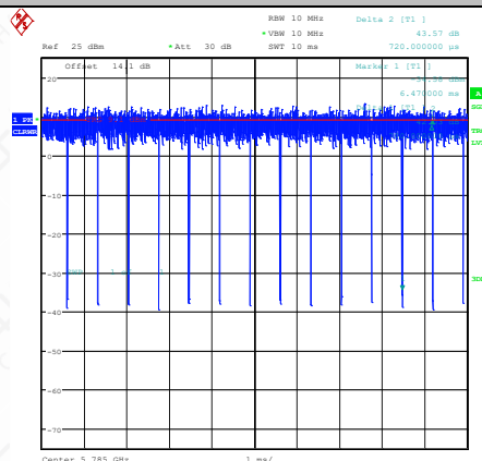
NTNV-11AC20MIMO-Ant2-5785
