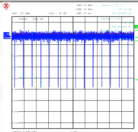
NTNV-11AC20MIMO-Ant2-5825
