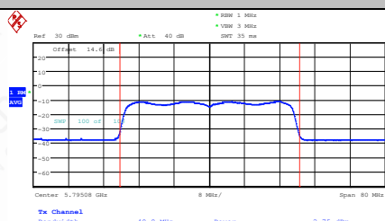
11AX40SISO-Ant1-5795-PASS
