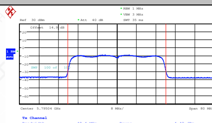
11AX40SISO-Ant2-5795-PASS
