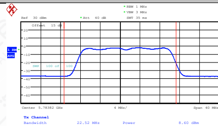
11N20MIMO-Ant2-5785-PASS
