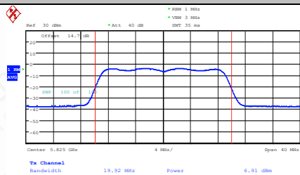
11N20MIMO-Ant1-5825-PASS
