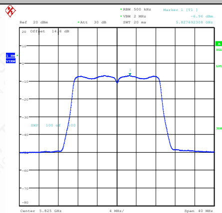
11N20SISO-Ant1-5825-PASS
