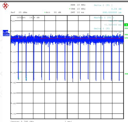
NTNV-11AC40SISO-Ant1-5795
