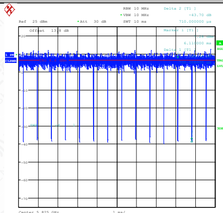
NTNV-11AC20MIMO-Ant1-5825
