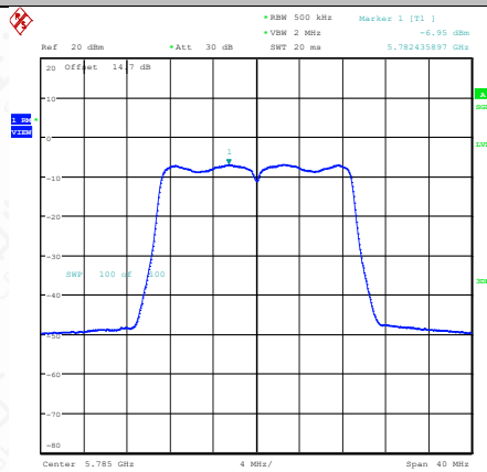
11N20MIMO-Ant1-5785-PASS
