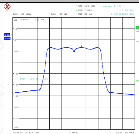
11N20SISO-Ant2-5825-PASS
