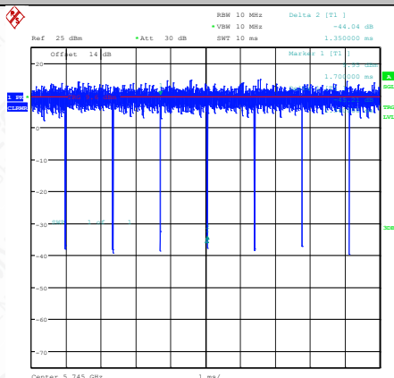
NTNV-11N20SISO-Ant1-5745
