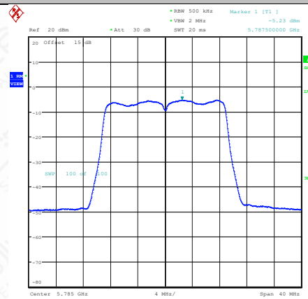
11N20MIMO-Ant2-5785-PASS
