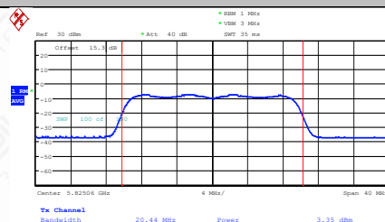
11AX20MIMO-Ant2-5825-PASS
