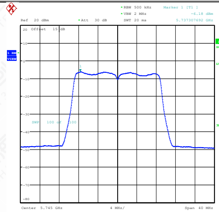
11N20MIMO-Ant2-5745-PASS
