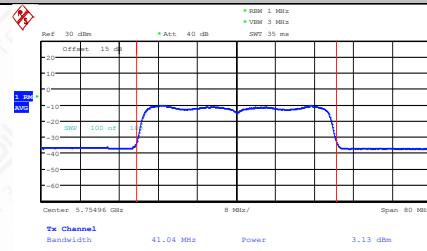
11AX40MIMO-Ant2-5755-PASS
