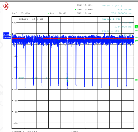
NTNV-11AC40SISO-Ant2-5795
