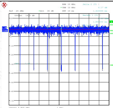
NTNV-11AC20SISO-Ant1-5825
