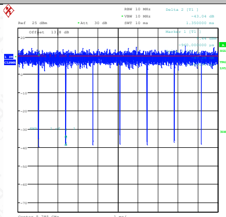
NTNV-11N20SISO-Ant1-5785
