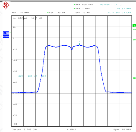
11N20MIMO-Ant1-5745-PASS
