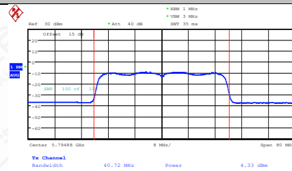
11AX40MIMO-Ant2-5795-PASS
