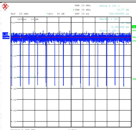
NTNV-11AC20MIMO-Ant1-5745
