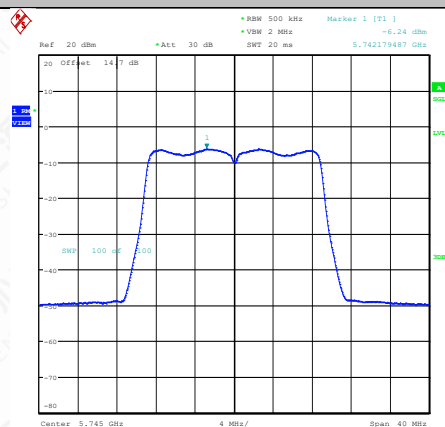
11N20SISO-Ant1-5745-PASS
