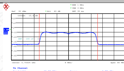
11AX40SISO-Ant2-5755-PASS
