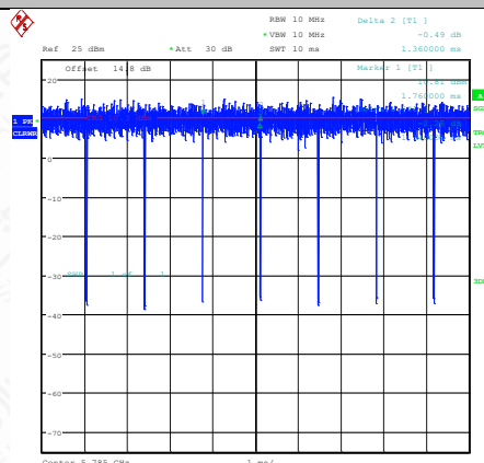
NTNV-11N20SISO-Ant2-5785
