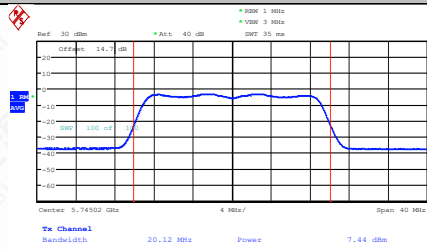
11N20MIMO-Ant1-5745-PASS
