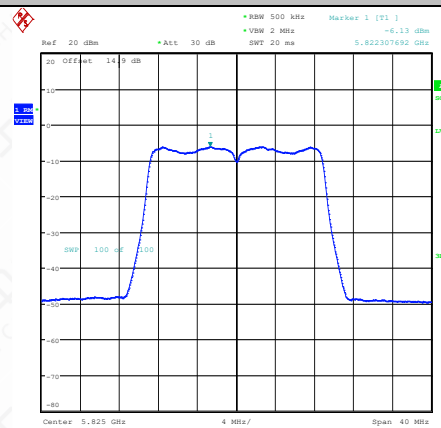
11N20MIMO-Ant2-5825-PASS
