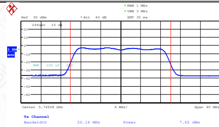
11N20MIMO-Ant2-5745-PASS
