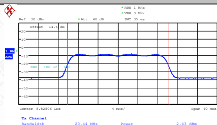
11AX20MIMO-Ant1-5825-PASS
