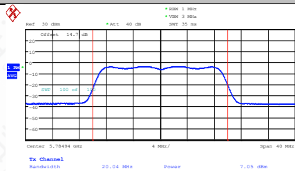
11N20MIMO-Ant1-5785-PASS
