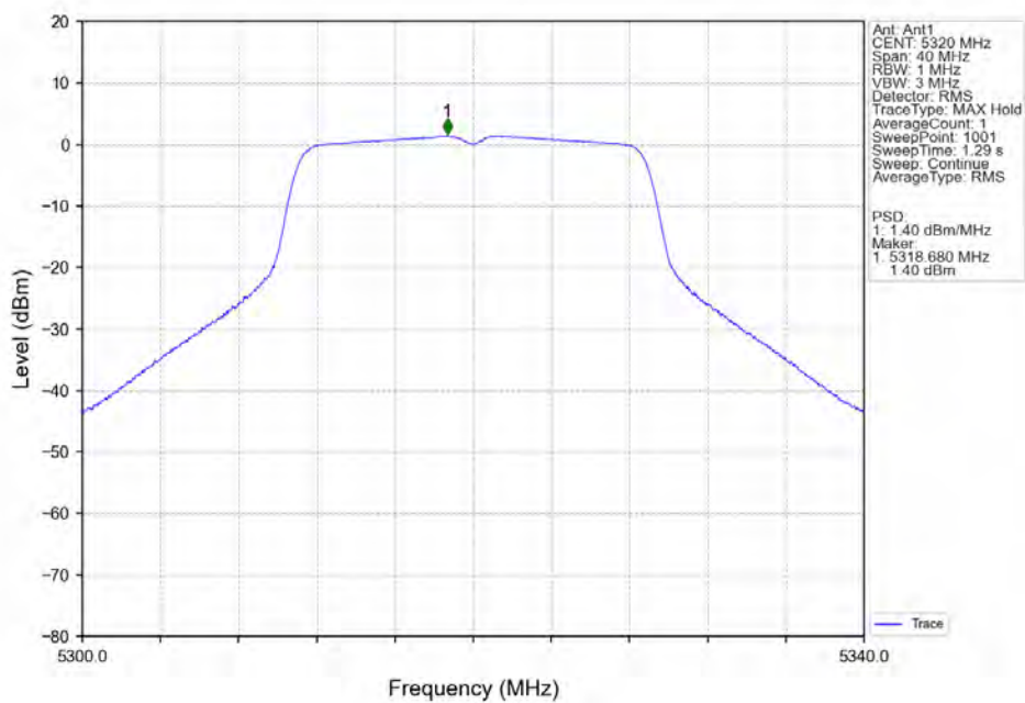
802.11ac(VHT20)_HCH_5320MHz_Ant1_NTNV
