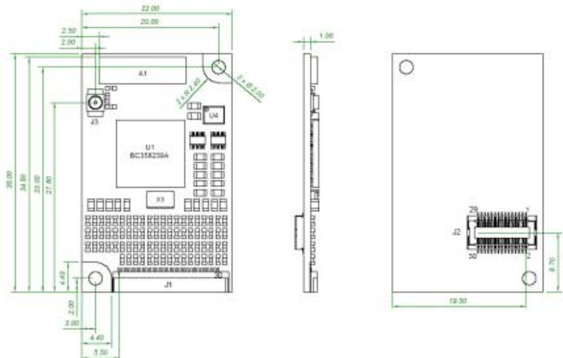
Figure 3 - PCB outline
