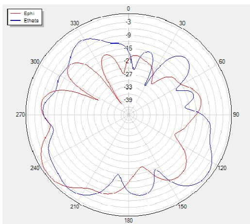
Phi=90 freq=5500MHz
