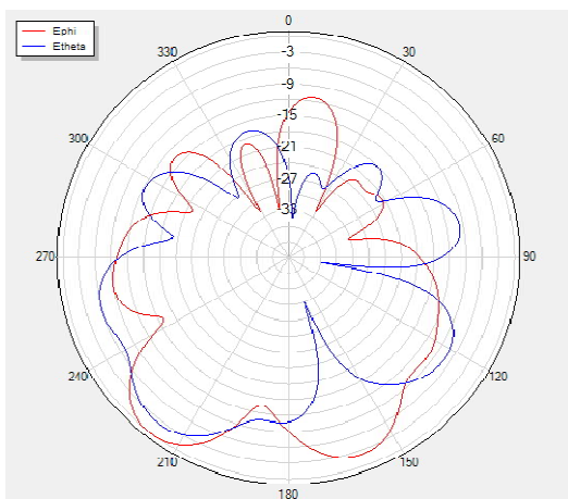
Theta=90 freq=5350MHz
