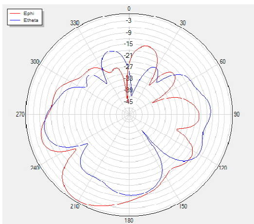
Theta=90 freq=5500MHz
