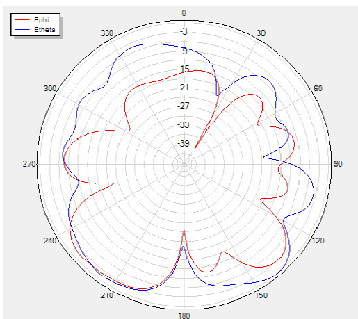
Phi=90 freq=5350MHz
