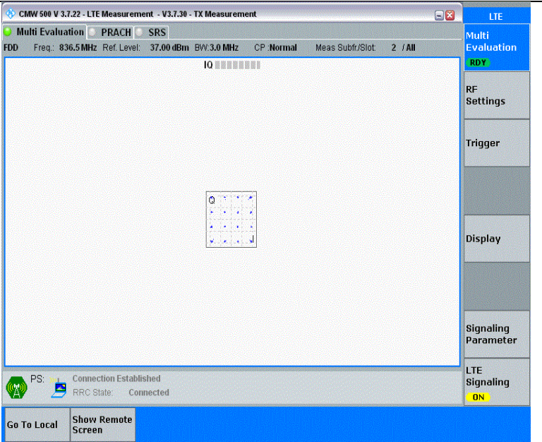
Band26(824-849)-3MHz-16QAM-26915-15RB#0-PASS
