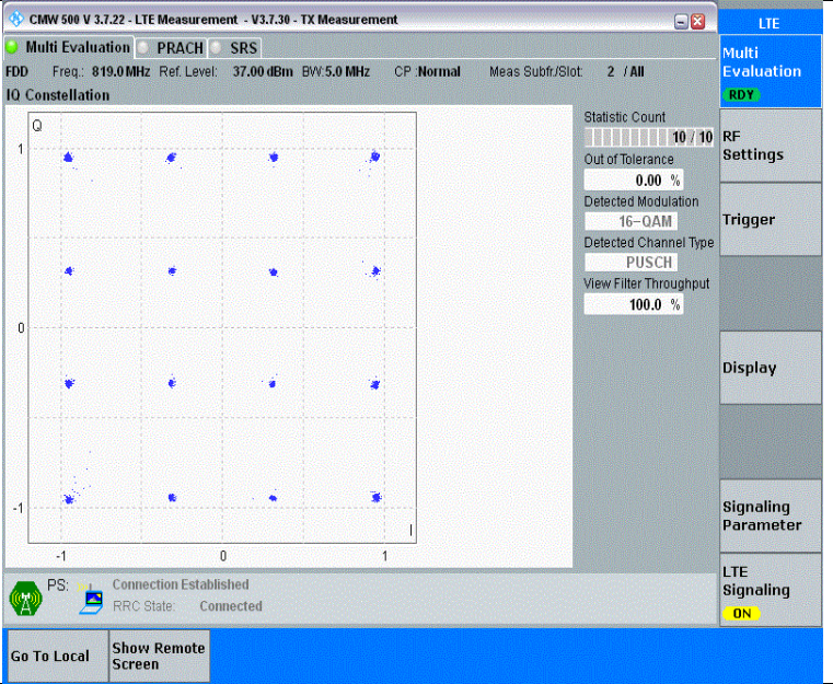
Band26(814-824)-5MHz-16QAM-26740-25RB#0-PASS
