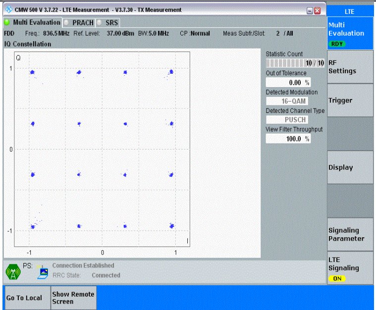
Band26(824-849)-5MHz-16QAM-26915-25RB#0-PASS
