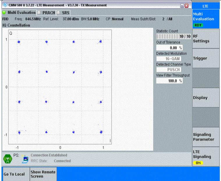
Band26(824-849)-5MHz-16QAM-27015-25RB#0-PASS
