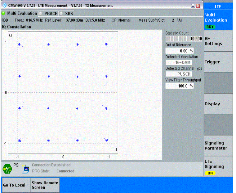
Band26(814-824)-5MHz-16QAM-26715-25RB#0-PASS
