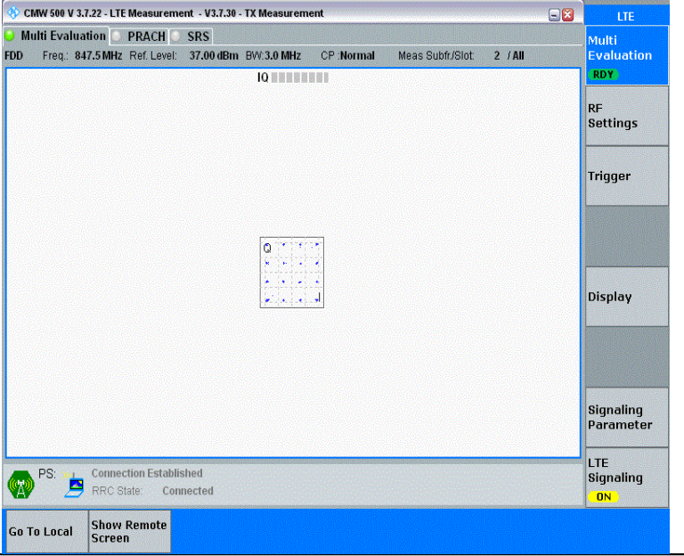
Band26(824-849)-3MHz-16QAM-27025-15RB#0-PASS
