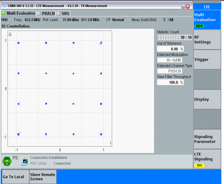
Band26(814-824)-3MHz-16QAM-26775-15RB#0-PASS
