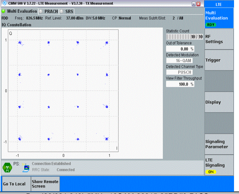
Band26(824-849)-5MHz-16QAM-26815-25RB#0-PASS
