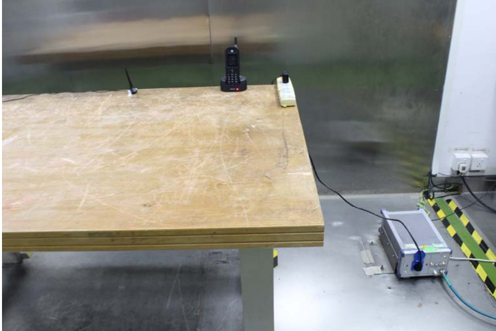
Conducted Emissions - Front View(Adapter 2)
