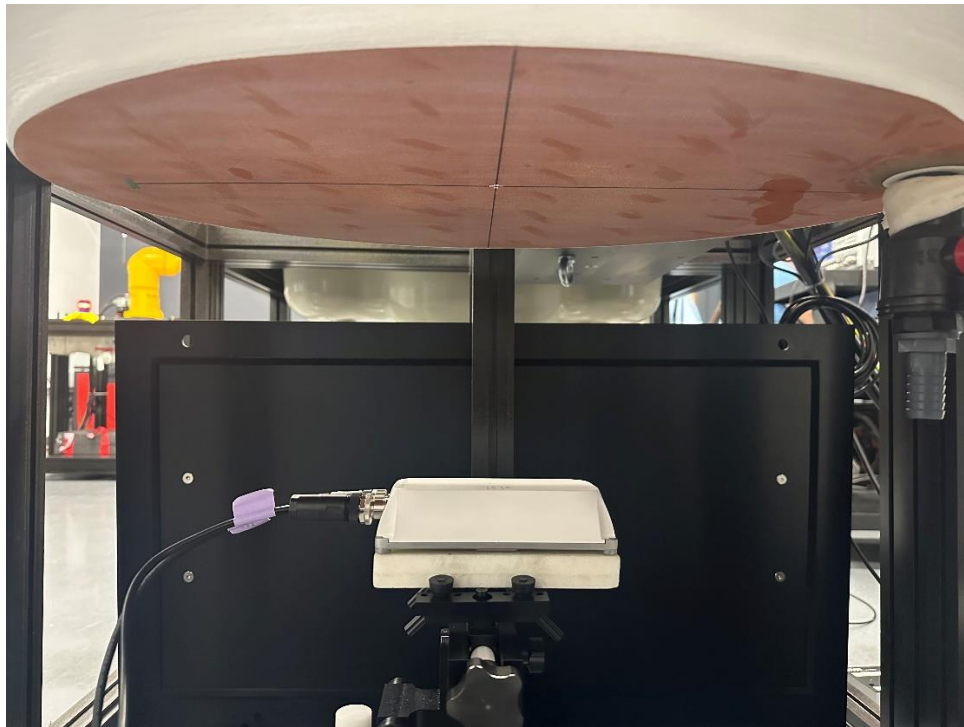
Figure A SAR Test Setup – Body/Whole Body – Front 200mm
