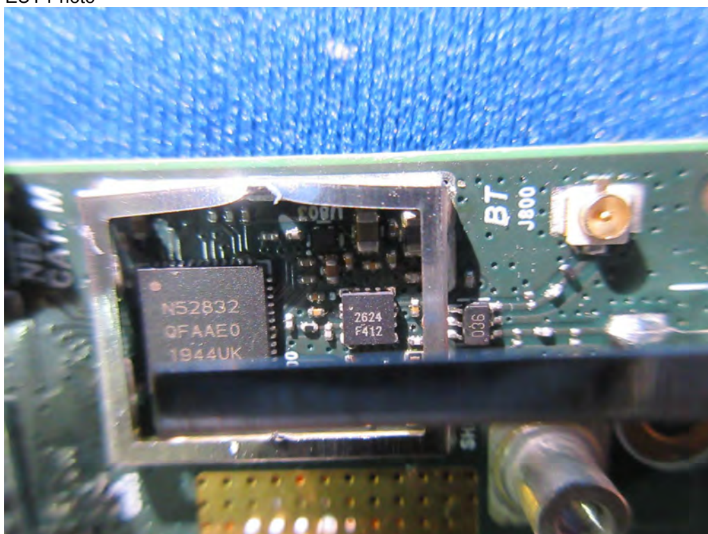
(32) EUT Photo
