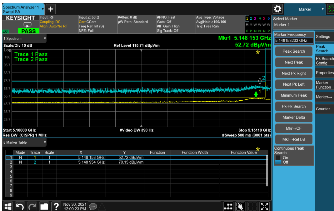
Graph 9: Radiated Lower Band Edge Plot – ac Mode 40 MHz
