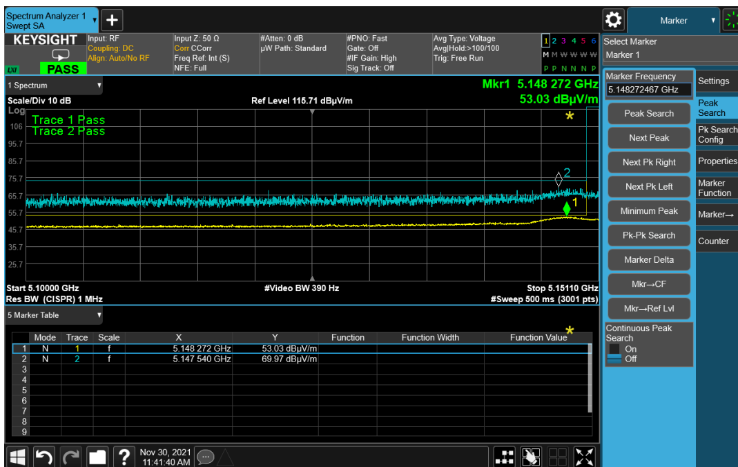
Graph 5: Radiated Lower Band Edge Plot – n Mode 40 MHz
