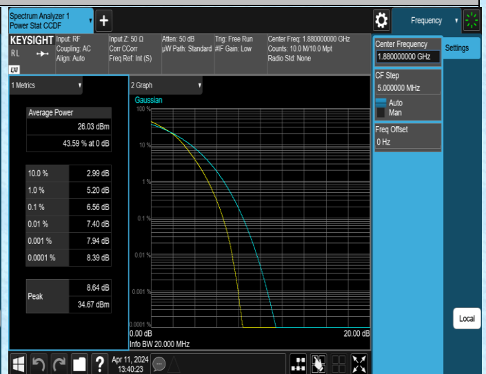
Band2-20MHz-16QAM-18900-100RB#0-PASS
