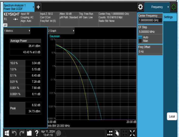
Band2-20MHz-16QAM-19100-100RB#0-PASS
