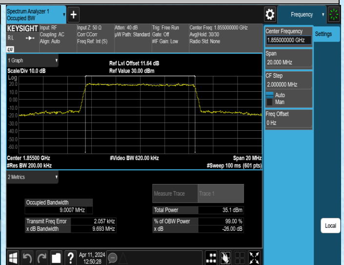
Band2-10MHz-16QAM-18650-50RB#0-PASS
