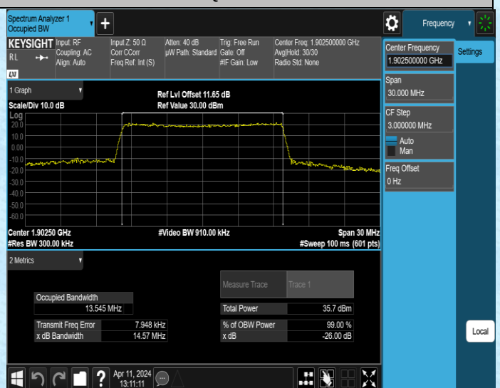
Band2-15MHz-16QAM-19125-75RB#0-PASS
