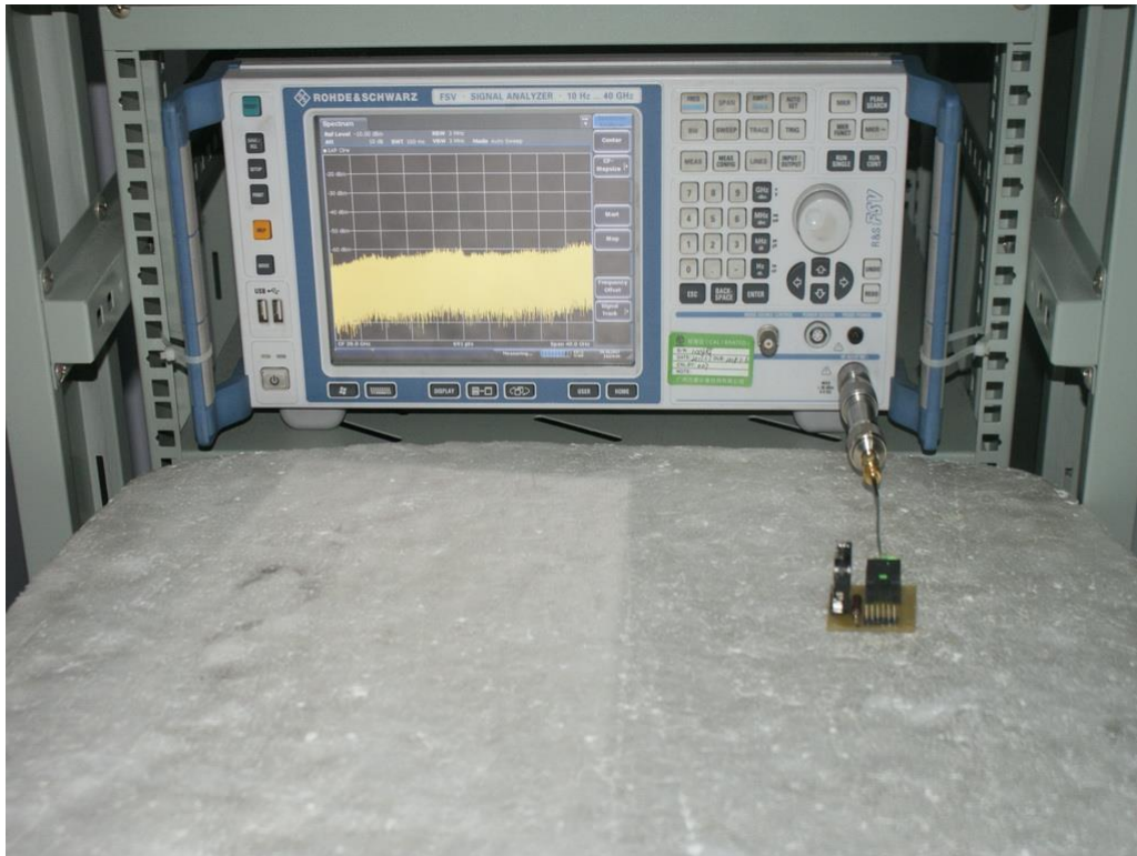
Photograph 1: Set-up for Radio Spectrum Test
