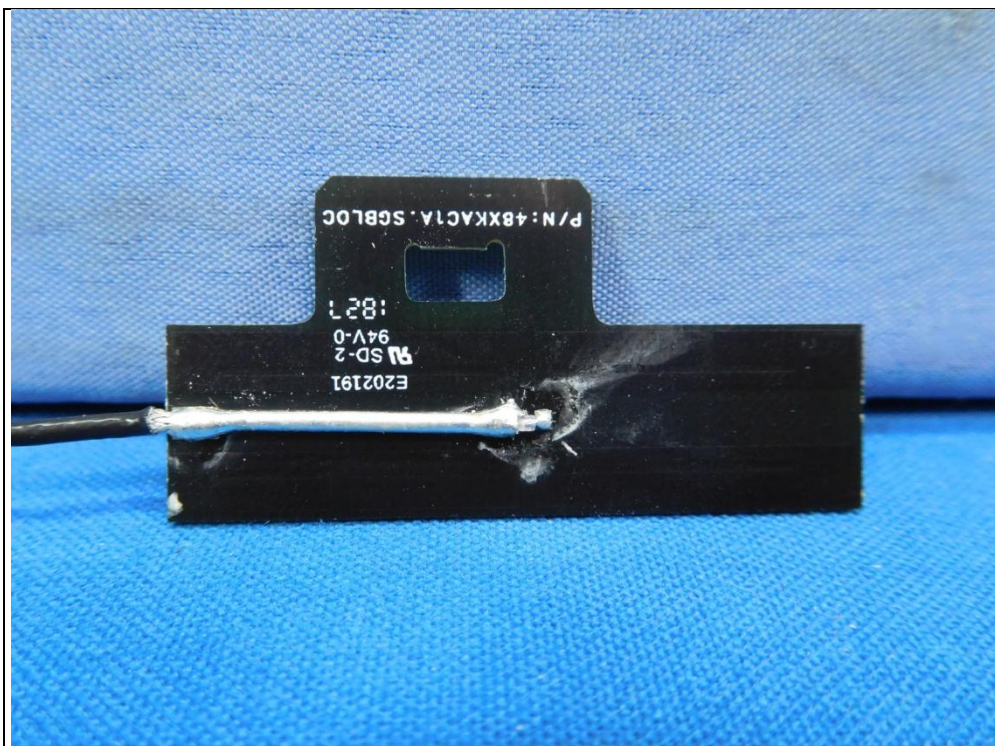
Antenna: Dual1
