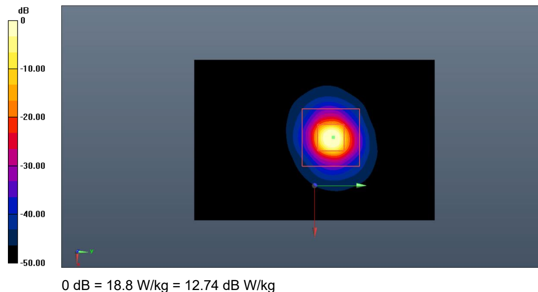
Fig.B.14. Validation 5750MHz 100mW
