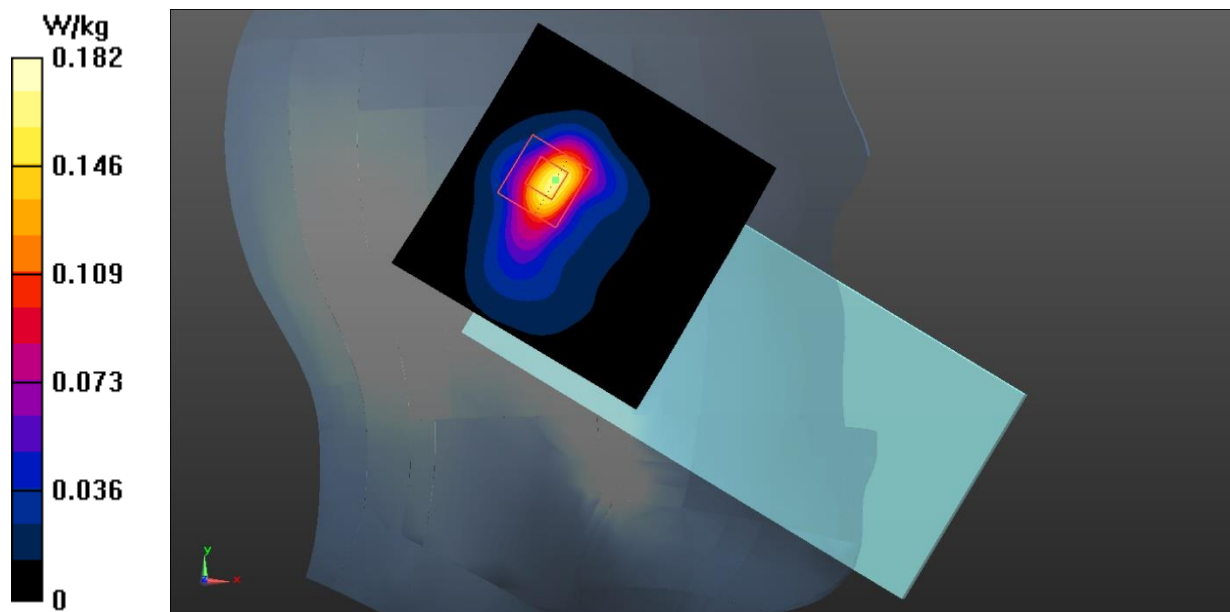
Fig.39 Bluetooth Head
