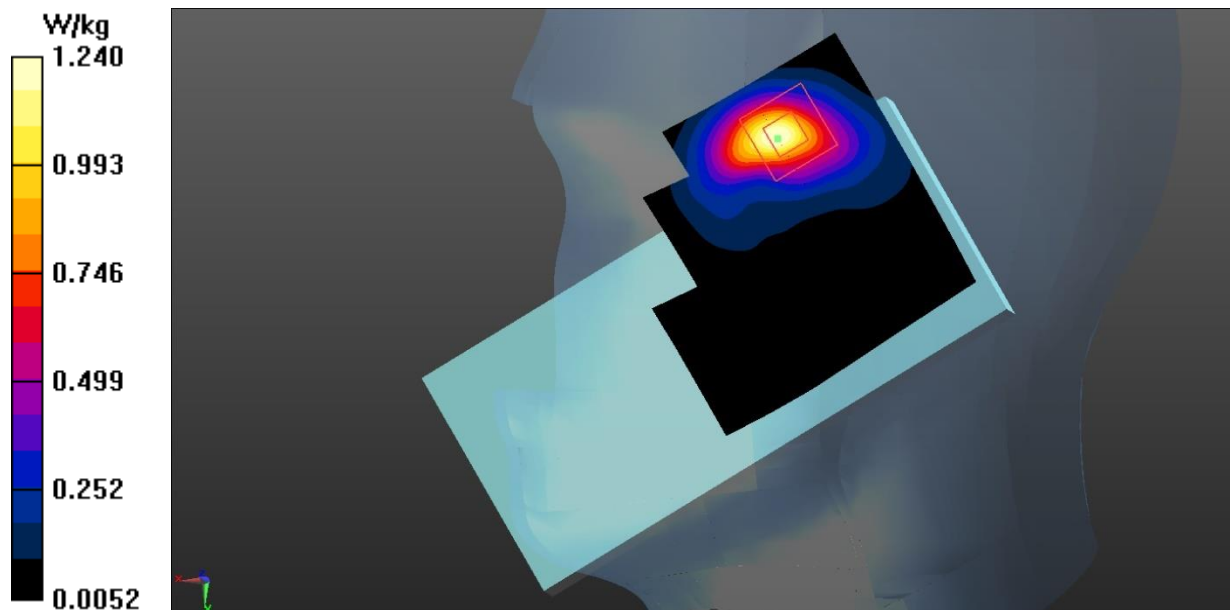
Fig.13 LTE Band 4 Head
