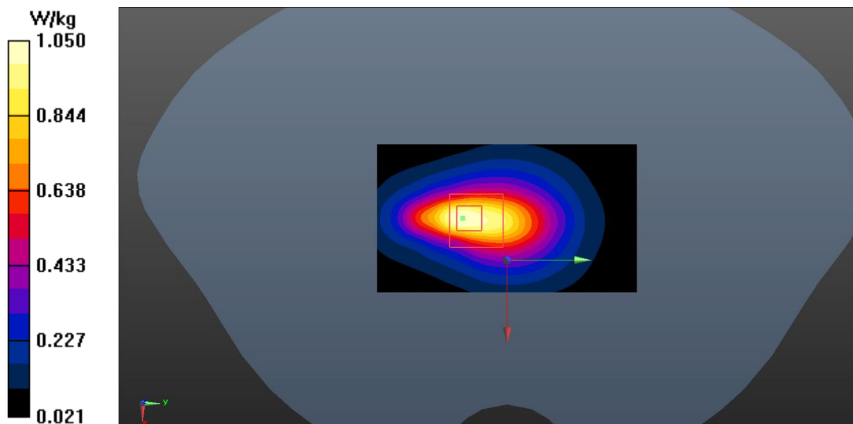
Fig.28 LTE Band 66 Body
