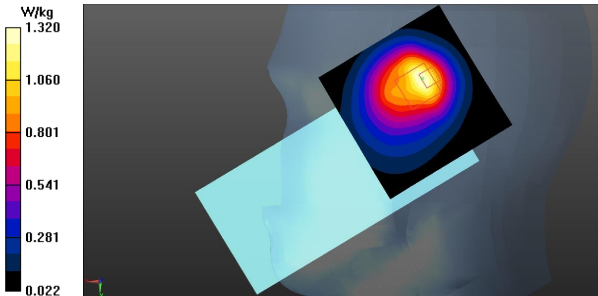
Fig.21 LTE Band 26 Head
