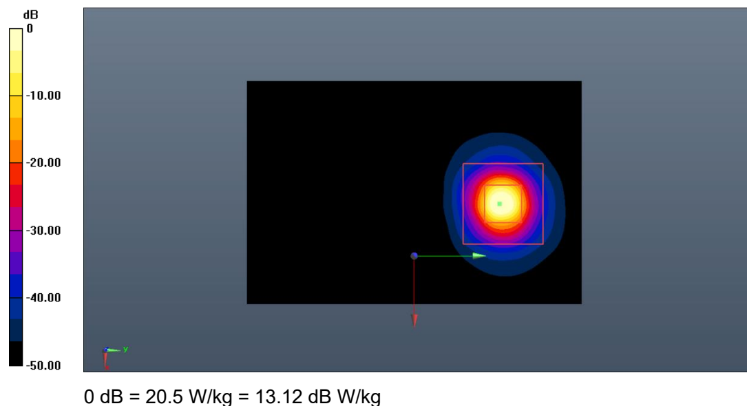
Fig.B.13. Validation 5600MHz 100mW
