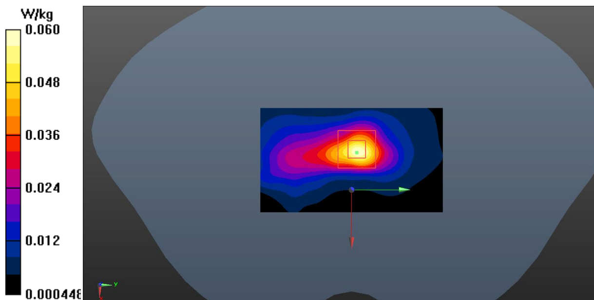
Fig.40 Bluetooth Body
