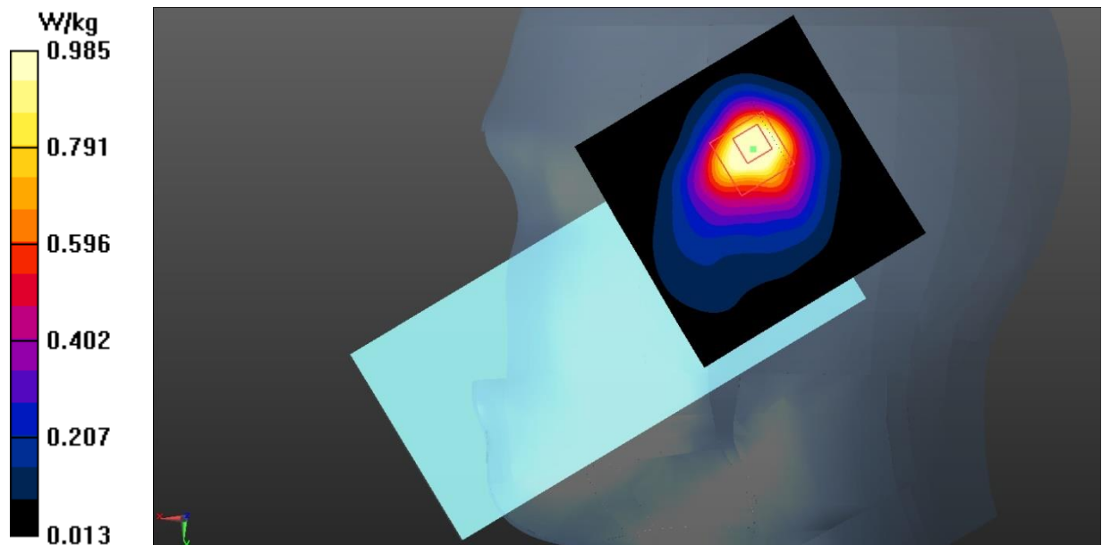
Fig.27 LTE Band 66 Head
