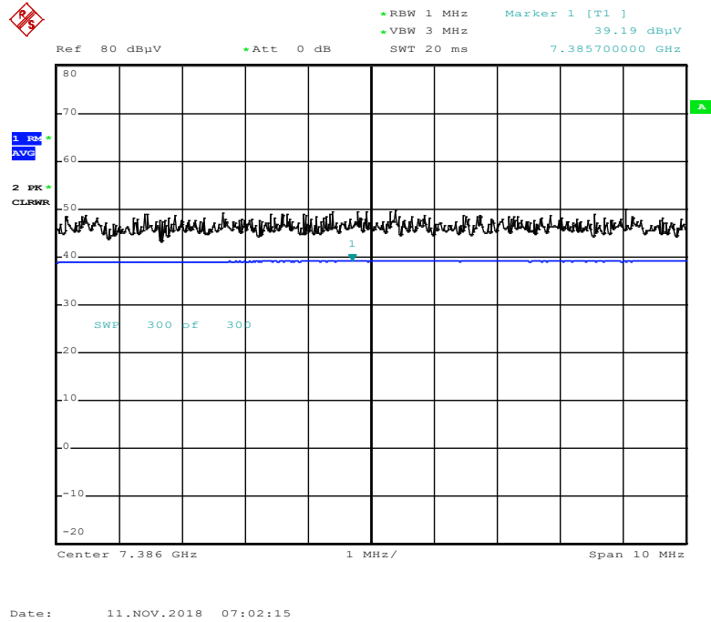
Radiated Spurious Emissions plot – Average Reading (802.11b, Ch.11 3rd Harmonic)
