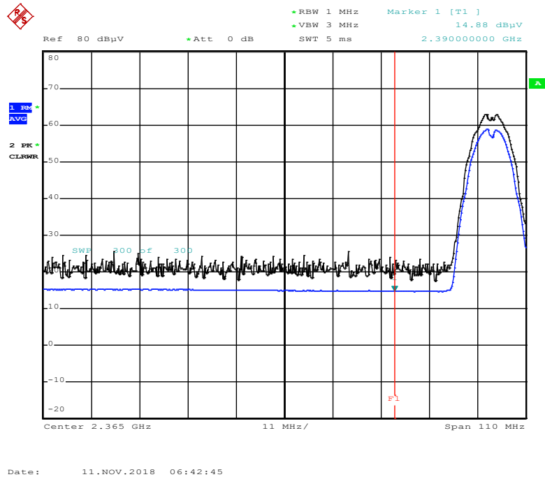
Radiated Restricted Band Edges plot – Average Reading (802.11b Ch.1)
