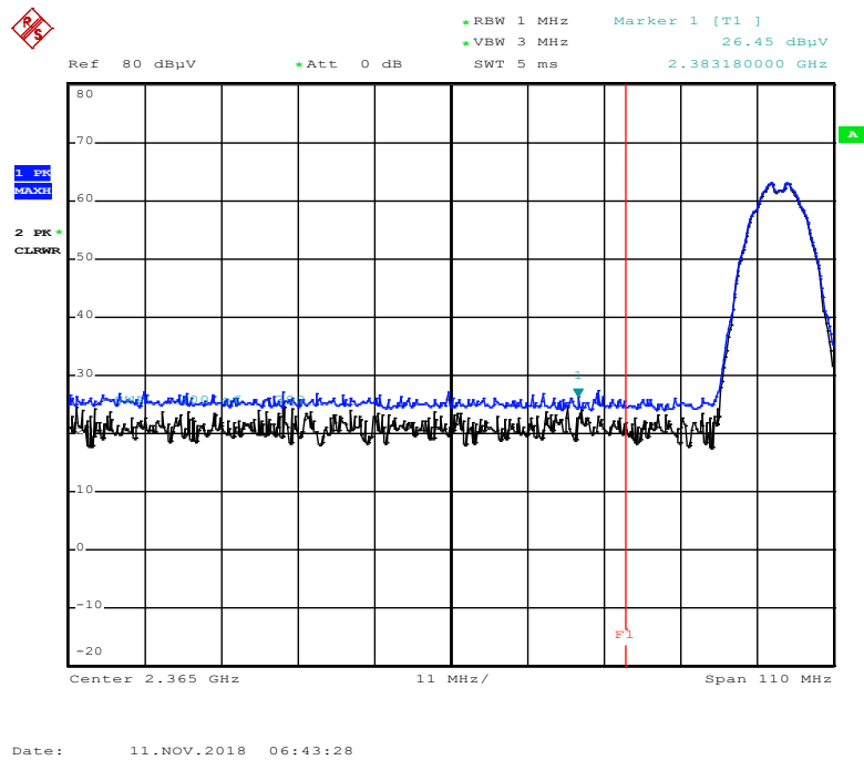
Radiated Restricted Band Edges plot – Peak Reading (802.11b Ch.1)
