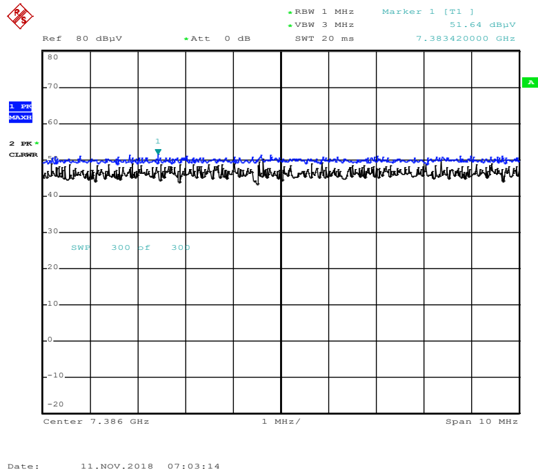
Radiated Spurious Emissions plot – Peak Reading (802.11b, Ch.11 3rd Harmonic)
