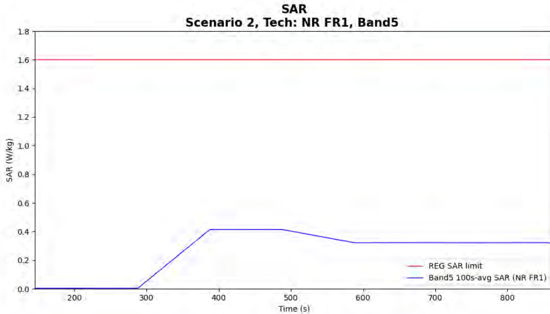
Figure 6-4 Time-averaged SAR for case 7 in table 6-1 (sub6 NR n5)
