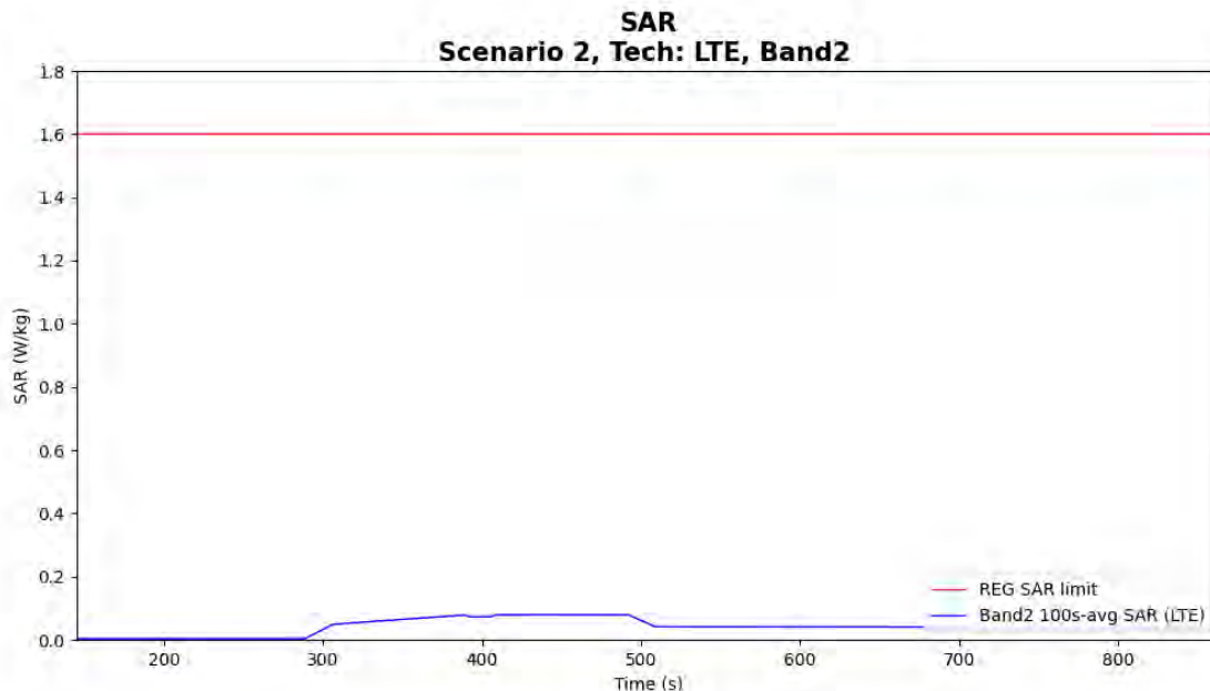
Figure 6-7 Time-averaged SAR for case 4 in table 6-1 (LTE B2)
