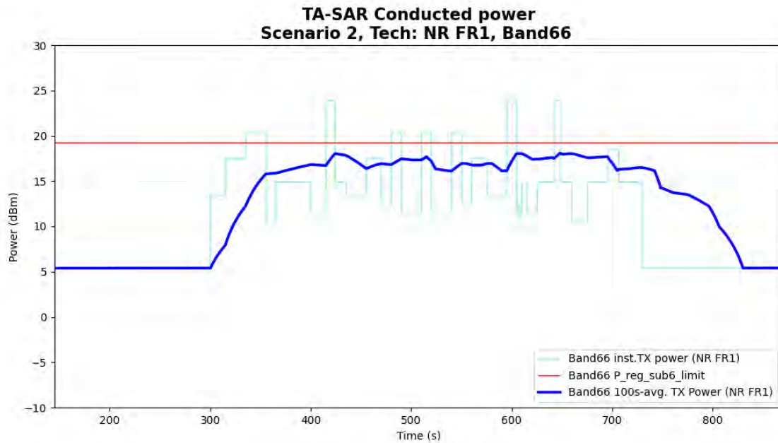
Figure 5- 14 Time-averaged conducted TX power over time for case 13 (sub6 NR n66)
