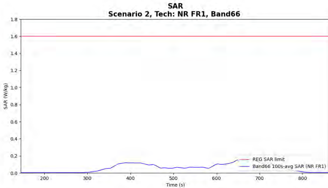
Figure 6-5 Time-averaged SAR for case 13 in table 6-1 (sub6 NR n66)
