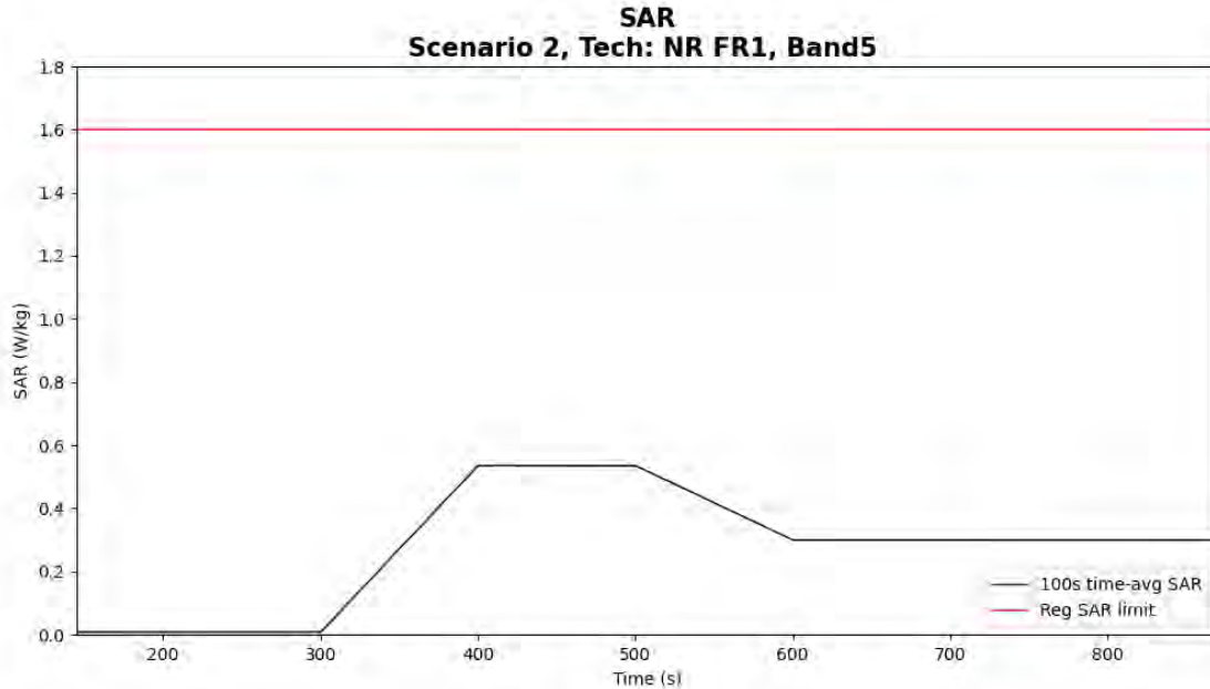
Figure 5- 13 Time-averaged SAR for case 7 (sub6 NR n5)
