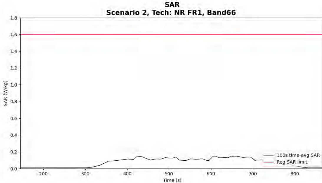
Figure 5- 15 Time-averaged SAR for case 13 (sub6 NR n66)
