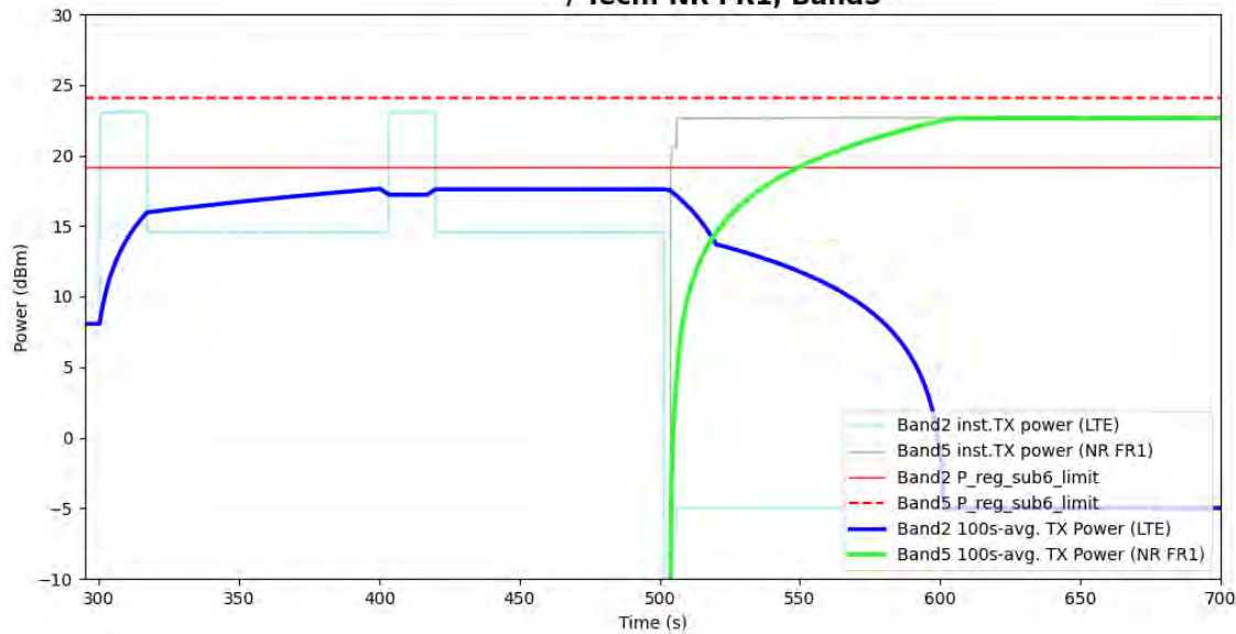
Figure 5- 44 Time-averaged conducted TX power over time for case 16 (LTE B2, sub6 NR B5)
