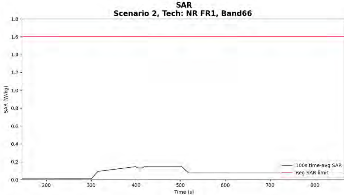
Figure 5- 11 Time-averaged SAR for case 6 (sub6 NR n66)
