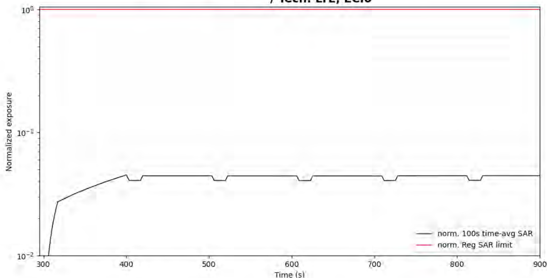
Figure 5- 47 Normalized time-averaged SAR for case 17 (LTE B2)
