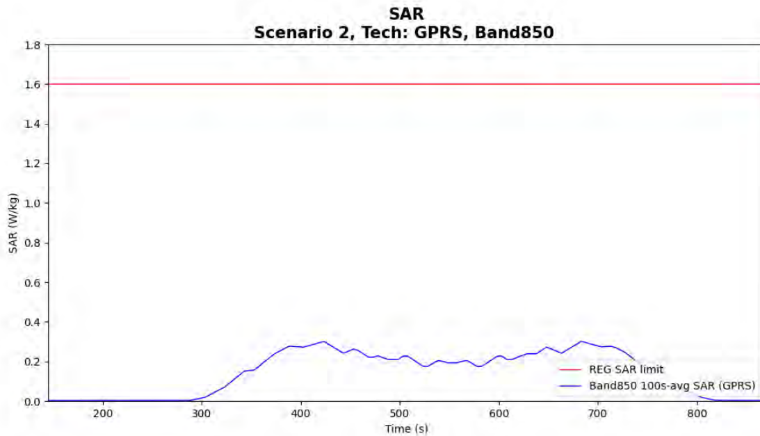
Figure 6-18 Time-averaged SAR for case 8 in table 6-1 (2G GPRS 850 4Tx)
