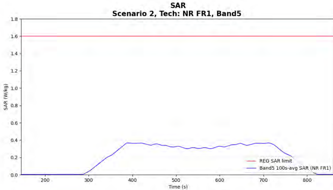
Figure 6-6 Time-averaged SAR for case 14 in table 6-1 (sub6 NR n5)
