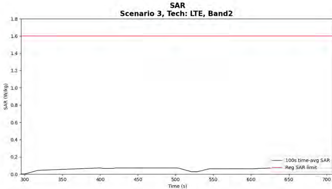
Figure 5- 43 Time-averaged SAR for case 15 (LTE B2)
