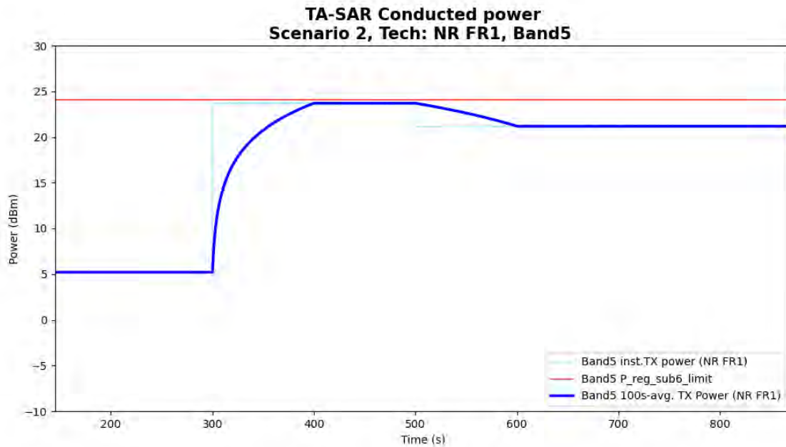
Figure 5- 12 Time-averaged conducted TX power over time for case 7 (sub6 NR n5)
