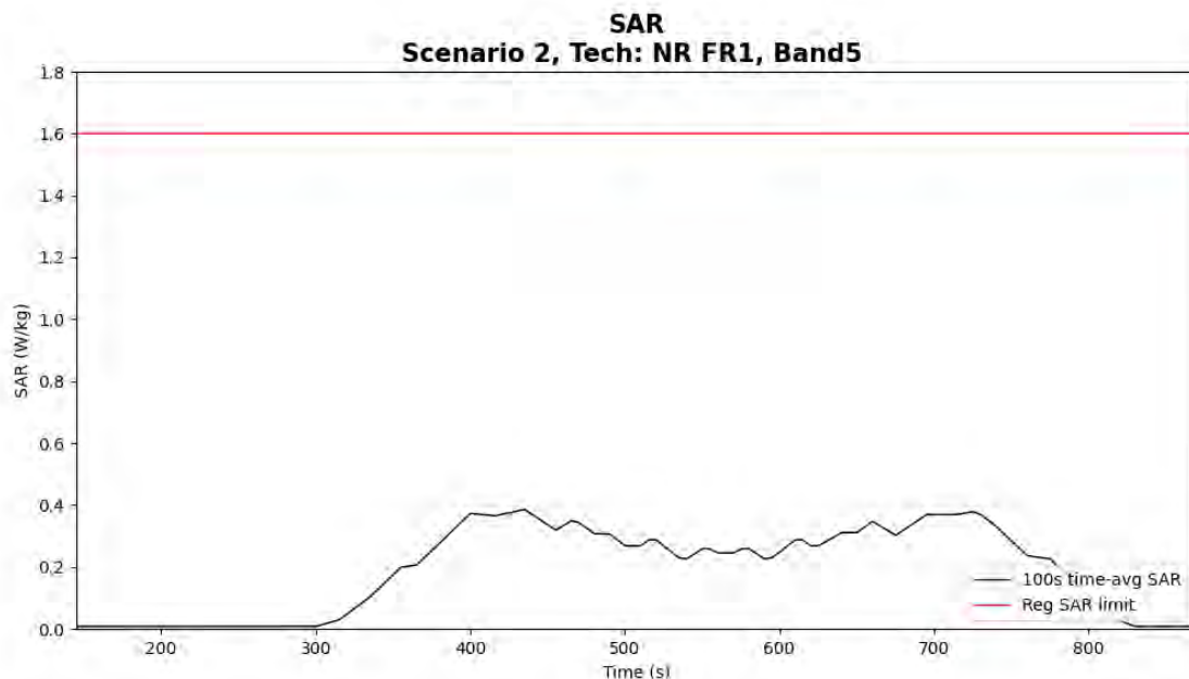
Figure 5- 17 Time-averaged SAR for case 14 (sub6 NR n5)
