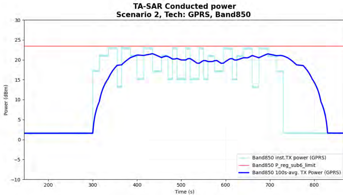
Figure 5- 40 Time-averaged conducted TX power over time for case 8 (2G GPRS 850 4Tx)
