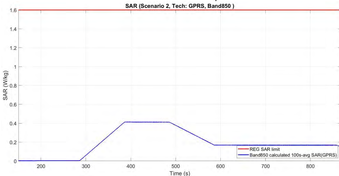
Figure 6-17 Time-averaged SAR for case 1 in table 6-1 (2G GPRS 850 4Tx)
