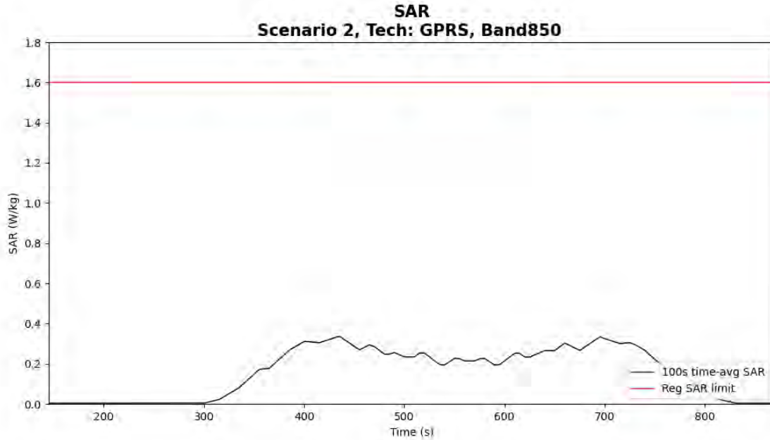
Figure 5- 41 Time-averaged SAR for case 8 (2G GPRS 850 4Tx)
