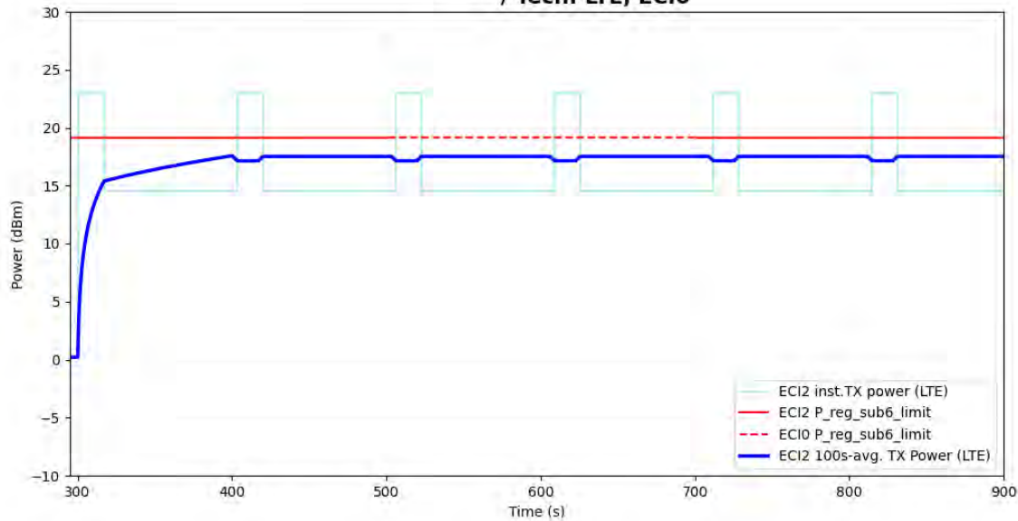
Figure 5- 46 Time-averaged conducted TX power over time for case 17 (LTE B2)
