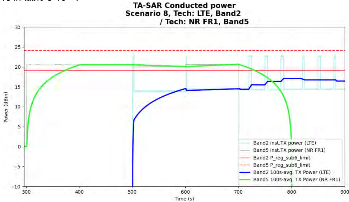
Figure 5- 54 Time-averaged conducted TX power over time for case 18 (LTE B2, sub6 NR n5)
