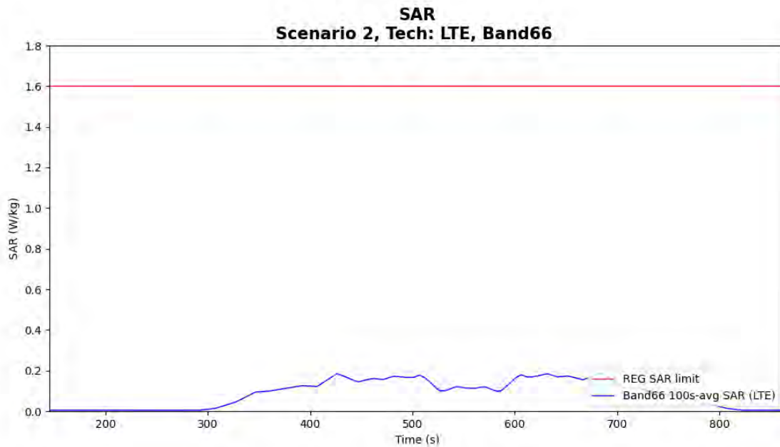
Figure 6-10 Time-averaged SAR for case 12 in table 6-1 (LTE B66)
