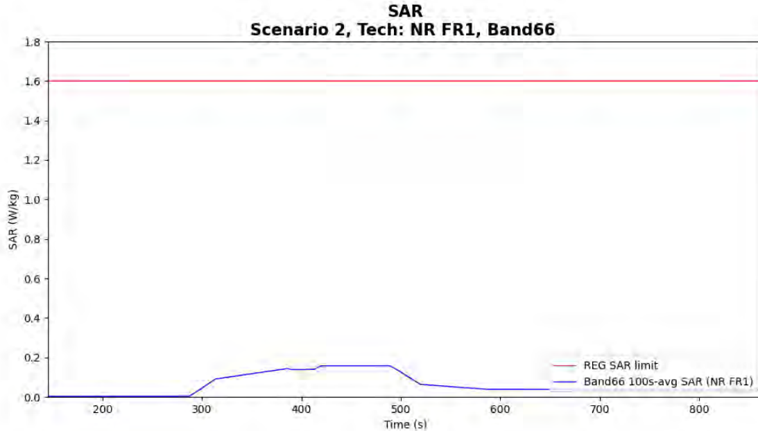
Figure 6-3 Time-averaged SAR for case 6 in table 6-1 (sub6 NR n66)
