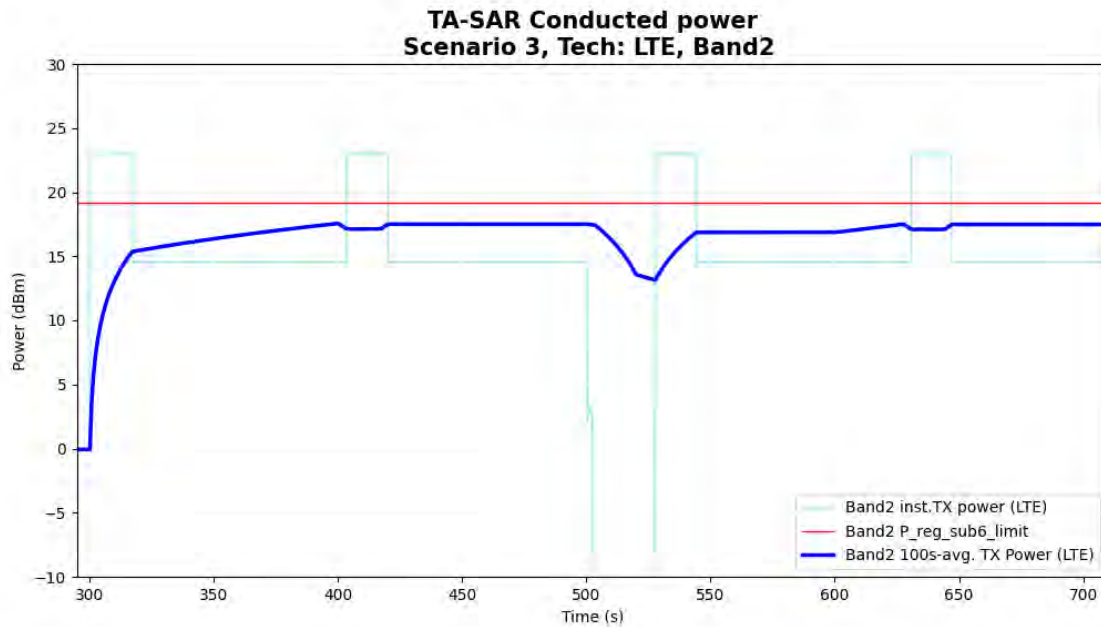
Figure 5- 42 Time-averaged conducted TX power over time for case 15 (LTE B2)
