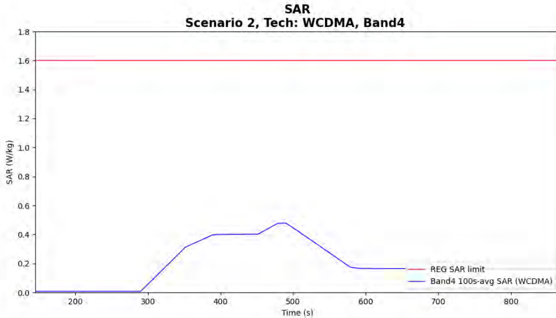
Figure 6-12 Time-averaged SAR for case 3 in table 6-1 (WCDMA B4)
