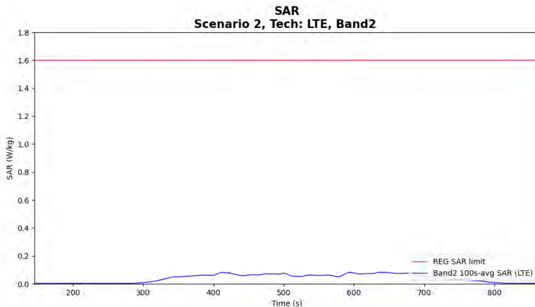
Figure 6-9 Time-averaged SAR for case 11 in table 6-1 (LTE B2)
