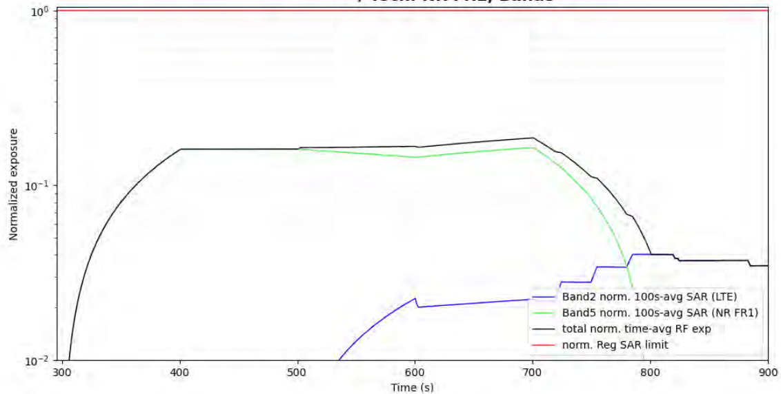
Figure 5- 55 Normalized time-averaged SAR for case 18 (LTE B2, sub6 NR n5)
