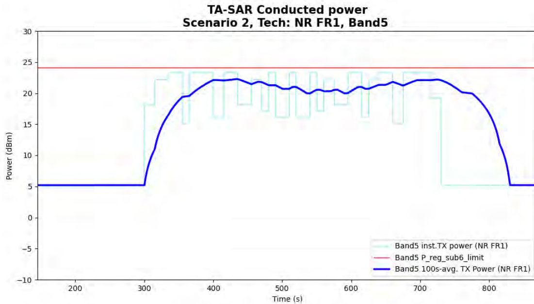
Figure 5- 16 Time-averaged conducted TX power over time for case 14 (sub6 NR n5)
