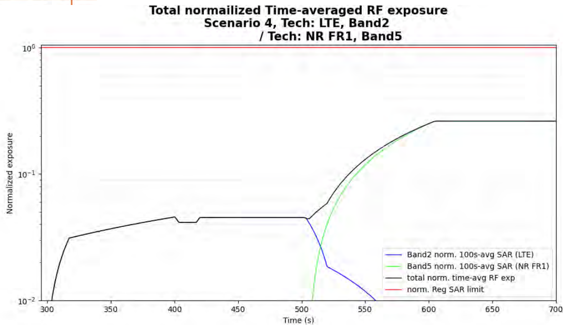
Figure 5- 45 Normalized time-averaged SAR for case 16 (LTE B2, sub6 NR B5)
