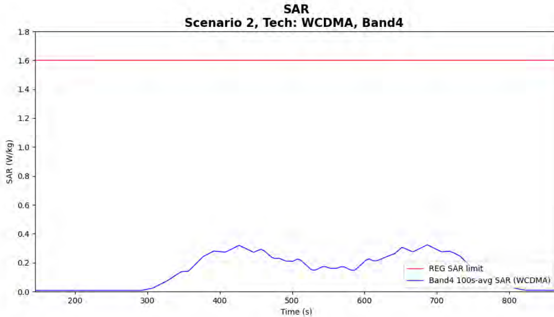
Figure 6-14 Time-averaged SAR for case 10 in table 6-1 (WCDMA B4)
