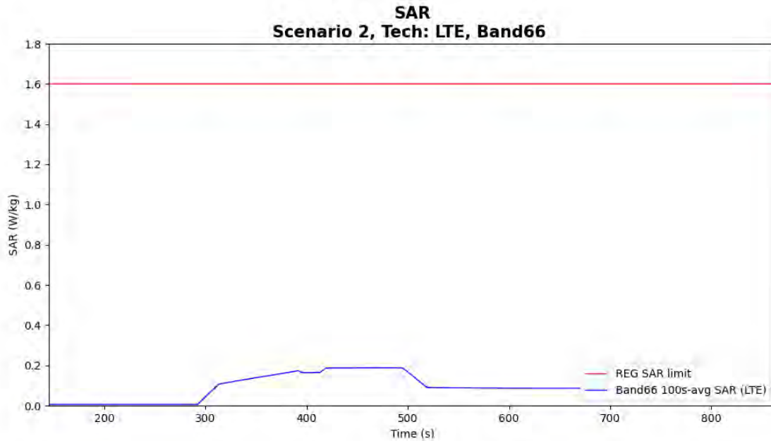
Figure 6-8 Time-averaged SAR for case 5 in table 6-1 (LTE B66)
