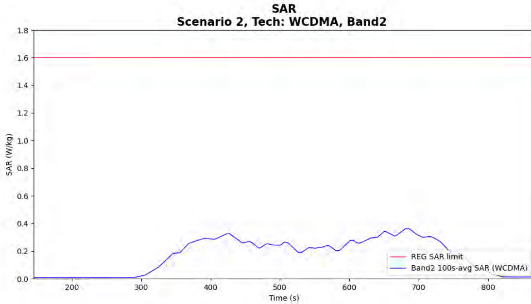
Figure 6-13 Time-averaged SAR for case 9 in table 6-1 (WCDMA B2)
