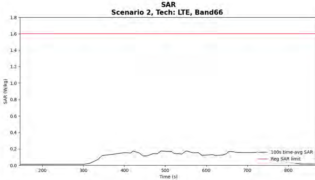
Figure 5- 25 Time-averaged SAR for case 12 (LTE B66)
