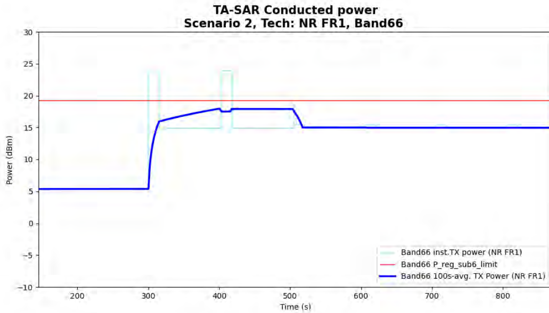
Figure 5- 10 Time-averaged conducted TX power over time for case 6 (sub6 NR n66)
