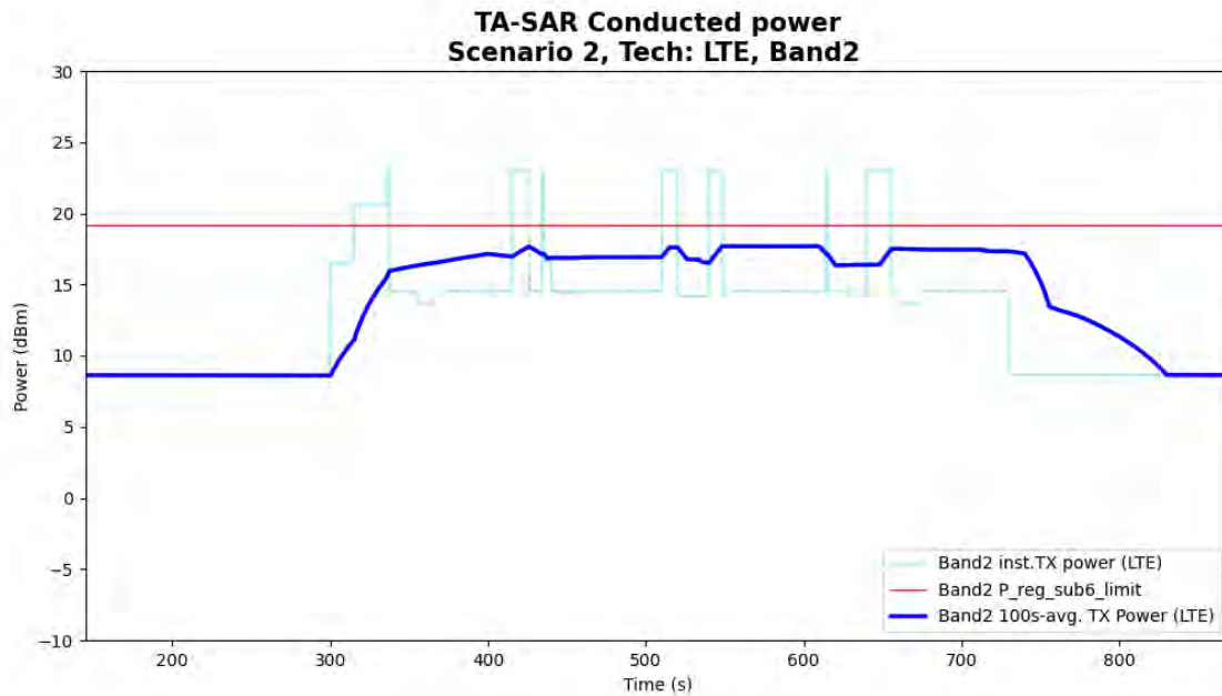
Figure 5- 22 Time-averaged conducted TX power over time for case 11 (LTE B2)
