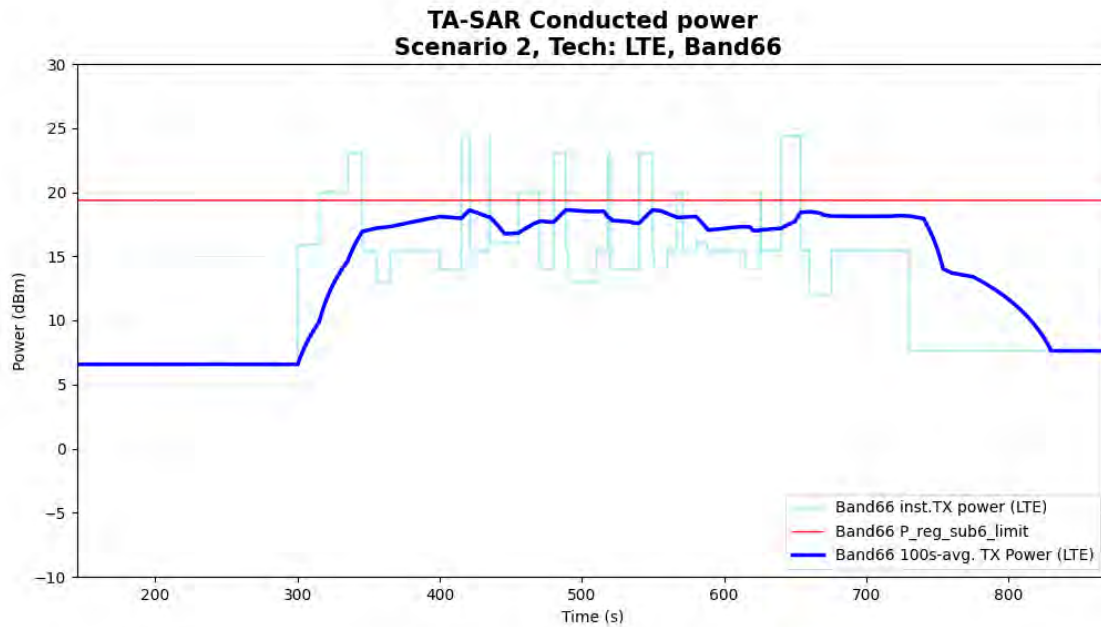
Figure 5- 24 Time-averaged conducted TX power over time for case 12 (LTE B66)
