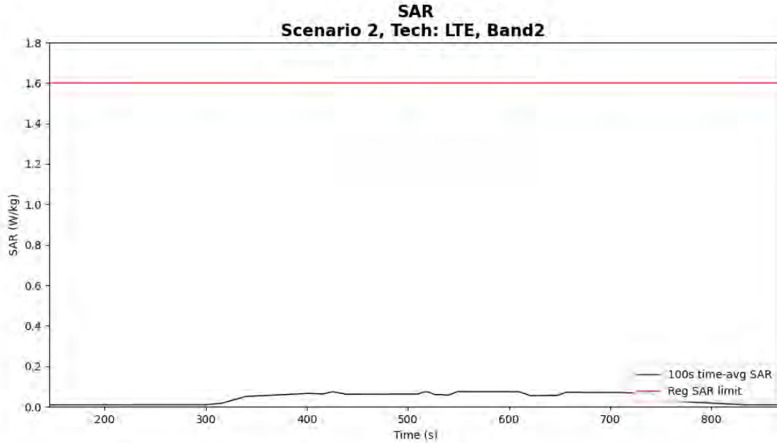
Figure 5- 23 Time-averaged SAR for case 11 (LTE B2)
