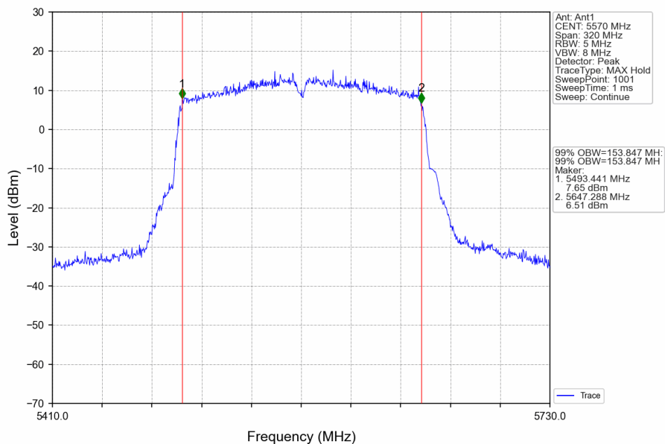
802.11ac(VHT160)_MCH_5570MHz_Ant1_NTNV
