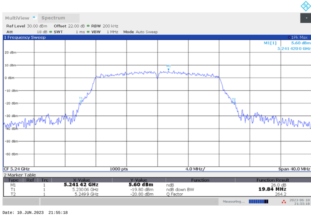
Fig.3 Occupied 26dB Bandwidth (802.11a, 5240MHz)
