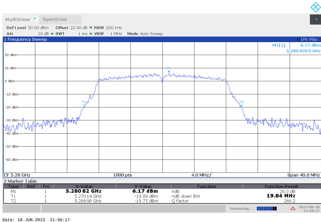
Fig.5 Occupied 26dB Bandwidth (802.11a, 5280MHz)
