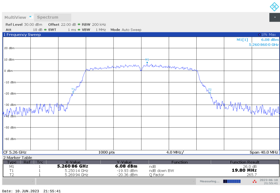
Fig.4 Occupied 26dB Bandwidth (802.11a, 5260MHz)
