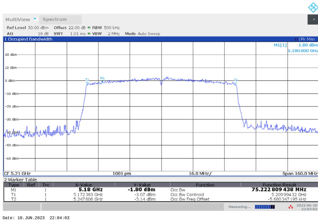
Fig.39 99% Occupied bandwidth (802.11ac-HT80, 5210MHz)
