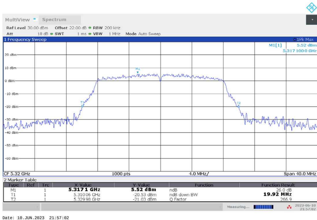
Fig.6 Occupied 26dB Bandwidth (802.11a, 5320MHz)
