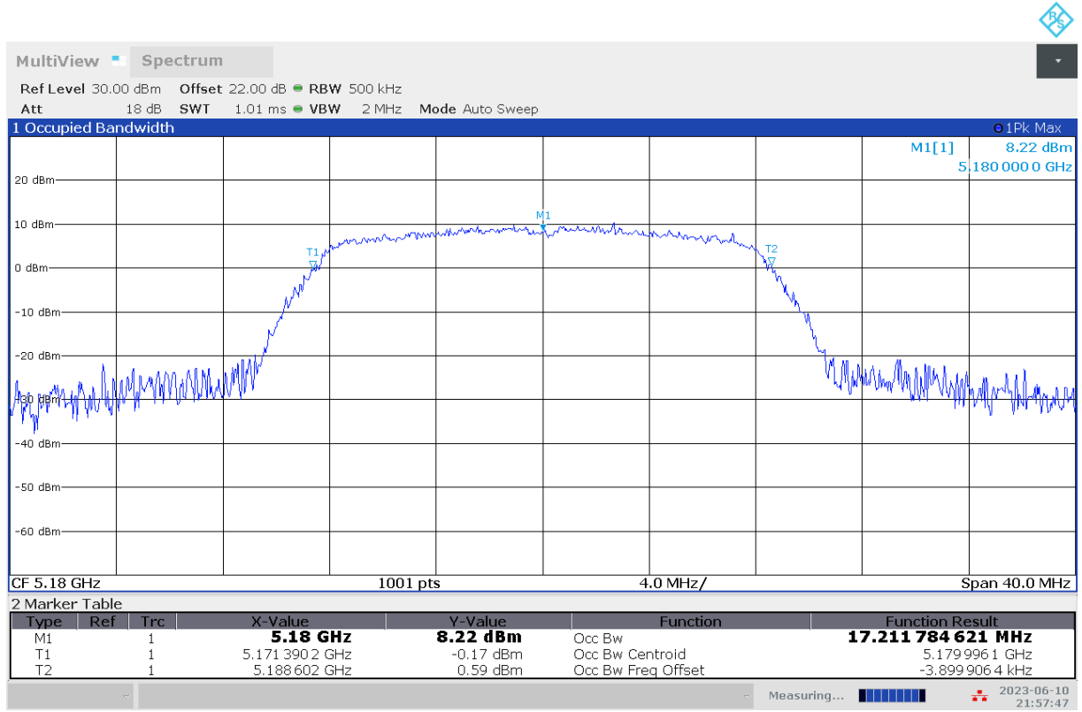
Fig.31 99% Occupied bandwidth (802.11a, 5180MHz)
