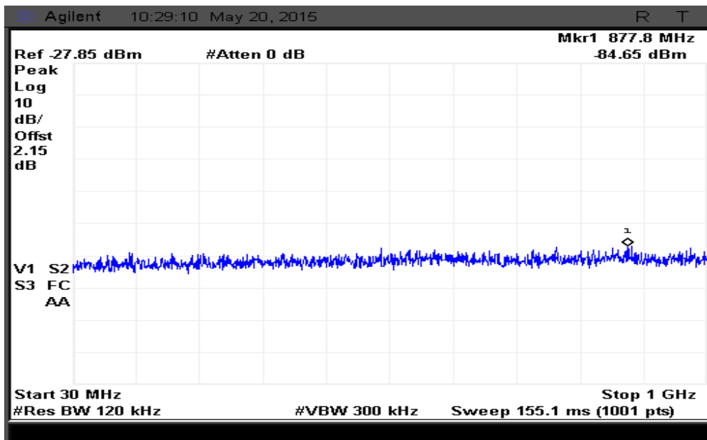
Figure 320: Spurious emission measured from 30 MHz to 1 GHz at Ch. 1-Peak
