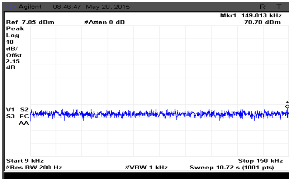
Figure 84: Spurious emission measured from 9 kHz to 150 kHz at Ch. 1-Peak
