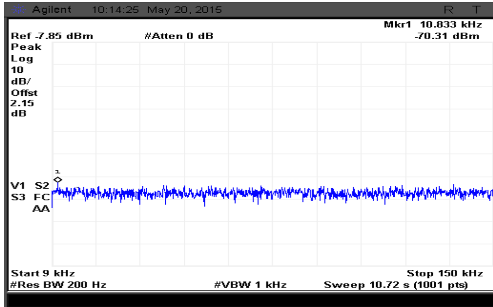
Figure 165: Spurious emission measured from 9 kHz to 150 kHz at Ch. 0-Peak
