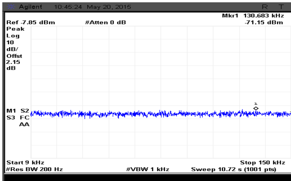
Figure 210: Spurious emission measured from 9 kHz to 150 kHz at Ch. 1-Peak
