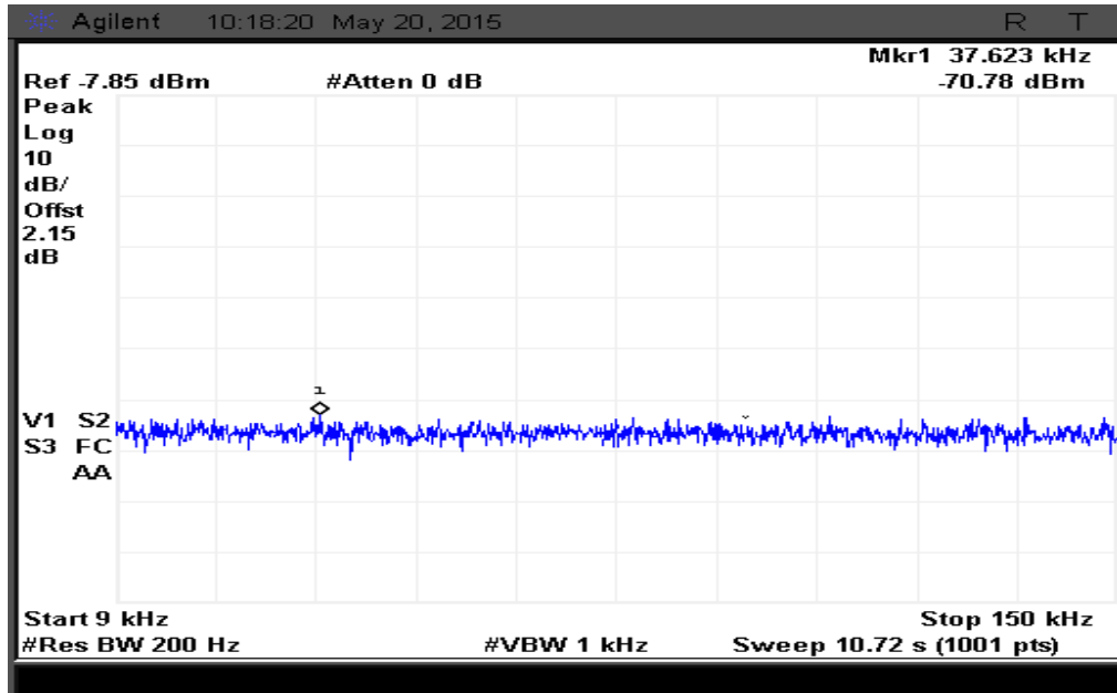
Figure 273: Spurious emission measured from 9 kHz to 150 kHz at Ch. 0-Peak
