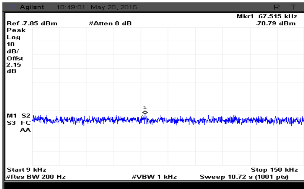
Figure 102: Spurious emission measured from 9 kHz to 150 kHz at Ch. 1-Peak
