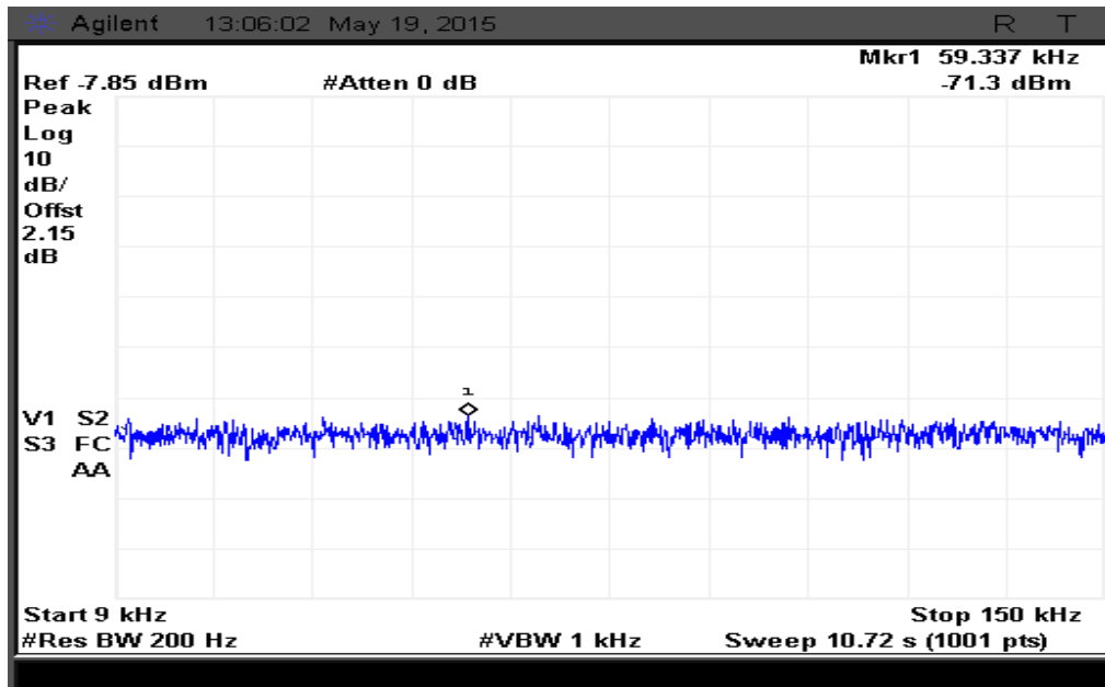
Figure 30: Spurious emission measured from 9 kHz to 150 kHz at Ch. 1-Peak
