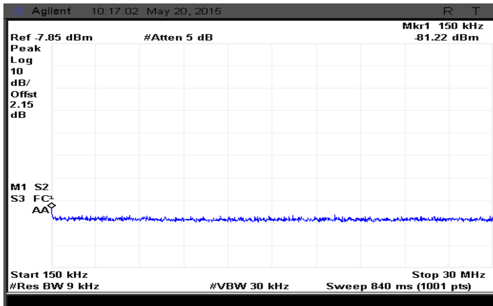
Figure 274: Spurious emission measured from 150 kHz to 30 MHz at Ch. 0-Peak
