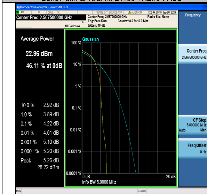
Band7-5MHz-16QAM-21425-1RB#0-PASS
