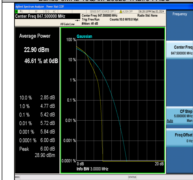
Band5-3MHz-16QAM-20635-1RB#0-PASS
