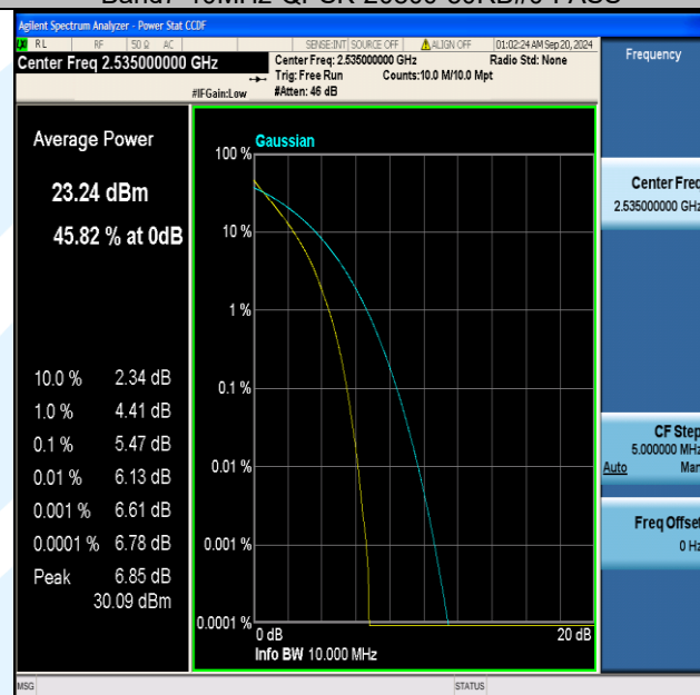
Band7-10MHz-QPSK-21100-50RB#0-PASS
