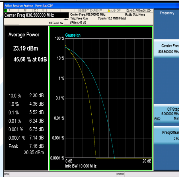
Band5-10MHz-QPSK-20525-50RB#0-PASS
