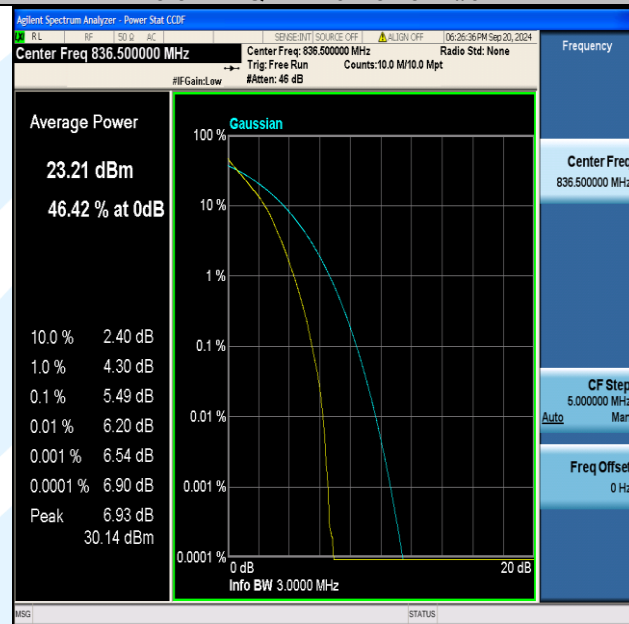
Band5-3MHz-QPSK-20525-15RB#0-PASS
