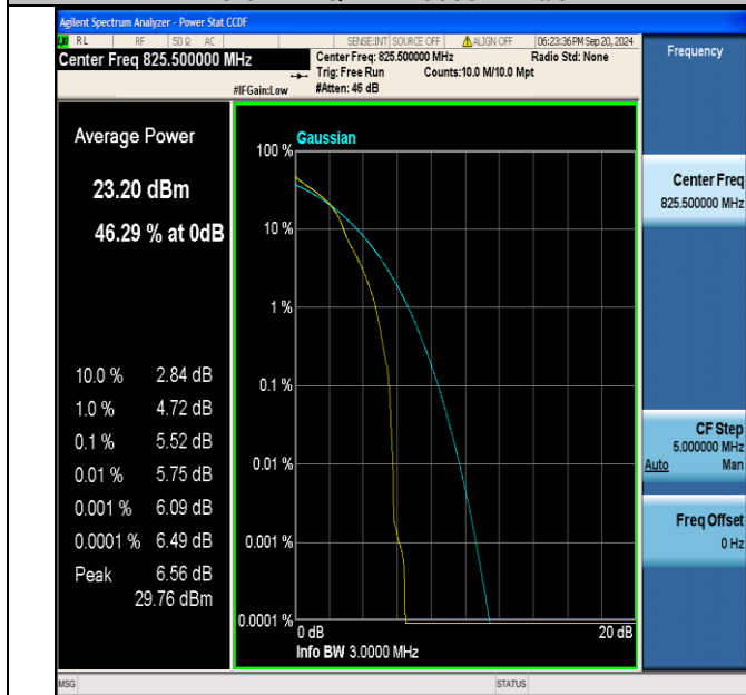
Band5-3MHz-16QAM-20415-1RB#0-PASS
