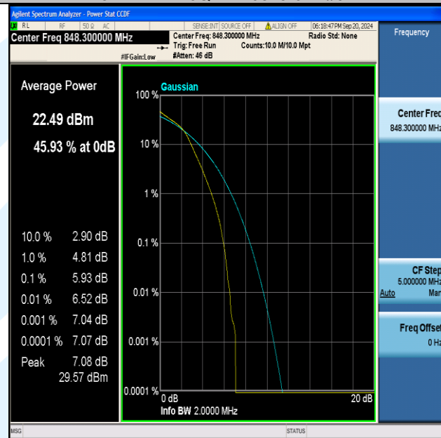
Band5-1.4MHz-16QAM-20643-6RB#0-PASS
