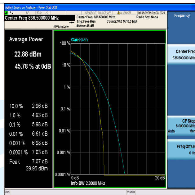
Band5-1.4MHz-16QAM-20525-6RB#0-PASS
