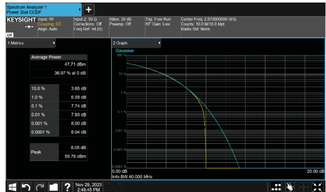
BRS Band n7, 2620 MHz - 2690 MHz 40 MHz Bandwidth 256QAM Modulation High Ch, 2670.0 MHz
