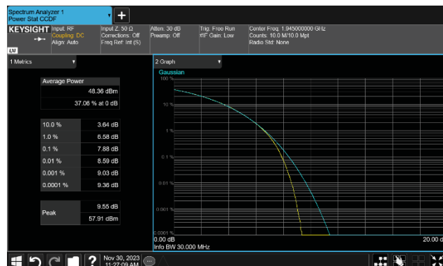
PCS Band n25, 1930 MHz - 1995 MHz 30 MHz Bandwidth 256QAM Modulation Low Ch, 1945.0 MHz
