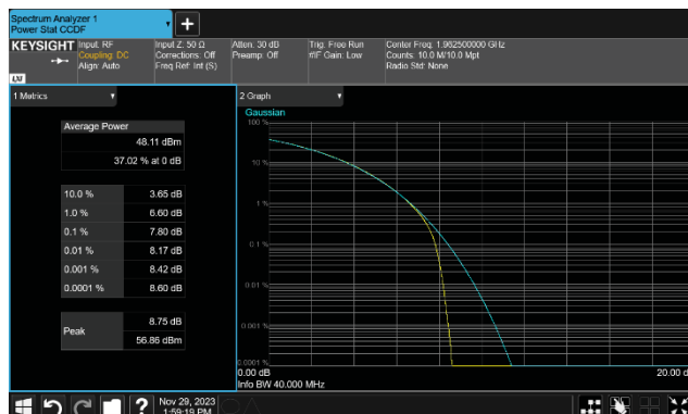
PCS Band n25, 1930 MHz - 1995 MHz 40 MHz Bandwidth 16QAM Modulation Mid Ch, 1962.5 MHz
