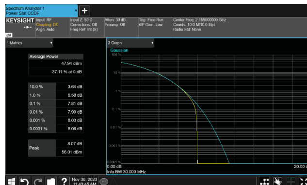
AWS Band n66, 2110 MHz - 2200 MHz 30 MHz Bandwidth 16QAM Modulation Mid Ch, 2155.0 MHz
