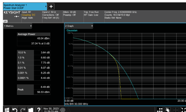
BRS Band n7, 2620 MHz - 2690 MHz 30 MHz Bandwidth 256QAM Modulation Low Ch, 2635.0 MHz
