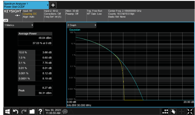
AWS Band n66, 2110 MHz - 2200 MHz 30 MHz Bandwidth 256QAM Modulation High Ch, 2185.0 MHz
