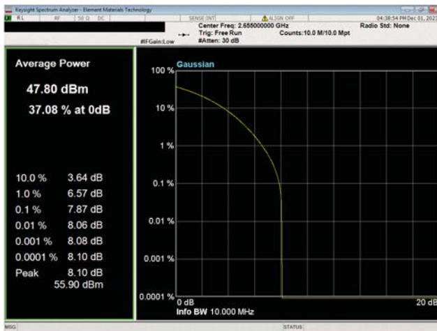
BRS Band n7, 2620 MHz - 2690 MHz 10 MHz Bandwidth QPSK Modulation Mid Ch, 2655.0 MHz
