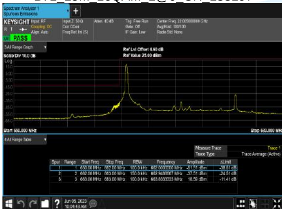
B71 15M 16QAM 1@0 CH 133197
