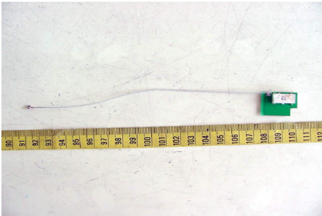
Front View of \lambda/4 Transmission track type antenna (KD02961-L05X)
