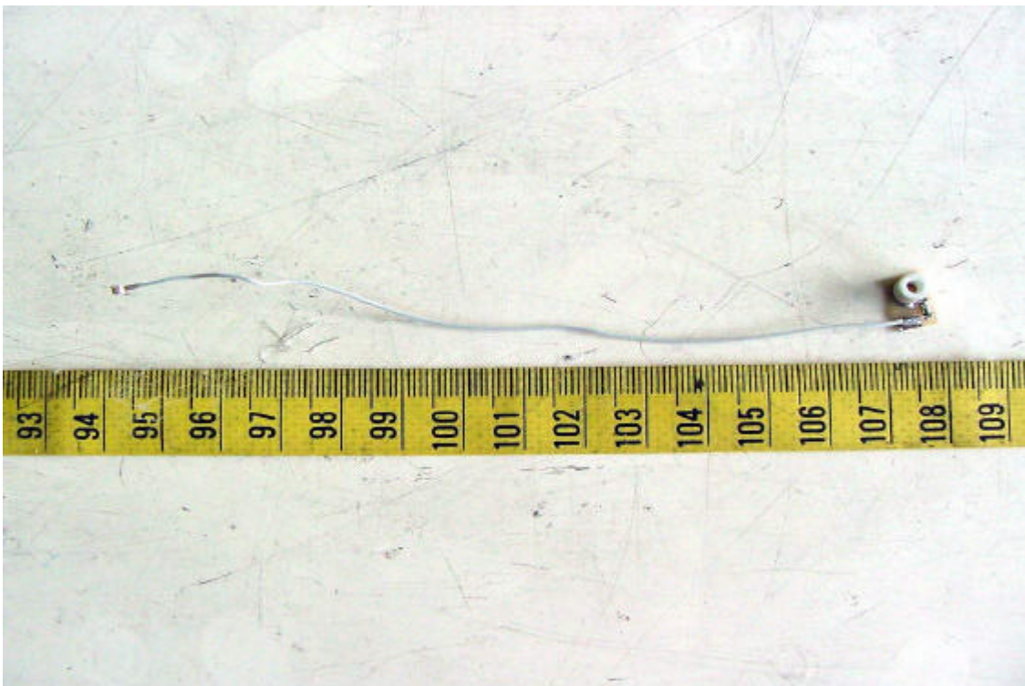
Front View of \lambda/4 Helical antenna (CA05951-738X)
