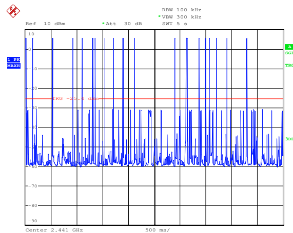
Plot 6 (DH5 packet) – N° of packets in 5s. (19 hops)
