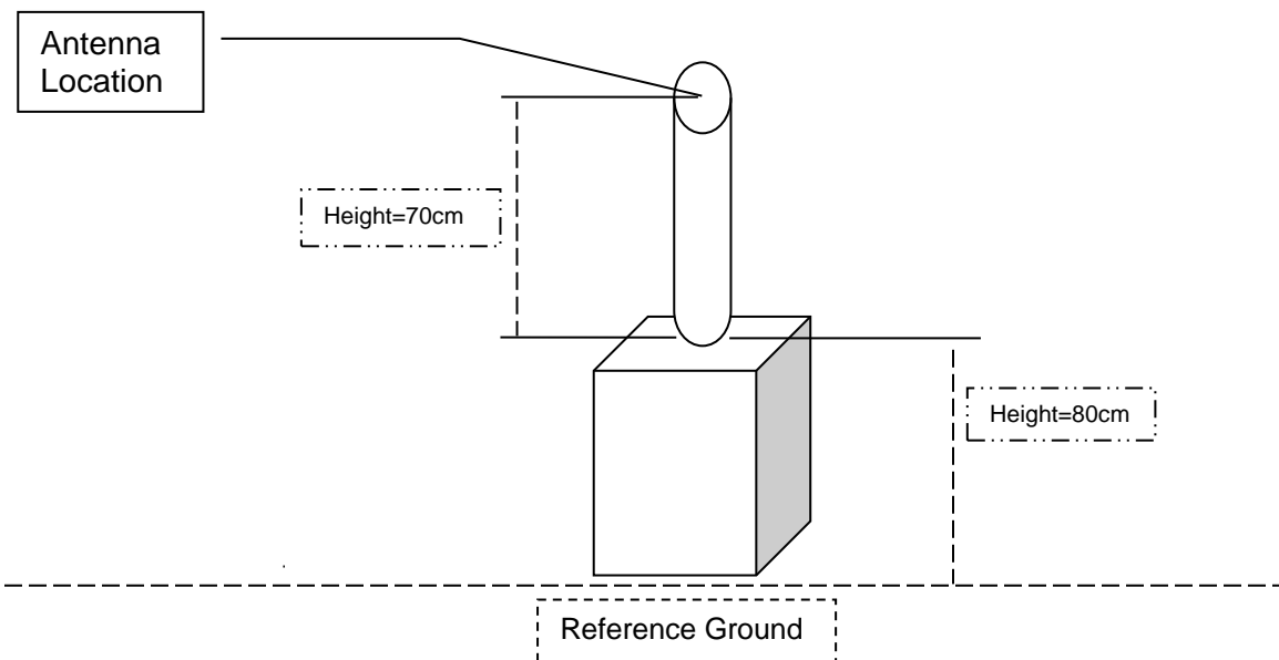
RADIATED RF MEASUREMENT SETUP (ABOVE 1 GHz- Xaxis)-Part 2
