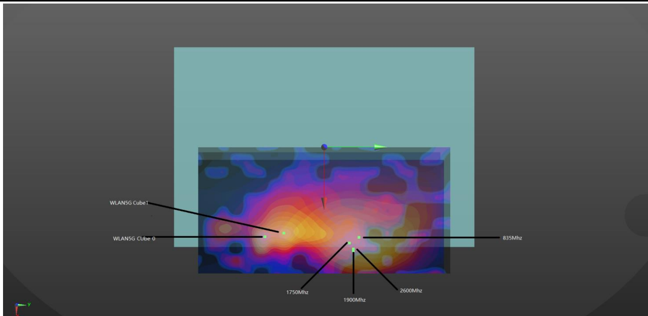
WWAN+WLAN 5GHz Bottom Face
