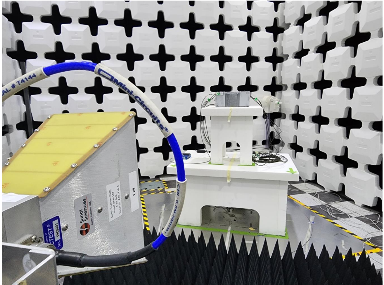
Above 1GHz Test Instrument & Measurement Setup > 1GHz
