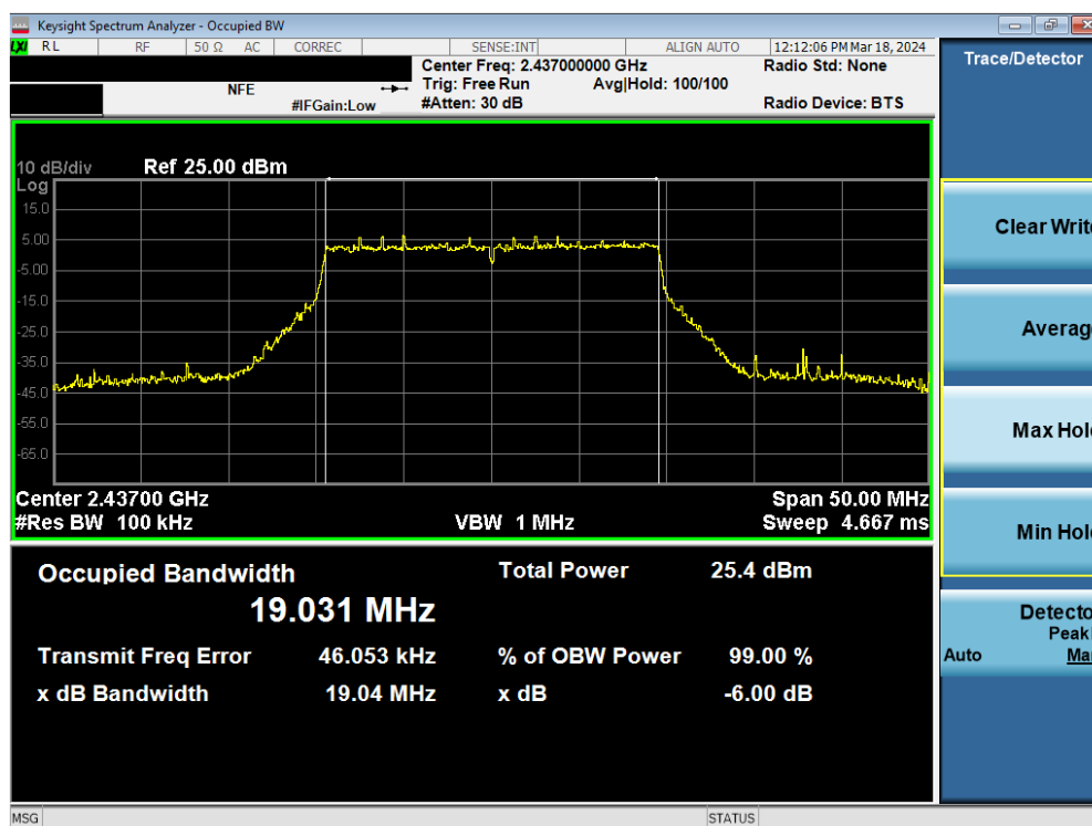
Plot 7-36. 6dB Bandwidth Plot MIMO ANT2 (802.11ax/be (2.4GHz) – Ch. 6)
