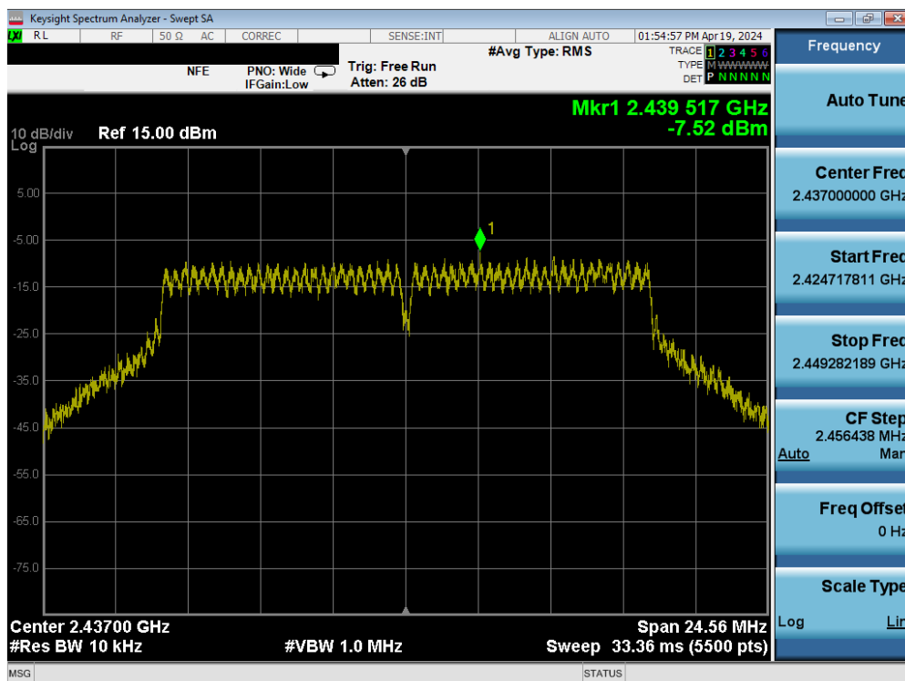
Plot 7-42. Power Spectral Density Plot SISO ANT2 (802.11g – Ch. 6)
