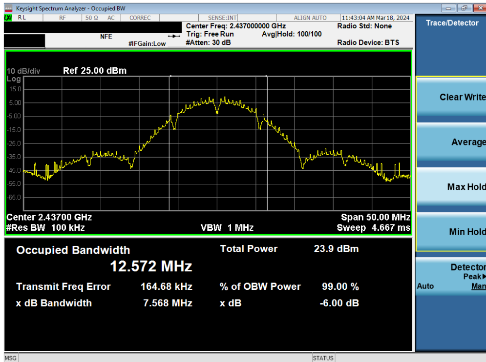
Plot 7-27. 6dB Bandwidth Plot MIMO ANT2 (802.11b – Ch. 6)
