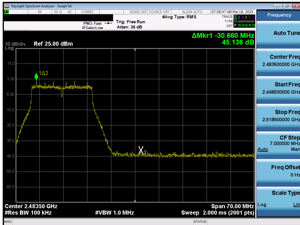
Plot 7-99. Band Edge Plot MIMO ANT1 (802.11n (2.4GHz) – Ch. 11)
