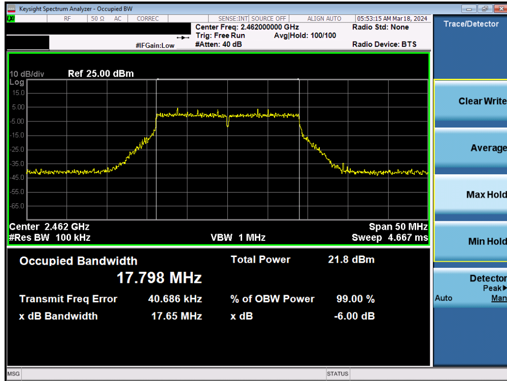
Plot 7-22. 6dB Bandwidth Plot MIMO ANT1 (802.11n (2.4GHz) – Ch. 11)
