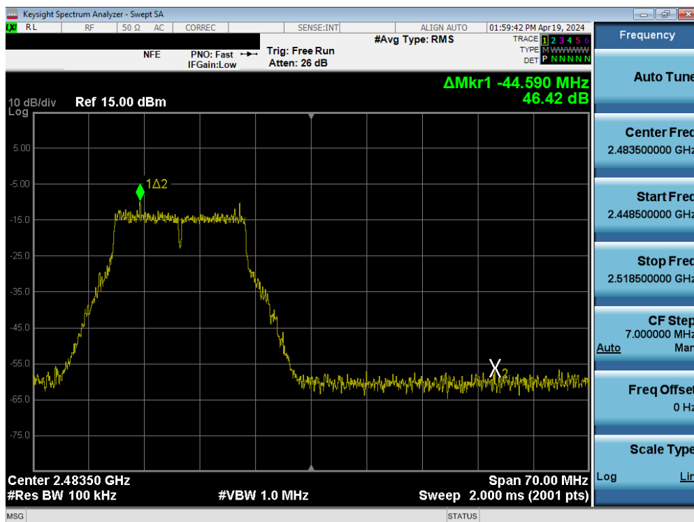
Plot 7-80. Band Edge Plot SISO ANT2 (802.11g – Ch. 12)
