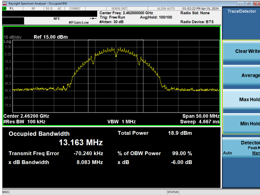
Plot 7-4. 6dB Bandwidth Plot SISO ANT2 (802.11b – Ch. 11)
