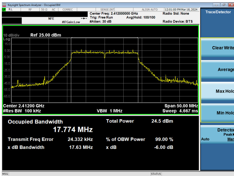
Plot 7-32. 6dB Bandwidth Plot MIMO ANT2 (802.11n (2.4GHz) – Ch. 1)
