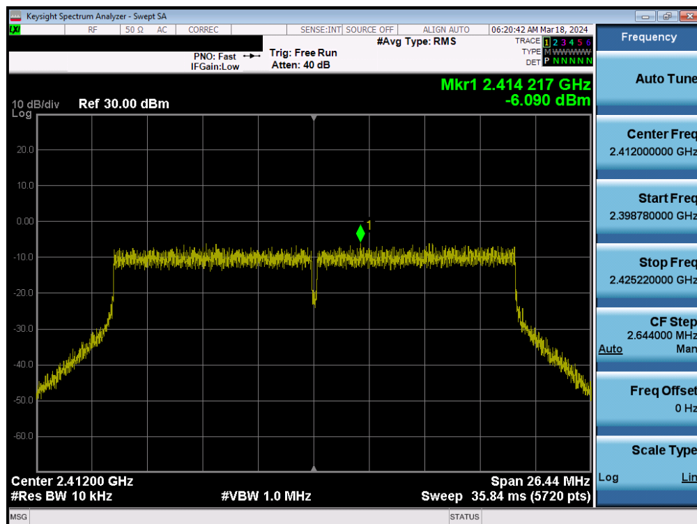
Plot 7-59. Power Spectral Density Plot MIMO ANT1 (802.11ax/be (2.4GHz) – Ch. 1)
