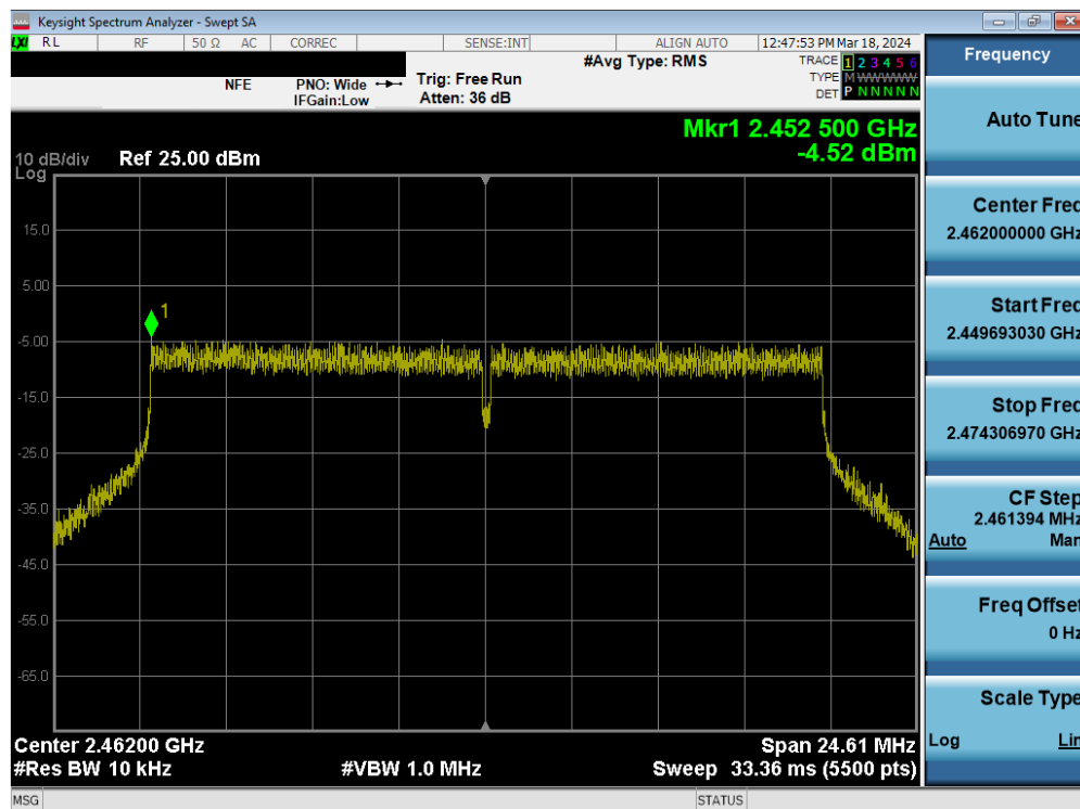
Plot 7-73. Power Spectral Density Plot MIMO ANT2 (802.11ax/be (2.4GHz) – Ch. 11)
