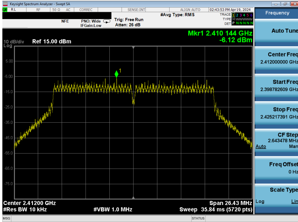
Plot 7-44. Power Spectral Density Plot SISO ANT2 (802.11n (2.4GHz) – Ch. 1)
