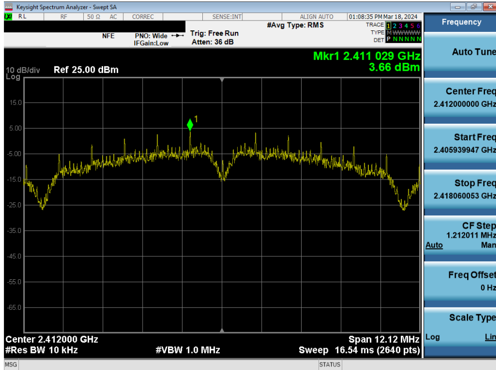
Plot 7-62. Power Spectral Density Plot MIMO ANT2 (802.11b – Ch. 1)
