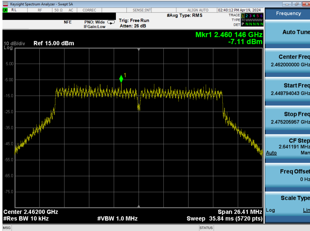
Plot 7-46. Power Spectral Density Plot SISO ANT2 (802.11n (2.4GHz) – Ch. 11)
