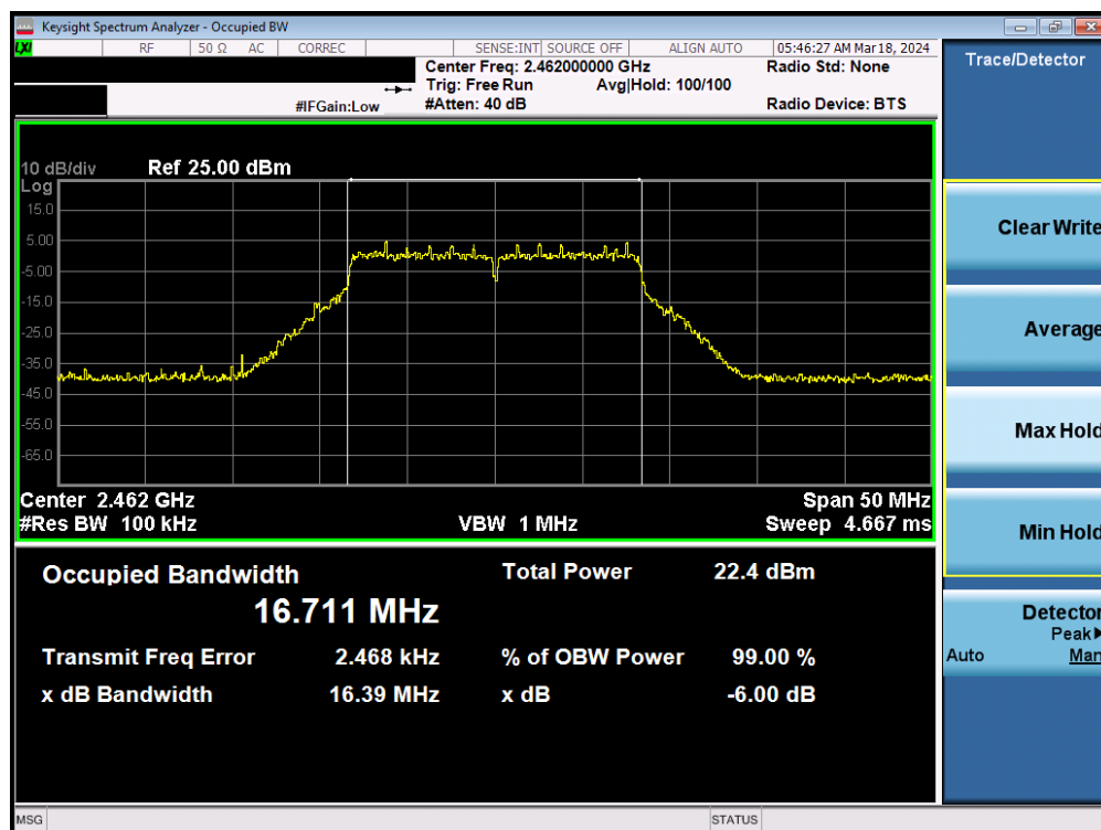
Plot 7-19. 6dB Bandwidth Plot MIMO ANT1 (802.11g – Ch. 11)
