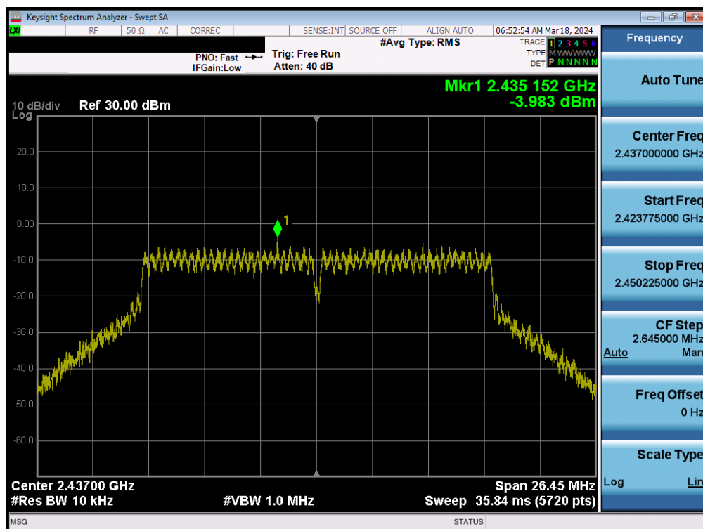
Plot 7-54. Power Spectral Density Plot MIMO ANT1 (802.11g – Ch. 6)
