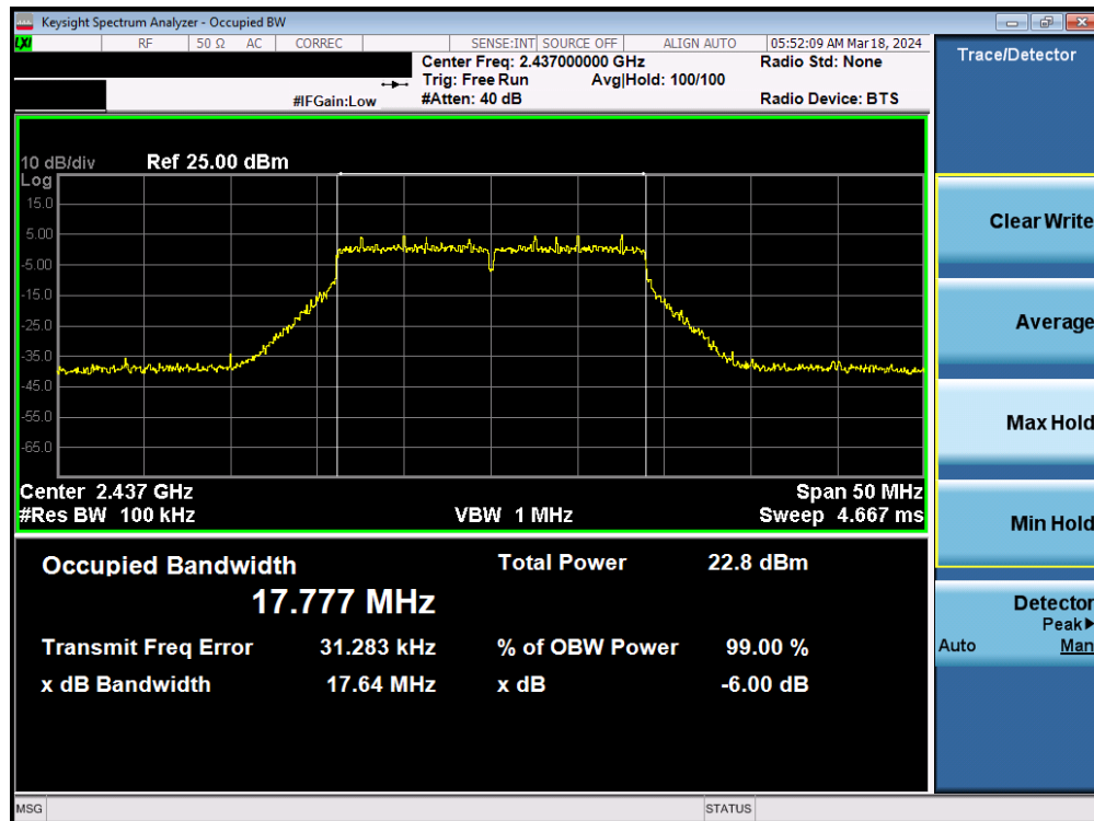
Plot 7-21. 6dB Bandwidth Plot MIMO ANT1 (802.11n (2.4GHz) – Ch. 6)
