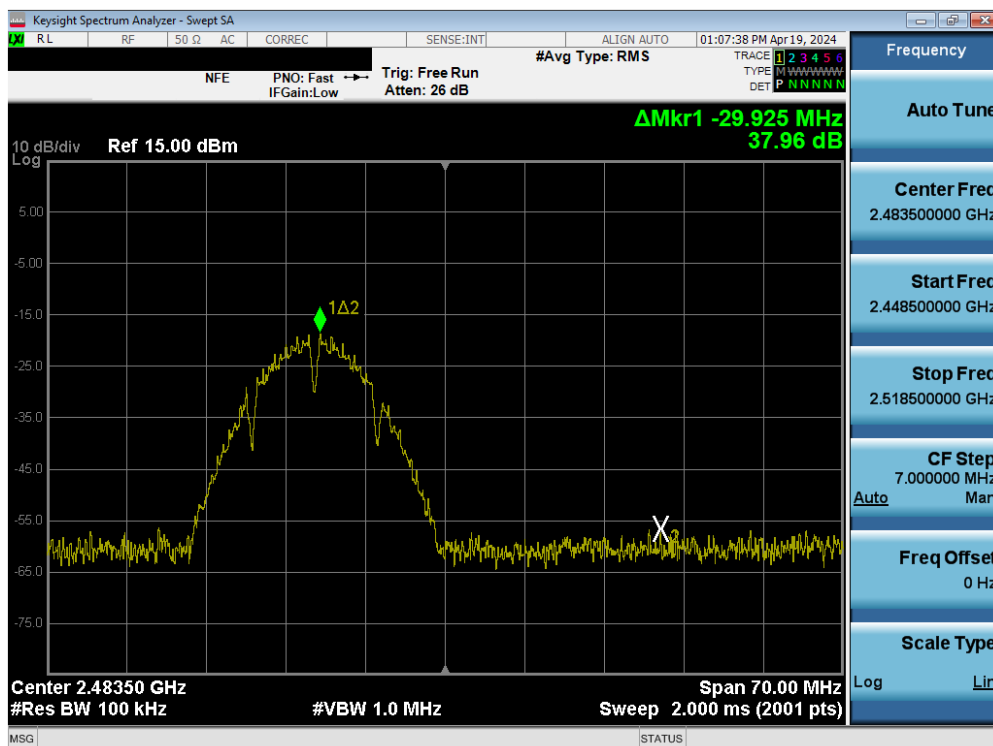
Plot 7-77. Band Edge Plot SISO ANT2 (802.11b – Ch. 13)
