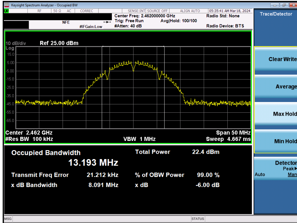
Plot 7-16. 6dB Bandwidth Plot MIMO ANT1 (802.11b – Ch. 11)
