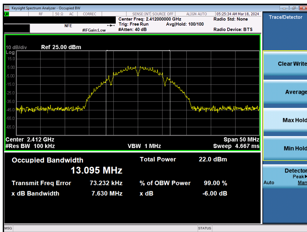
Plot 7-14. 6dB Bandwidth Plot MIMO ANT1 (802.11b – Ch. 1)
