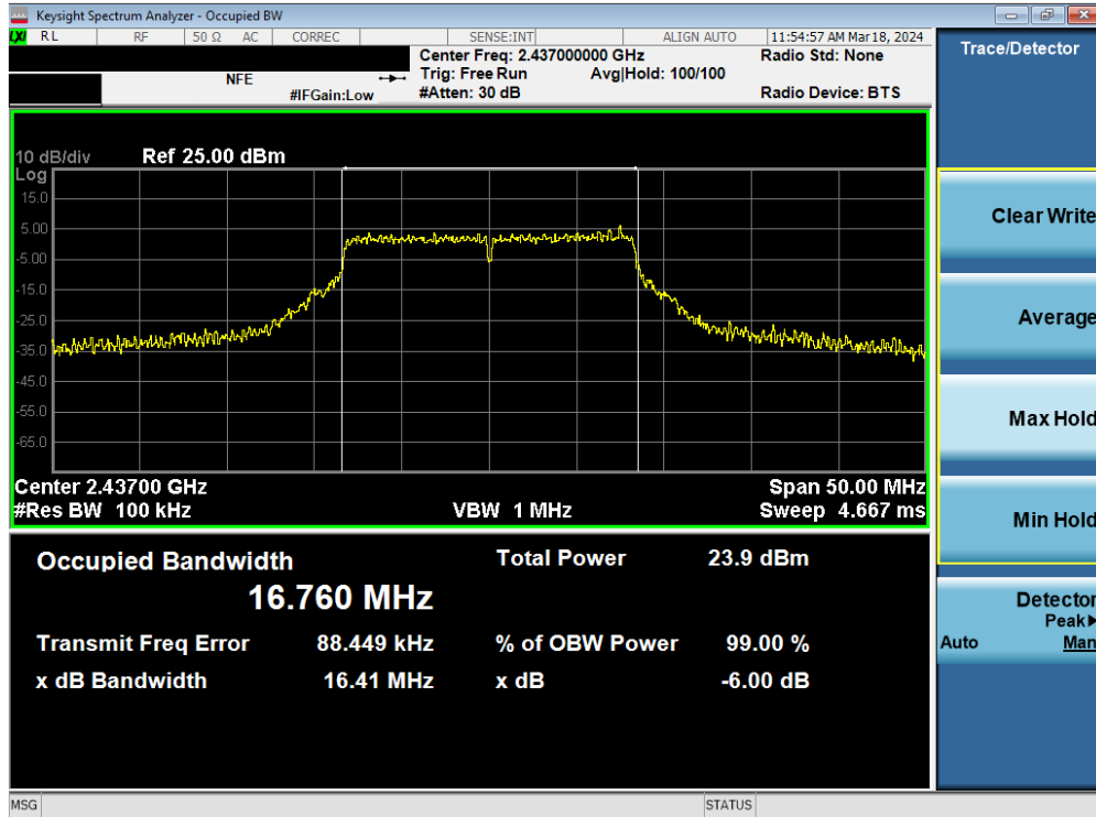
Plot 7-30. 6dB Bandwidth Plot MIMO ANT2 (802.11g – Ch. 6)
