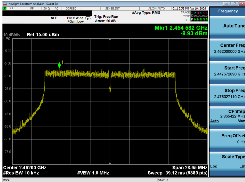
Plot 7-49. Power Spectral Density Plot SISO ANT2 (802.11ax/be (2.4GHz) – Ch. 11)
