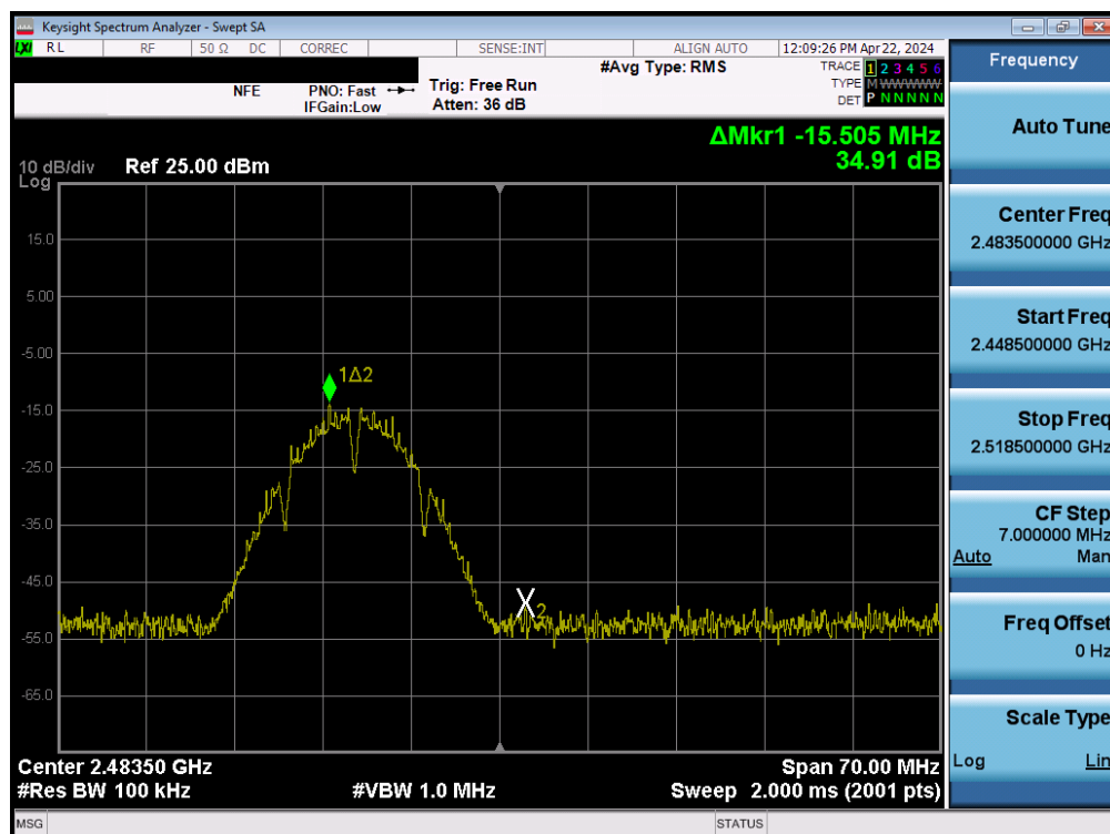
Plot 7-93. Band Edge Plot MIMO ANT1 (802.11b – Ch. 13)
