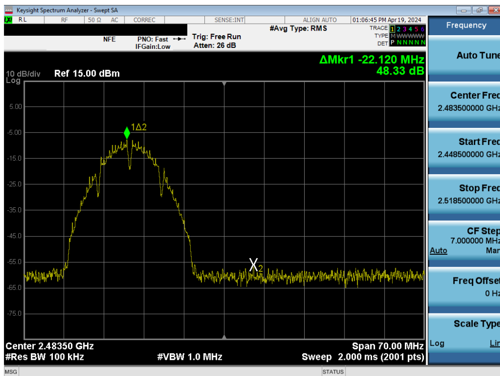
Plot 7-76. Band Edge Plot SISO ANT2 (802.11b – Ch. 12)
