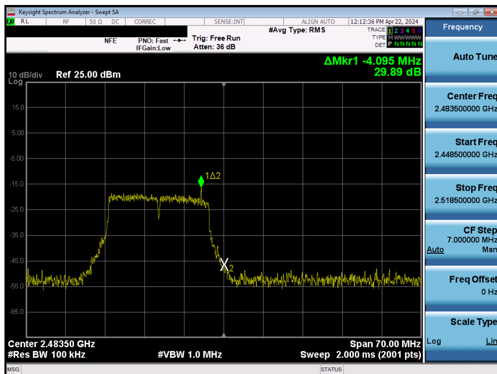
Plot 7-101. Band Edge Plot MIMO ANT1 (802.11n (2.4GHz) – Ch. 13)
