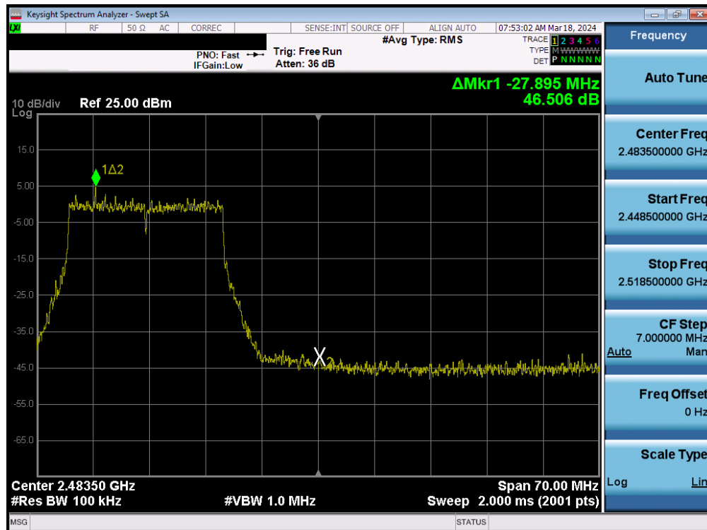
Plot 7-103. Band Edge Plot MIMO ANT1 (802.11ax/be (2.4GHz) – Ch. 11)
