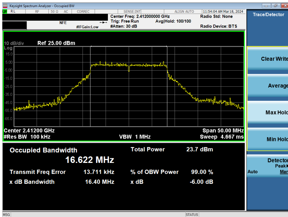
Plot 7-29. 6dB Bandwidth Plot MIMO ANT2 (802.11g – Ch. 1)
