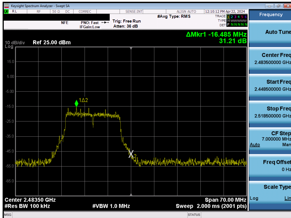
Plot 7-97. Band Edge Plot MIMO ANT1 (802.11g – Ch. 13)
