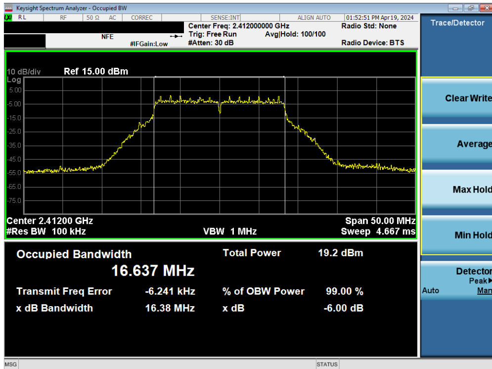
Plot 7-5. 6dB Bandwidth Plot SISO ANT2 (802.11g – Ch. 1)
