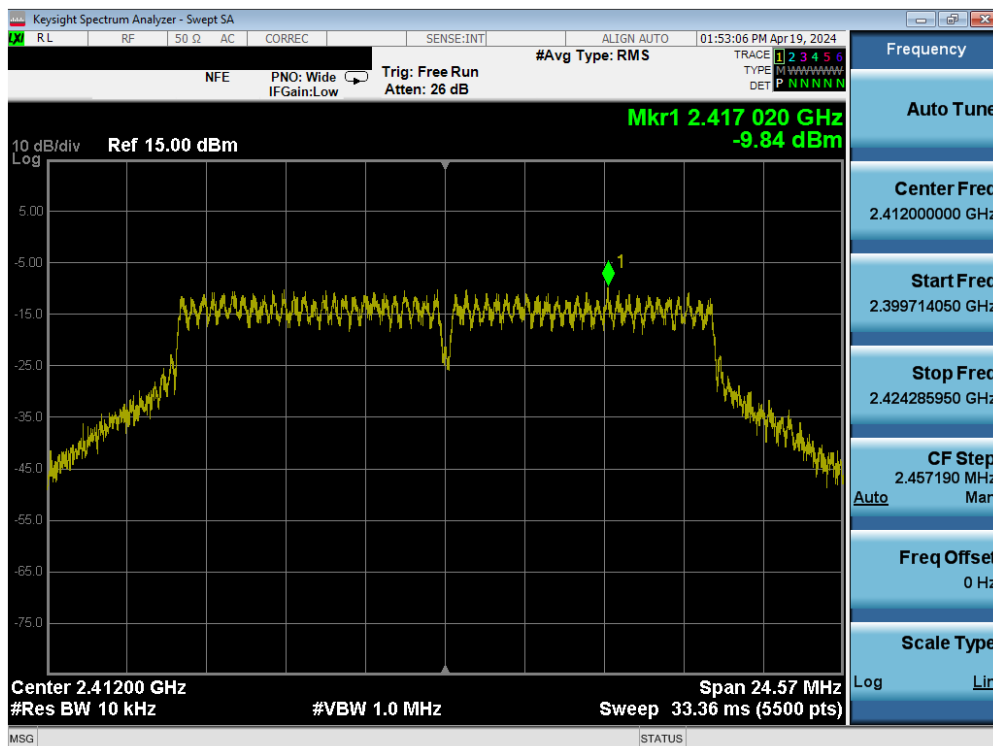
Plot 7-41. Power Spectral Density Plot SISO ANT2 (802.11g – Ch. 1)
