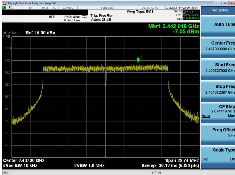
Plot 7-48. Power Spectral Density Plot SISO ANT2 (802.11ax/be (2.4GHz) – Ch. 6)
