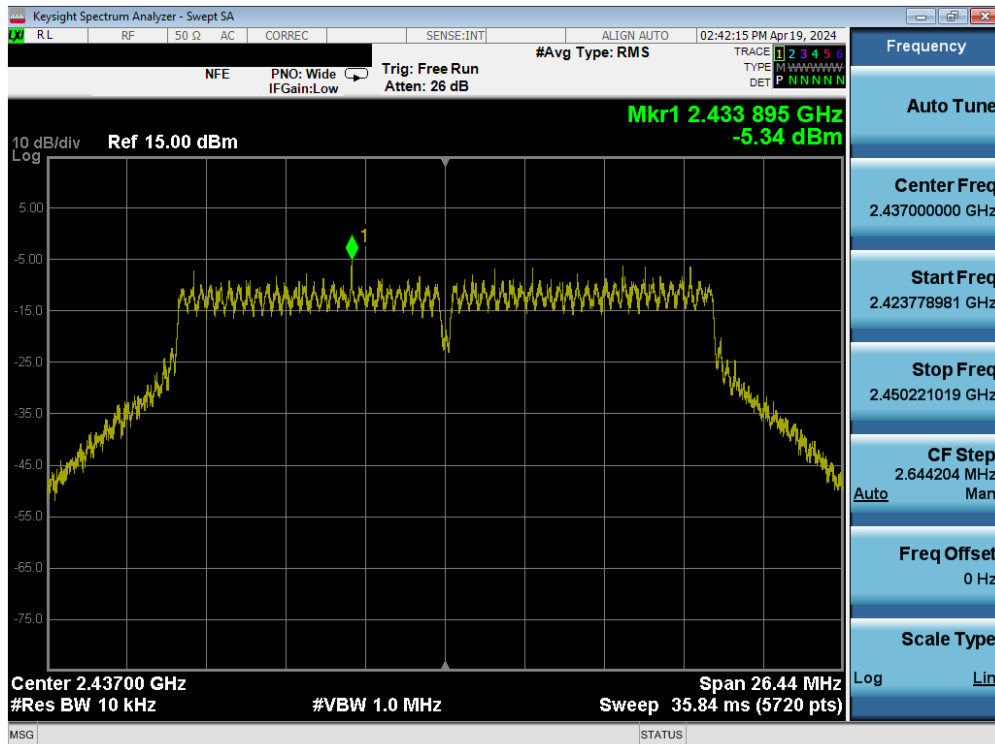
Plot 7-45. Power Spectral Density Plot SISO ANT2 (802.11n (2.4GHz) – Ch. 6)
