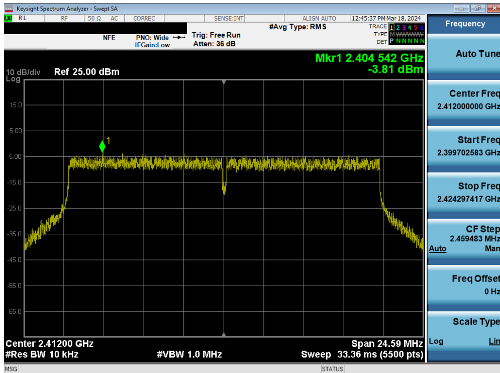
Plot 7-71. Power Spectral Density Plot MIMO ANT2 (802.11ax/be (2.4GHz) – Ch. 1)
