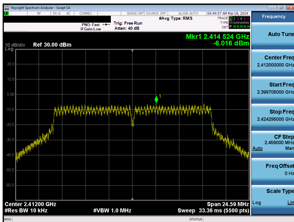
Plot 7-53. Power Spectral Density Plot MIMO ANT1 (802.11g – Ch. 1)
