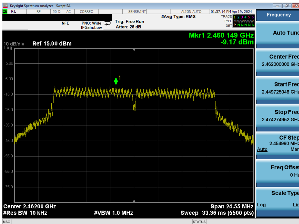
Plot 7-43. Power Spectral Density Plot SISO ANT2 (802.11g – Ch. 11)
