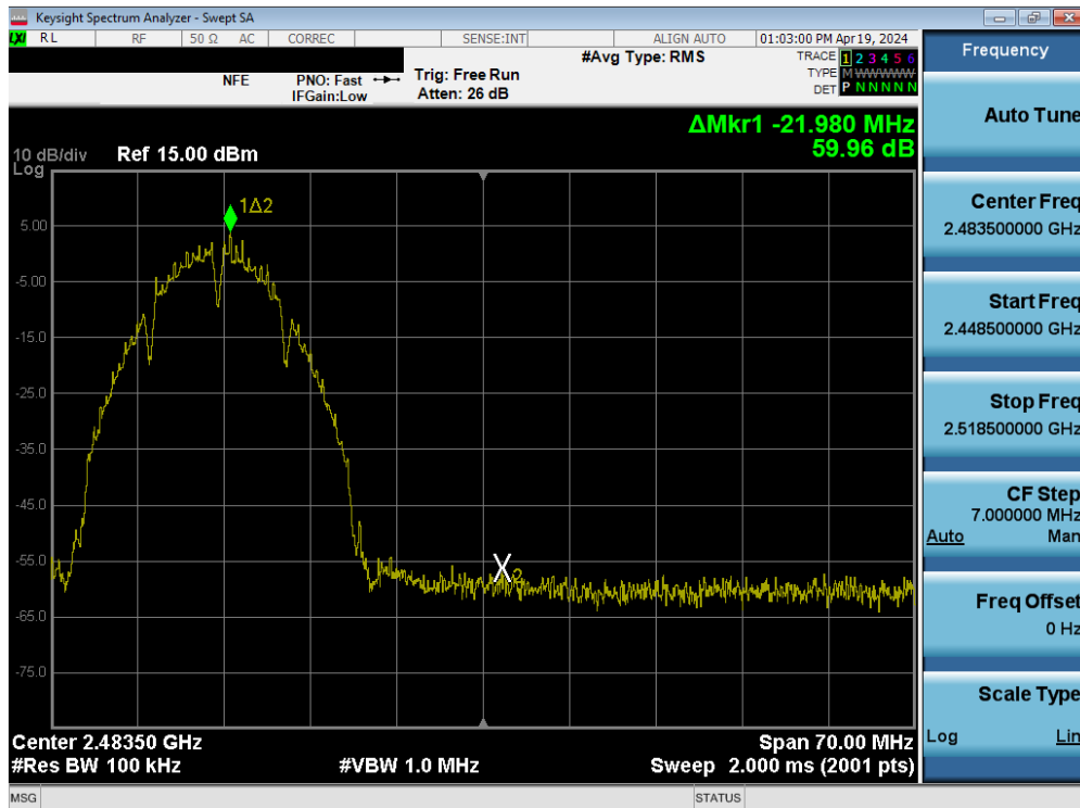
Plot 7-75. Band Edge Plot SISO ANT2 (802.11b – Ch. 11)
