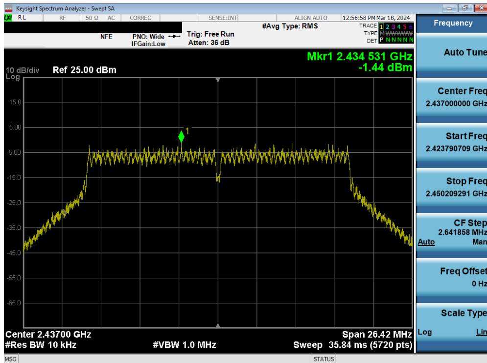
Plot 7-69. Power Spectral Density Plot MIMO ANT2 (802.11n (2.4GHz) – Ch. 6)
