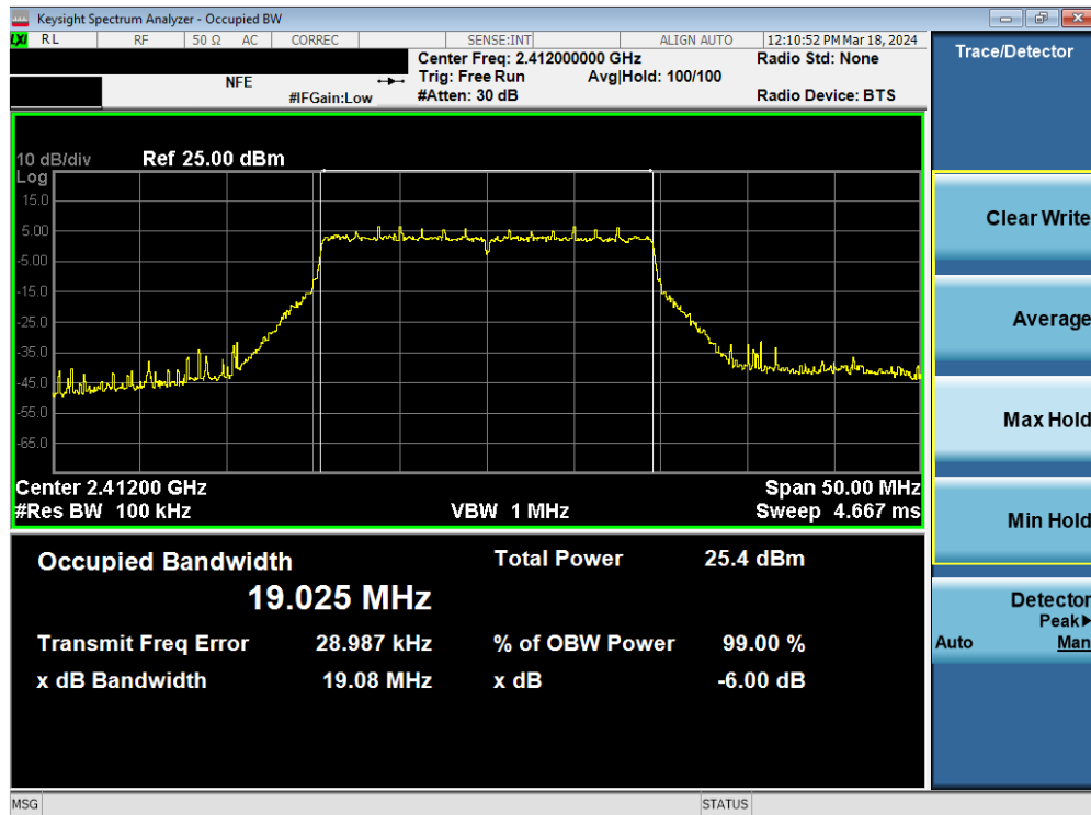
Plot 7-35. 6dB Bandwidth Plot MIMO ANT2 (802.11ax/be (2.4GHz) – Ch. 1)
