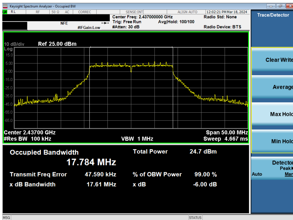
Plot 7-33. 6dB Bandwidth Plot MIMO ANT2 (802.11n (2.4GHz) – Ch. 6)
