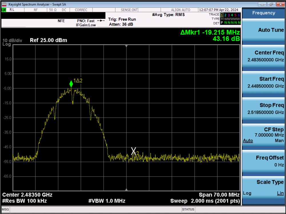
Plot 7-108. Band Edge Plot MIMO ANT2 (802.11b – Ch. 12)
