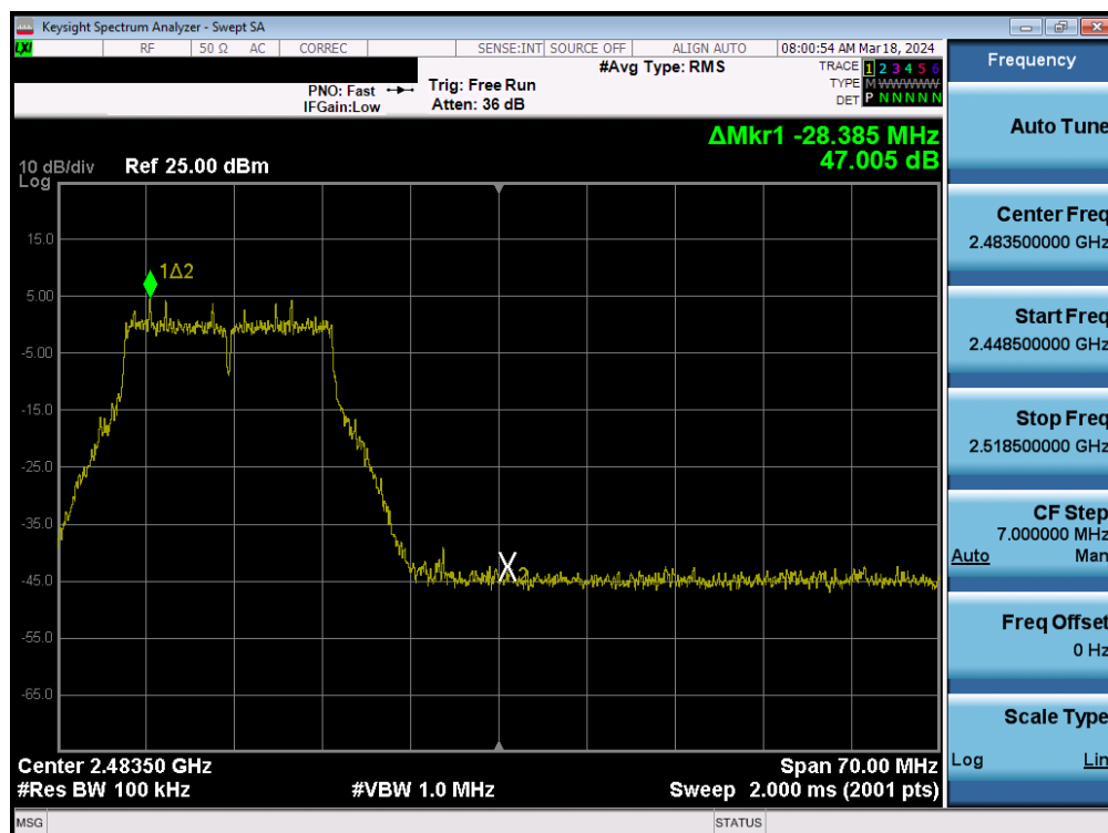
Plot 7-95. Band Edge Plot MIMO ANT1 (802.11g – Ch. 11)
