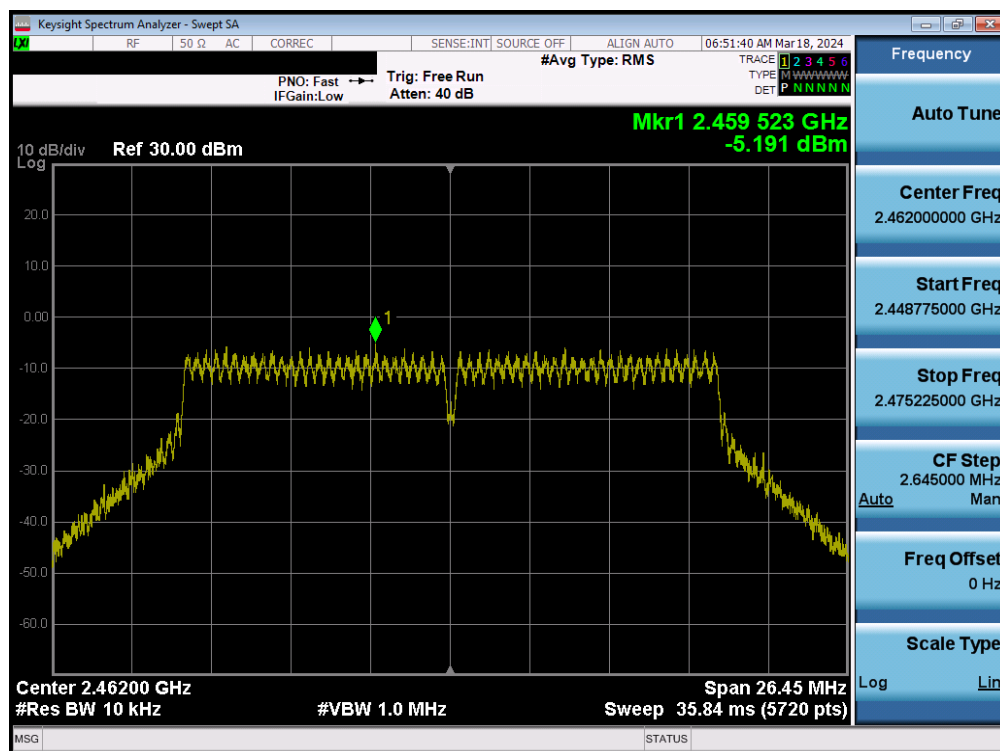
Plot 7-58. Power Spectral Density Plot MIMO ANT1 (802.11n (2.4GHz) – Ch. 11)
