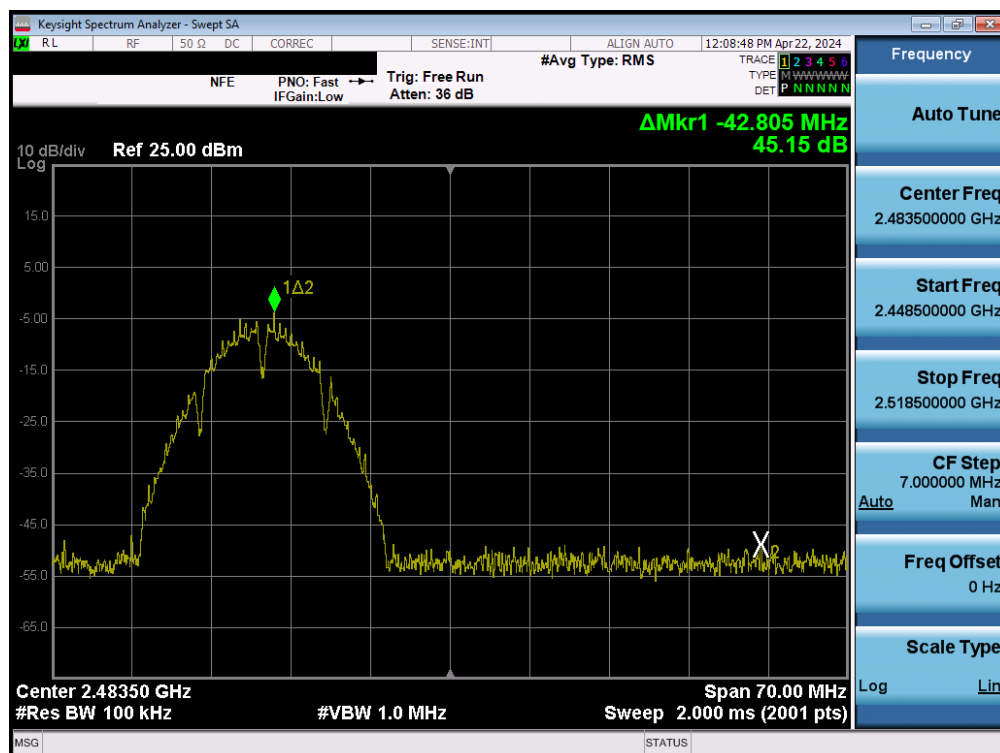
Plot 7-92. Band Edge Plot MIMO ANT1 (802.11b – Ch. 12)
