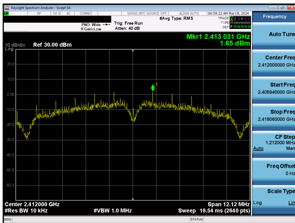
Plot 7-50. Power Spectral Density Plot MIMO ANT1 (802.11b – Ch. 1)
