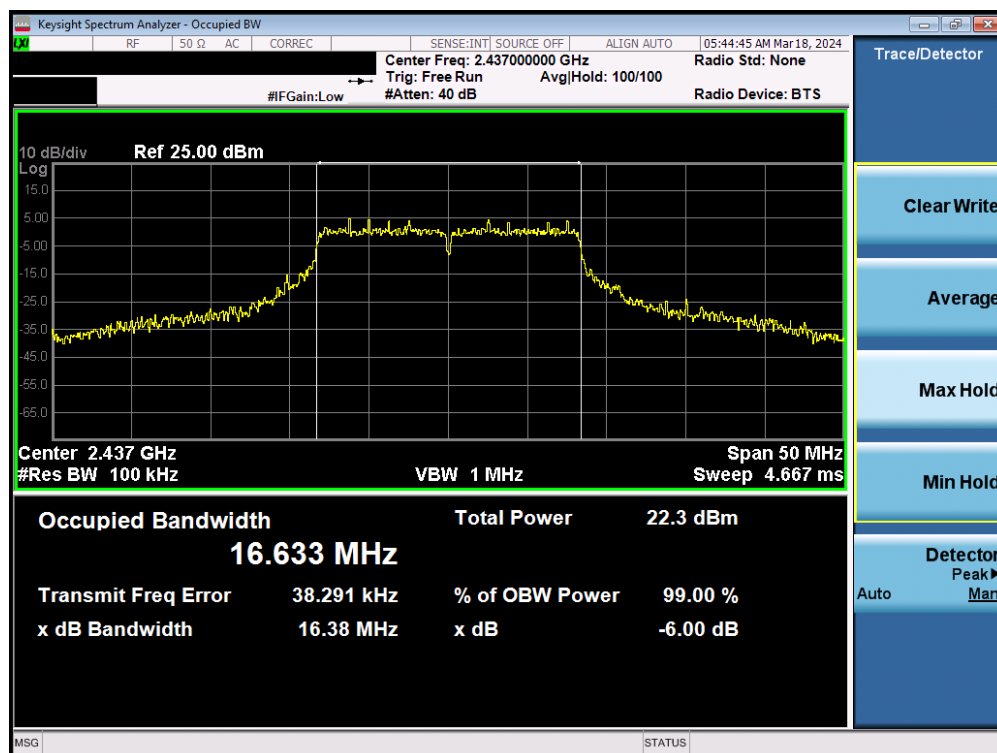
Plot 7-18. 6dB Bandwidth Plot MIMO ANT1 (802.11g – Ch. 6)
