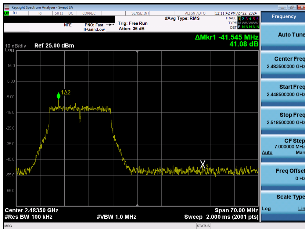
Plot 7-100. Band Edge Plot MIMO ANT1 (802.11n (2.4GHz) – Ch. 12)
