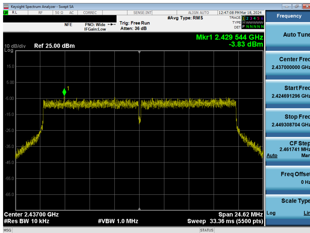
Plot 7-72. Power Spectral Density Plot MIMO ANT2 (802.11ax/be (2.4GHz) – Ch. 6)
