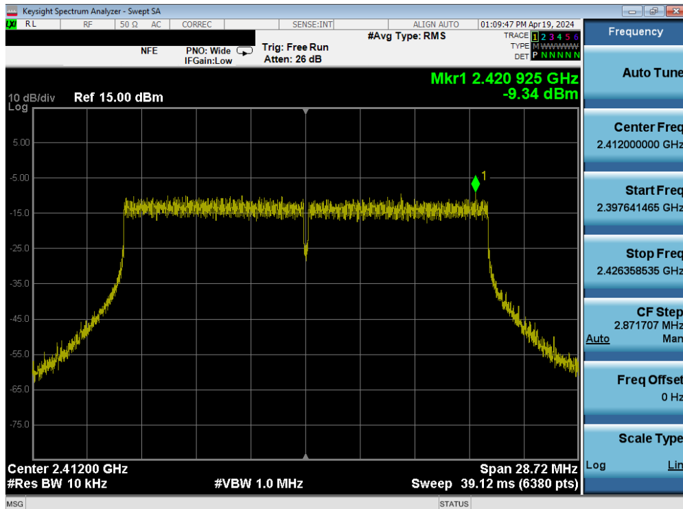
Plot 7-47. Power Spectral Density Plot SISO ANT2 (802.11ax/be (2.4GHz) – Ch. 1)
