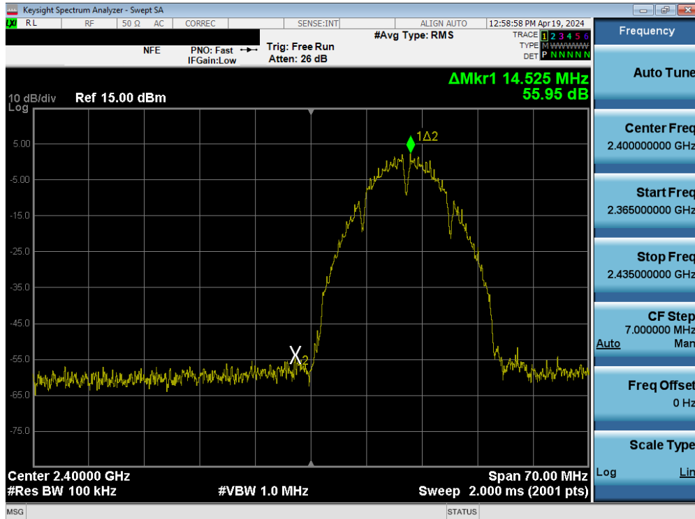
Plot 7-74. Band Edge Plot SISO ANT2 (802.11b – Ch. 1)
