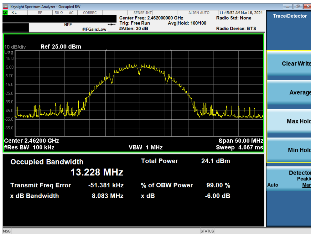
Plot 7-28. 6dB Bandwidth Plot MIMO ANT2 (802.11b – Ch. 11)
