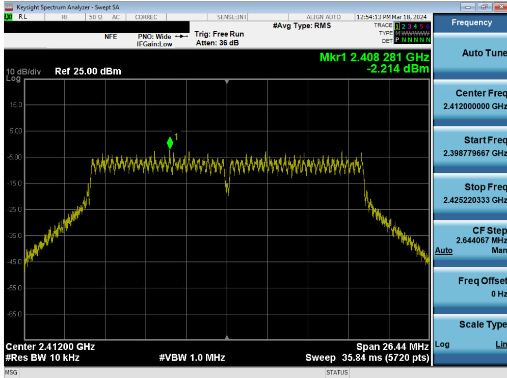
Plot 7-68. Power Spectral Density Plot MIMO ANT2 (802.11n (2.4GHz) – Ch. 1)
