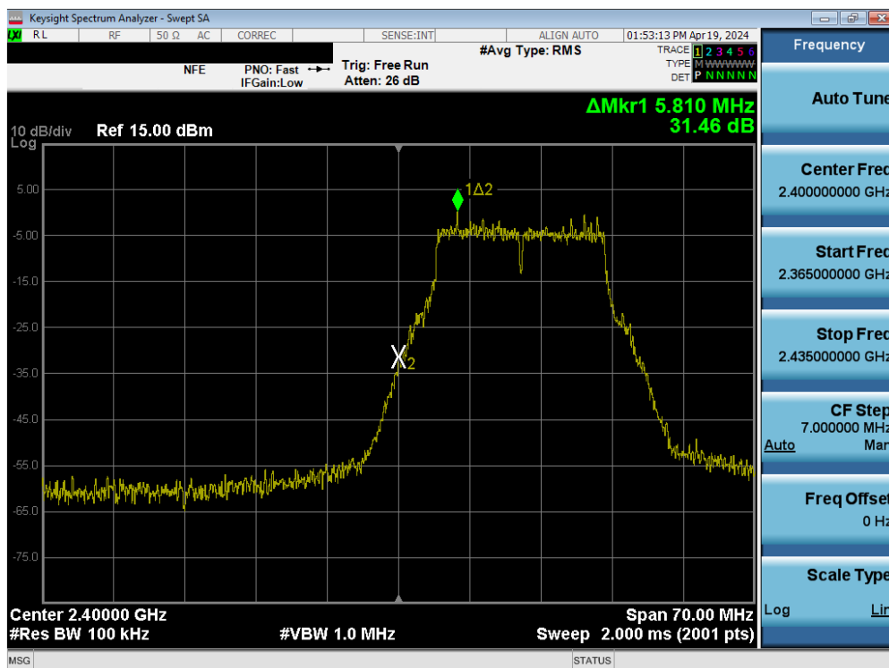
Plot 7-78. Band Edge Plot SISO ANT2 (802.11g- Ch. 1)
