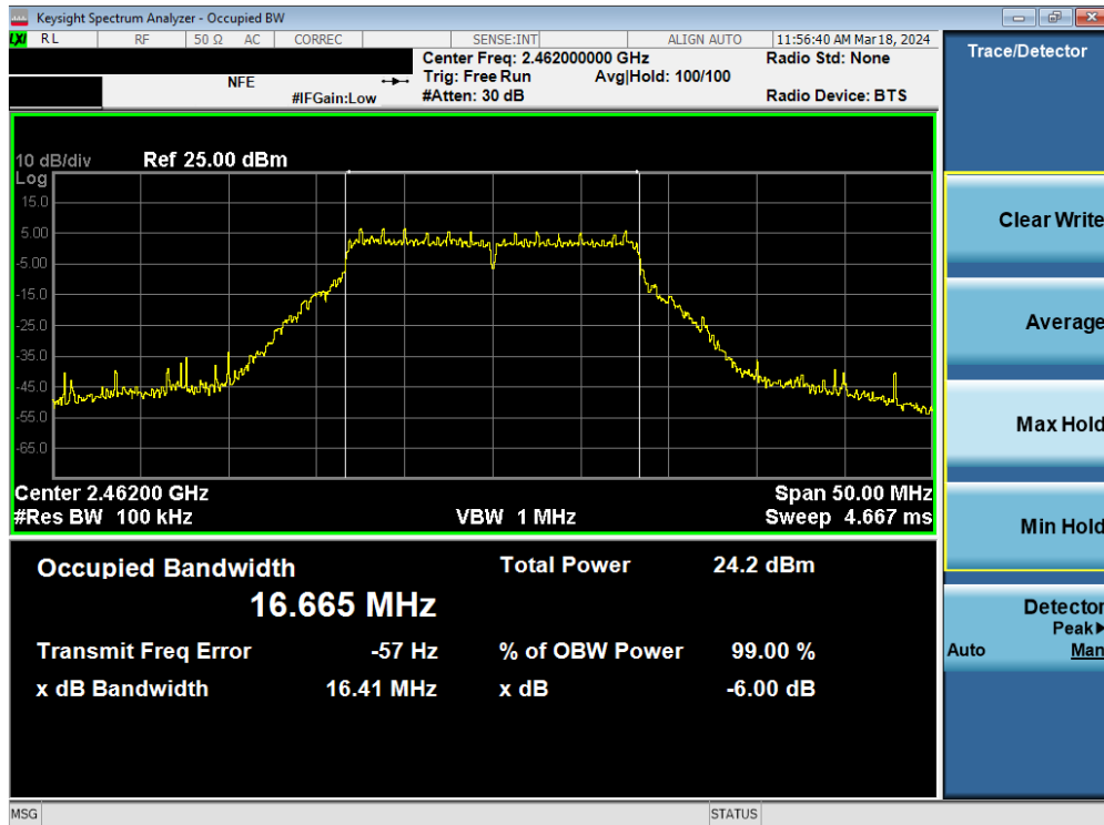
Plot 7-31. 6dB Bandwidth Plot MIMO ANT2 (802.11g – Ch. 11)
