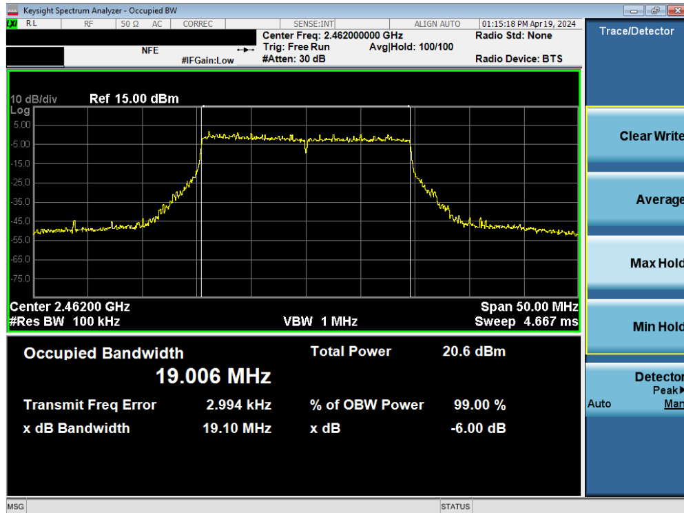
Plot 7-13. 6dB Bandwidth Plot SISO ANT2 (802.11ax/be (2.4GHz) – Ch. 11)
