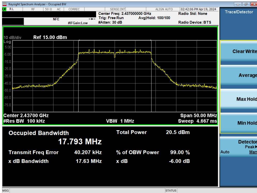
Plot 7-9. 6dB Bandwidth Plot SISO ANT2 (802.11n (2.4GHz) – Ch. 6)
