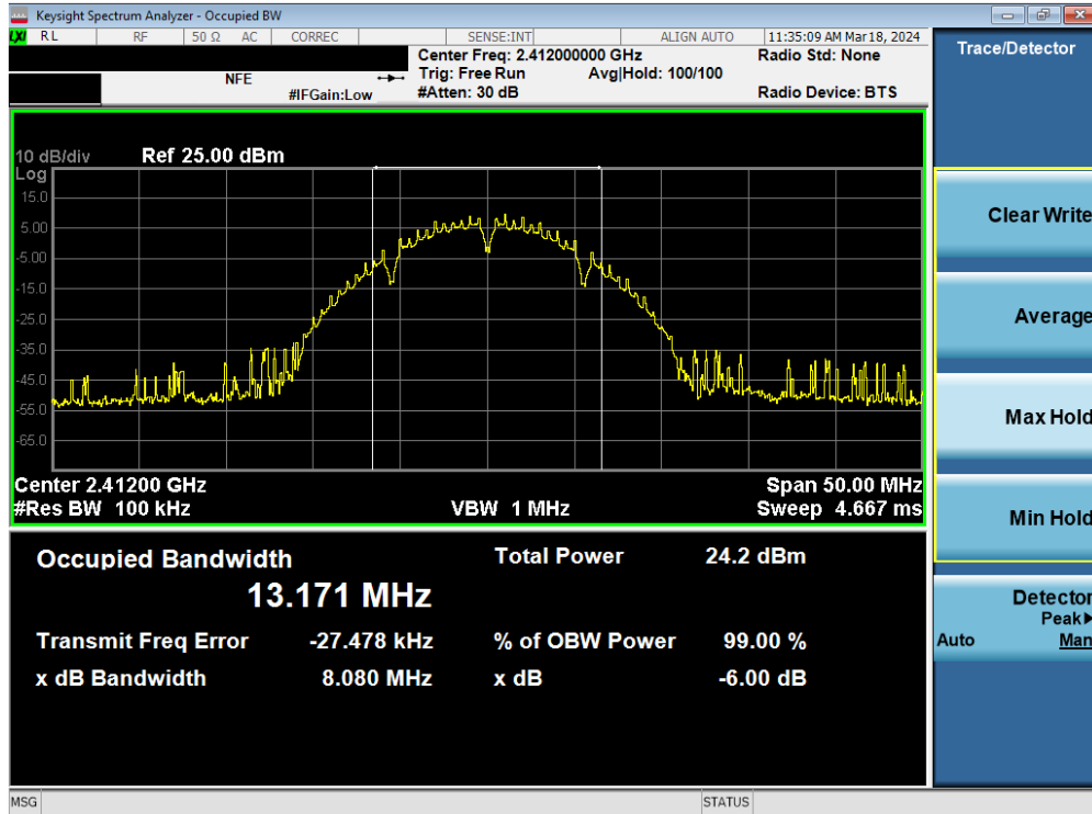
Plot 7-26. 6dB Bandwidth Plot MIMO ANT2 (802.11b – Ch. 1)
