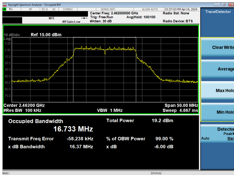
Plot 7-7. 6dB Bandwidth Plot SISO ANT2 (802.11g – Ch. 11)
