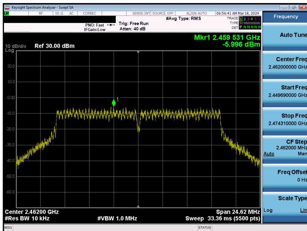
Plot 7-55. Power Spectral Density Plot MIMO ANT1 (802.11g – Ch. 11)
