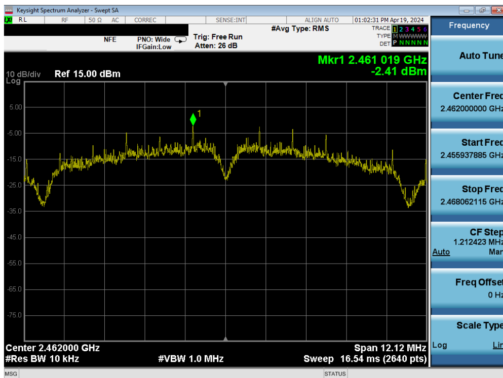
Plot 7-40. Power Spectral Density Plot SISO ANT2 (802.11b – Ch. 11)
