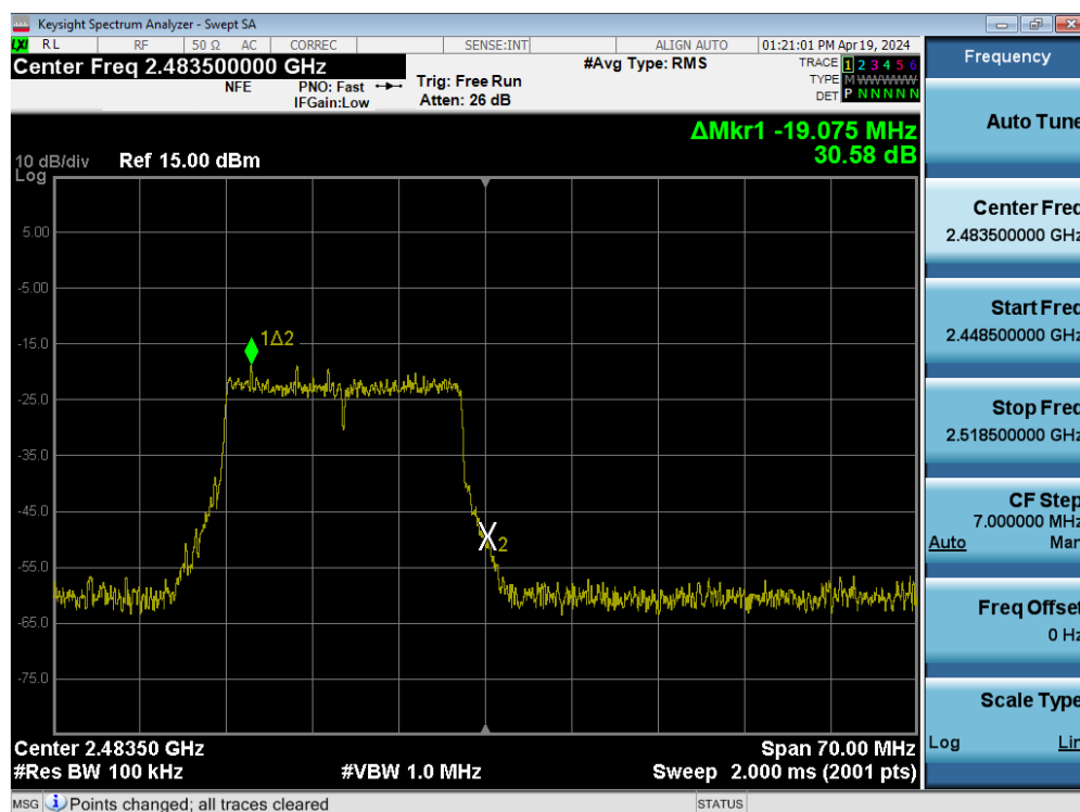
Plot 7-89. Band Edge Plot SISO ANT2 (802.11ax/be (2.4GHz) – Ch. 13)
