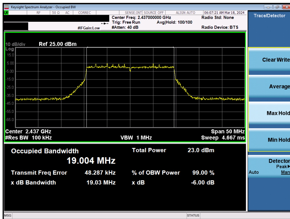
Plot 7-24. 6dB Bandwidth Plot MIMO ANT1 (802.11ax/be (2.4GHz) – Ch. 6)
