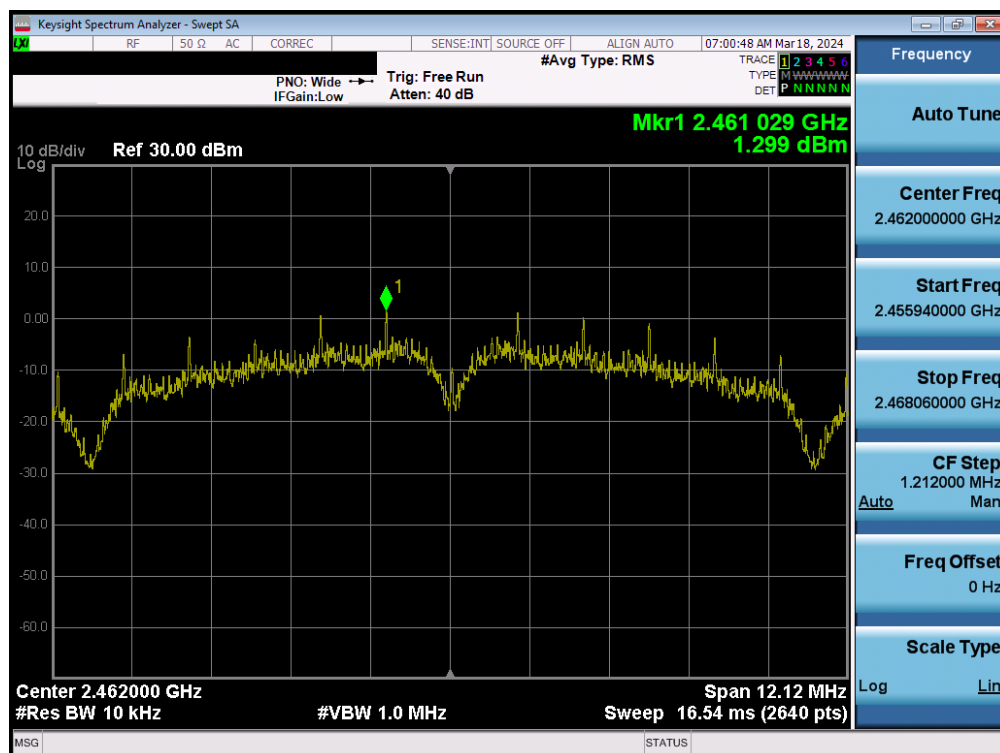
Plot 7-52. Power Spectral Density Plot MIMO ANT1 (802.11b – Ch. 11)
