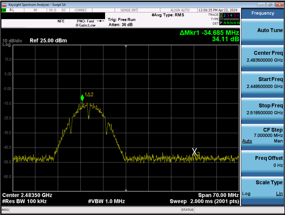
Plot 7-109. Band Edge Plot MIMO ANT2 (802.11b – Ch. 13)
