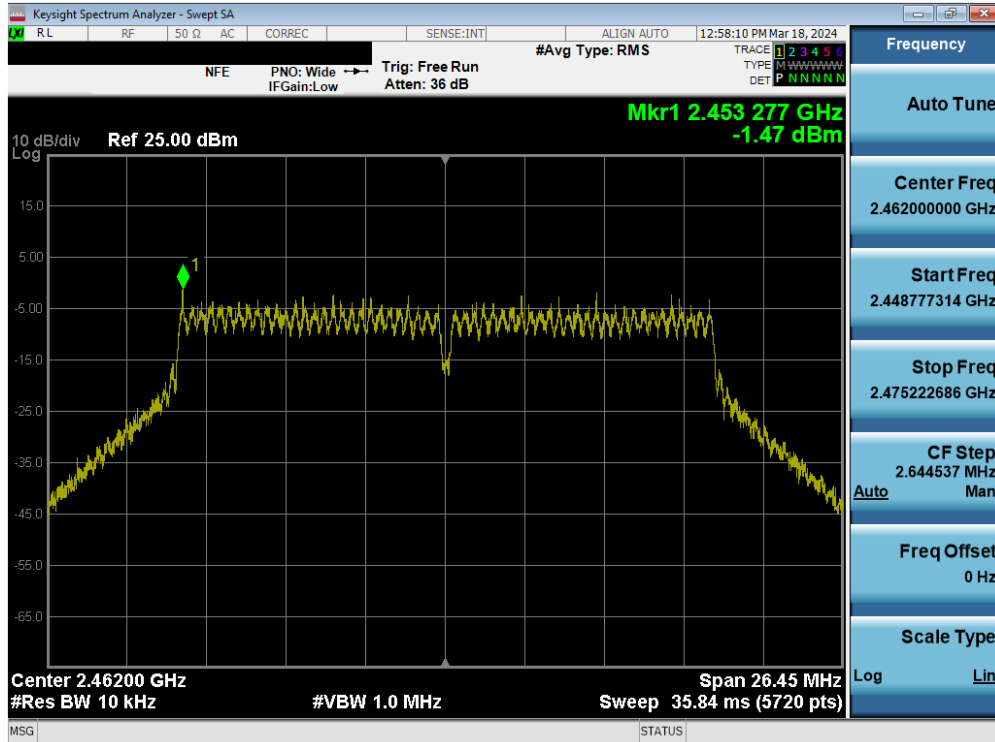
Plot 7-70. Power Spectral Density Plot MIMO ANT2 (802.11n (2.4GHz) – Ch. 11)
