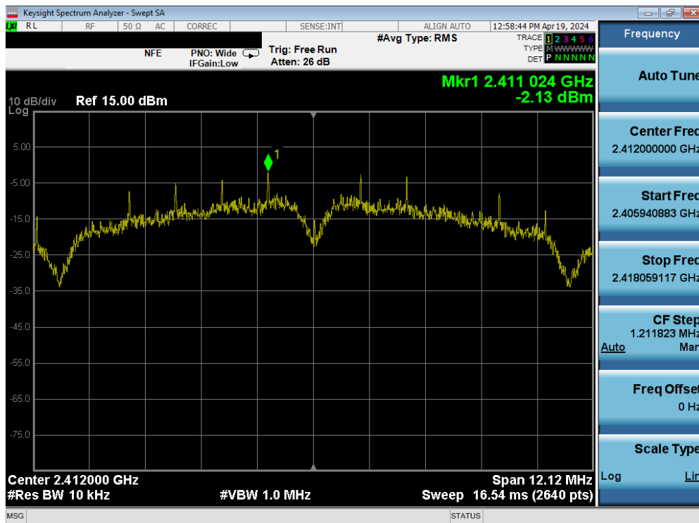
Plot 7-38. Power Spectral Density Plot SISO ANT2 (802.11b – Ch. 1)
