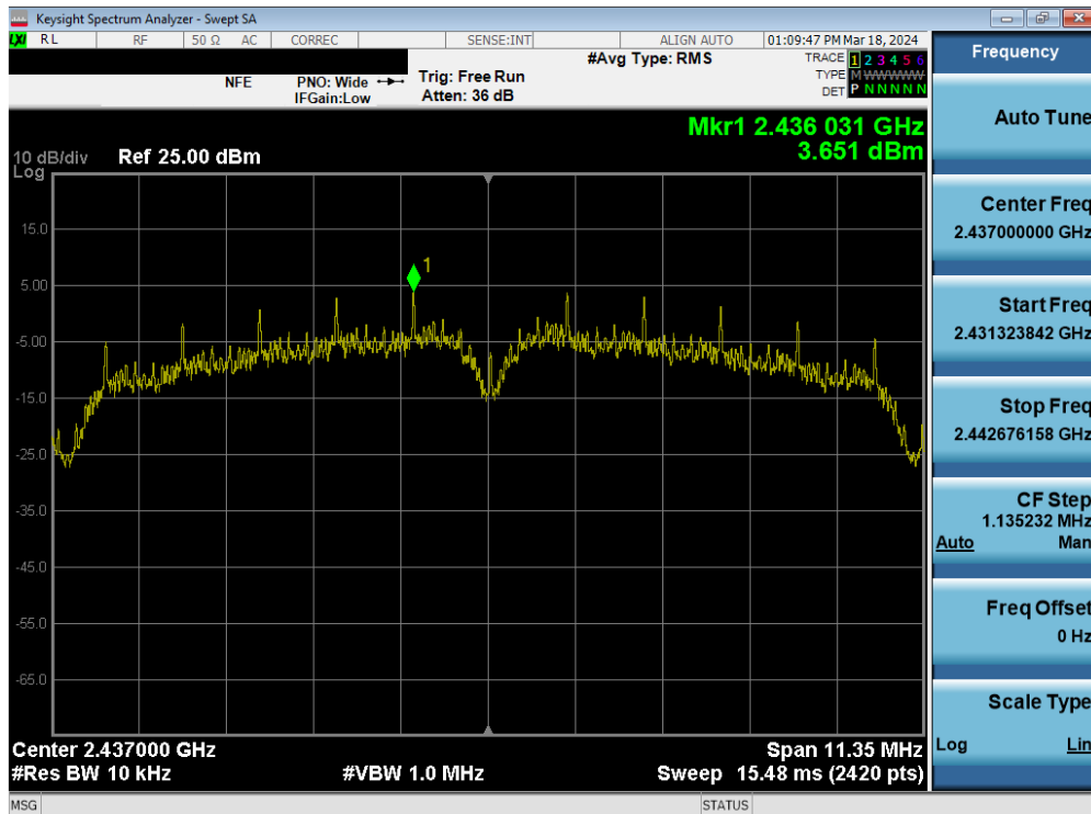
Plot 7-63. Power Spectral Density Plot MIMO ANT2 (802.11b – Ch. 6)
