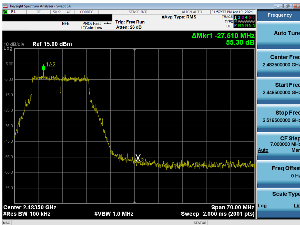
Plot 7-79. Band Edge Plot SISO ANT2 (802.11g - Ch. 11)
