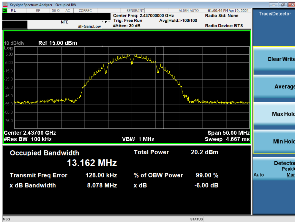
Plot 7-3. 6dB Bandwidth Plot SISO ANT2 (802.11b – Ch. 6)
