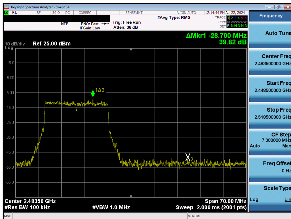
Plot 7-104. Band Edge Plot MIMO ANT1 (802.11ax/be (2.4GHz) - Ch. 12)
