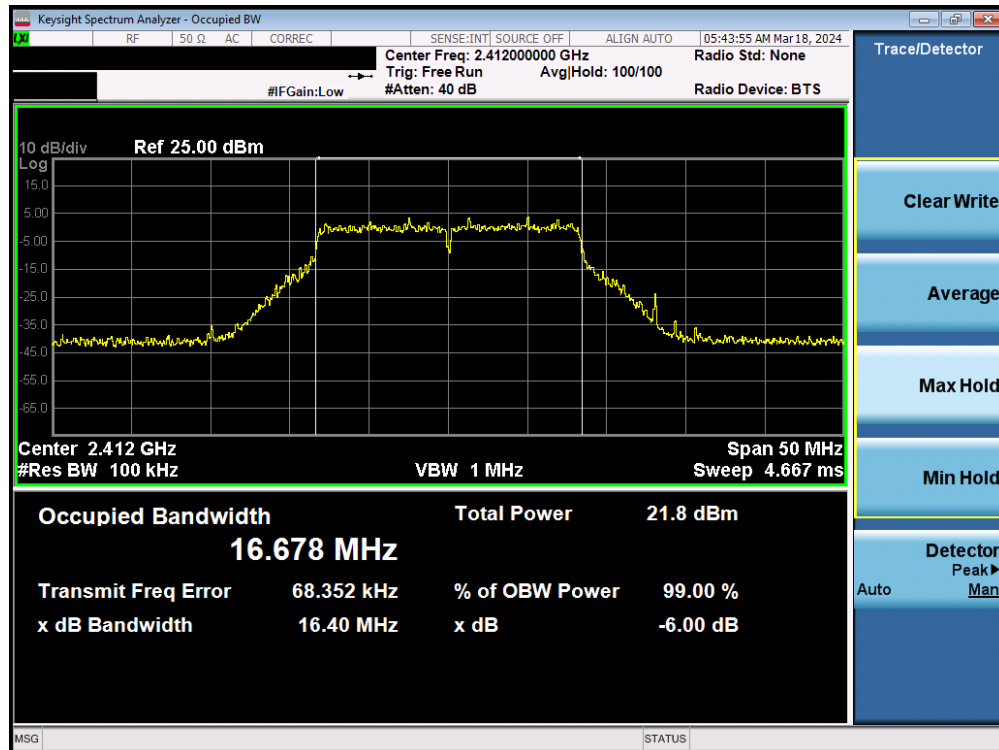
Plot 7-17. 6dB Bandwidth Plot MIMO ANT1 (802.11g – Ch. 1)
