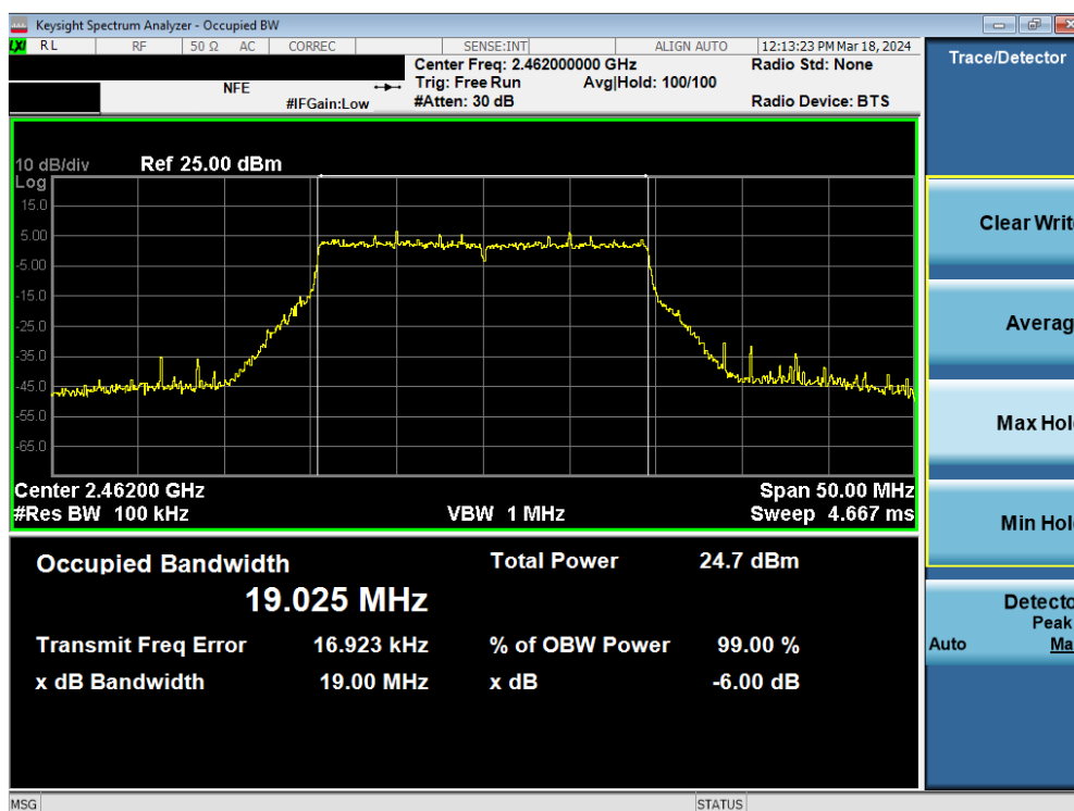
Plot 7-37. 6dB Bandwidth Plot MIMO ANT2 (802.11ax/be (2.4GHz) – Ch. 11)
