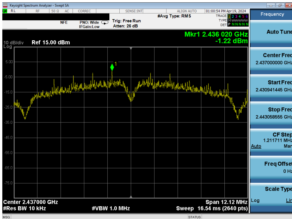
Plot 7-39. Power Spectral Density Plot SISO ANT2 (802.11b – Ch. 6)
