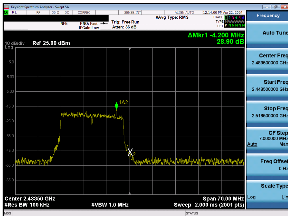
Plot 7-105. Band Edge Plot MIMO ANT1 (802.11ax/be (2.4GHz) - Ch. 13)
