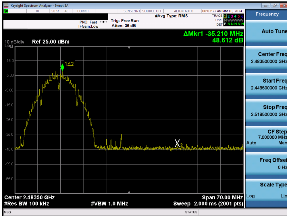
Plot 7-91. Band Edge Plot MIMO ANT1 (802.11b – Ch. 11)
