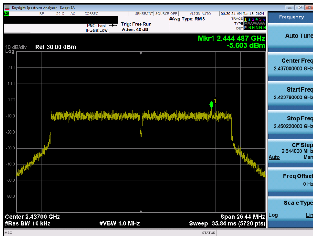
Plot 7-60. Power Spectral Density Plot MIMO ANT1 (802.11ax/be (2.4GHz) – Ch. 6)
