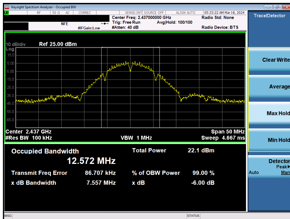
Plot 7-15. 6dB Bandwidth Plot MIMO ANT1 (802.11b – Ch. 6)
