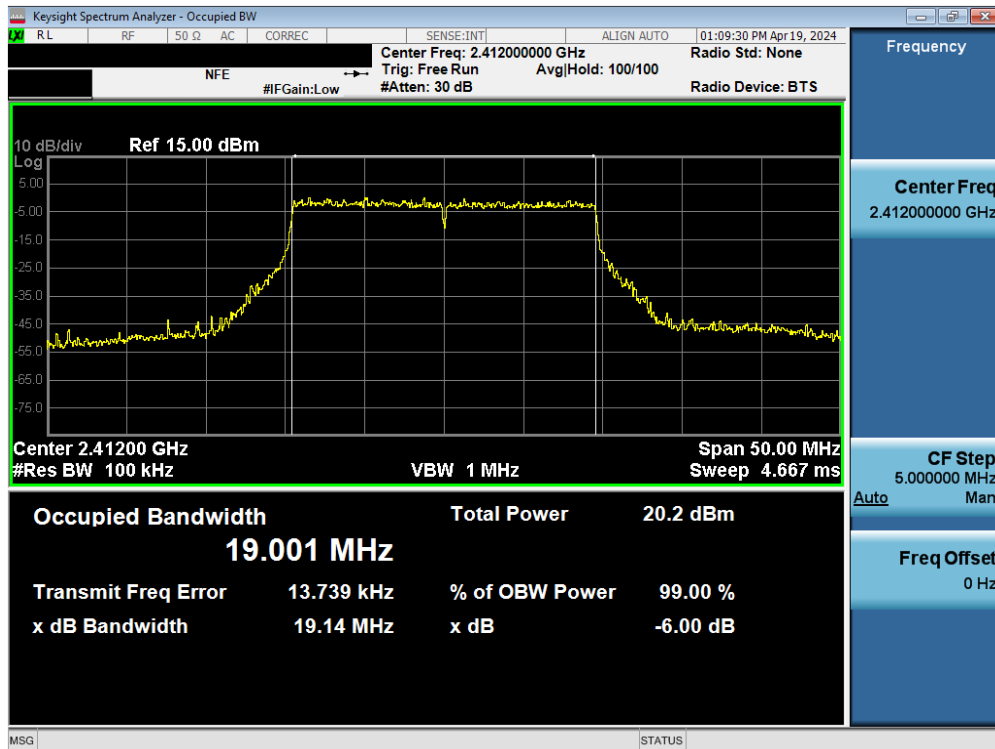
Plot 7-11. 6dB Bandwidth Plot SISO ANT2 (802.11ax/be (2.4GHz) – Ch. 1)
