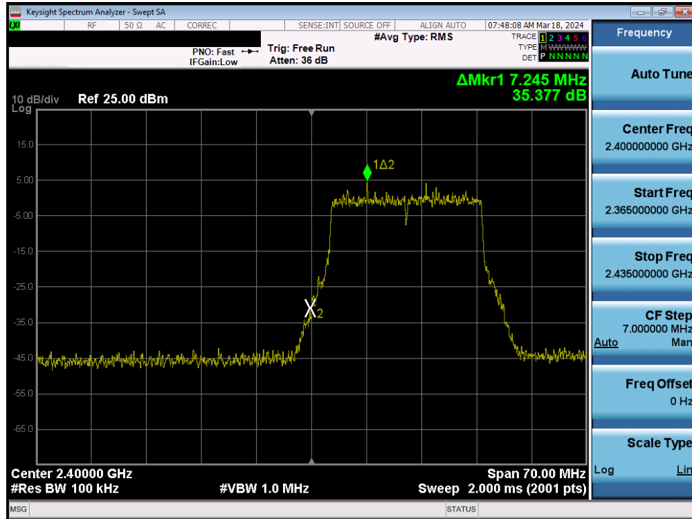
Plot 7-102. Band Edge Plot MIMO ANT1 (802.11ax/be (2.4GHz) – Ch. 1)
