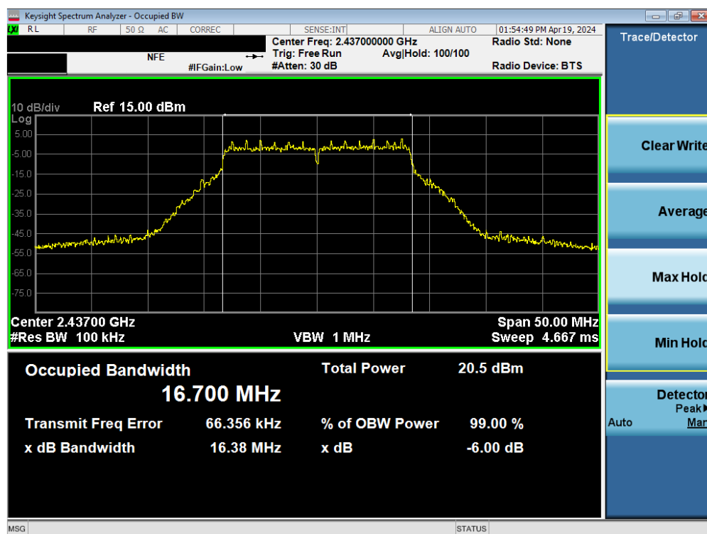
Plot 7-6. 6dB Bandwidth Plot SISO ANT2 (802.11g – Ch. 6)
