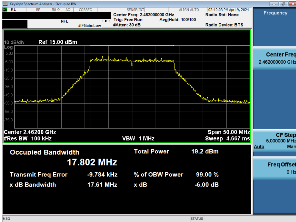
Plot 7-10. 6dB Bandwidth Plot SISO ANT2 (802.11n (2.4GHz) – Ch. 11)
