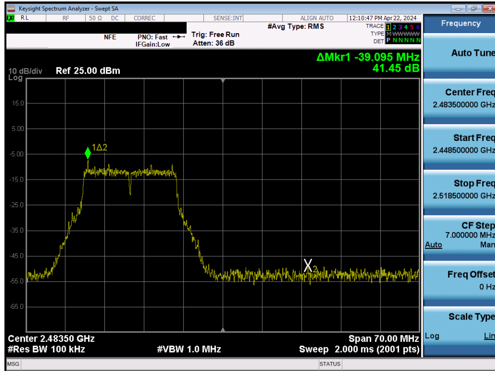
Plot 7-96. Band Edge Plot MIMO ANT1 (802.11g – Ch. 12)
