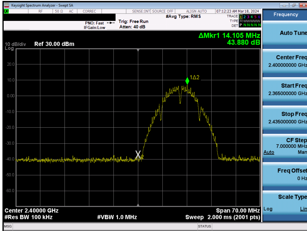
Plot 7-90. Band Edge Plot MIMO ANT1 (802.11b – Ch. 1)
