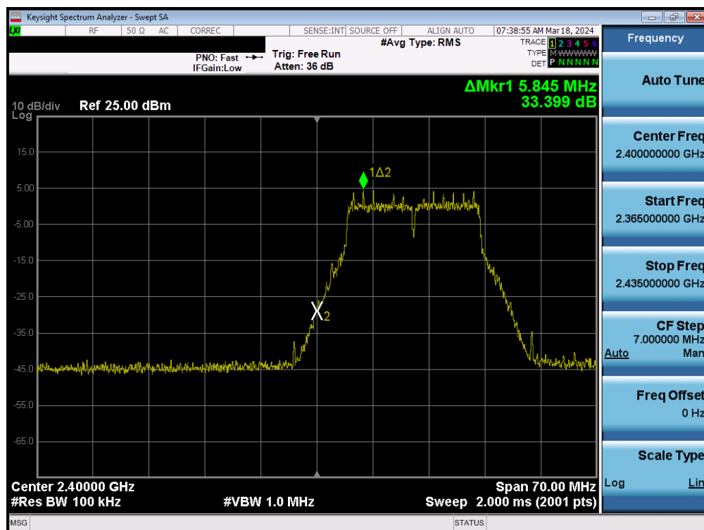
Plot 7-94. Band Edge Plot MIMO ANT1 (802.11g– Ch. 1)
