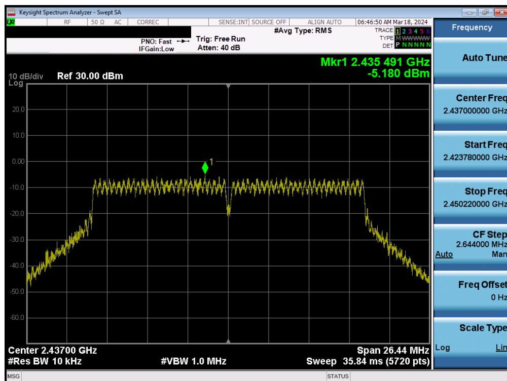
Plot 7-57. Power Spectral Density Plot MIMO ANT1 (802.11n (2.4GHz) – Ch. 6)
