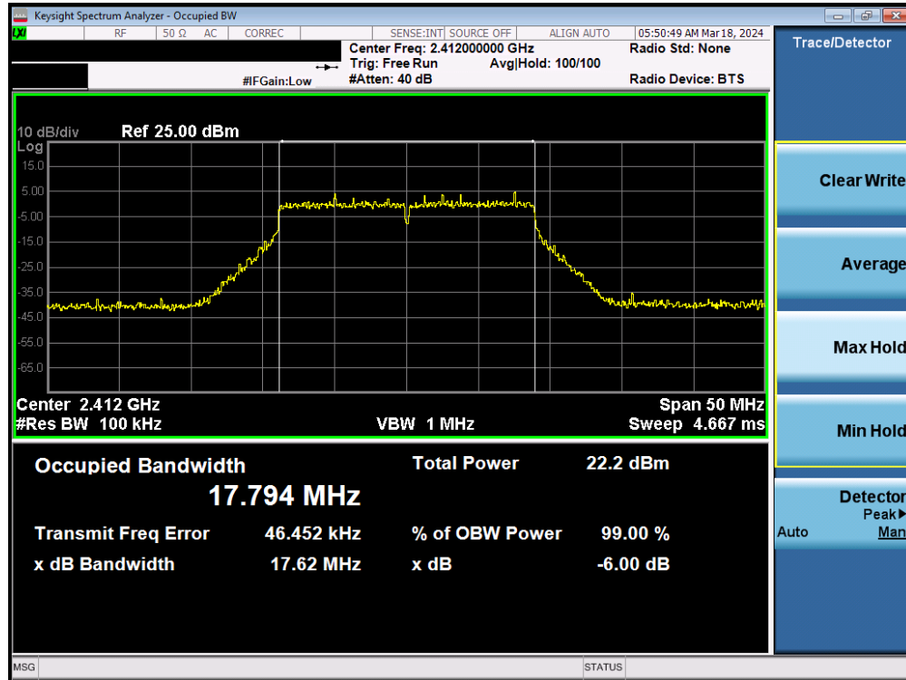
Plot 7-20. 6dB Bandwidth Plot MIMO ANT1 (802.11n (2.4GHz) – Ch. 1)
