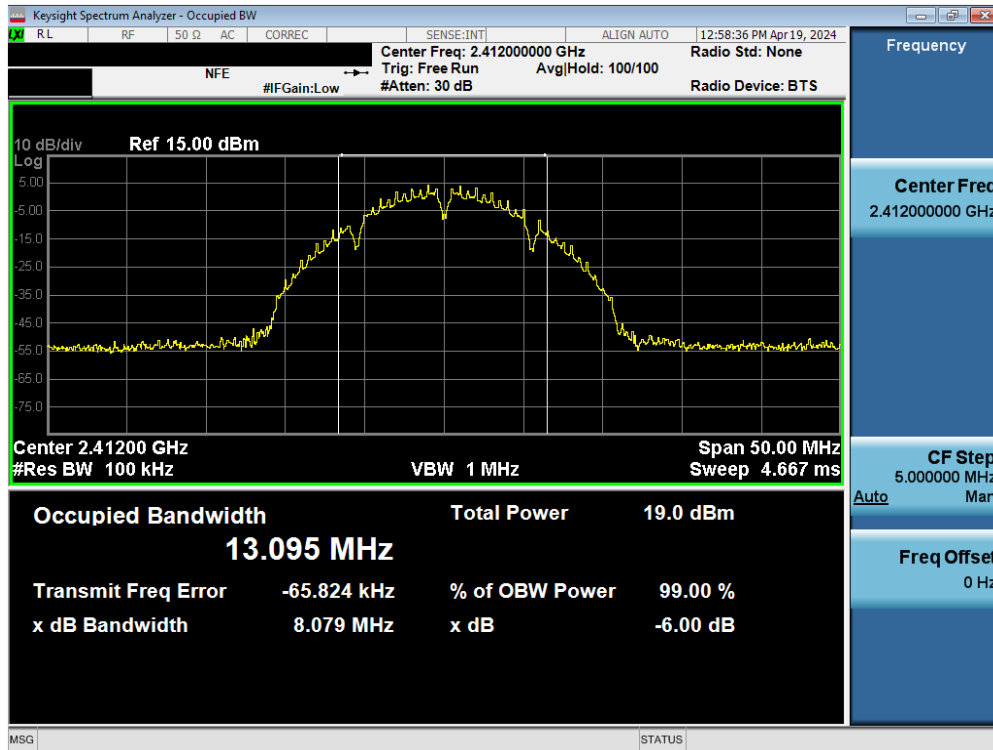
Plot 7-2. 6dB Bandwidth Plot SISO ANT2 (802.11b – Ch. 1)
