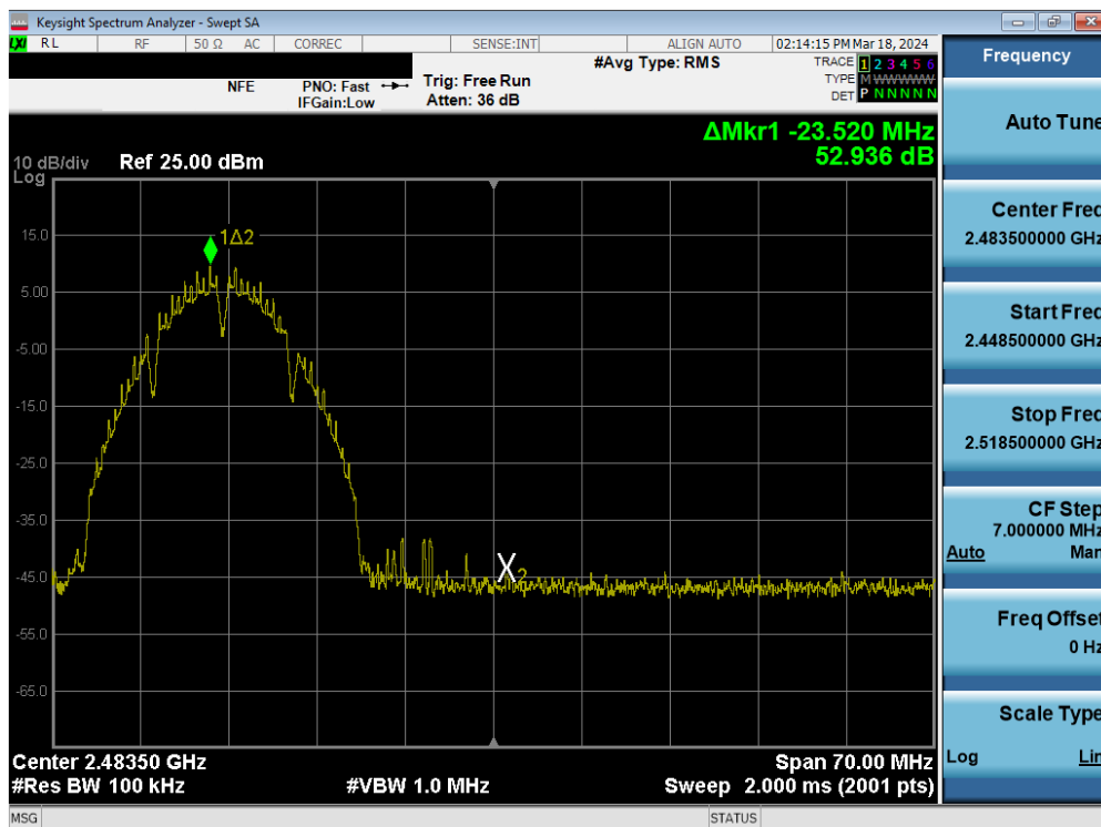
Plot 7-107. Band Edge Plot MIMO ANT2 (802.11b – Ch. 11)
