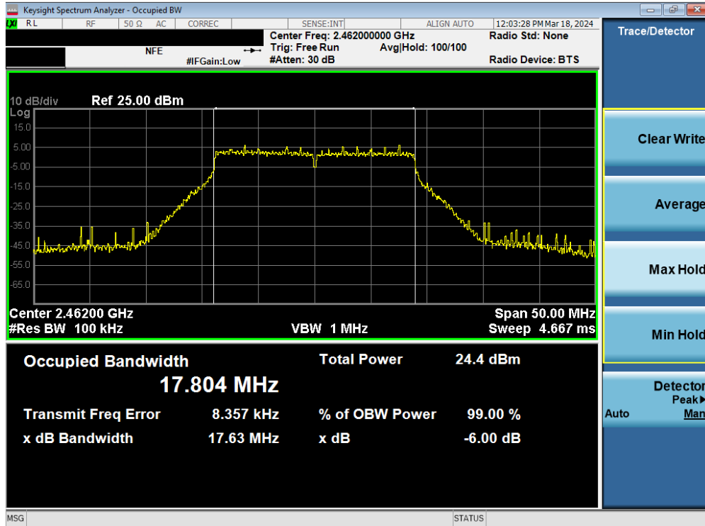
Plot 7-34. 6dB Bandwidth Plot MIMO ANT2 (802.11n (2.4GHz) – Ch. 11)
