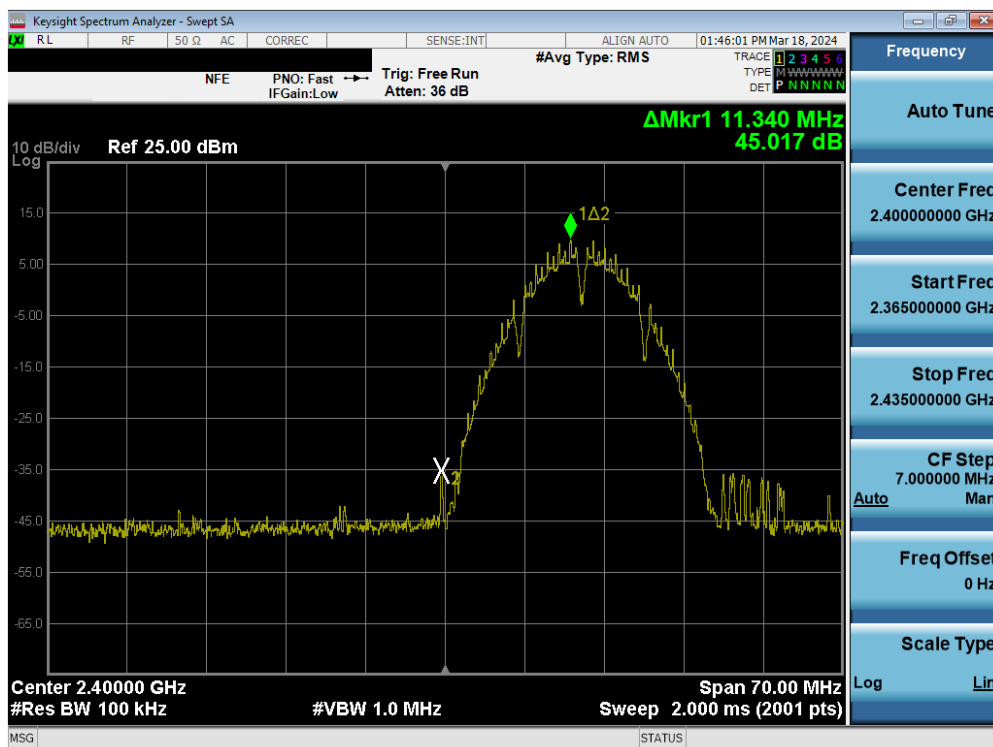
Plot 7-106. Band Edge Plot MIMO ANT2 (802.11b – Ch. 1)
