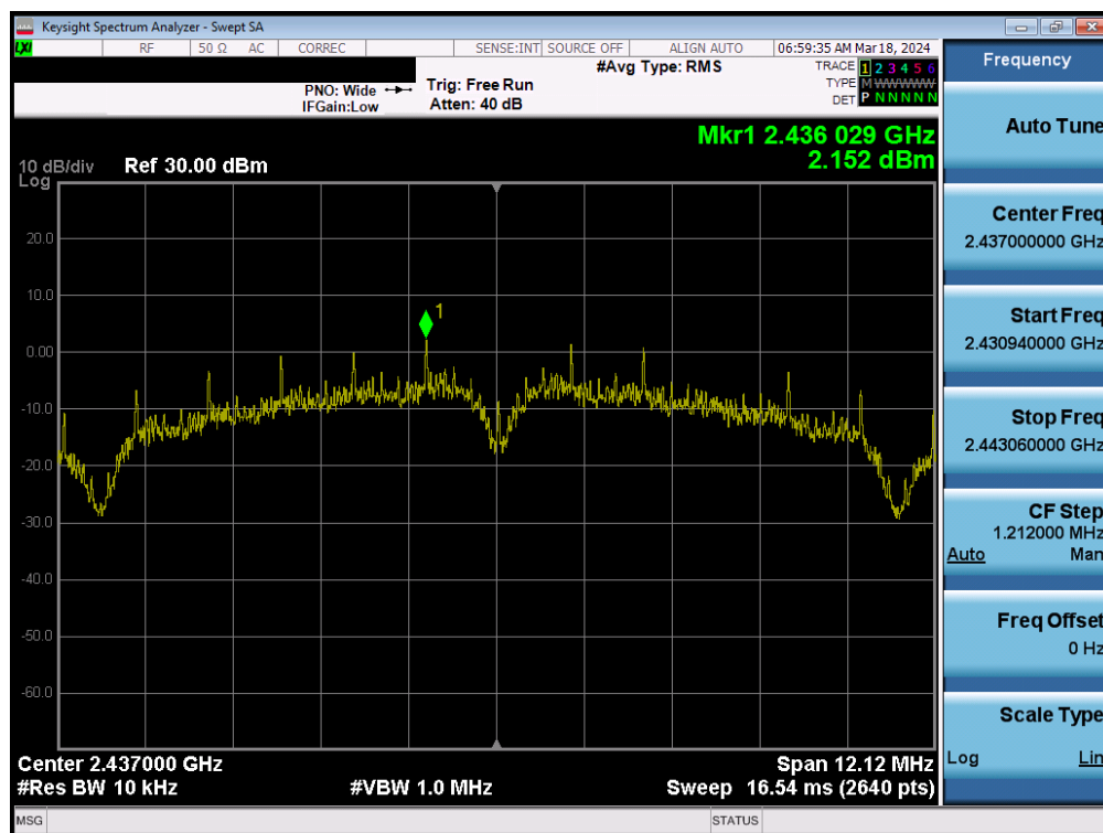
Plot 7-51. Power Spectral Density Plot MIMO ANT1 (802.11b – Ch. 6)
