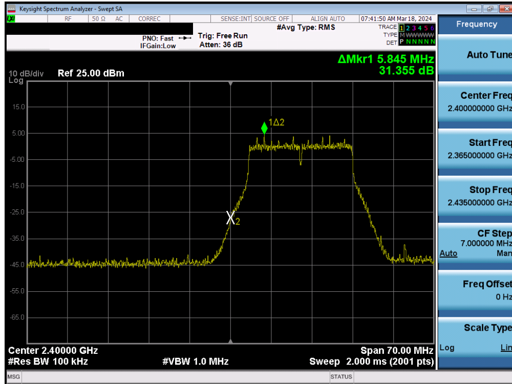
Plot 7-98. Band Edge Plot MIMO ANT1 (802.11n (2.4GHz) – Ch. 1)
