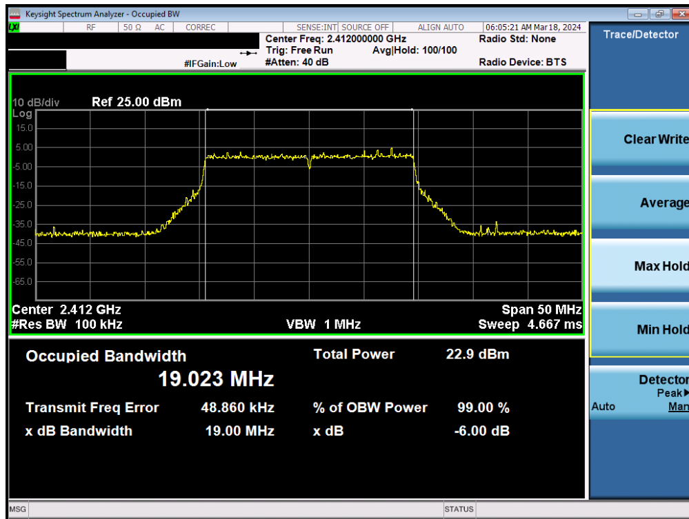
Plot 7-23. 6dB Bandwidth Plot MIMO ANT1 (802.11ax/be (2.4GHz) – Ch. 1)
