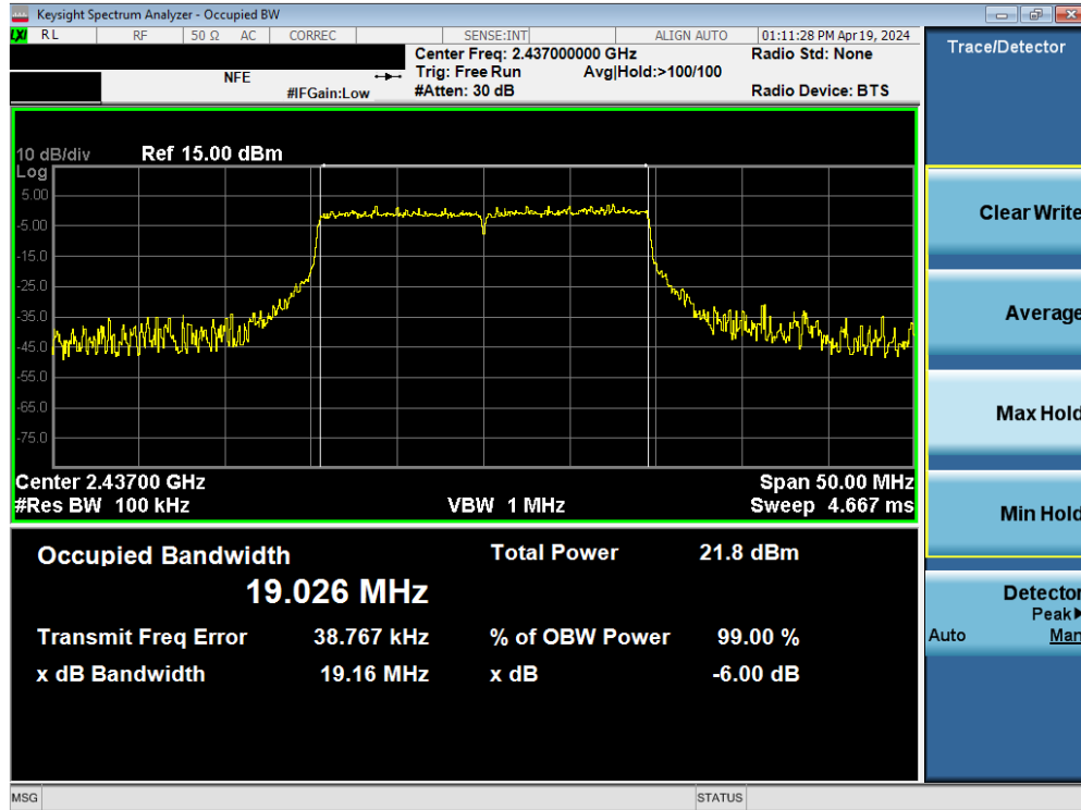
Plot 7-12. 6dB Bandwidth Plot SISO ANT2 (802.11ax/be (2.4GHz) – Ch. 6)
