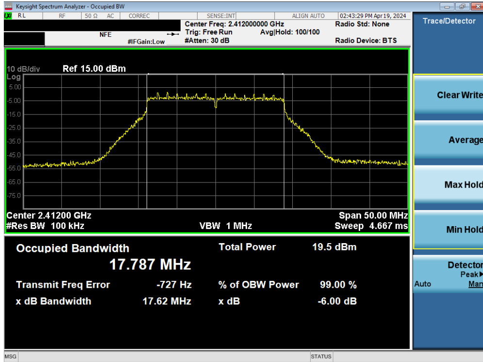
Plot 7-8. 6dB Bandwidth Plot SISO ANT2 (802.11n (2.4GHz) – Ch. 1)
