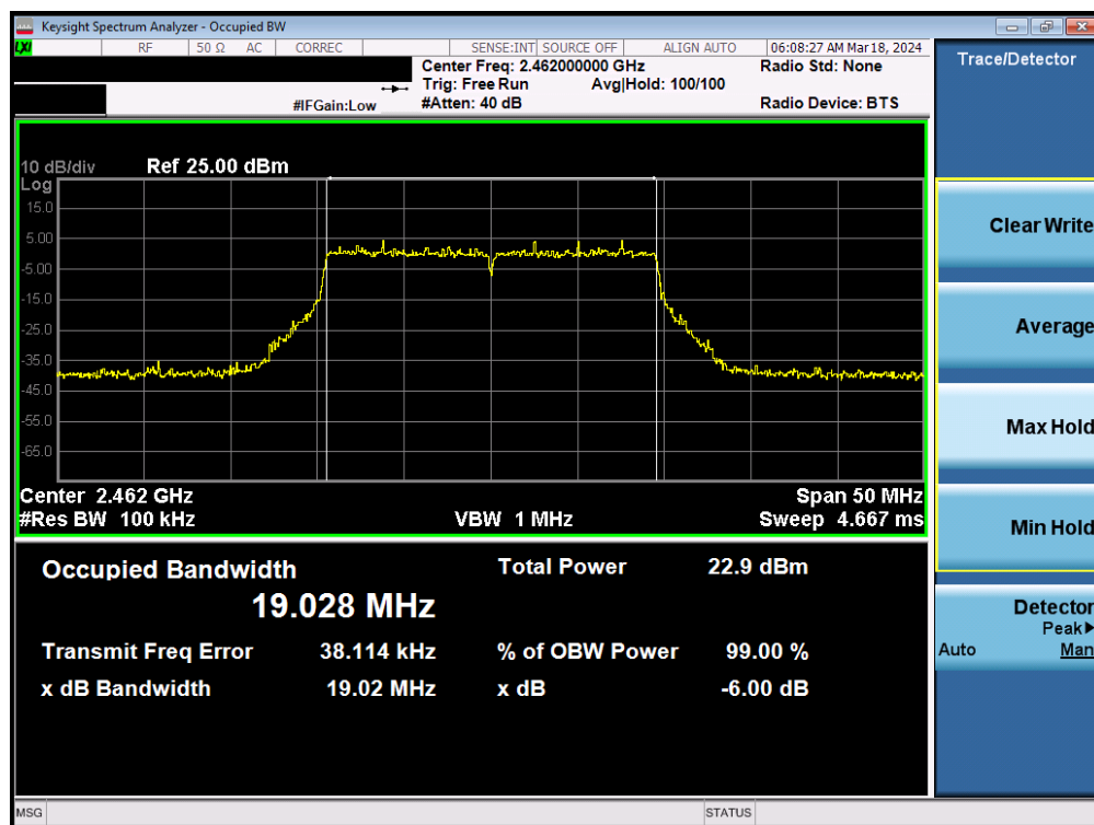
Plot 7-25. 6dB Bandwidth Plot MIMO ANT1 (802.11ax/be (2.4GHz) – Ch. 11)
