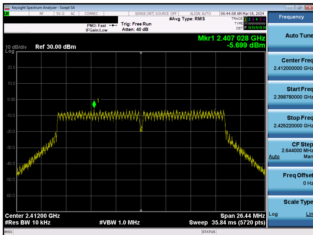
Plot 7-56. Power Spectral Density Plot MIMO ANT1 (802.11n (2.4GHz) – Ch. 1)
