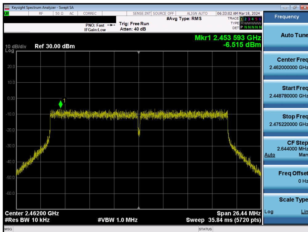
Plot 7-61. Power Spectral Density Plot MIMO ANT1 (802.11ax/be (2.4GHz) – Ch. 11)
