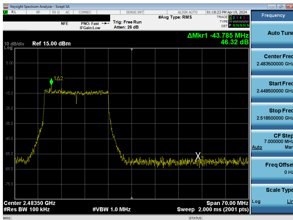
Plot 7-88. Band Edge Plot SISO ANT2 (802.11ax/be (2.4GHz) – Ch. 12)
