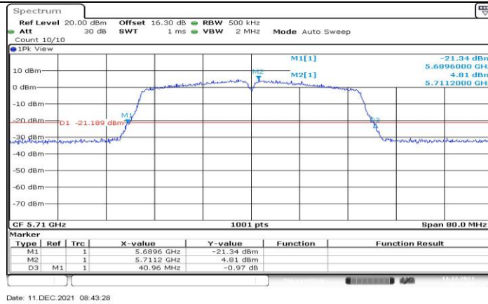
11AC40MIMO Ant1 5710
