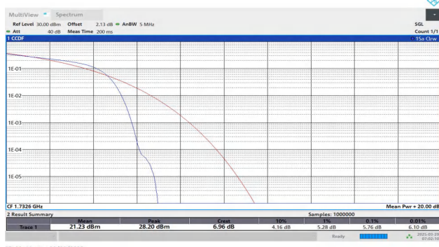
Band4-1413-2-PASS
