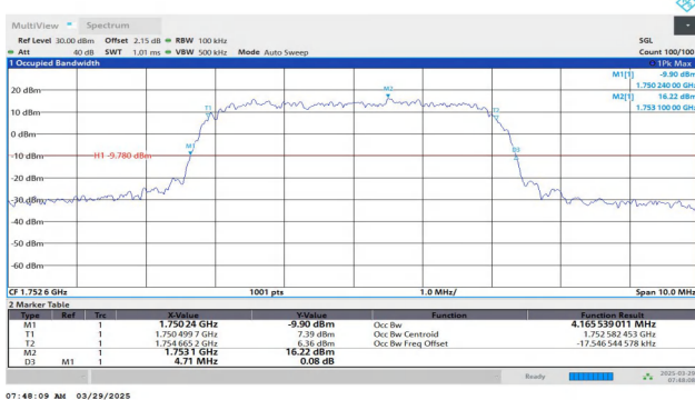
Band4-1513-3-PASS
