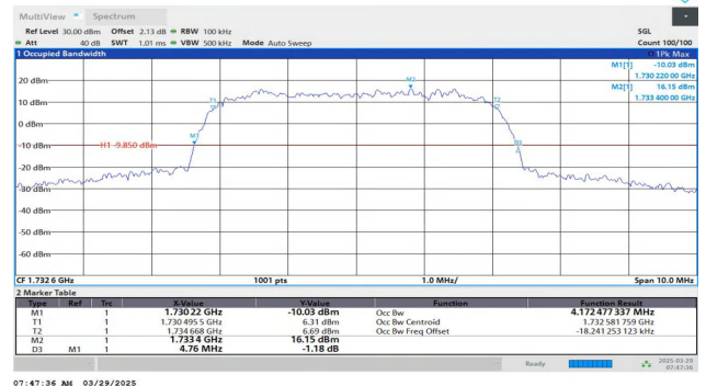
Band4-1413-3-PASS
