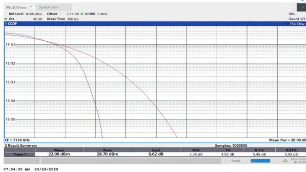
Band4-1312-3-PASS
