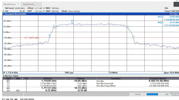
Band4-1312-3-PASS
