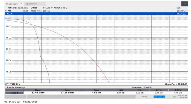
Band4-1513-4-PASS
