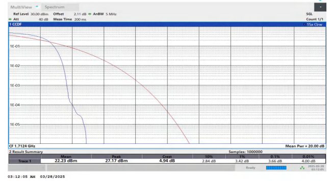
Band4-1312-2-PASS
