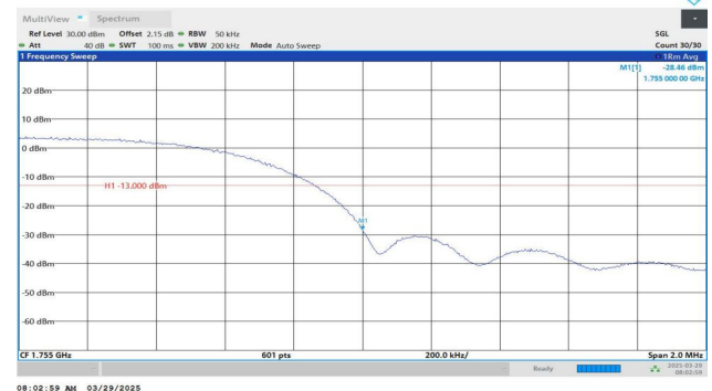
Band4-1513-3-PASS
