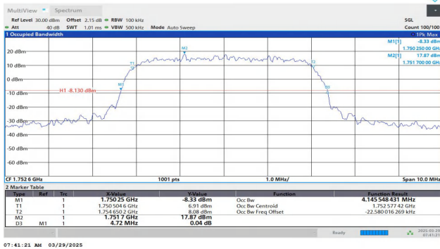
Band4-1513-1-PASS
