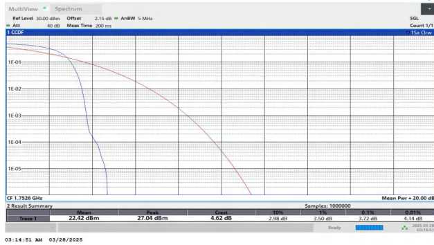
Band4-1513-3-PASS
