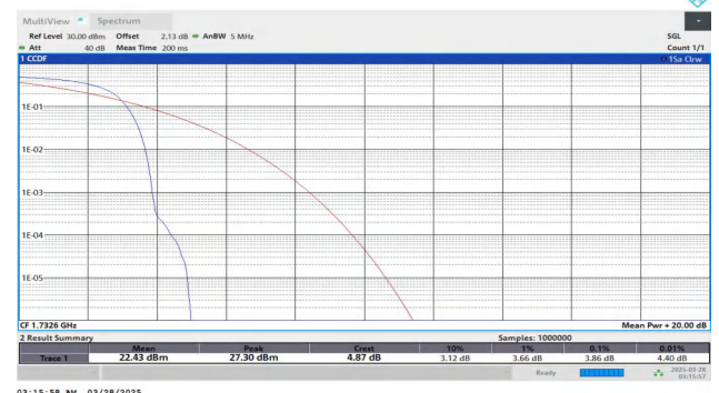
Band4-1413-4-PASS
