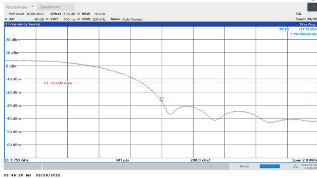
Band4-1513-1-PASS
