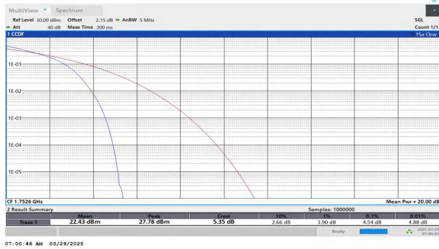
Band4-1513-1-PASS
