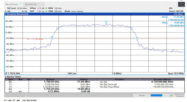
Band4-1513-2-PASS
