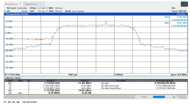
Band4-1312-2-PASS
