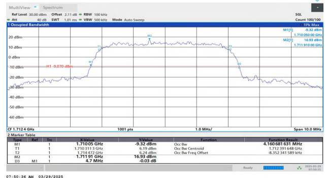
Band4-1312-4-PASS
