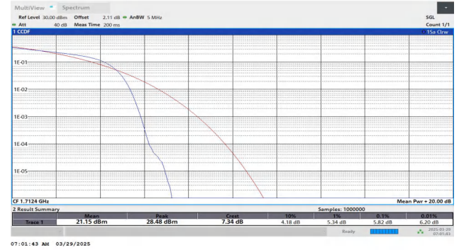
Band4-1312-2-PASS
