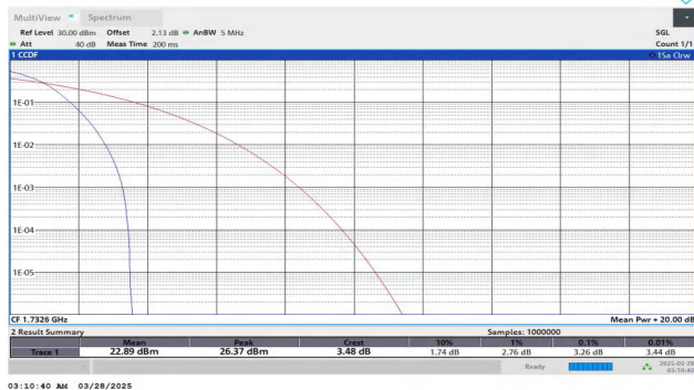
Band4-1413-1-PASS
