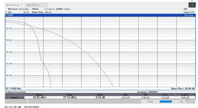
Band4-1413-2-PASS
