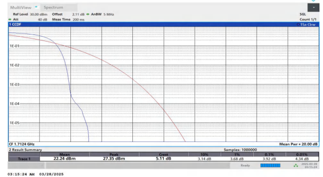
Band4-1312-4-PASS
