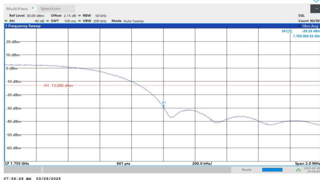
Band4-1513-2-PASS
