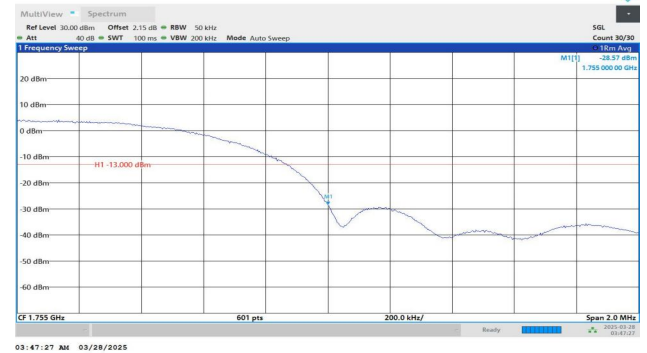
Band4-1513-2-PASS
