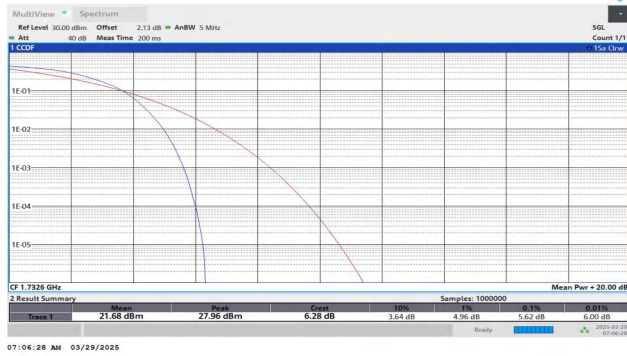
Band4-1413-4-PASS
