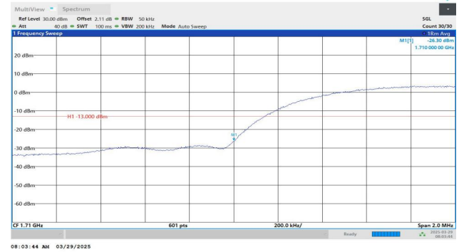
Band4-1312-4-PASS
