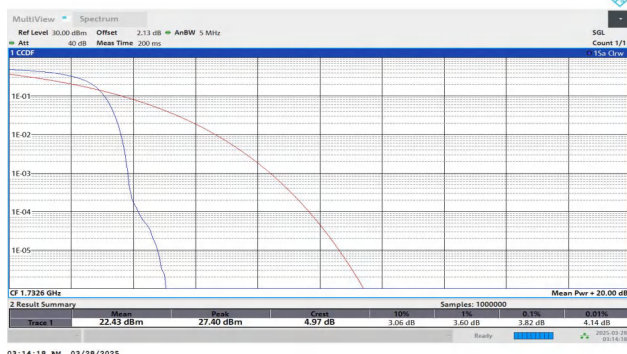
Band4-1413-3-PASS
