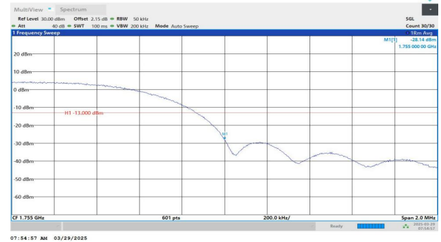
Band4-1513-1-PASS
