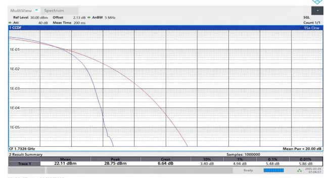
Band4-1413-3-PASS
