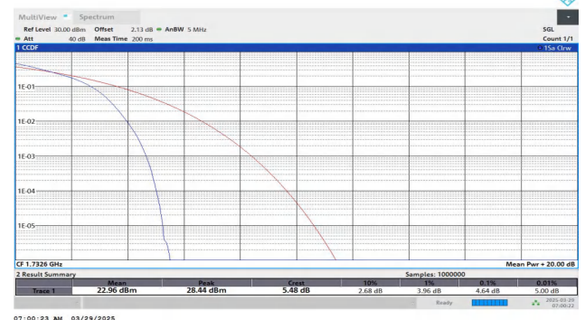
Band4-1413-1-PASS
