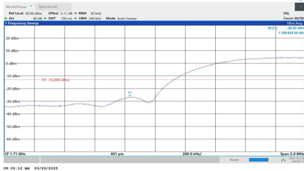
Band4-1312-5-PASS
