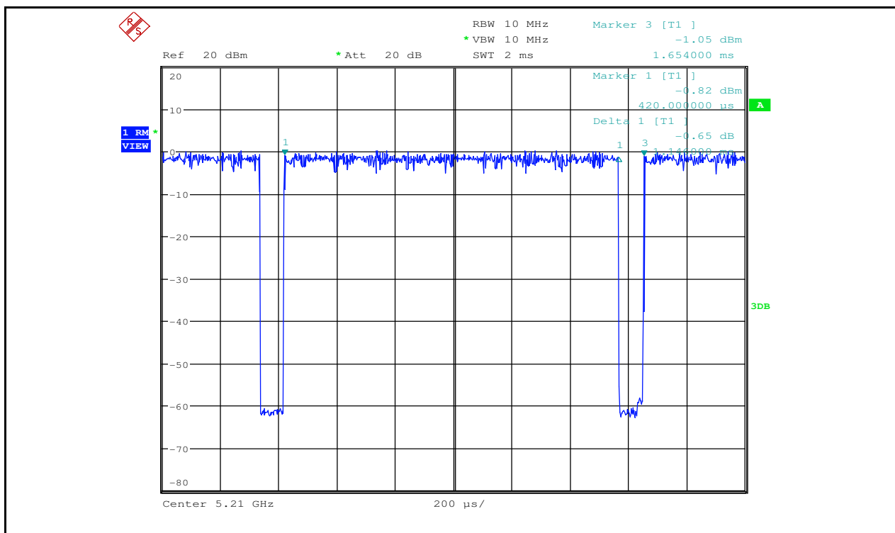
Duty Cycle_11AC80_5210_Ant2
