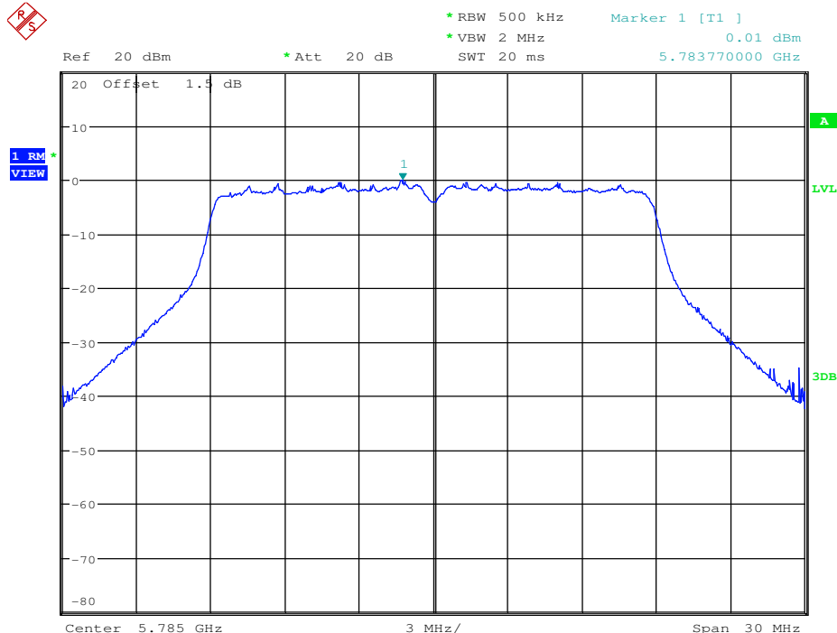
Maximum Power Spectral Density_TNVN_11AC20_5785_Ant2
