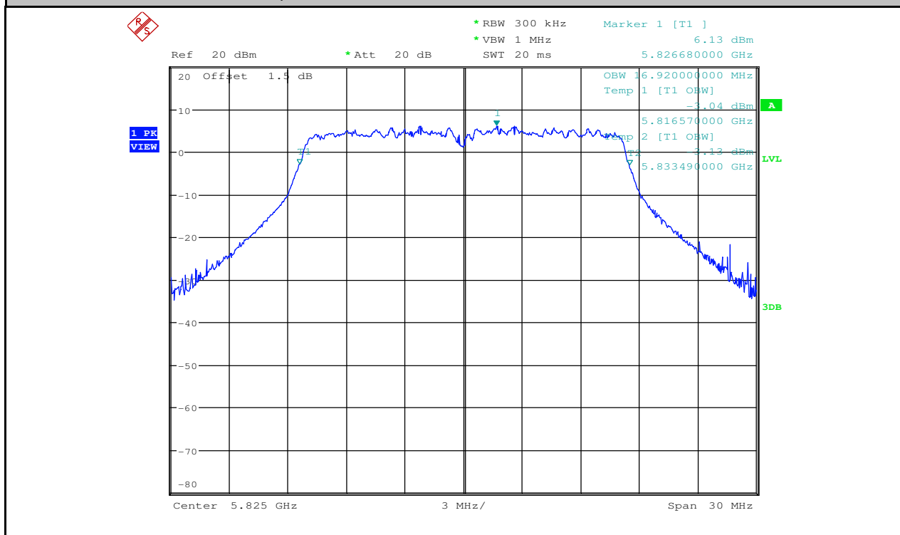
Occupied Bandwidth Measurement_11N20_5180_Ant1
