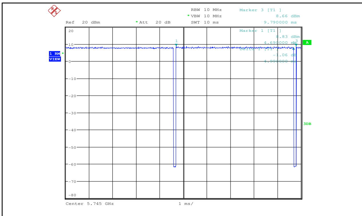
Duty Cycle_11N20_5745_Ant2
