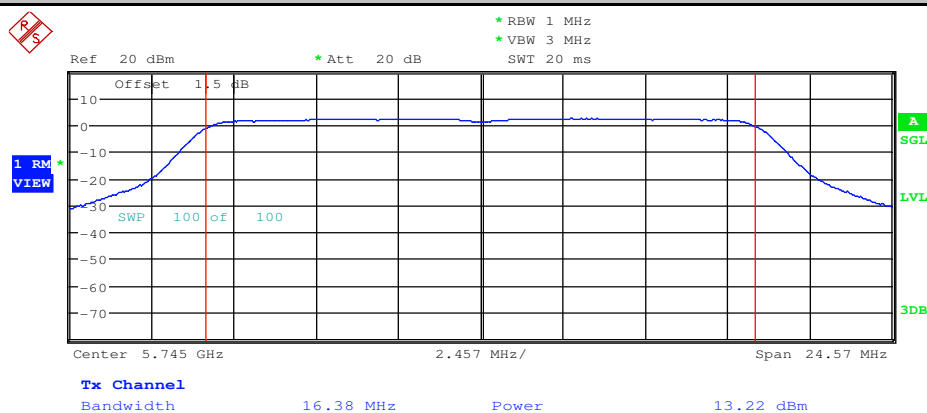
Maximum Conduct Output Power_11A_5745_Ant2
