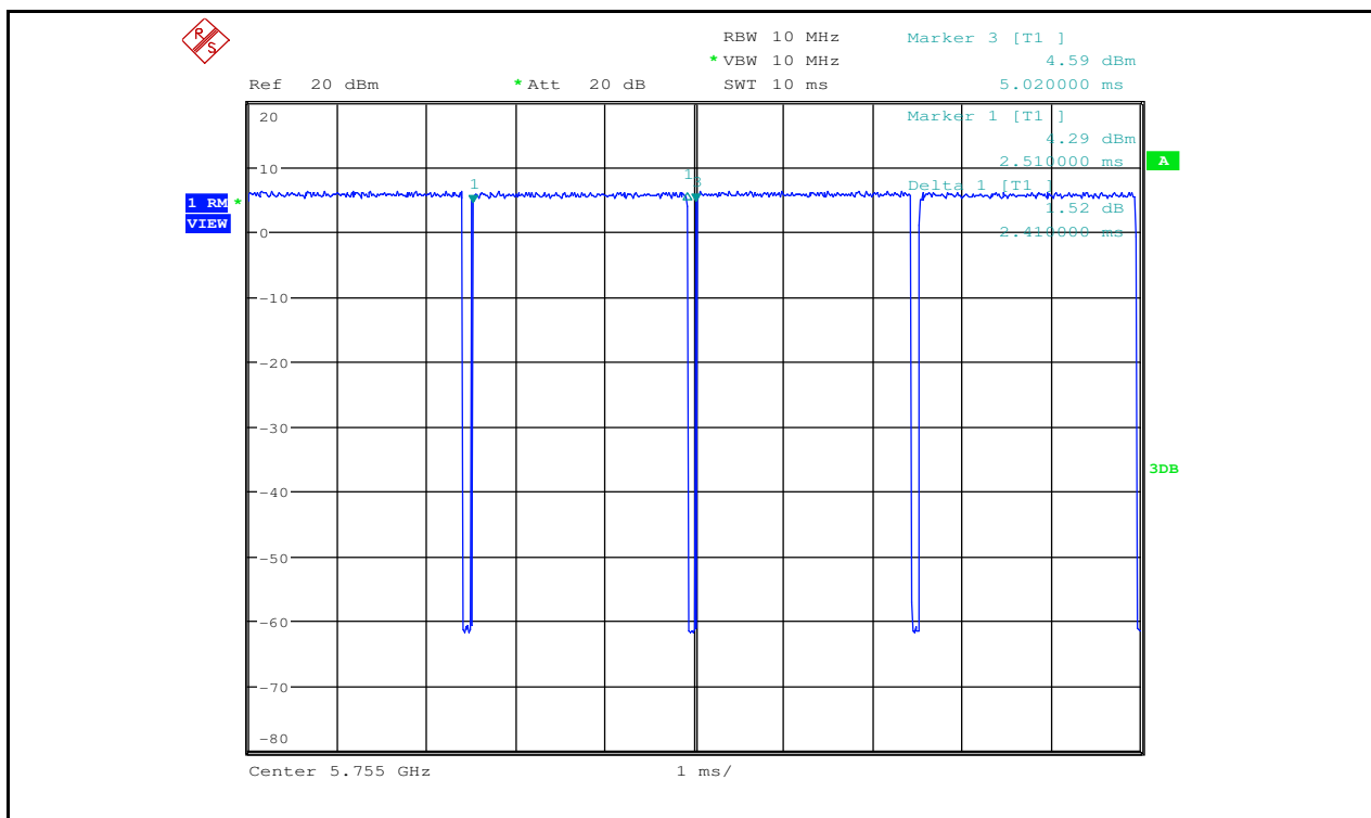
Duty Cycle_11AC40_5755_Ant2
