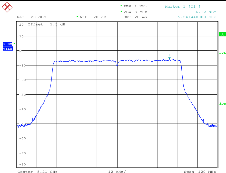
Maximum Power Spectral Density_TNVN_11AC80_5210_Ant2
