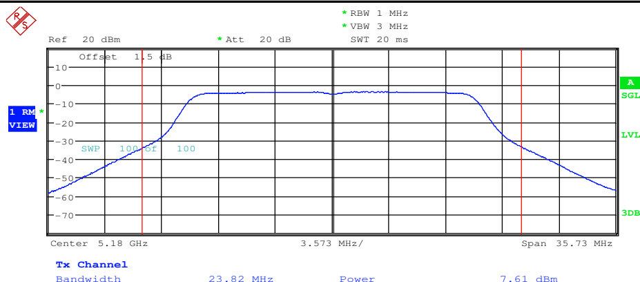
Maximum Conduct Output Power_11N20_5180_Ant2
