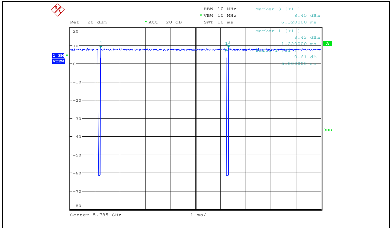
Duty Cycle_11N20_5785_Ant2
