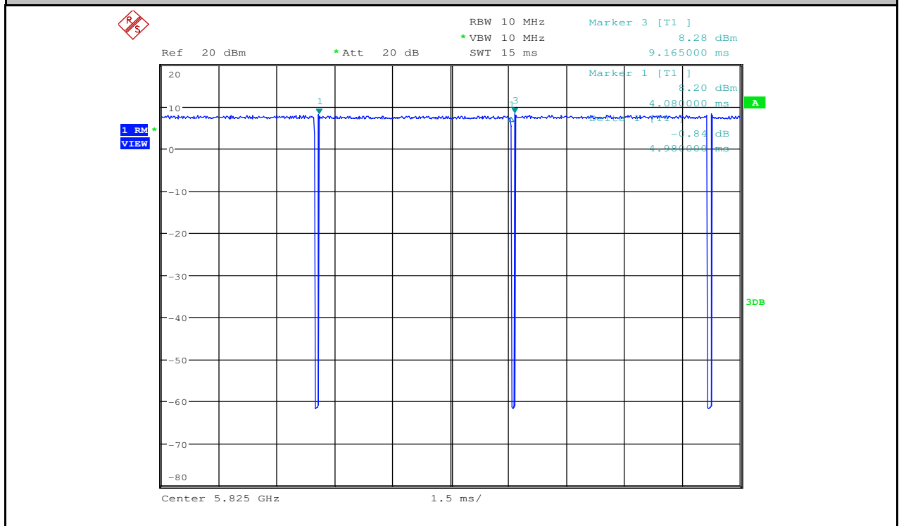
Duty Cycle_11AC80_5210_Ant1
