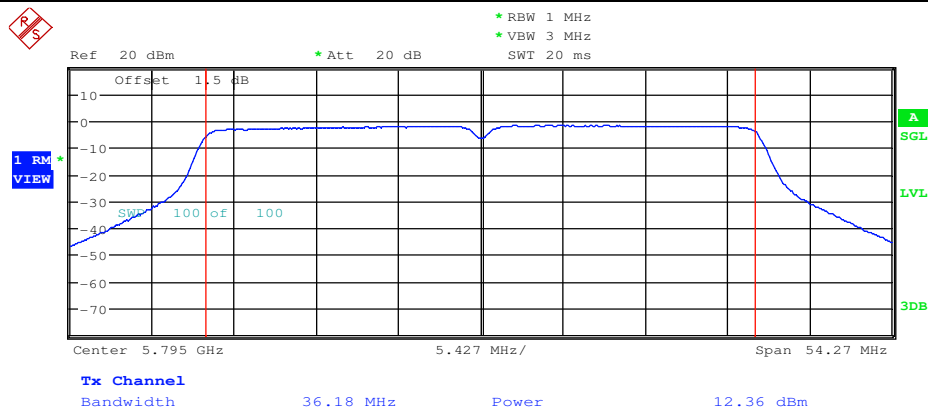
Maximum Conduct Output Power_11N40_5795_Ant2
