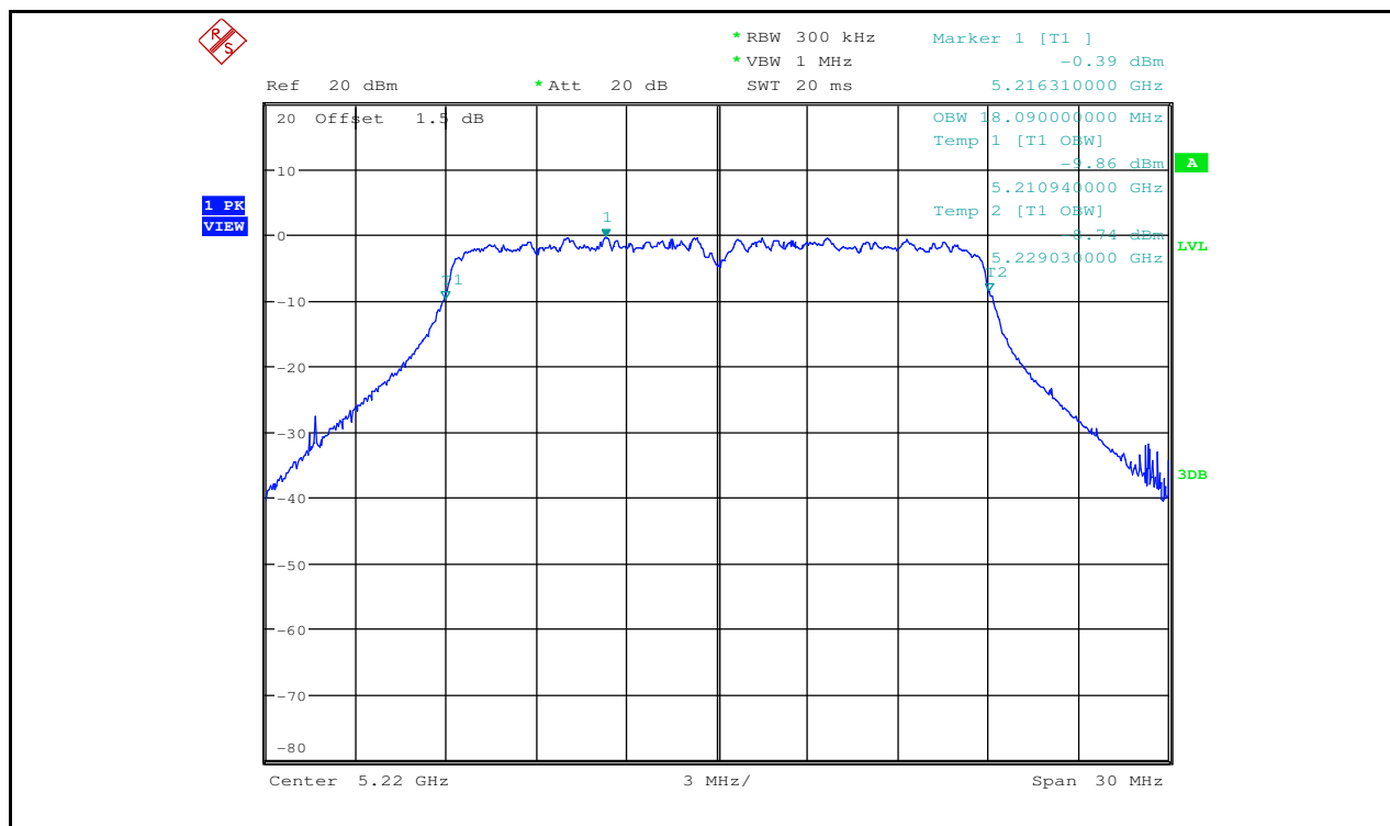
Occupied Bandwidth Measurement_11N20_5220_Ant2
