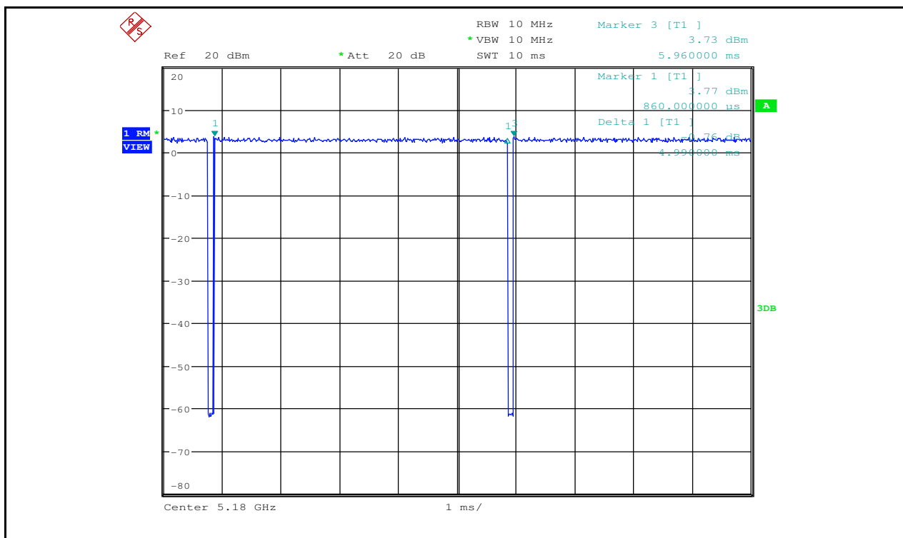
Duty Cycle_11N20_5180_Ant2
