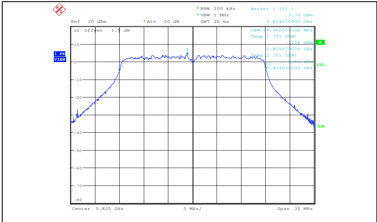
Occupied Bandwidth Measurement_11AC20_5825_Ant2
