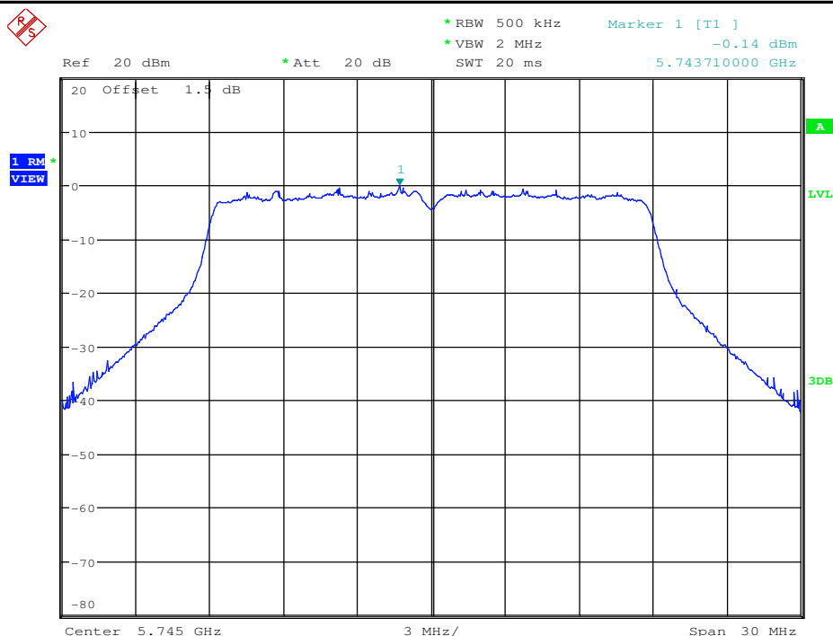
Maximum Power Spectral Density_TNVN_11AC20_5745_Ant2
