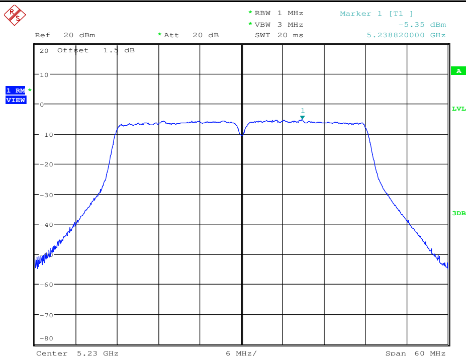
Maximum Power Spectral Density_TNVN_11AC40_5230_Ant2
