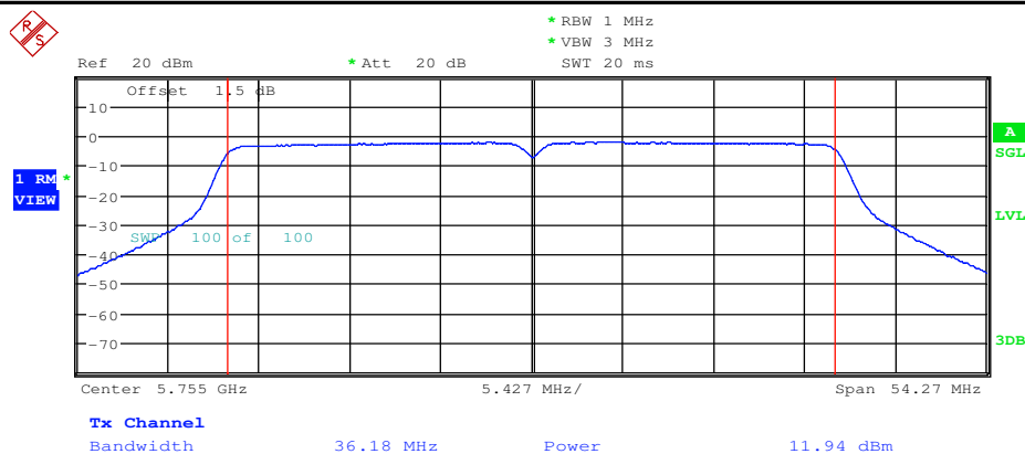
Maximum Conduct Output Power_11AC40_5755_Ant2
