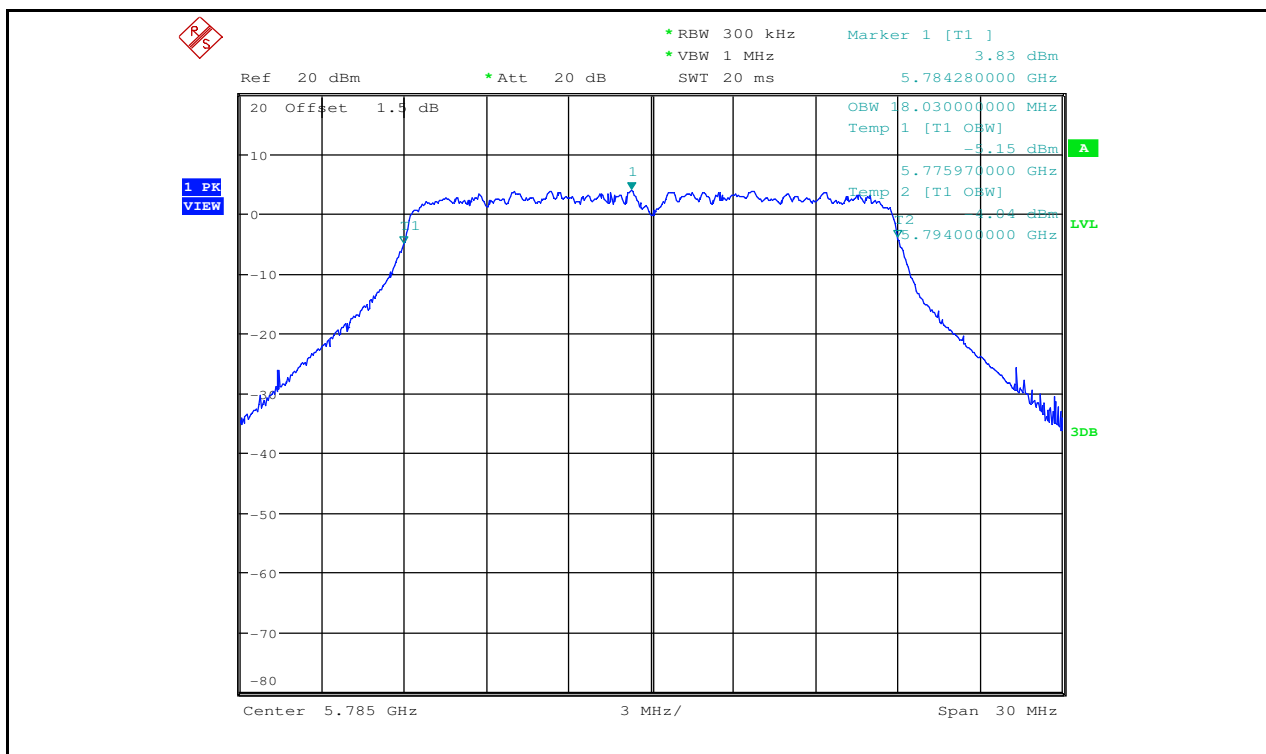
Occupied Bandwidth Measurement_11N20_5785_Ant2
