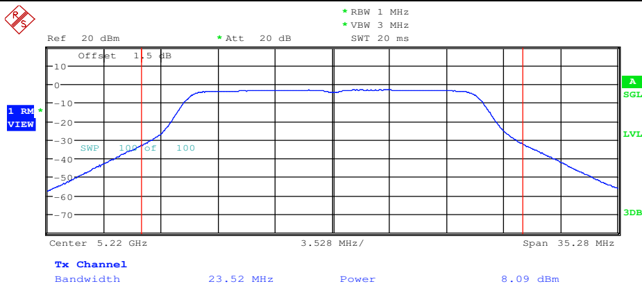
Maximum Conduct Output Power_11N20_5220_Ant2
