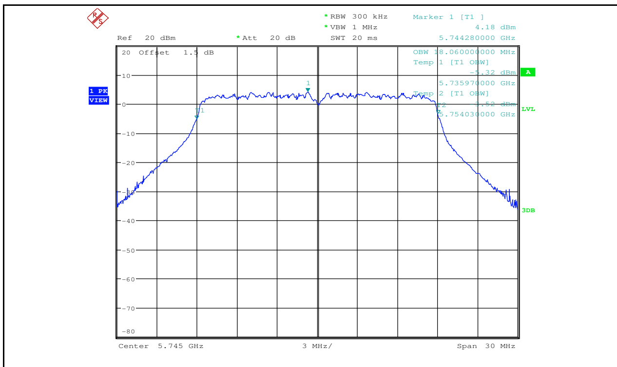
Occupied Bandwidth Measurement_11AC20_5745_Ant2
