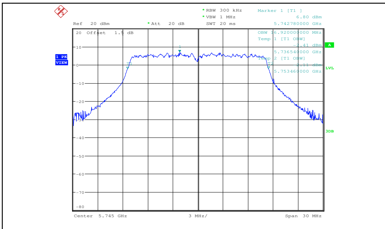
Occupied Bandwidth Measurement_11A_5745_Ant2
