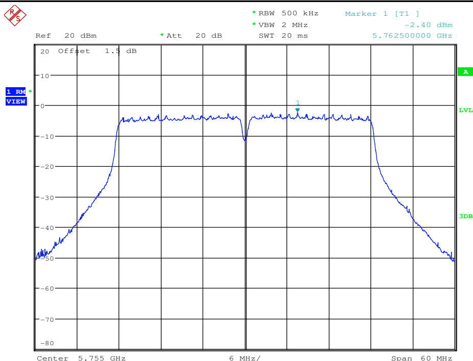
Maximum Power Spectral Density_TNVN_11N40_5755_Ant2
