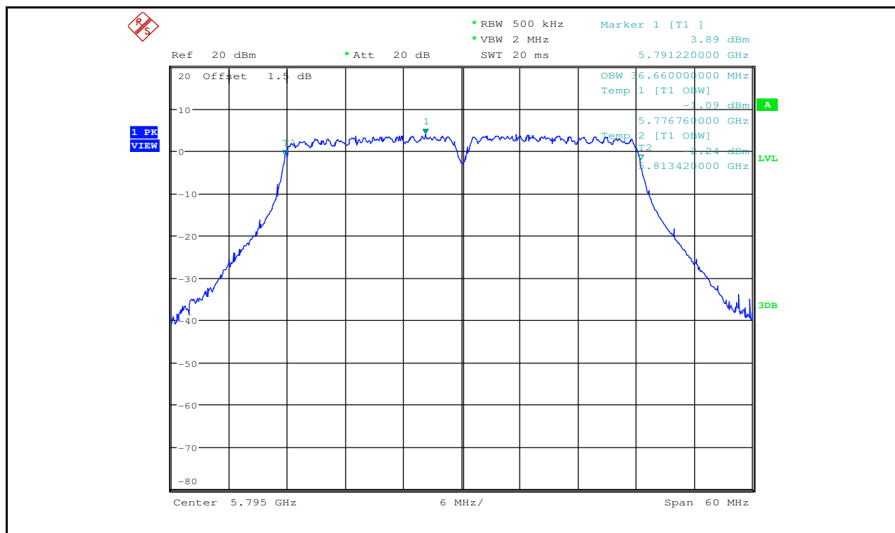
Occupied Bandwidth Measurement_11N40_5795_Ant2
