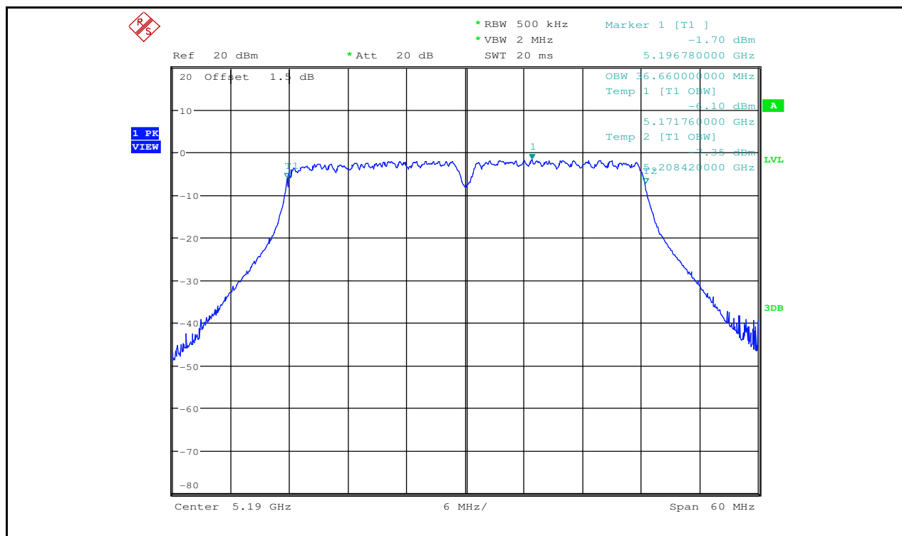
Occupied Bandwidth Measurement_11N40_5190_Ant2
