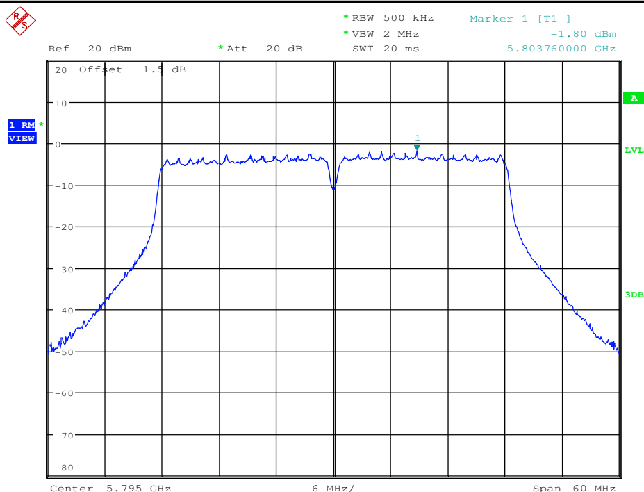
Maximum Power Spectral Density_TNVN_11AC40_5795_Ant2
