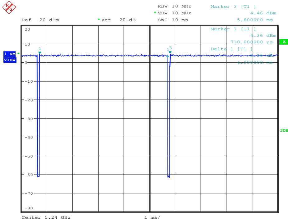
Duty Cycle_11N20_5240_Ant2
