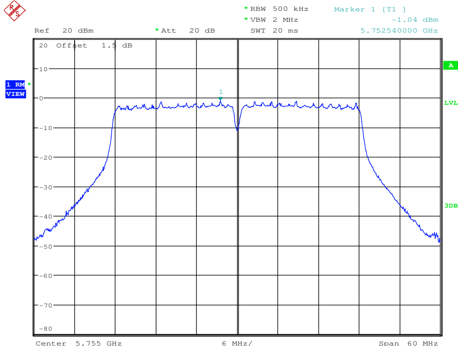
Maximum Power Spectral Density_TNVN_11AC40_5755_Ant2
