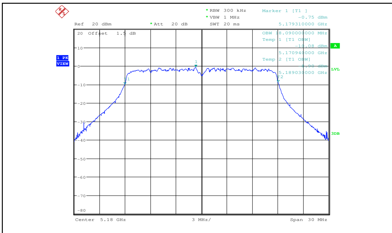
Occupied Bandwidth Measurement_11N20_5180_Ant2
