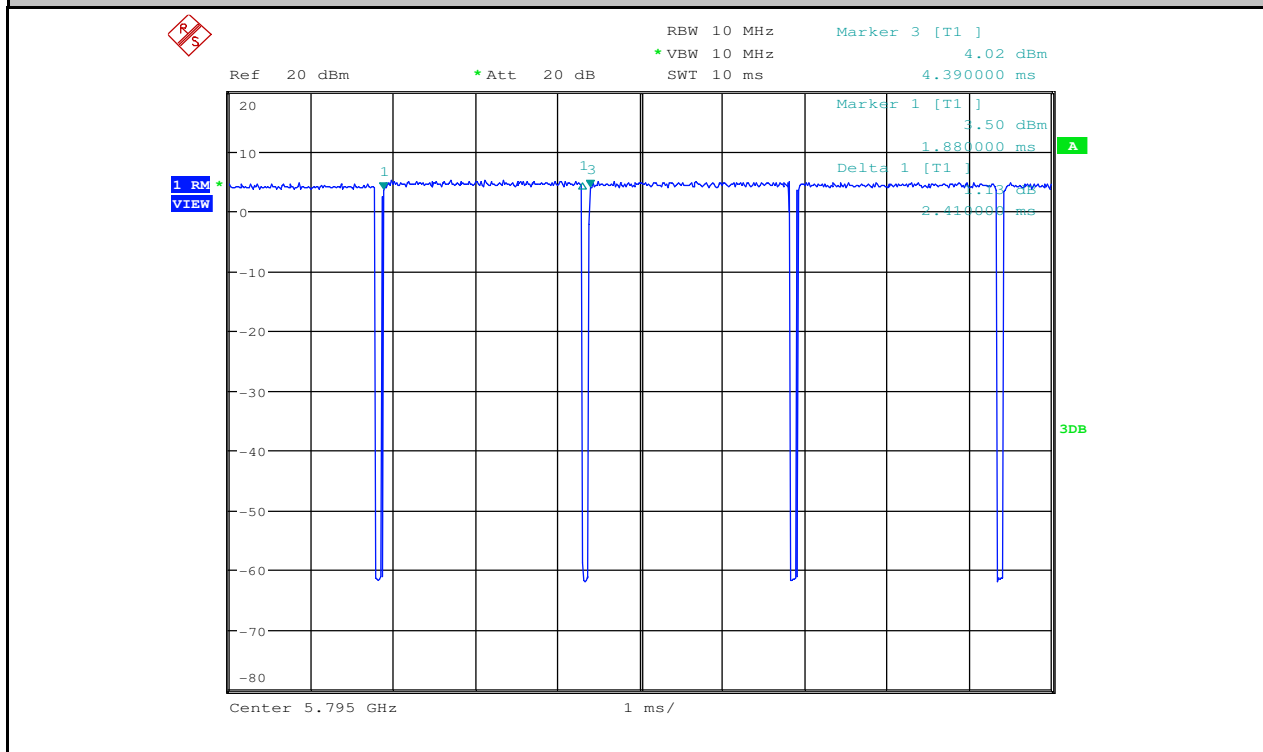
Duty Cycle_11AC40_5795_Ant2
