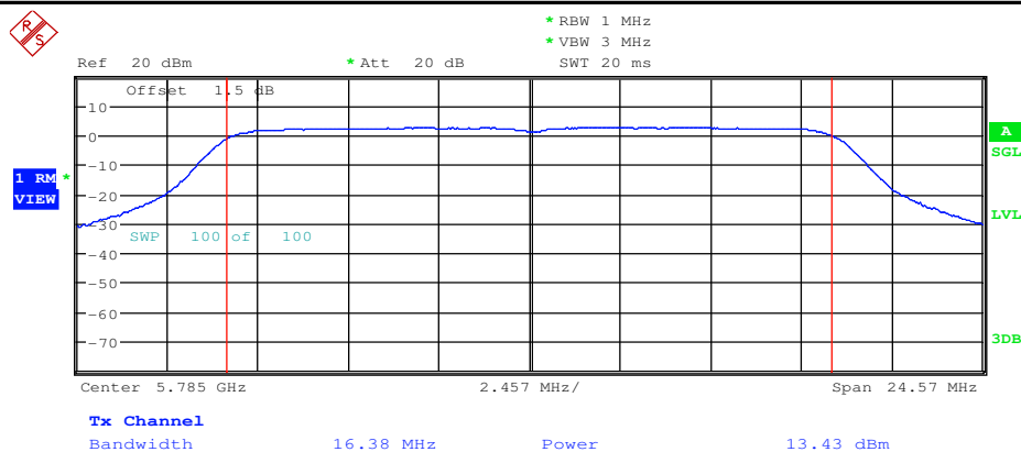
Maximum Conduct Output Power_11A_5785_Ant2
