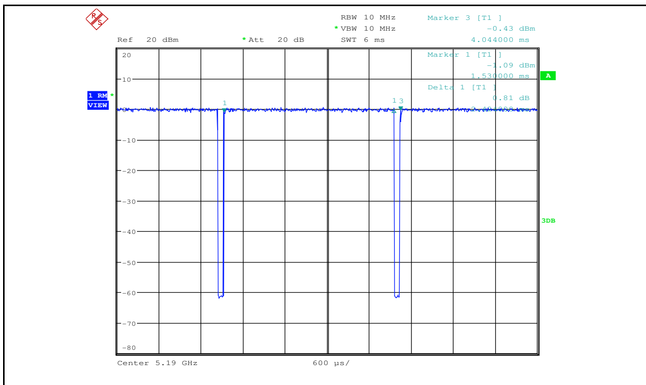
Duty Cycle_11N40_5190_Ant2
