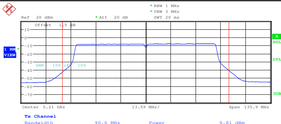
Maximum Conduct Output Power_11AC80_5210_Ant2
