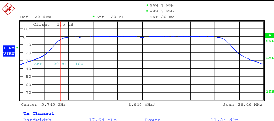
Maximum Conduct Output Power_11N20_5745_Ant2
