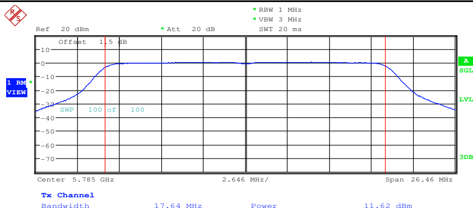
Maximum Conduct Output Power_11N20_5785_Ant2
