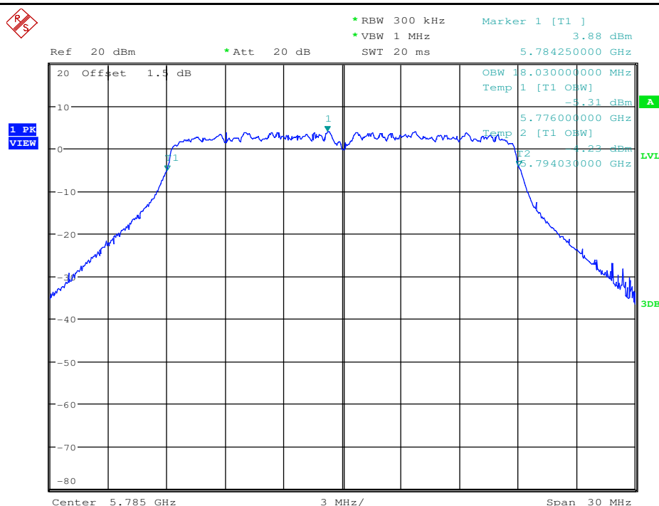
Occupied Bandwidth Measurement_11AC20_5785_Ant2
