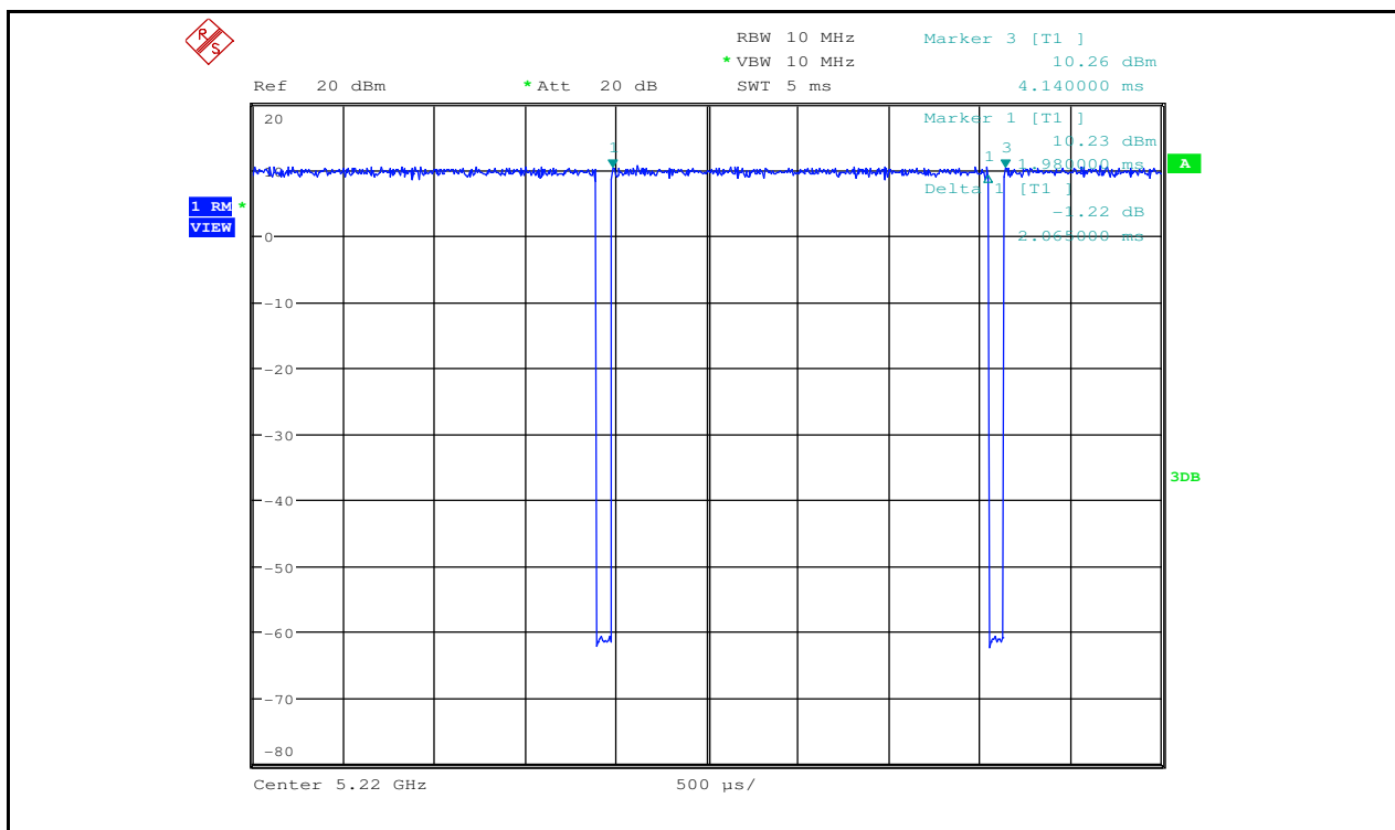
Duty Cycle_11A_5220_Ant2
