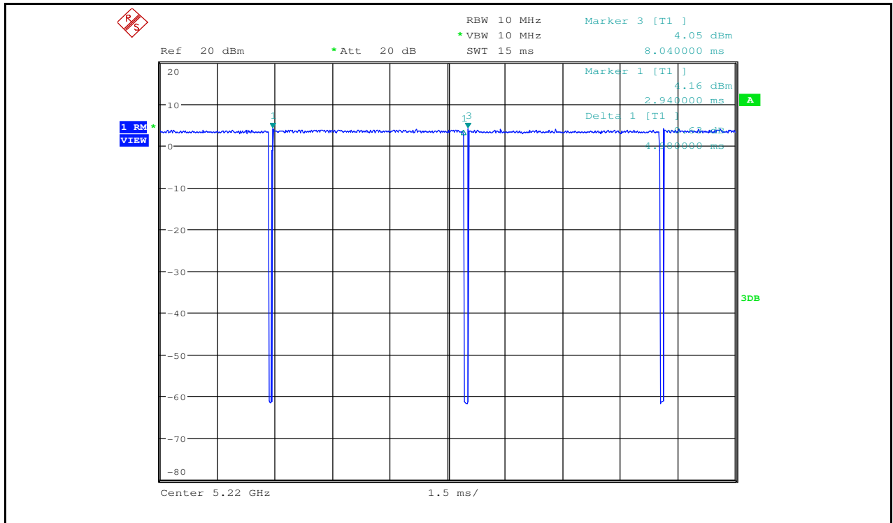
Duty Cycle_11AC20_5220_Ant2
