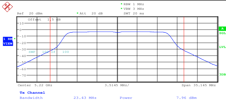
Maximum Conduct Output Power_11AC20_5220_Ant2
