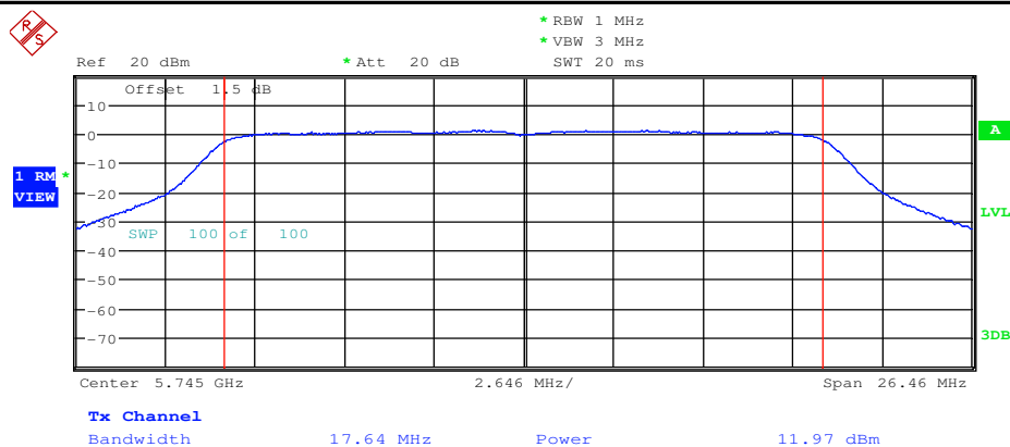
Maximum Conduct Output Power_11AC20_5745_Ant2
