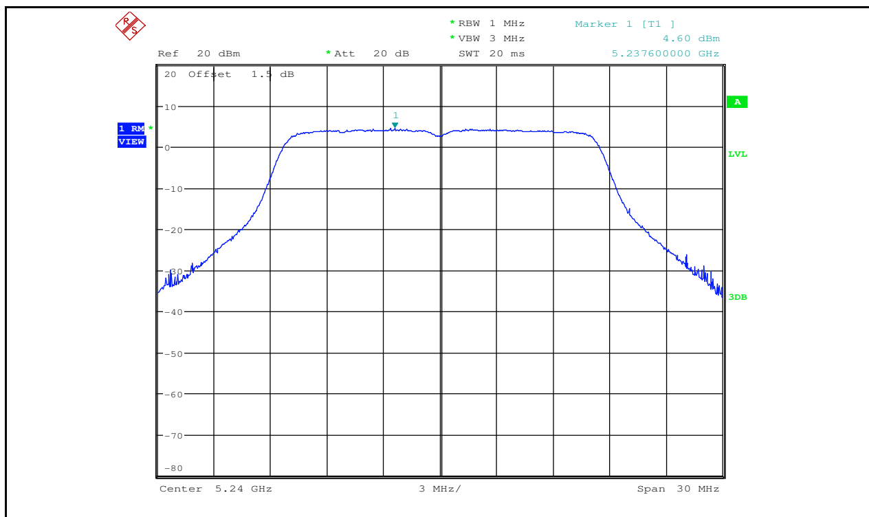
Maximum Power Spectral Density_TNVN_11A_5240_Ant2
