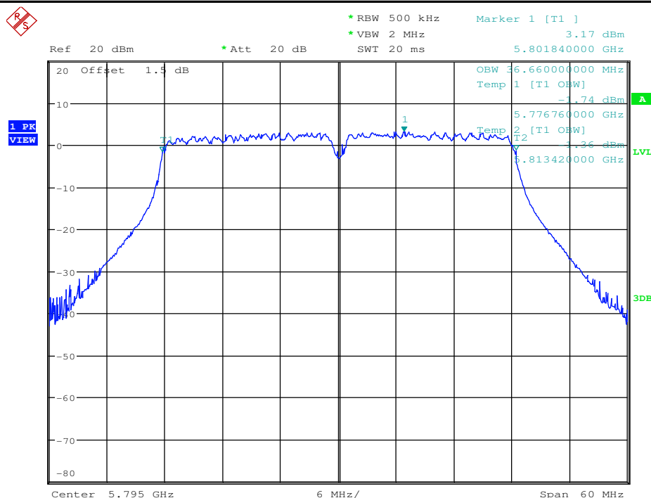
Occupied Bandwidth Measurement_11AC40_5795_Ant2
