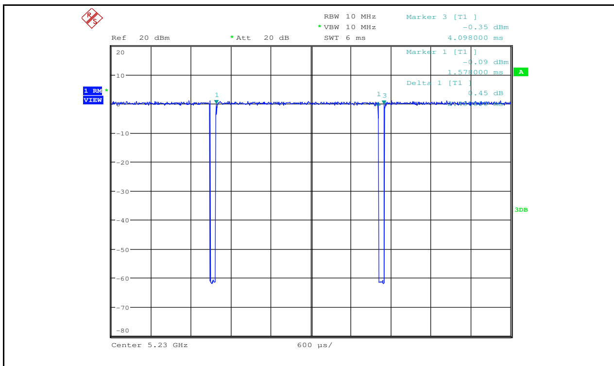
Duty Cycle_11N40_5230_Ant2
