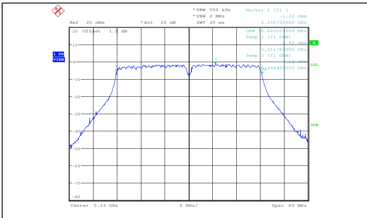
Occupied Bandwidth Measurement_11N40_5230_Ant2
