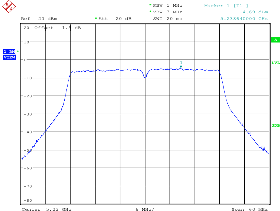
Maximum Power Spectral Density_TNVN_11N40_5230_Ant2
