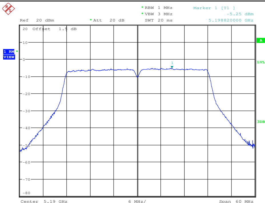
Maximum Power Spectral Density_TNVN_11N40_5190_Ant2
