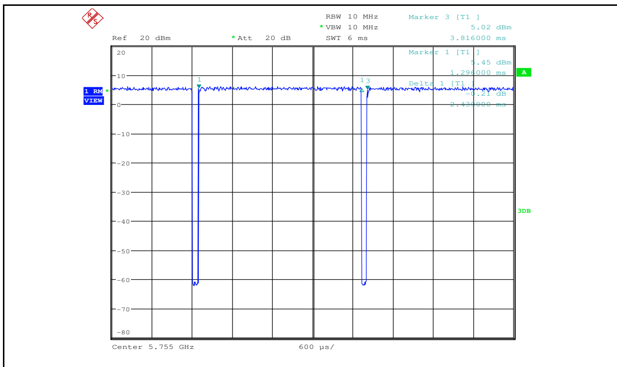
Duty Cycle_11N40_5755_Ant2
