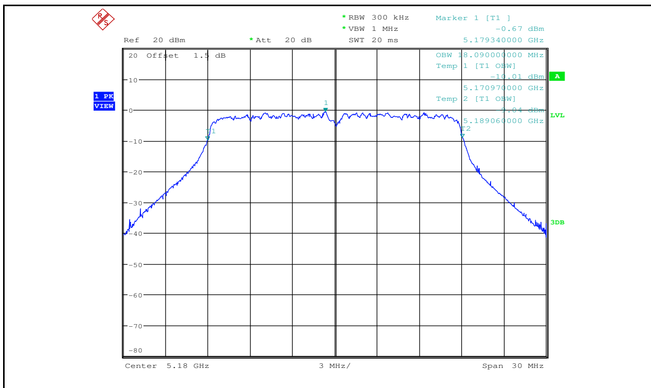
Occupied Bandwidth Measurement_11AC20_5180_Ant2
