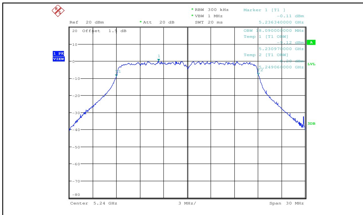
Occupied Bandwidth Measurement_11AC20_5240_Ant2
