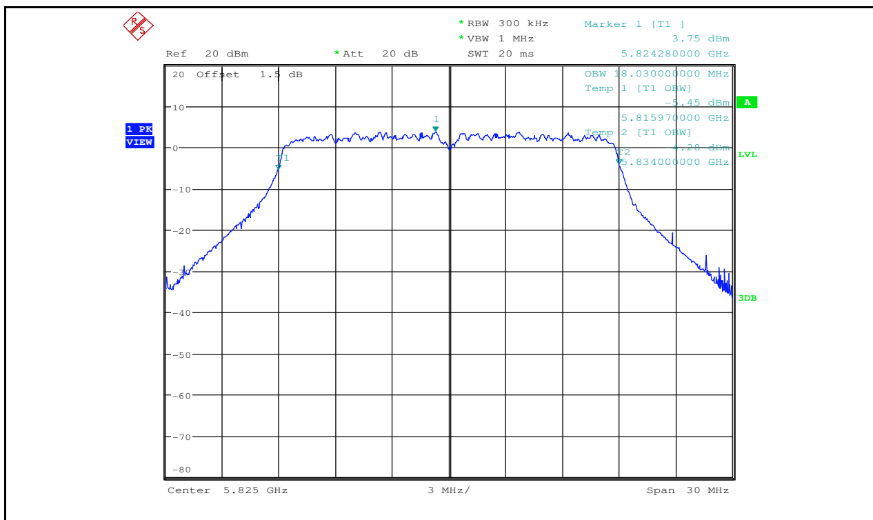
Occupied Bandwidth Measurement_11N20_5825_Ant2
