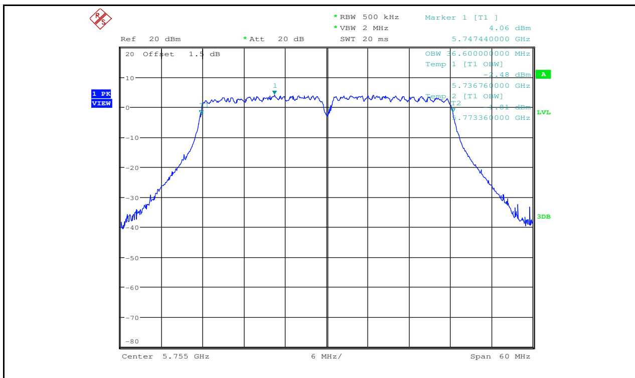
Occupied Bandwidth Measurement_11N40_5755_Ant2
