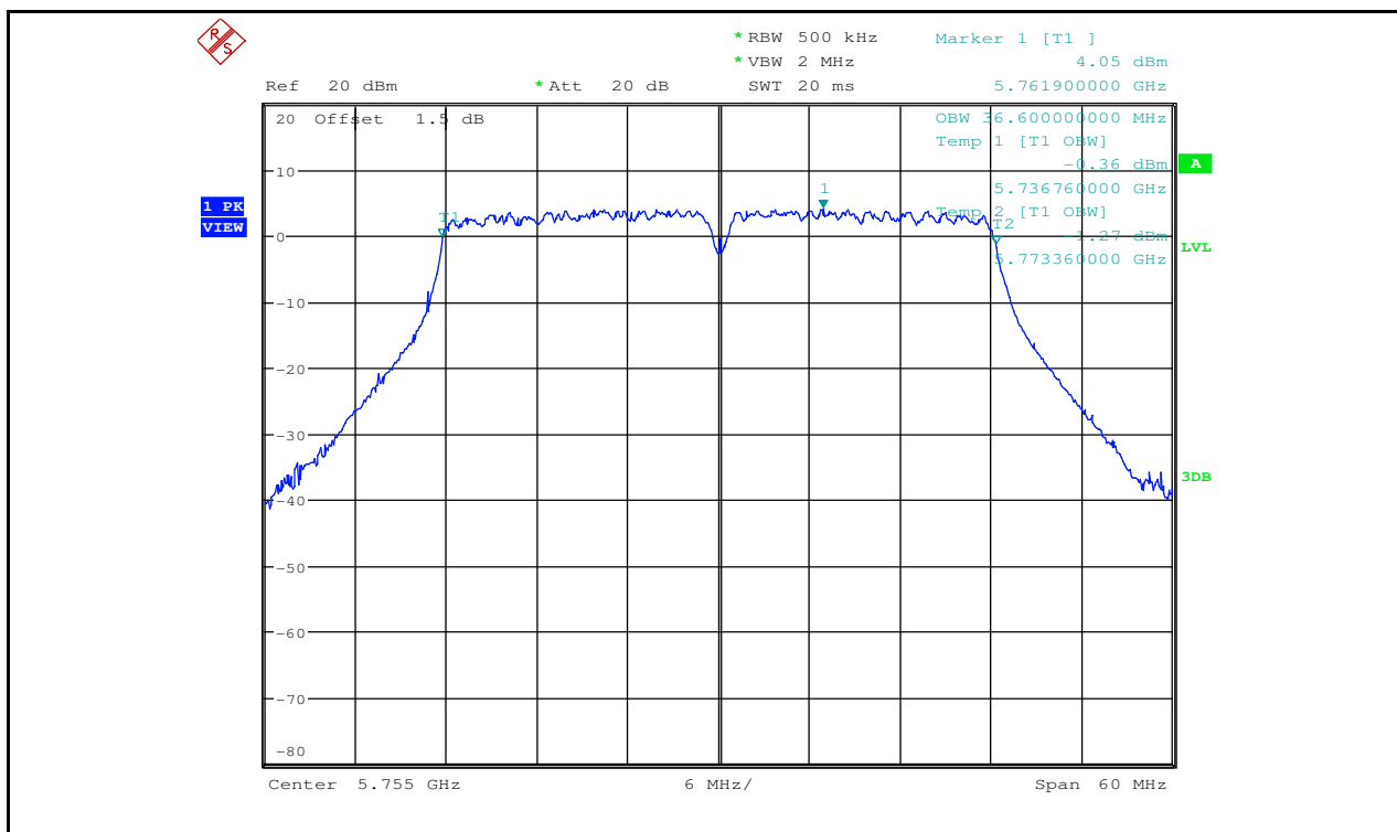
Occupied Bandwidth Measurement_11AC40_5755_Ant2
