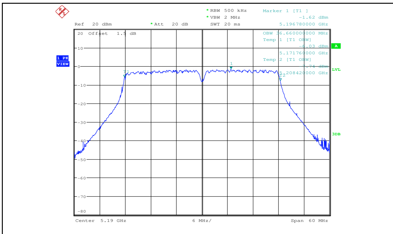
Occupied Bandwidth Measurement_11AC40_5190_Ant2
