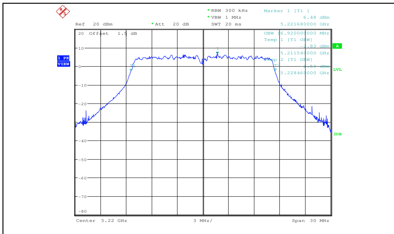
Occupied Bandwidth Measurement_11A_5220_Ant2
