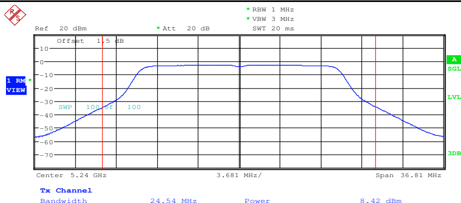
Maximum Conduct Output Power_11N20_5240_Ant2
