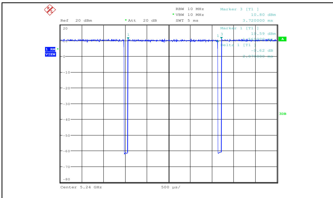
Duty Cycle_11A_5240_Ant2
