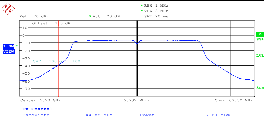
Maximum Conduct Output Power_11AC40_5230_Ant2
