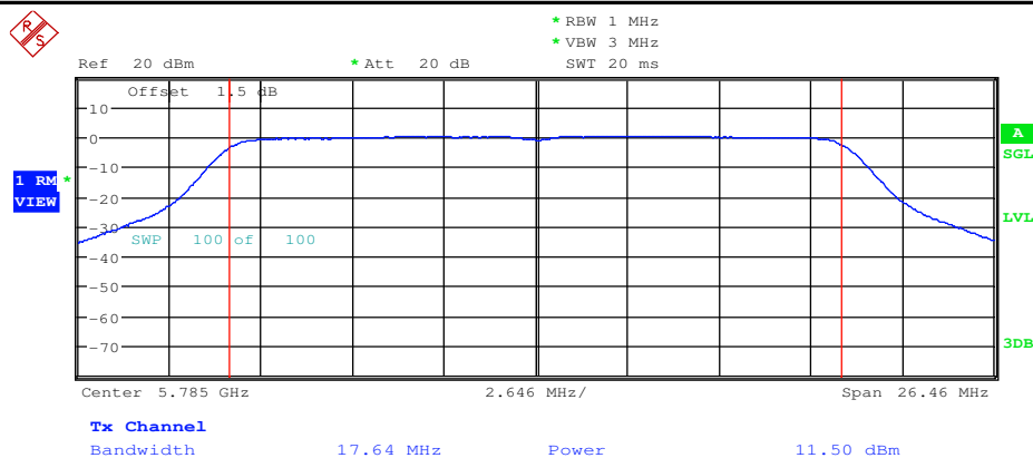
Maximum Conduct Output Power_11AC20_5785_Ant2
