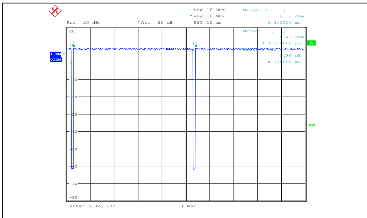
Duty Cycle_11N20_5825_Ant2
