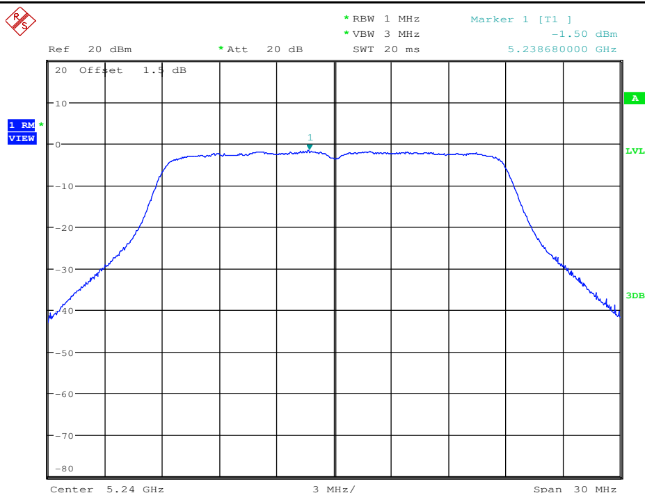
Maximum Power Spectral Density_TNVN_11AC20_5240_Ant2
