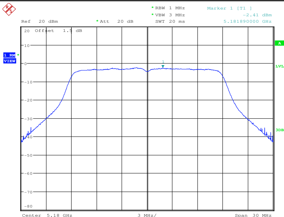
Maximum Power Spectral Density_TNVN_11AC20_5180_Ant2
