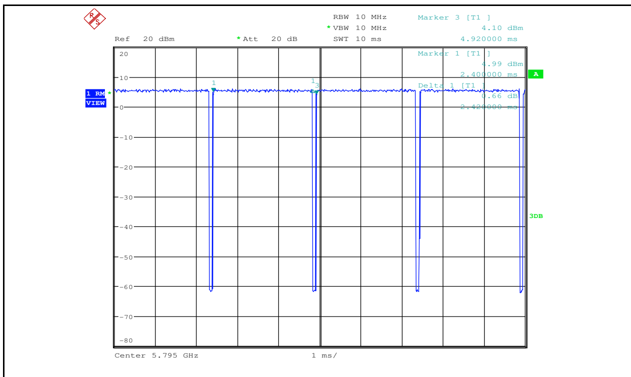
Duty Cycle_11AC40_5795_Ant2
