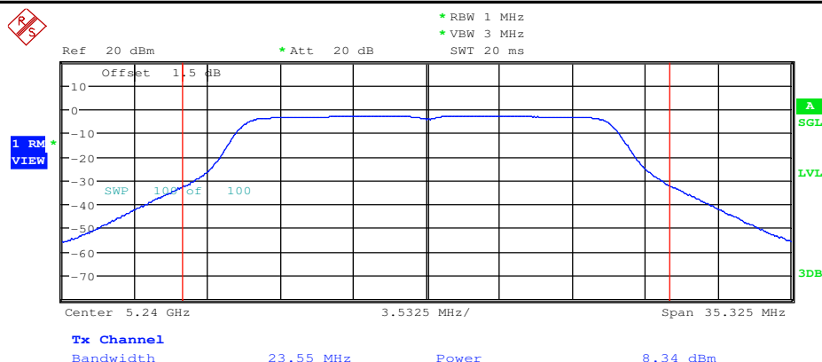
Maximum Conduct Output Power_11AC20_5240_Ant2
