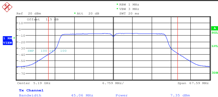
Maximum Conduct Output Power_11AC40_5190_Ant2
