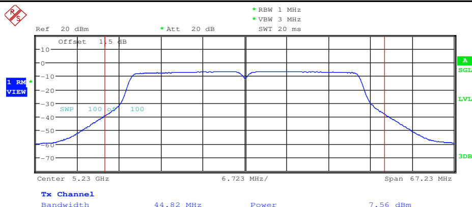
Maximum Conduct Output Power_11N40_5230_Ant2
