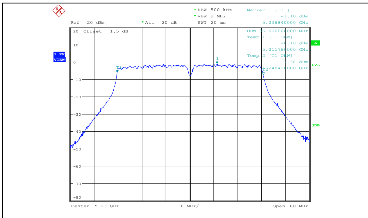
Occupied Bandwidth Measurement_11AC40_5230_Ant2
