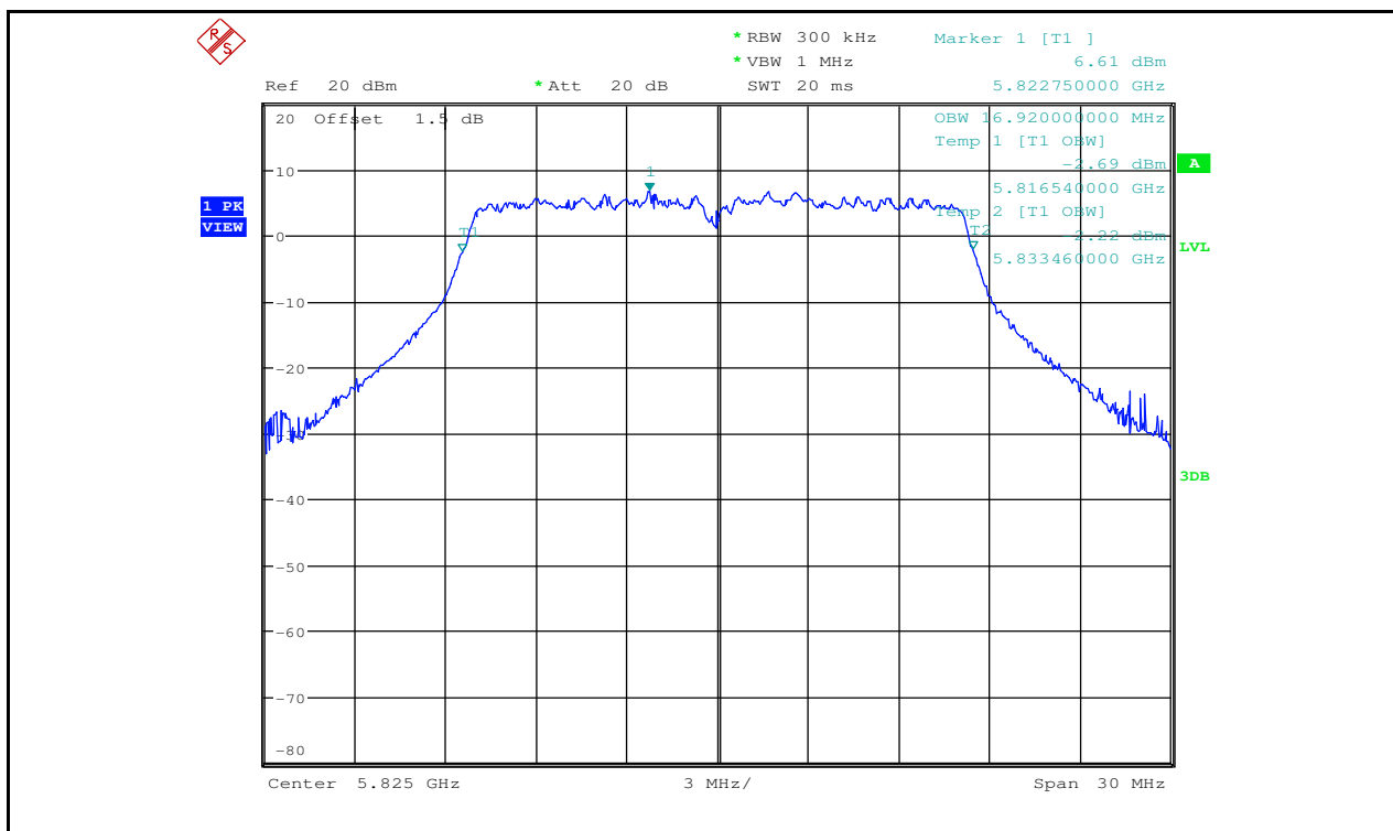
Occupied Bandwidth Measurement_11A_5825_Ant2
