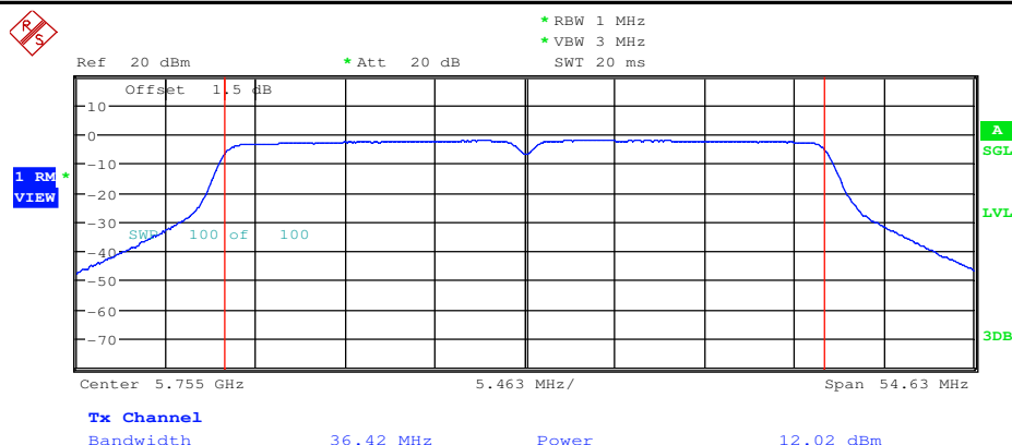
Maximum Conduct Output Power_11N40_5755_Ant2
