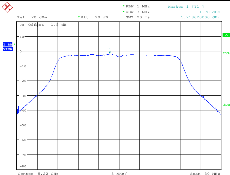
Maximum Power Spectral Density_TNVN_11AC20_5220_Ant2
