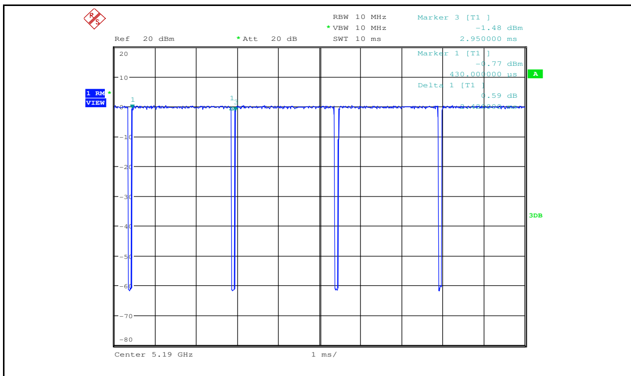
Duty Cycle_11AC40_5190_Ant2
