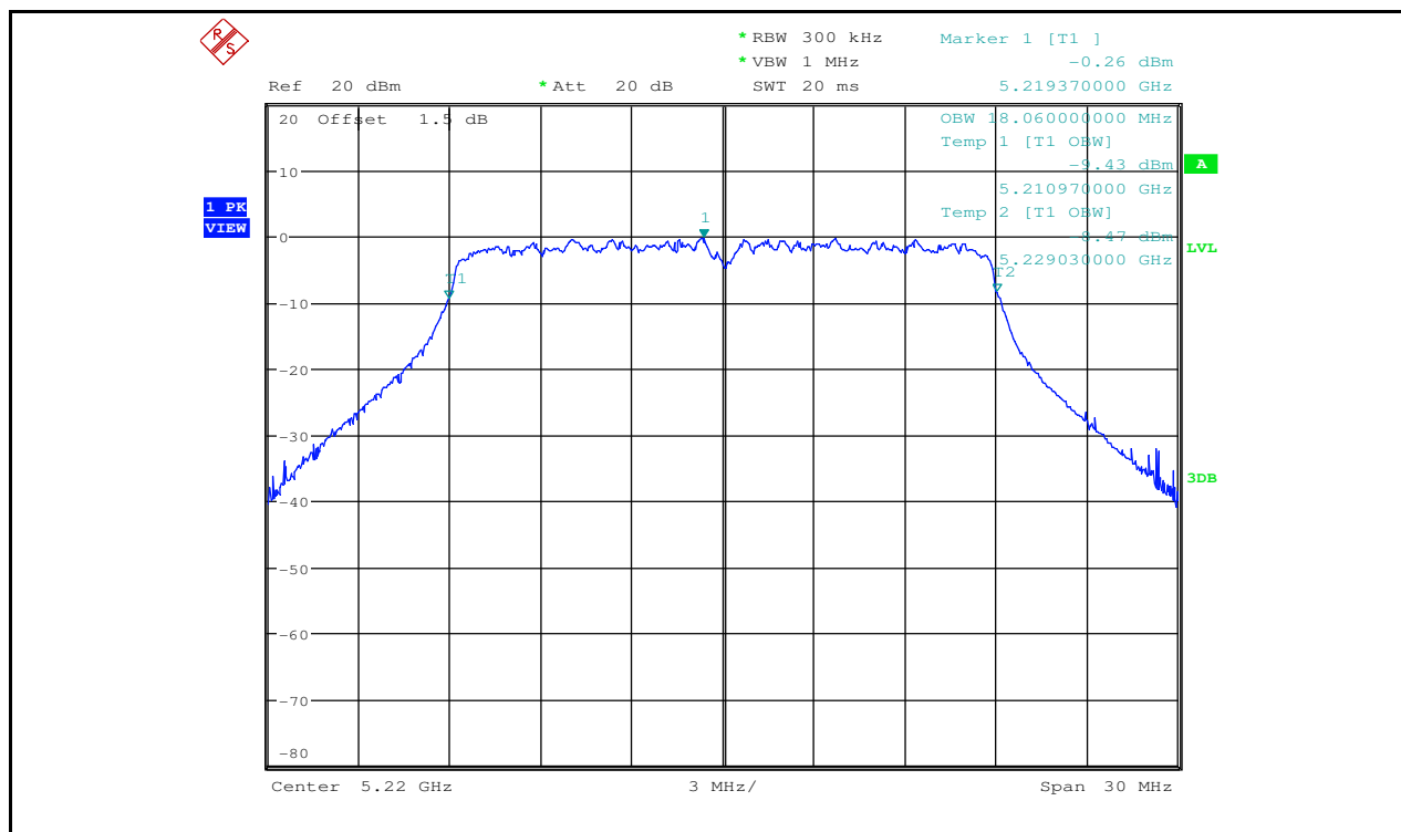
Occupied Bandwidth Measurement_11AC20_5220_Ant2
