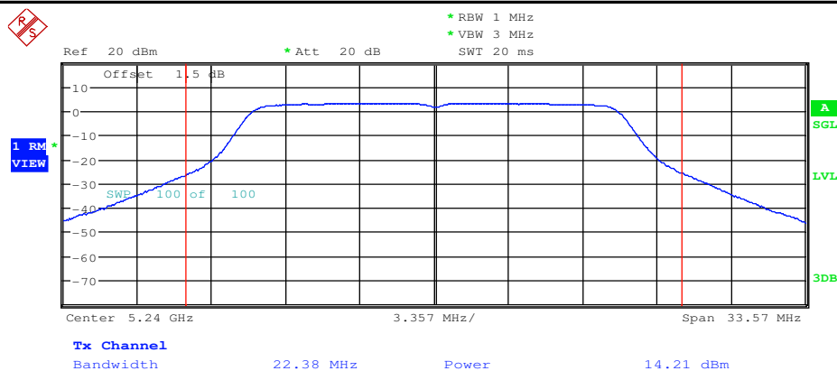
Maximum Conduct Output Power_11A_5240_Ant2
