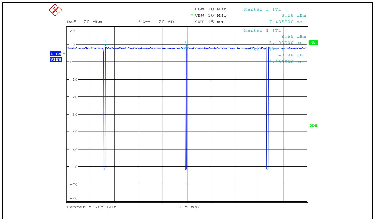
Duty Cycle_11AC20_5785_Ant2
