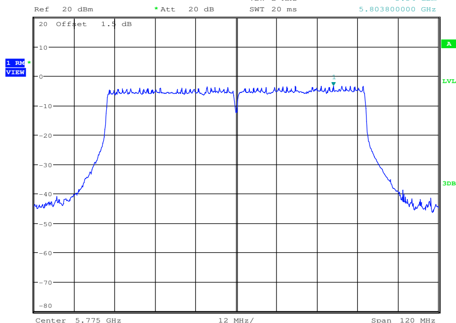
Maximum Power Spectral Density_TNVN_11AC80_5775_Ant2
