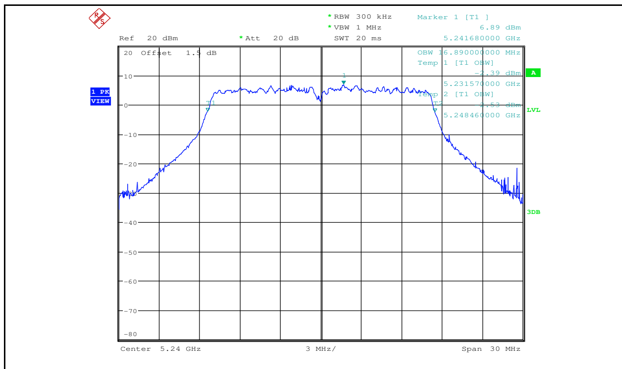
Occupied Bandwidth Measurement_11A_5240_Ant2
