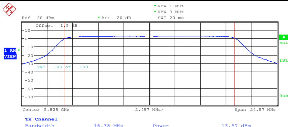
Maximum Conduct Output Power_11A_5825_Ant2
