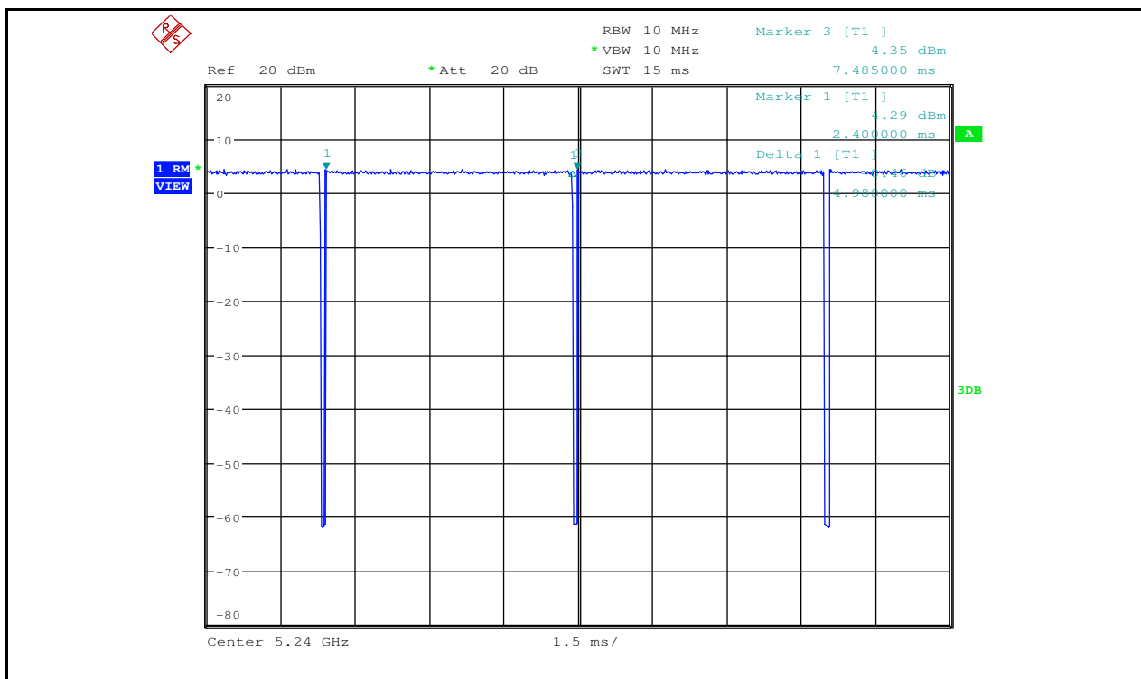
Duty Cycle_11AC20_5240_Ant2
