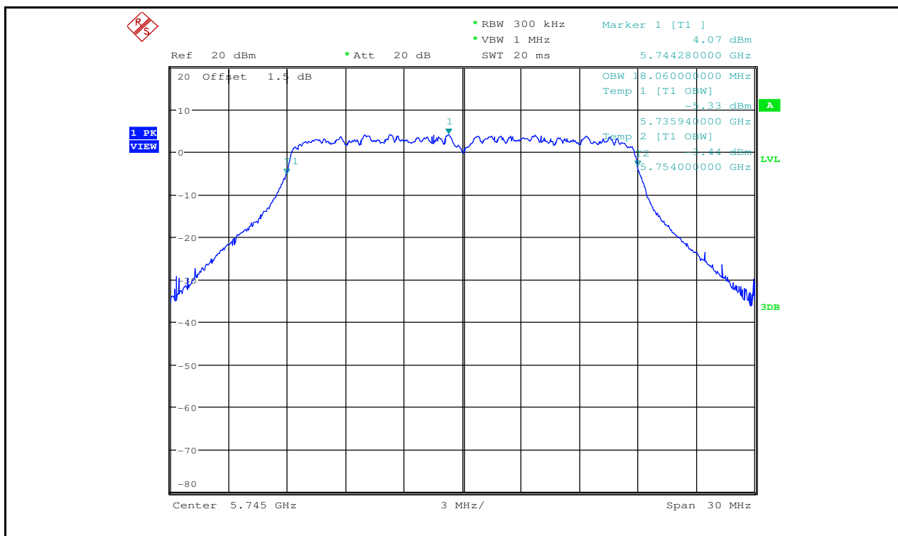
Occupied Bandwidth Measurement_11N20_5745_Ant2
