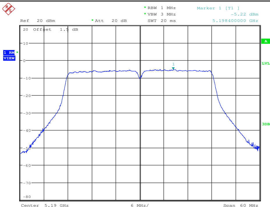
Maximum Power Spectral Density_TNVN_11AC40_5190_Ant2
