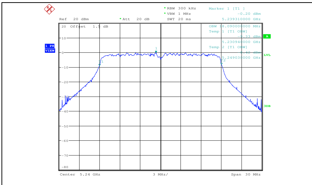
Occupied Bandwidth Measurement_11N20_5240_Ant2
