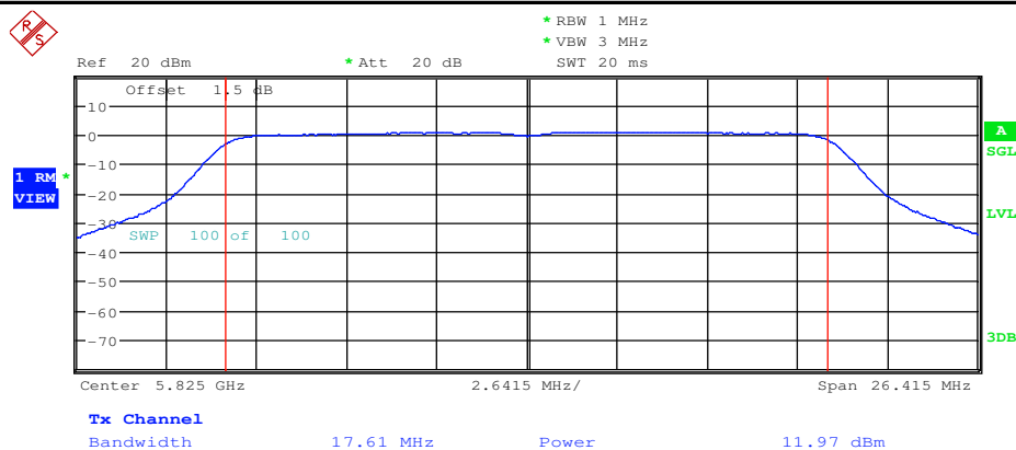
Maximum Conduct Output Power_11N20_5825_Ant2
