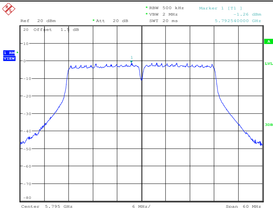
Maximum Power Spectral Density_TNVN_11N40_5795_Ant2
