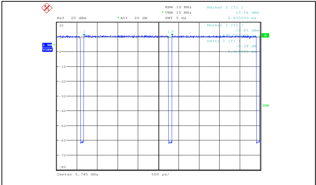
Duty Cycle_11A_5745_Ant2
