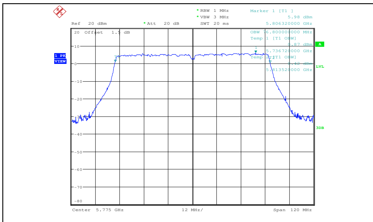
Occupied Bandwidth Measurement_11AC80_5775_Ant2
