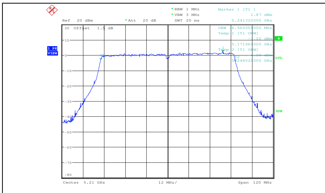
Occupied Bandwidth Measurement_11AC80_5210_Ant2
