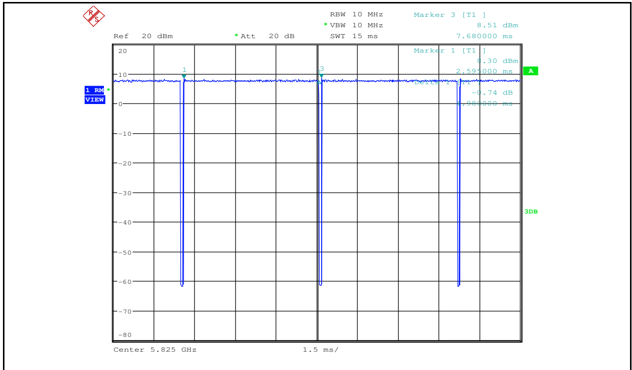
Duty Cycle_11AC20_5825_Ant2
