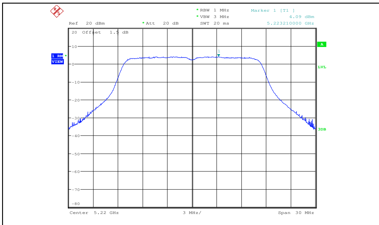
Maximum Power Spectral Density_TNVN_11A_5220_Ant2
