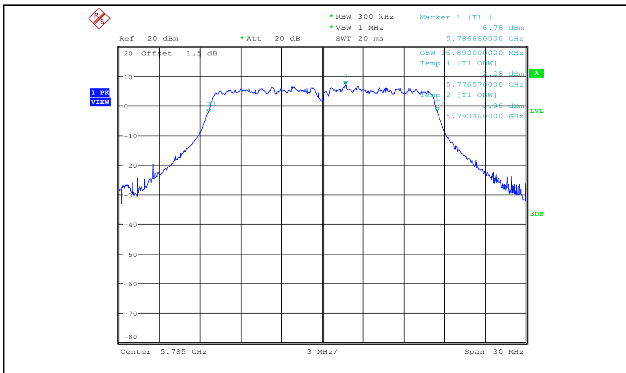
Occupied Bandwidth Measurement_11A_5785_Ant2
