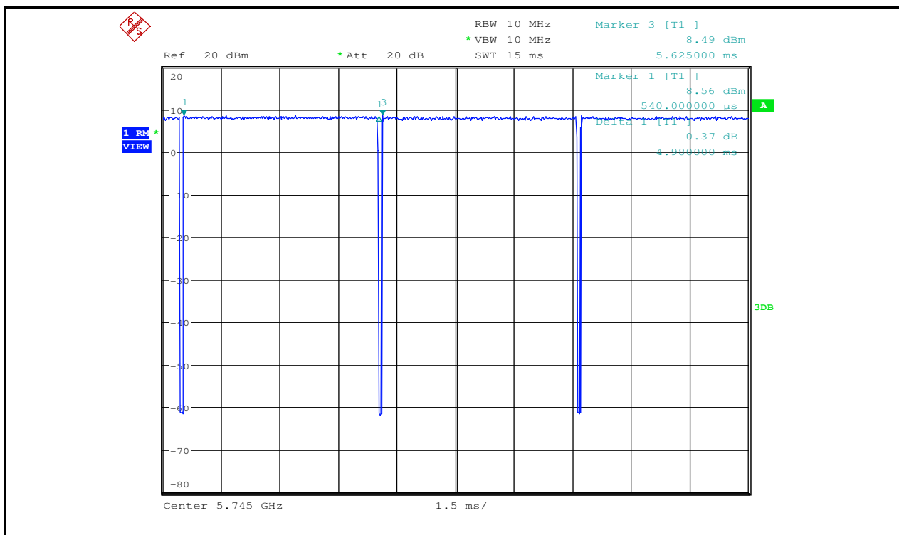
Duty Cycle_11AC20_5745_Ant2
