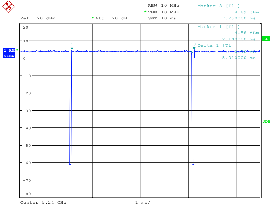
Duty Cycle_11N20_5240_Ant2
