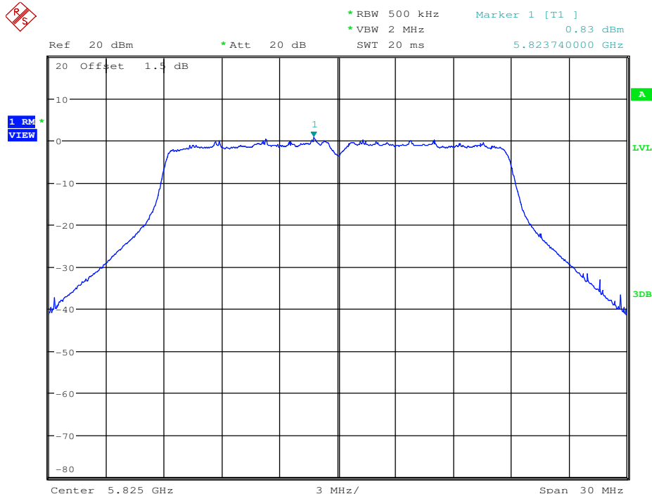
Maximum Power Spectral Density_TNVN_11AC20_5825_Ant2
