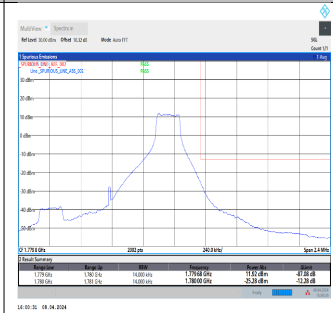
Band66_1.4MHz_64QAM_132665_1RB#5
