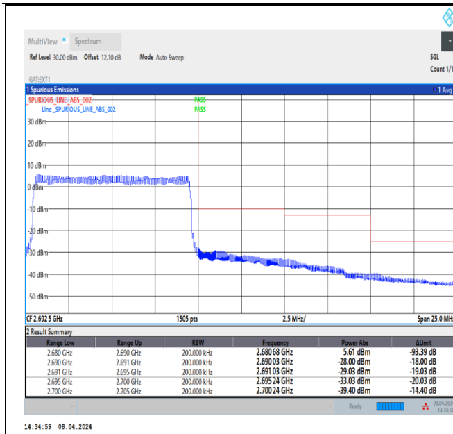
Band41_10MHz_16QAM_41540_50RB#0
