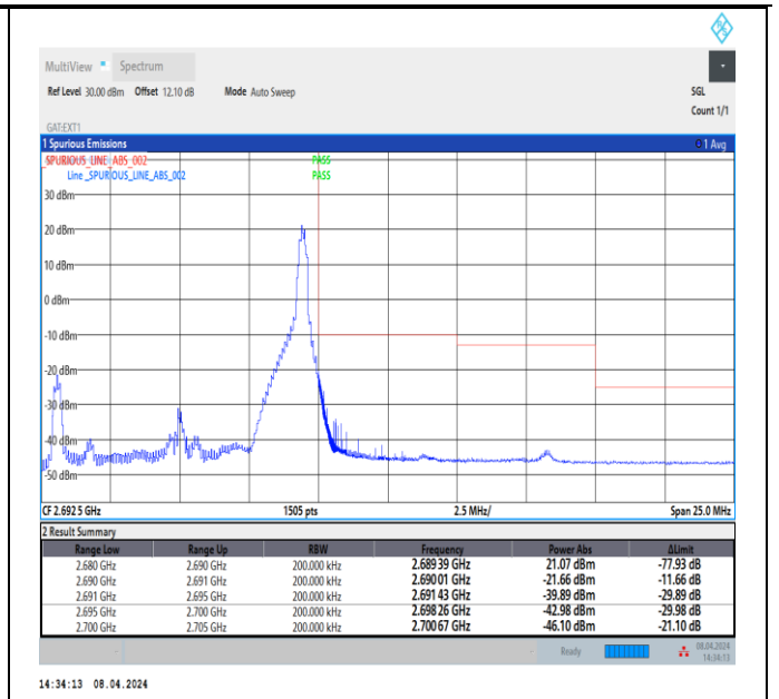
Band41_10MHz_64QAM_41540_1RB#49
