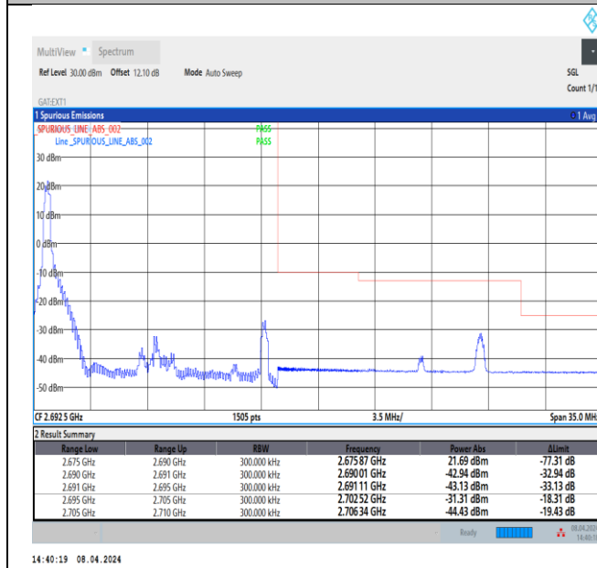
Band41_15MHz_64QAM_41515_1RB#0
