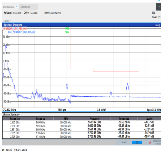
Band41_15MHz_QPSK_41515_1RB#0
