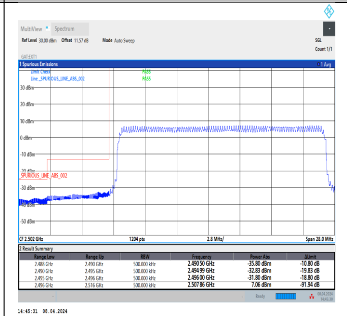
Band41_20MHz_QPSK_39750_100RB#0
