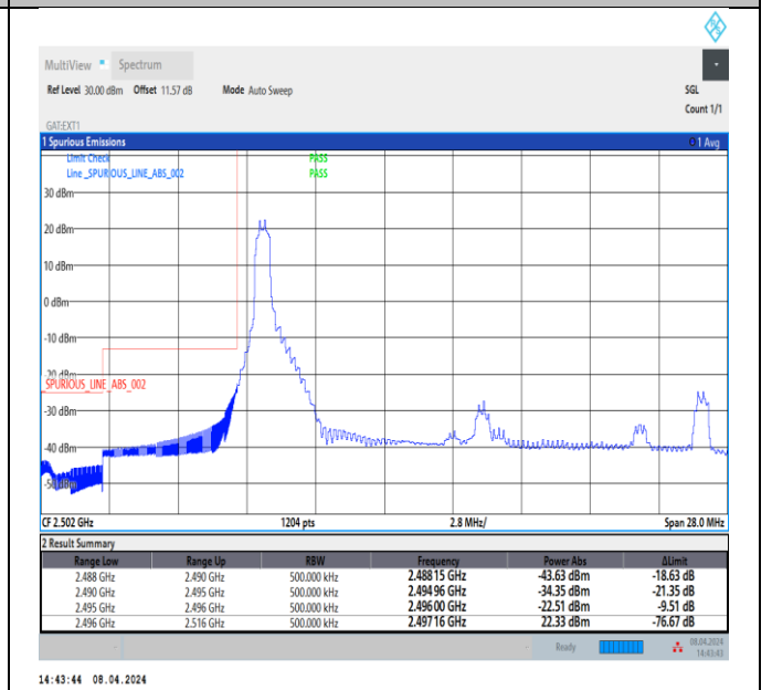
Band41_20MHz_16QAM_39750_1RB#0
