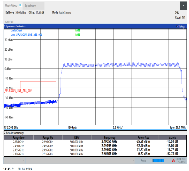
Band41_20MHz_16QAM_39750_100RB#0
