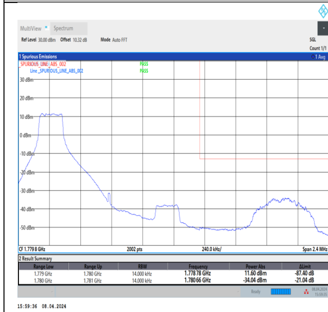
Band66_1.4MHz_64QAM_132665_1RB#0
