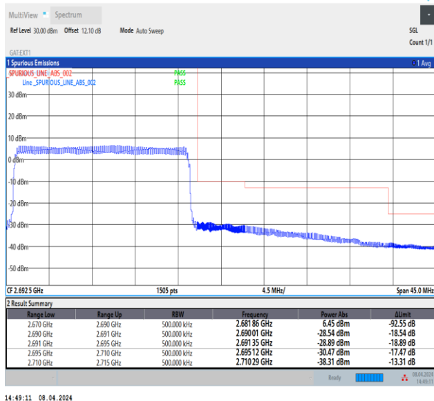
Band41_20MHz_16QAM_41490_100RB#0
