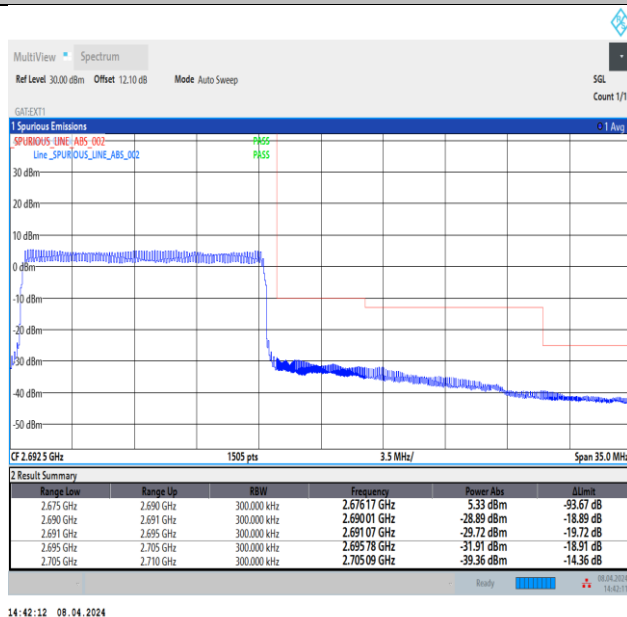
Band41_15MHz_16QAM_41515_75RB#0
