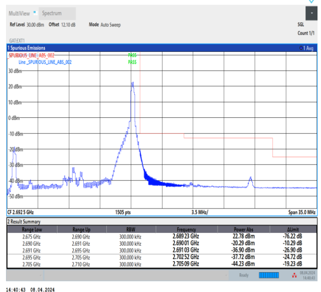
Band41_15MHz_QPSK_41515_1RB#74
