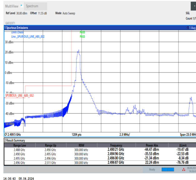
Band41_15MHz_16QAM_39725_1RB#0
