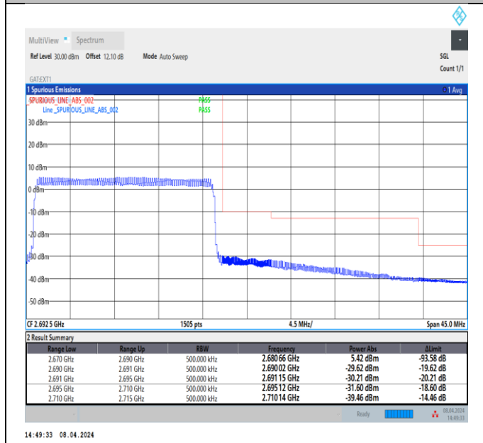
Band41_20MHz_64QAM_41490_100RB#0
