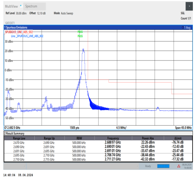
Band41_20MHz_16QAM_41490_1RB#99
