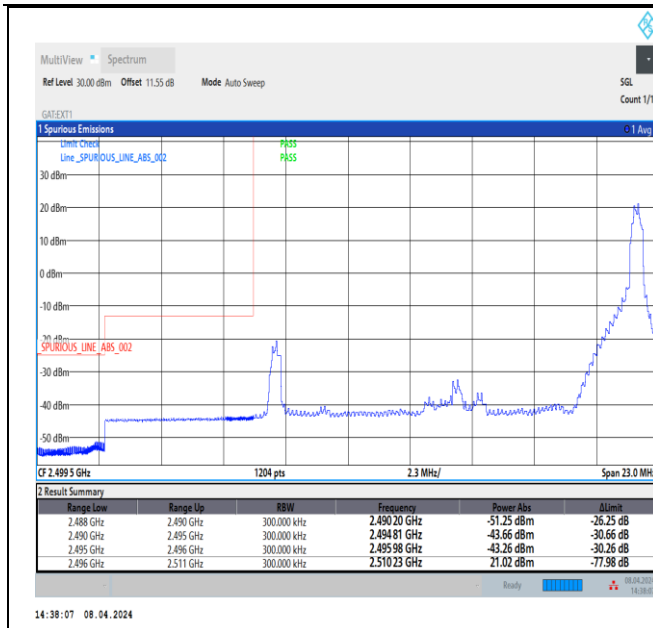
Band41_15MHz_64QAM_39725_1RB#74
