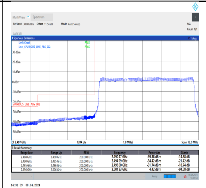
Band41_10MHz_64QAM_39700_50RB#0
