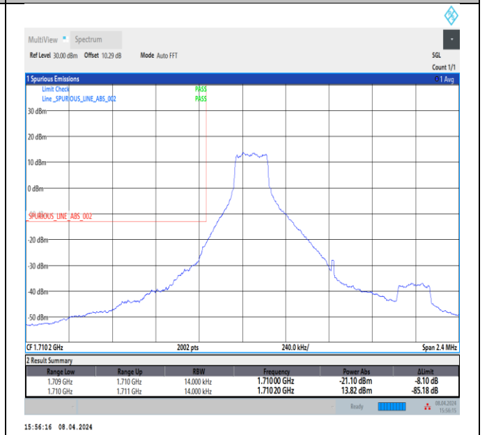
Band66_1.4MHz_QPSK_131979_1RB#0
