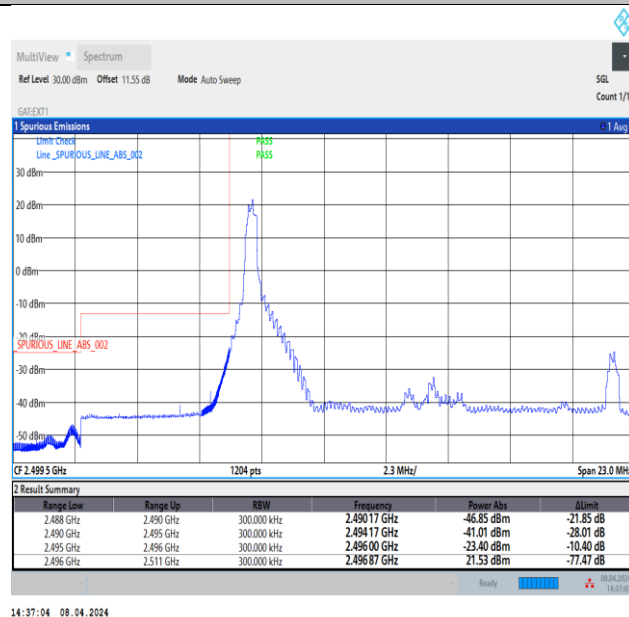
Band41_15MHz_64QAM_39725_1RB#0
