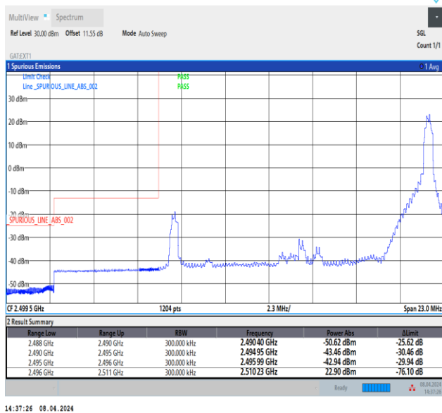
Band41_15MHz_QPSK_39725_1RB#74
