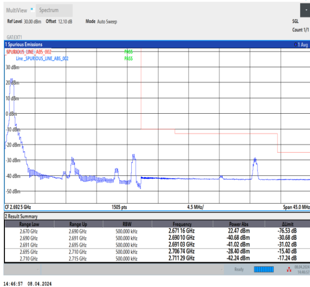
Band41_20MHz_16QAM_41490_1RB#0
