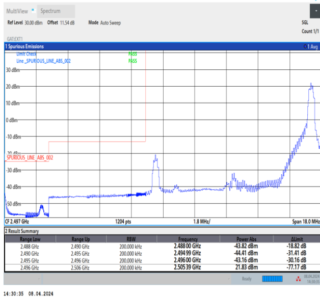
Band41_10MHz_16QAM_39700_1RB#49
