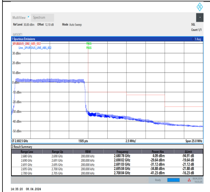
Band41_10MHz_64QAM_41540_50RB#0
