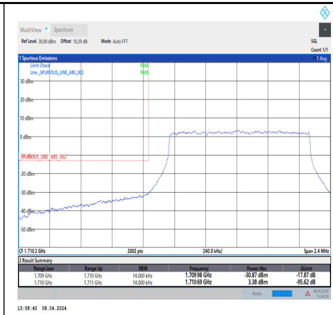
Band66_1.4MHz_64QAM_131979_6RB#0
