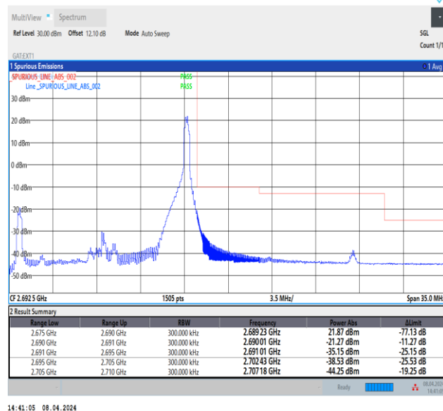
Band41_15MHz_16QAM_41515_1RB#74
