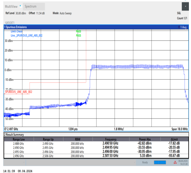
Band41_10MHz_16QAM_39700_50RB#0
