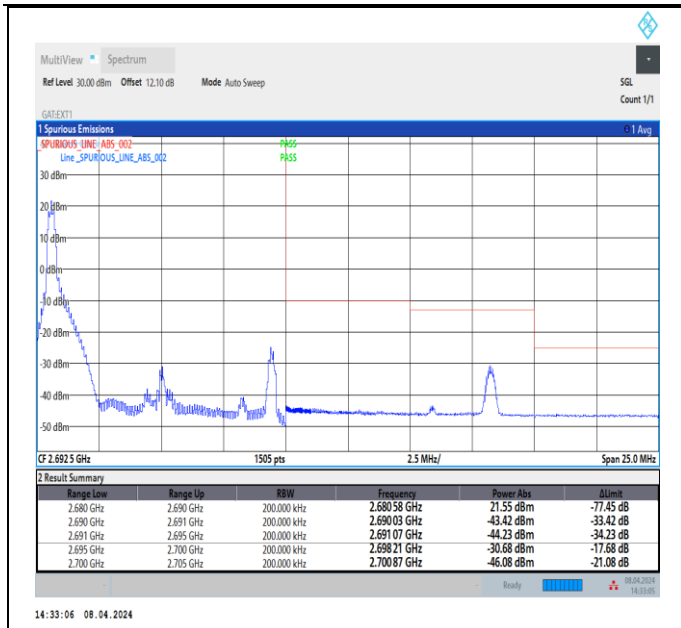
Band41_10MHz_64QAM_41540_1RB#0
