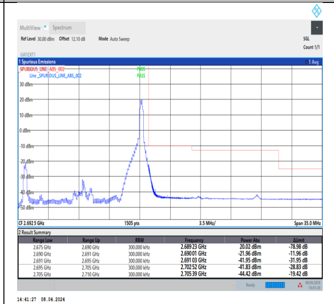
Band41_15MHz_64QAM_41515_1RB#74
