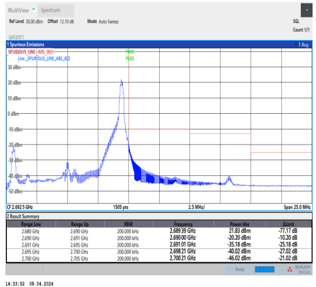
Band41_10MHz_16QAM_41540_1RB#49
