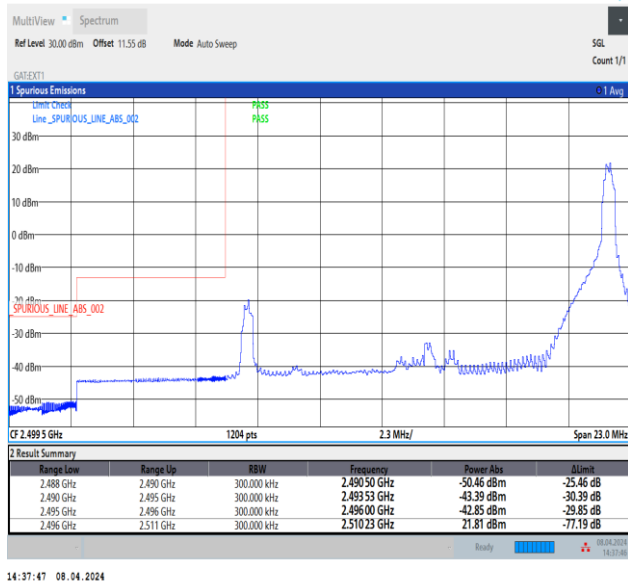
Band41_15MHz_16QAM_39725_1RB#74
