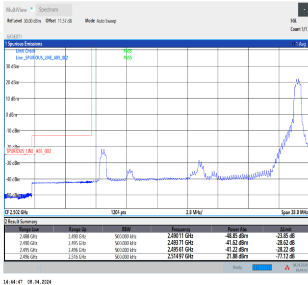
Band41_20MHz_16QAM_39750_1RB#99
