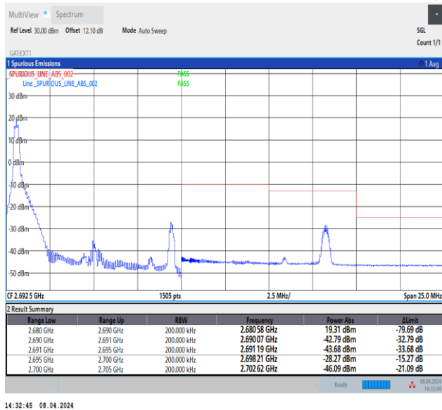
Band41_10MHz_16QAM_41540_1RB#0
