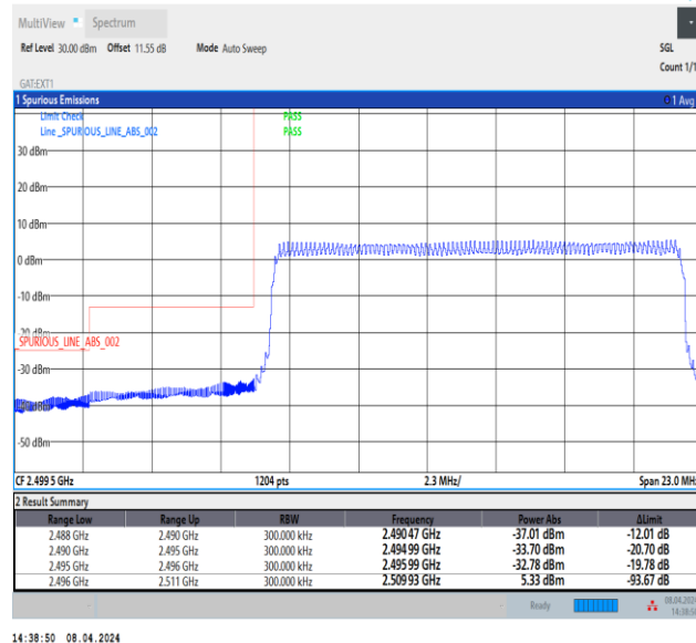
Band41_15MHz_16QAM_39725_75RB#0
