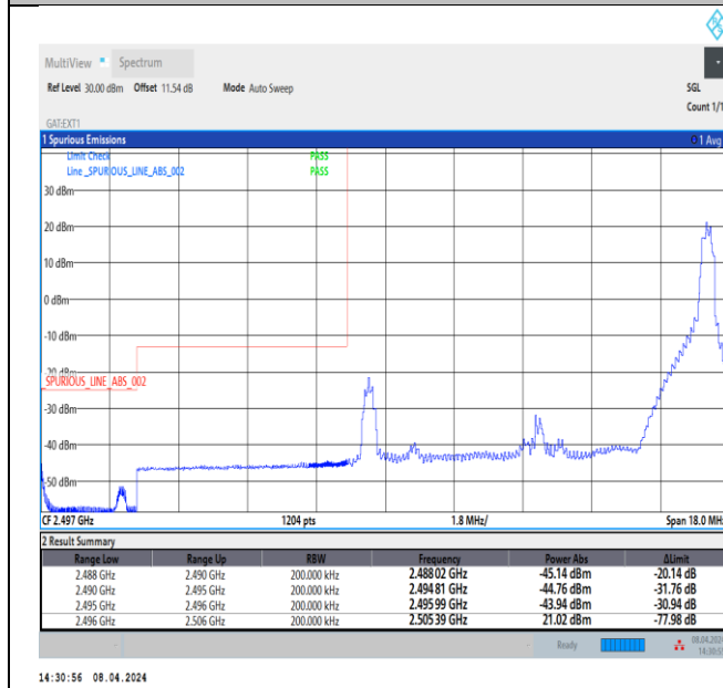
Band41_10MHz_64QAM_39700_1RB#49
