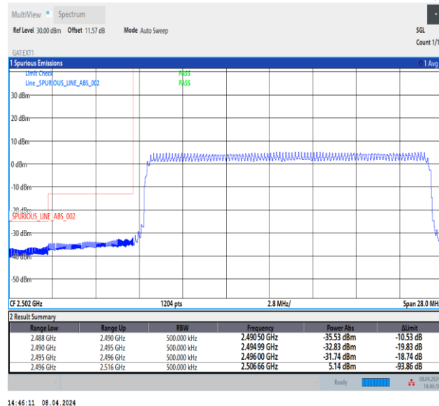
Band41_20MHz_64QAM_39750_100RB#0
