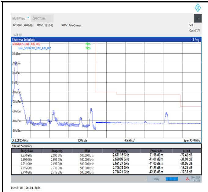
Band41_20MHz_64QAM_41490_1RB#0
