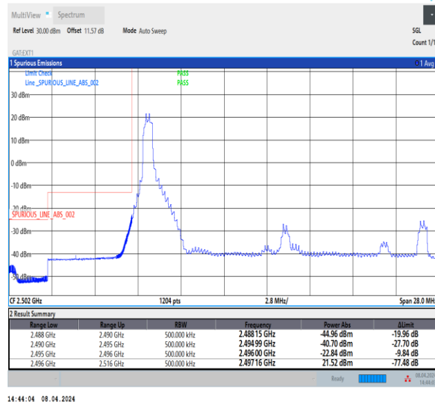
Band41_20MHz_64QAM_39750_1RB#0
