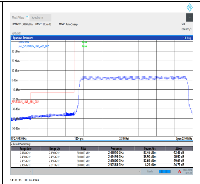
Band41_15MHz_64QAM_39725_75RB#0
