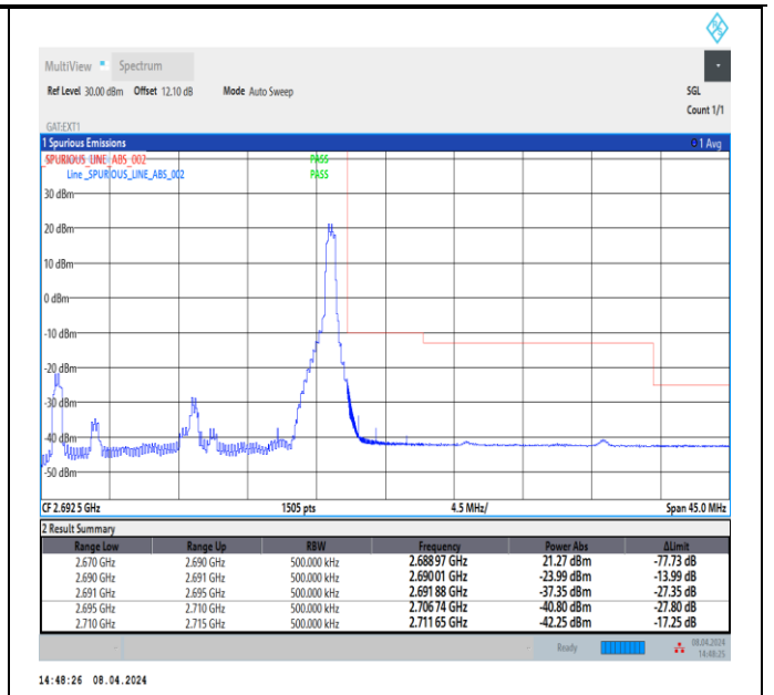
Band41_20MHz_64QAM_41490_1RB#99
