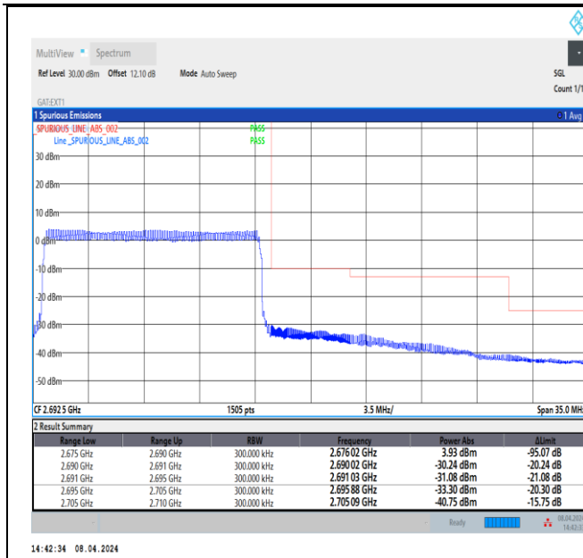
Band41_15MHz_64QAM_41515_75RB#0
