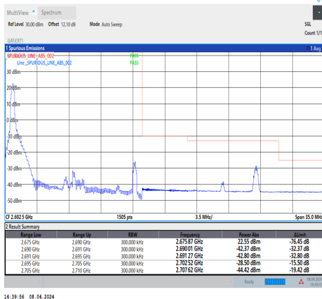
Band41_15MHz_16QAM_41515_1RB#0
