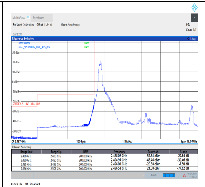
Band41_10MHz_64QAM_39700_1RB#0
