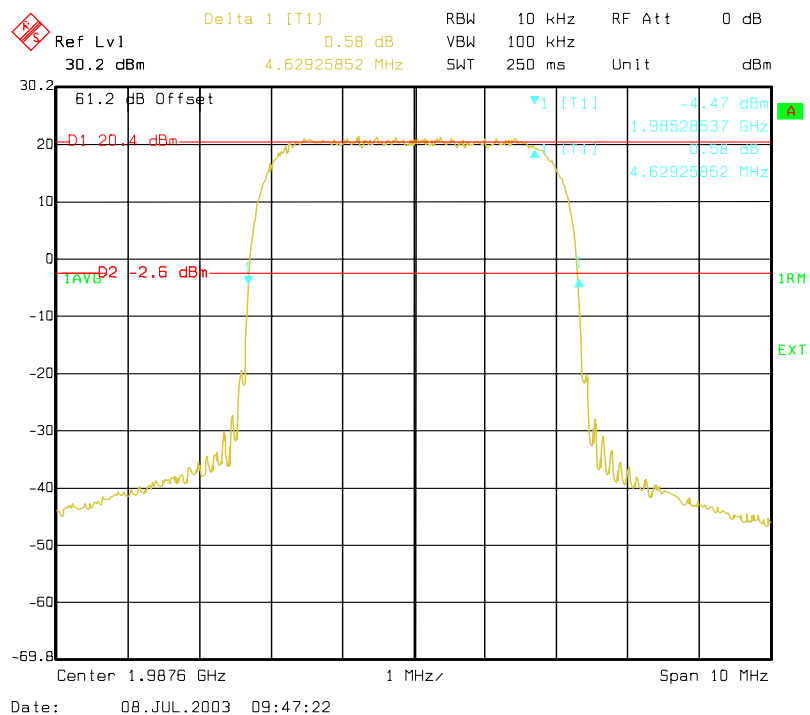
Figure 4. Sample plot for Occupied Bandwidth @ 1987.6 MHz
