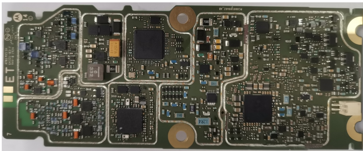
RF board without Shields (Top), Model MTP8550Ex / MTP8500Ex
