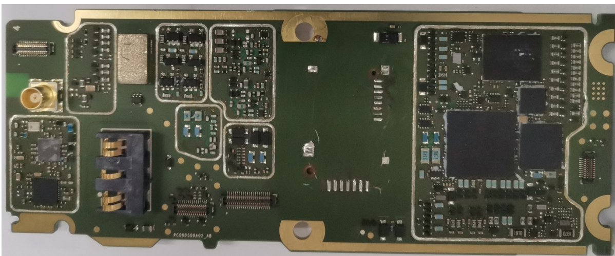
RF board without Shields (Bottom), Model MTP8550Ex / MTP8500Ex
