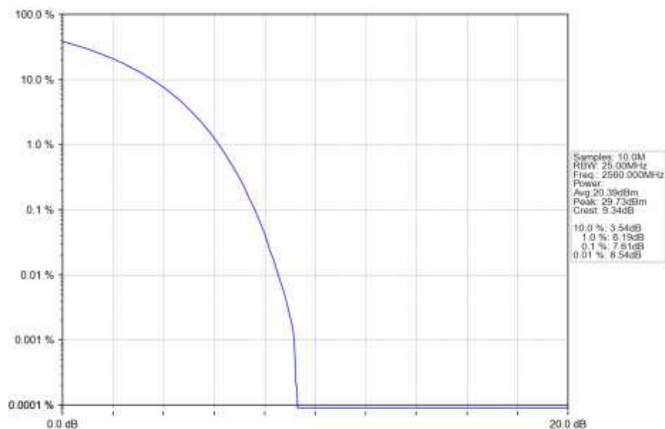
n7_15kHz_SISO_NTNV_20MHz_CP-OFDM_QPSK_2560MHz_Outer_Full_Ant1
