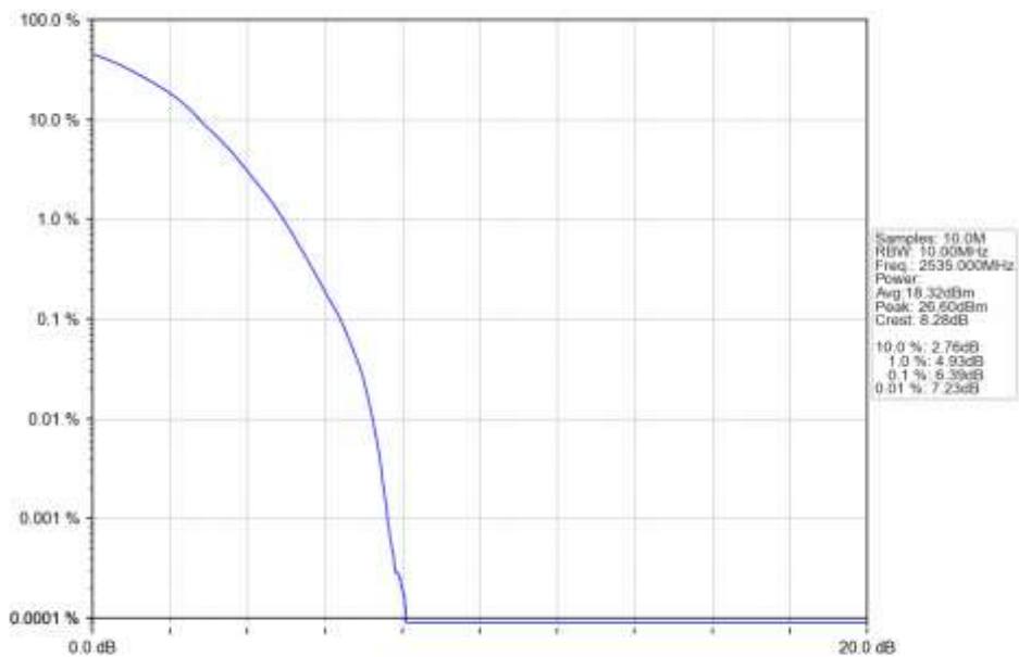
n7_15kHz_SISO_NTNV_10MHz_DFT-s-OFDM_64_QAM_2535MHz_Outer_Full_Ant1
