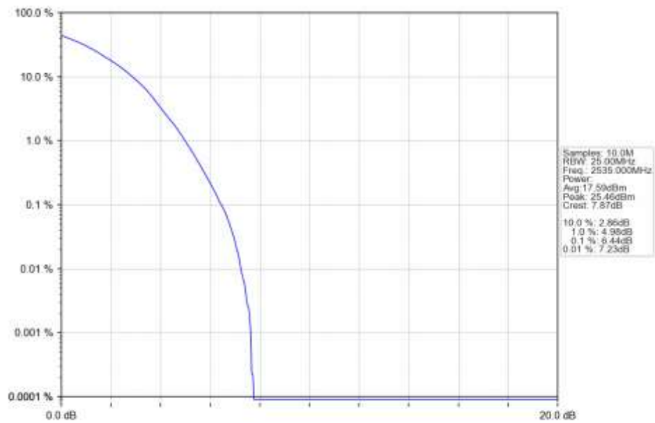
n7_15kHz_SISO_NTNV_20MHz_DFT-s-OFDM_64_QAM_2535MHz_Outer_Full_Ant1
