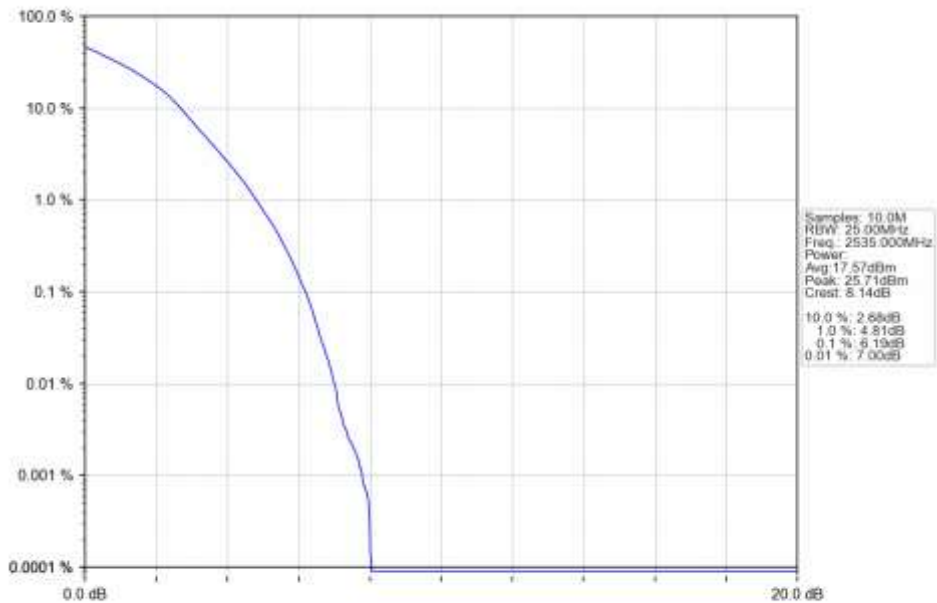
n7_15kHz_SISO_NTNV_15MHz_DFT-s-OFDM_16_QAM_2535MHz_Outer_Full_Ant1
