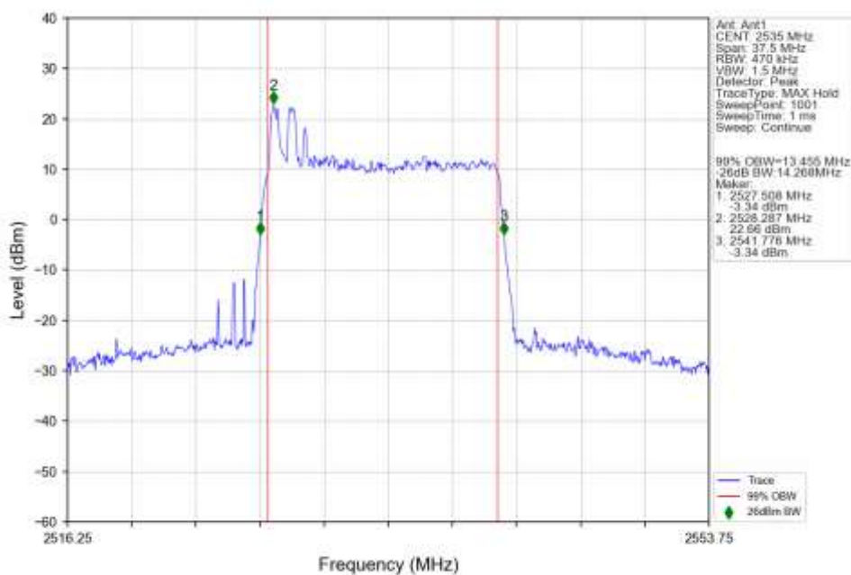
n7_15kHz_SISO_NTNV_15MHz_DFT-s-OFDM_64_QAM_2535MHz_Outer_Full_Ant1
