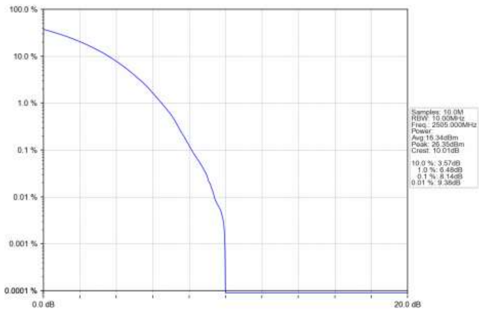
n7_15kHz_SISO_NTNV_10MHz_CP-OFDM_256_QAM_2505MHz_Outer_Full_Ant1
