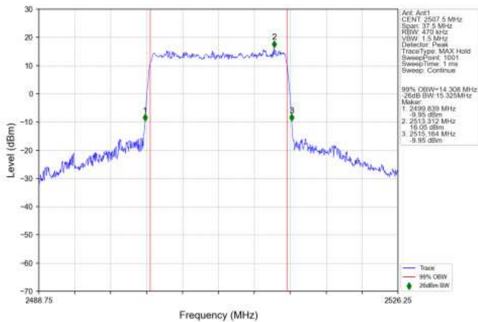
n7_15kHz_SISO_NTNV_15MHz_CP-OFDM_16_QAM_2507.5MHz_Outer_Full_Ant1
