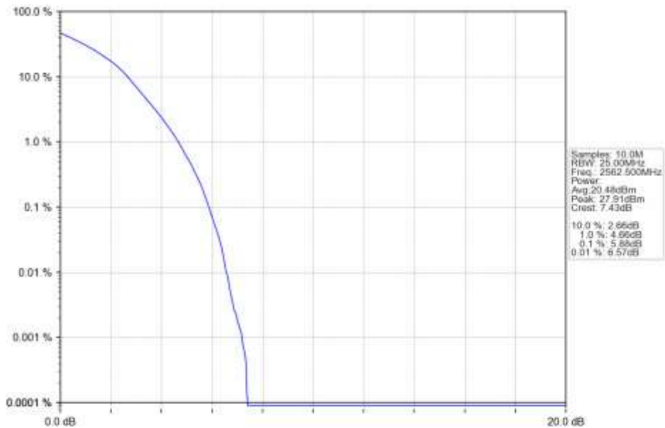
n7_15kHz_SISO_NTNV_15MHz_DFT-s-OFDM_16_QAM_2562.5MHz_Outer_Full_Ant1
