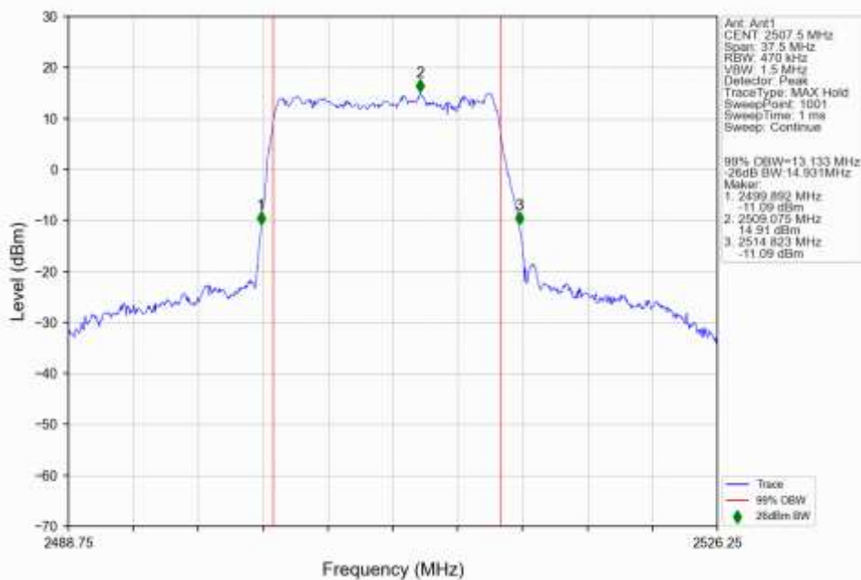
n7_30kHz_SISO_NTNV_15MHz_DFT-s-OFDM_16_QAM_2507.5MHz_Outer_Full_Ant1
