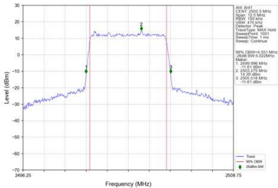
n7_15kHz_SISO_NTNV_5MHz_CP-OFDM_16_QAM_2502.5MHz_Outer_Full_Ant1
