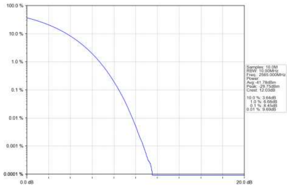
n7_15kHz_SISO_NTNV_10MHz_CP-OFDM_256_QAM_2565MHz_Outer_Full_Ant1
