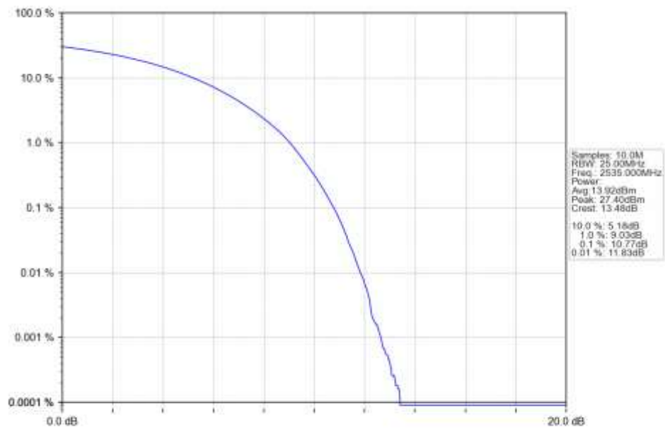
n7_15kHz_SISO_NTNV_15MHz_CP-OFDM_64_QAM_2535MHz_Outer_Full_Ant1
