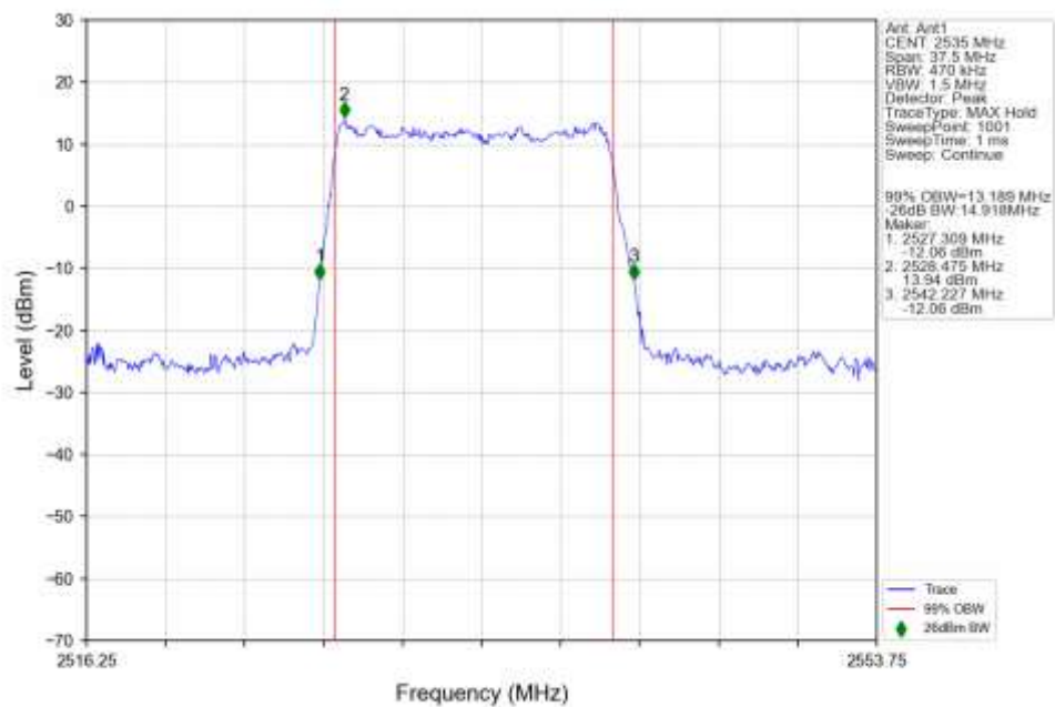
n7_30kHz_SISO_NTNV_15MHz_DFT-s-OFDM QPSK_2535MHz_Outer_Full_Ant1
