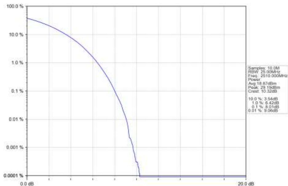
n7_15kHz_SISO_NTNV_20MHz_CP-OFDM_16_QAM_2510MHz_Outer_Full_Ant1
