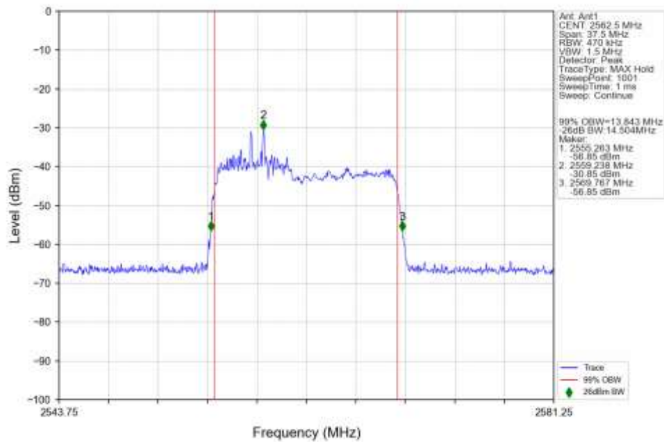
n7_30kHz_SISO_NTNV_15MHz_CP-OFDM_256_QAM_2562.5MHz_Outer_Full_Ant1
