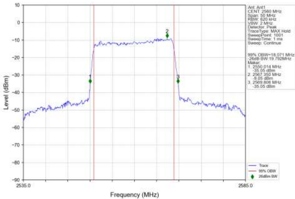
n7_30kHz_SISO_NTNV_20MHz_DFT-s-OFDM_16_QAM_2560MHz_Outer_Full_Ant1
