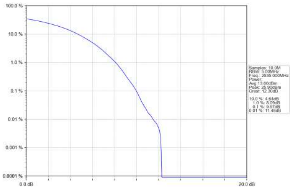
n7_15kHz_SISO_NTNV_5MHz_CP-OFDM_256_QAM_2535MHz_Outer_Full_Ant1
