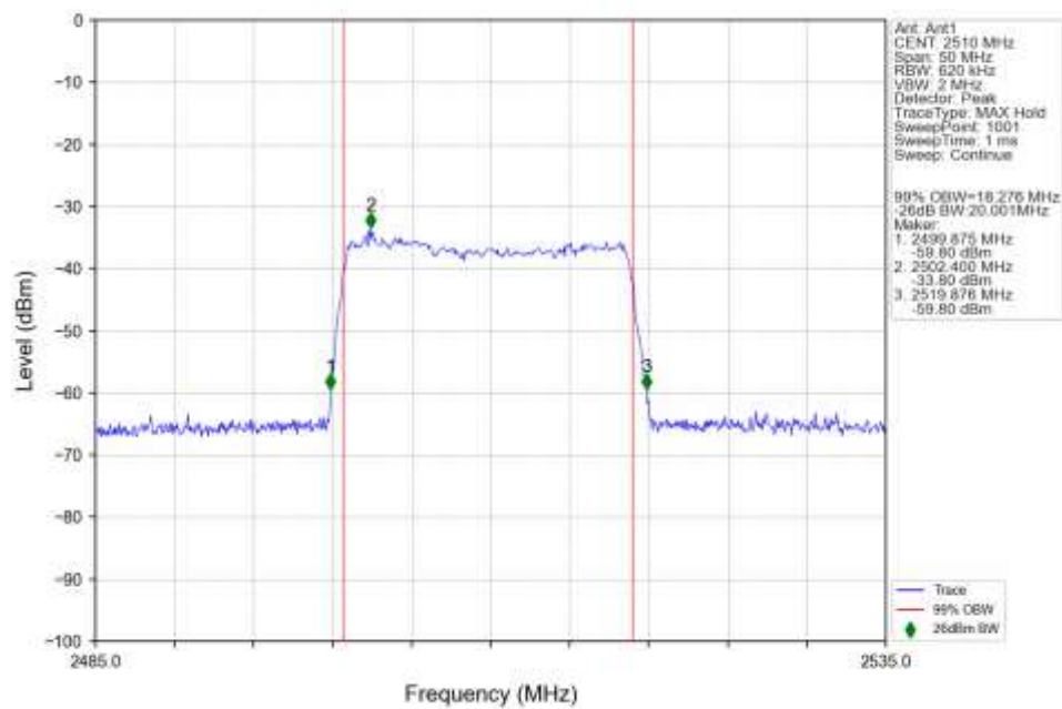
n7_30kHz_SISO_NTNV_20MHz_DFT-s-OFDM_16_QAM_2510MHz_Outer_Full_Ant1
