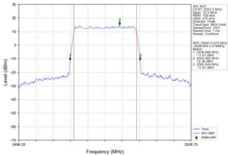
n7_15kHz_SISO_NTNV_5MHz_DFT-s-OFDM_16_QAM_2502.5MHz_Outer_Full_Ant1
