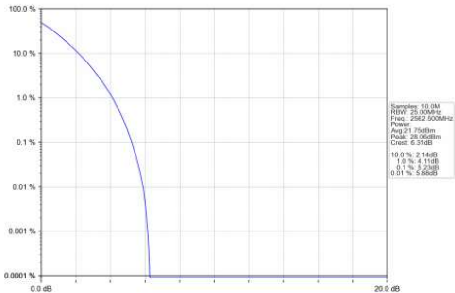
n7_15kHz_SISO_NTNV_15MHz_DFT-s-OFDM_QPSK_2562.5MHz_Outer_Full_Ant1
