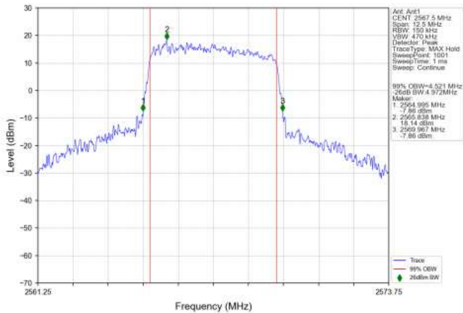
n7_15kHz_SISO_NTNV_5MHz_CP-OFDM_16_QAM_2567.5MHz_Outer_Full_Ant1
