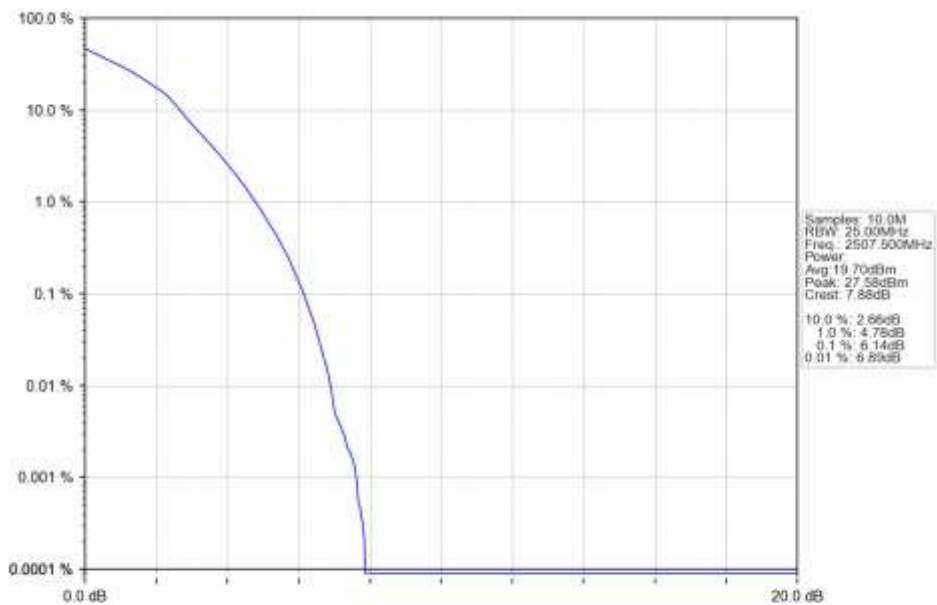
n7_15kHz_SISO_NTNV_15MHz_DFT-s-OFDM_16_QAM_2507.5MHz_Outer_Full_Ant1
