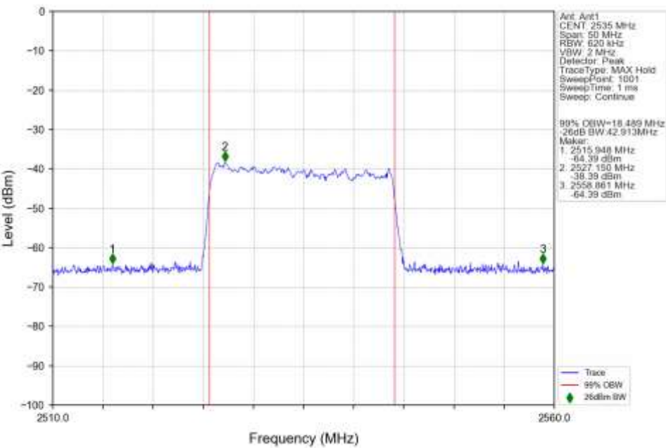
n7_30kHz_SISO_NTNV_20MHz_DFT-s-OFDM_64_QAM_2535MHz_Outer_Full_Ant1
