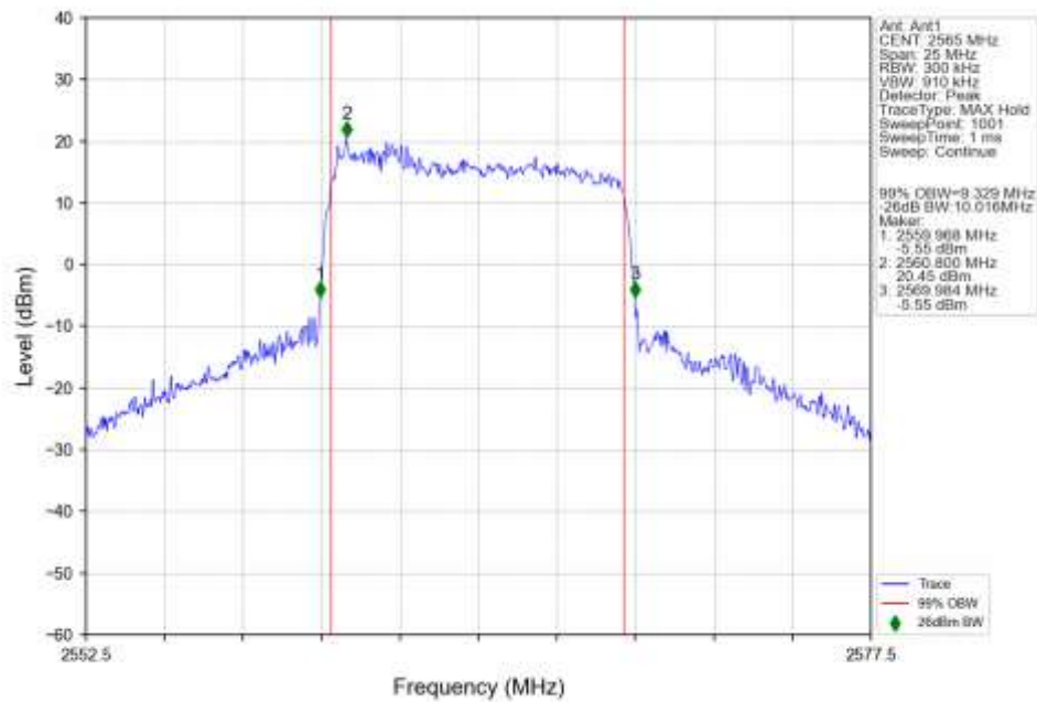
n7_15kHz_SISO_NTNV_10MHz_CP-OFDM_16_QAM_2565MHz_Outer_Full_Ant1
