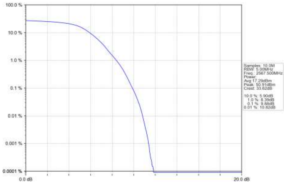
n7_15kHz_SISO_NTNV_5MHz_DFT-s-OFDM_QPSK_2567.5MHz_Outer_Full_Ant1
