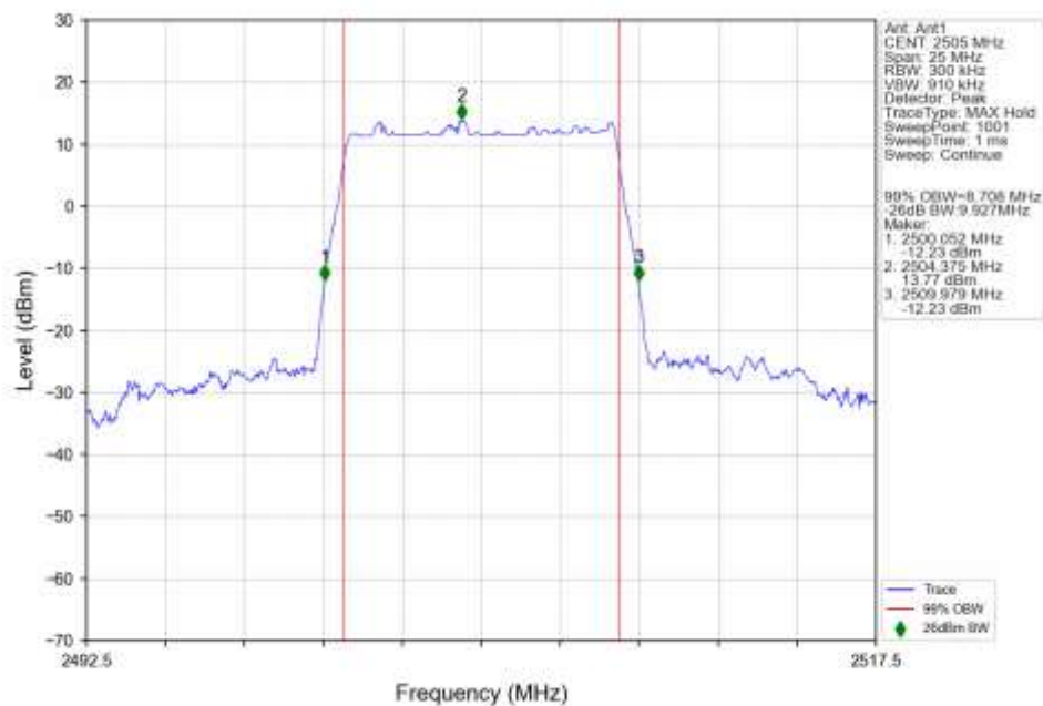
n7_30kHz_SISO_NTNV_10MHz_DFT-s-OFDM_256_QAM_2505MHz_Outer_Full_Ant1
