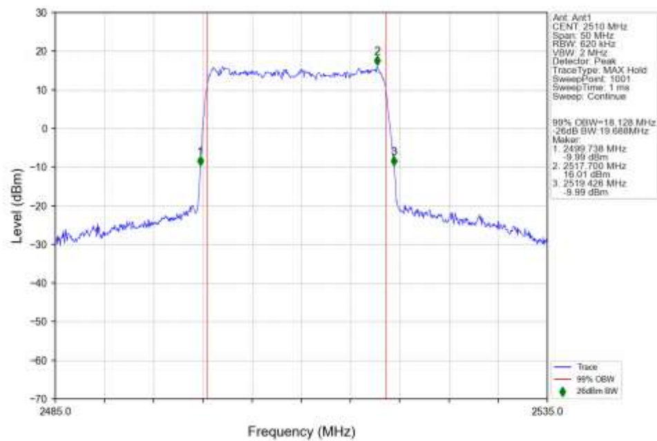
n7_15kHz_SISO_NTNV_20MHz_DFT-s-OFDM_16_QAM_2510MHz_Outer_Full_Ant1
