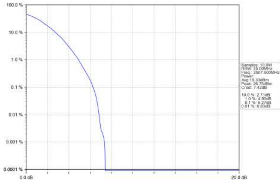
n7_15kHz_SISO_NTNV_15MHz_DFT-s-OFDM_64_QAM_2507.5MHz_Outer_Full_Ant1
