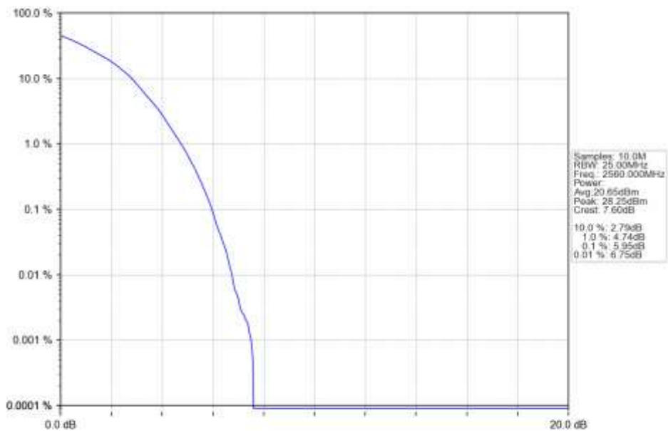
n7_15kHz_SISO_NTNV_20MHz_DFT-s-OFDM_16_QAM_2560MHz_Outer_Full_Ant1
