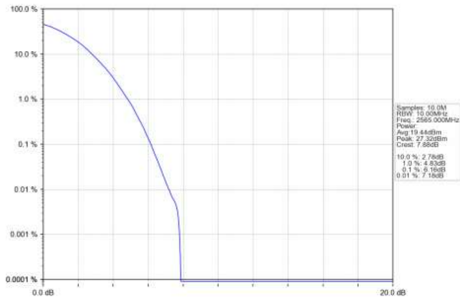
n7_15kHz_SISO_NTNV_10MHz_DFT-s-OFDM_256_QAM_2565MHz_Outer_Full_Ant1
