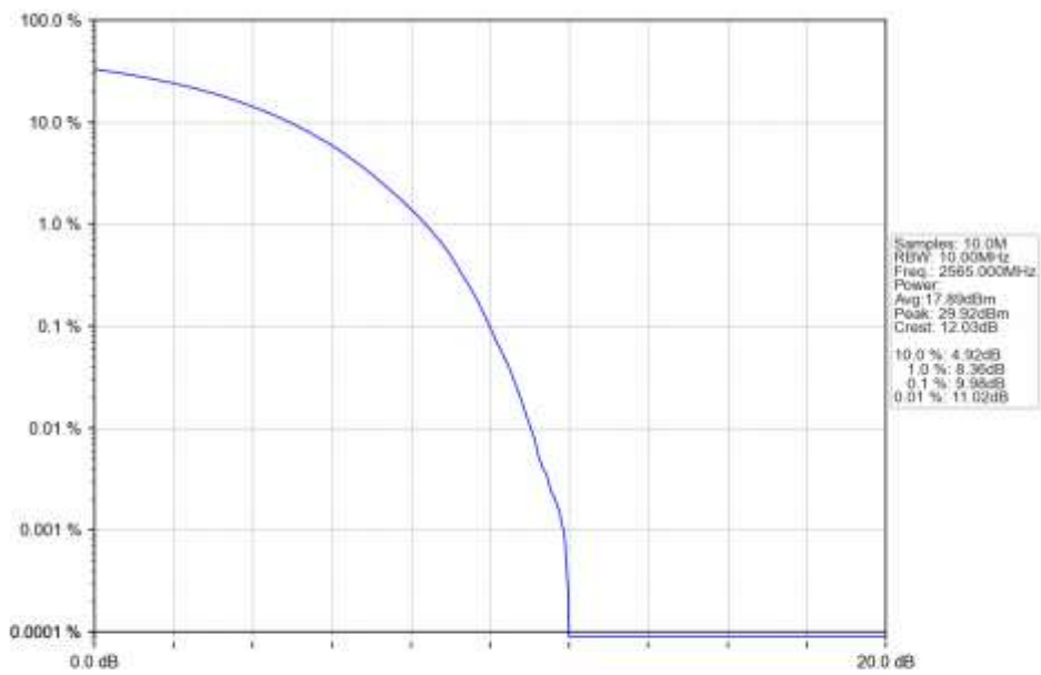
n7_15kHz_SISO_NTNV_10MHz_CP-OFDM_64_QAM_2565MHz_Outer_Full_Ant1
