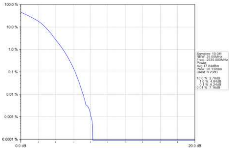
n7_15kHz_SISO_NTNV_20MHz_DFT-s-OFDM_16_QAM_2535MHz_Outer_Full_Ant1
