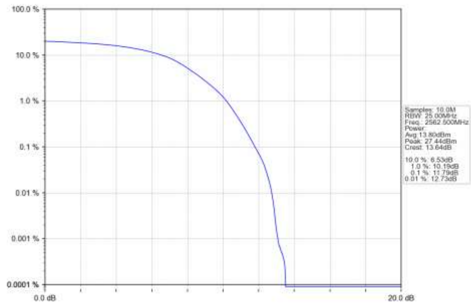
n7_15kHz_SISO_NTNV_15MHz_DFT-s-OFDM_64_QAM_2562.5MHz_Outer_Full_Ant1
