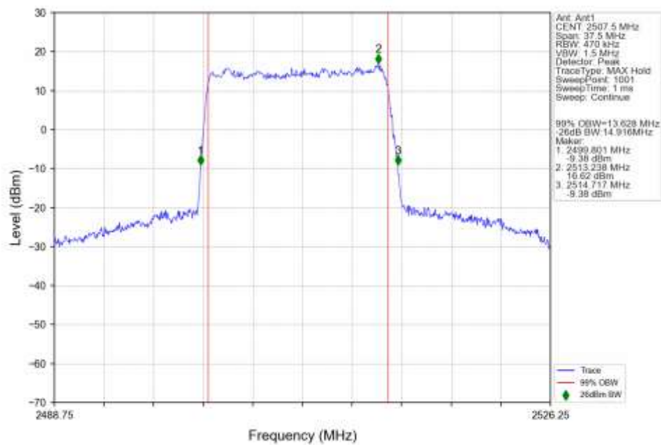
n7_15kHz_SISO_NTNV_15MHz_DFT-s-OFDM_16_QAM_2507.5MHz_Outer_Full_Ant1
