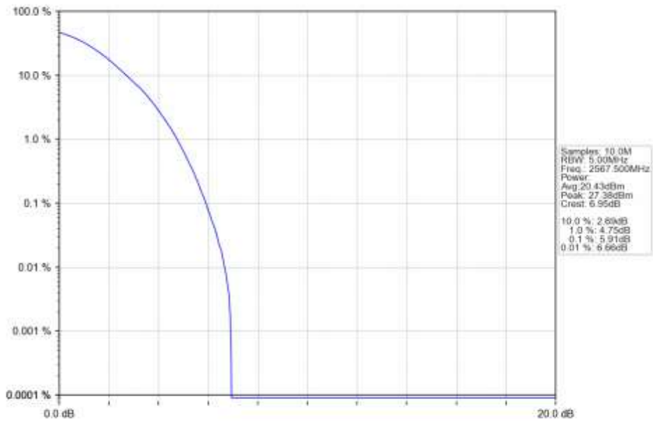
n7_15kHz_SISO_NTNV_5MHz_DFT-s-OFDM_64_QAM_2567.5MHz_Outer_Full_Ant1
