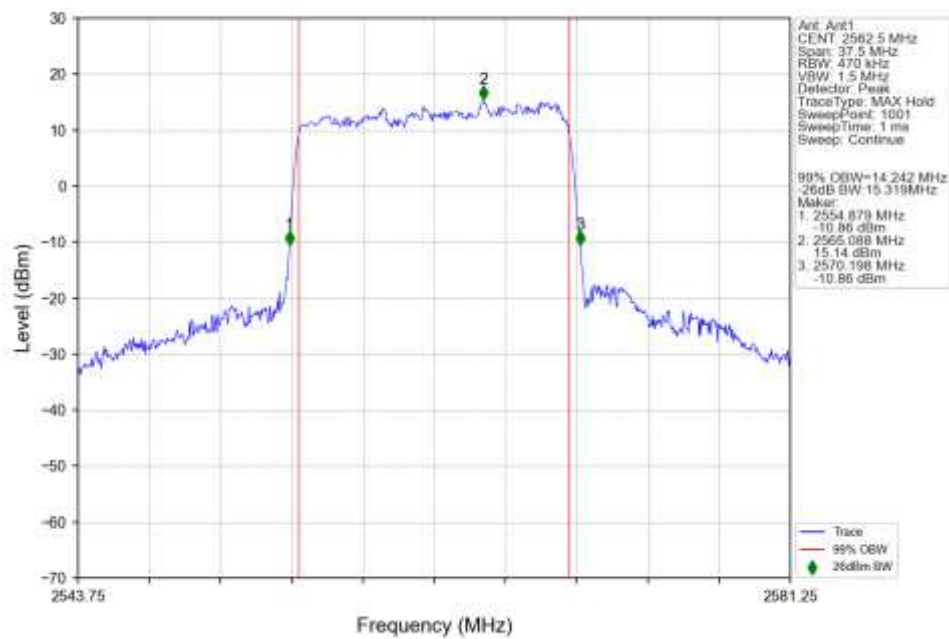
n7_15kHz_SISO_NTNV_15MHz_CP-OFDM_256_QAM_2562.5MHz_Outer_Full_Ant1
