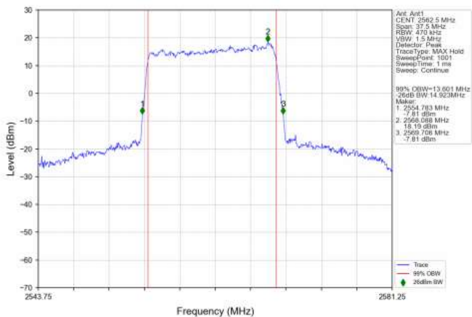
n7_15kHz_SISO_NTNV_15MHz_DFT-s-OFDM_16_QAM_2562.5MHz_Outer_Full_Ant1
