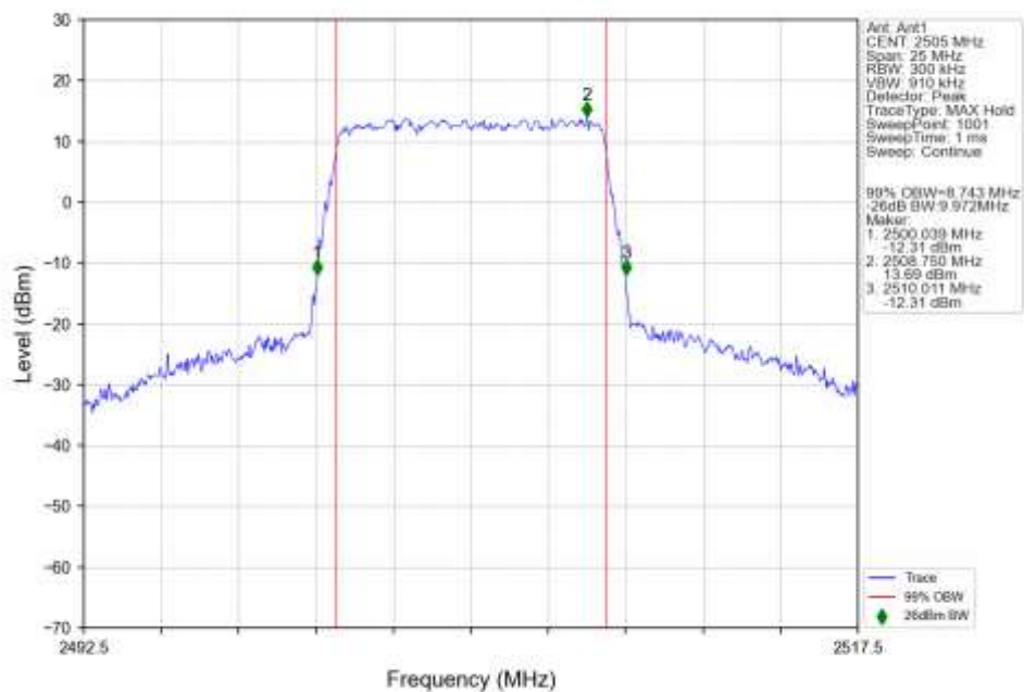
n7_30kHz_SISO_NTNV_10MHz_CP-OFDM_16_QAM_2505MHz_Outer_Full_Ant1
