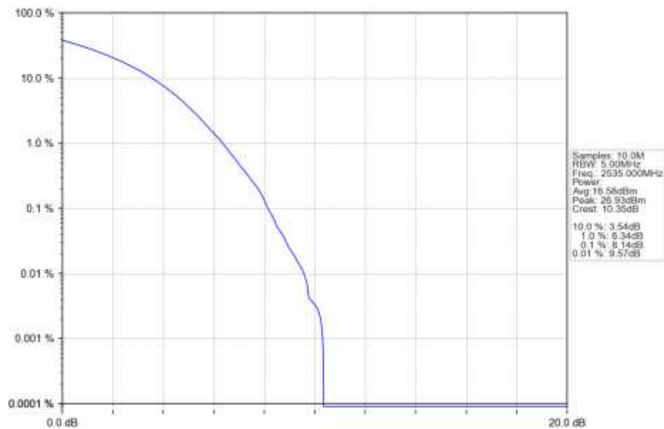
n7_15kHz_SISO_NTNV_5MHz_CP-OFDM_64_QAM_2535MHz_Outer_Full_Ant1
