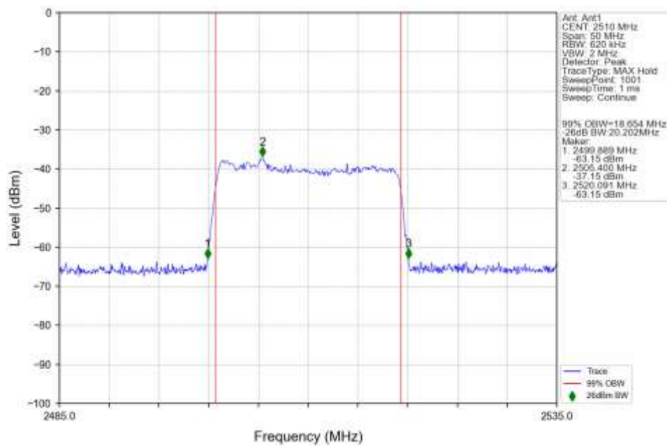
n7_30kHz_SISO_NTNV_20MHz_CP-OFDM_256_QAM_2510MHz_Outer_Full_Ant1
