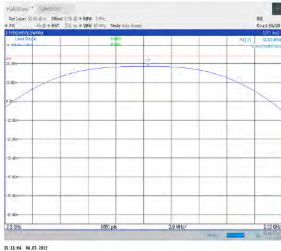
1-N30-PC3-15-10-M-3-DFT-PI2BPSK-Outer_Full- 50@0-2300-2320-Ant1-18.53-23.98-PASS
