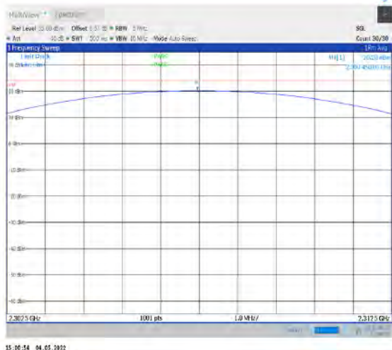
1-N30-PC3-15-5-L-3-DFT-PI2BPSK-Outer_Full- 25@0-2302.5-2312.5-Ant1-20.20-23.98-PASS
