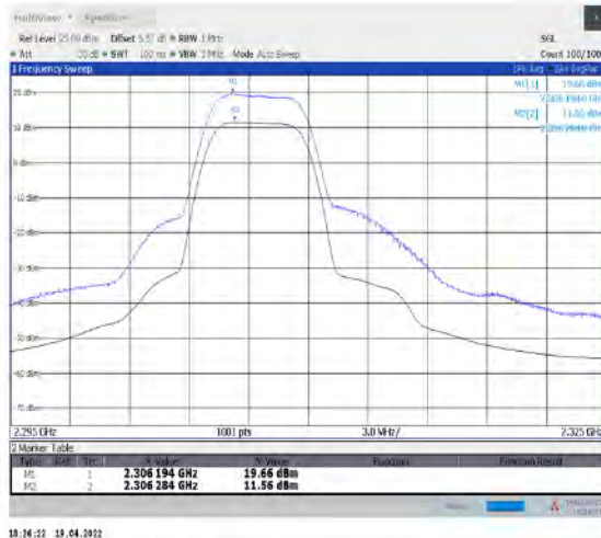
1-N30--15-10-M-1-DFT-256QAM-Outer_Full-24@0-Ant1-8.10-100%-0.00-8.10-PASS-≤13
