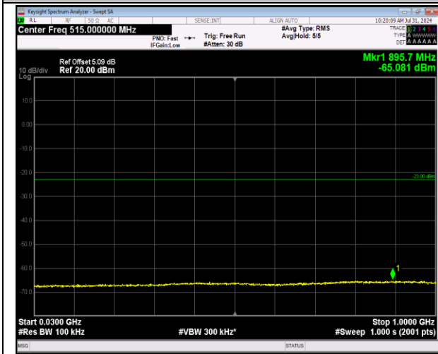
2-2-20MHz-20MHz-64QAM-64QAM-18902-19100-100RB#0-100RB#0-30~1000MHz-PASS
