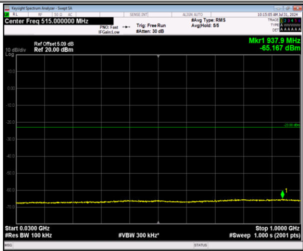
2-2-20MHz-20MHz-64QAM-64QAM-18700-18898-100RB#0-100RB#0-30~1000MHz-PASS
