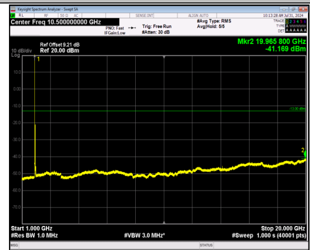
2-2-20MHz-20MHz-64QAM-64QAM-18700-18898-1RB#0 -0RB#0-1000~20000MHz-PASS
