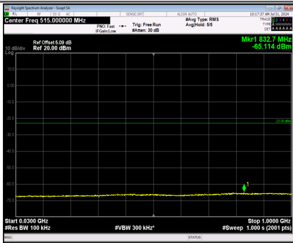
2-2-20MHz-20MHz-64QAM-64QAM-18801-18999-100RB#0 B#0-100RB#0-30~1000MHz-PASS
