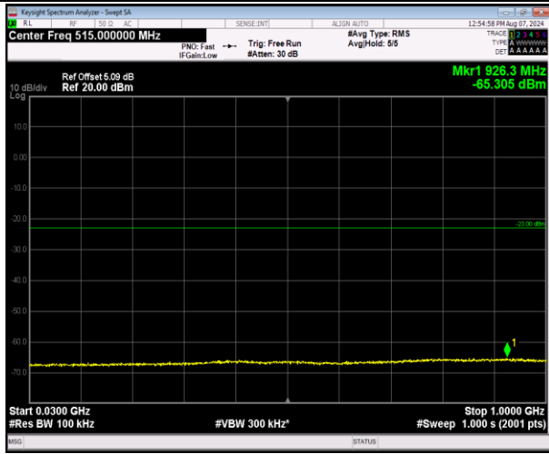
2-2-5MHz-20MHz-16QAM-16QAM-18983-19100-25RB#0 0-100RB#0-30~1000MHz-PASS
