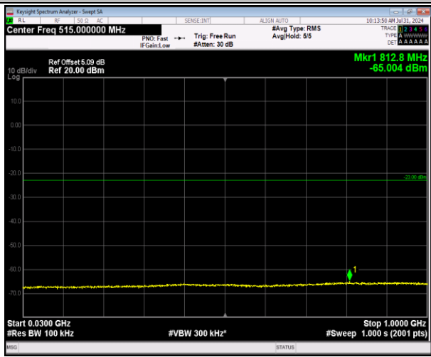
2-2-20MHz-20MHz-64QAM-64QAM-18700-18898-1RB#99-0RB#0-30~1000MHz-PASS
