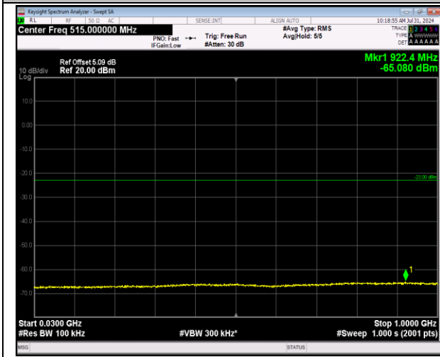
2-2-20MHz-20MHz-64QAM-64QAM-18902-19100-1RB#99-0RB#0-30~1000MHz-PASS
