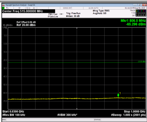
2-2-20MHz-20MHz-16QAM-16QAM-18700-18898-100R B#0-100RB#0-30~1000MHz-PASS
