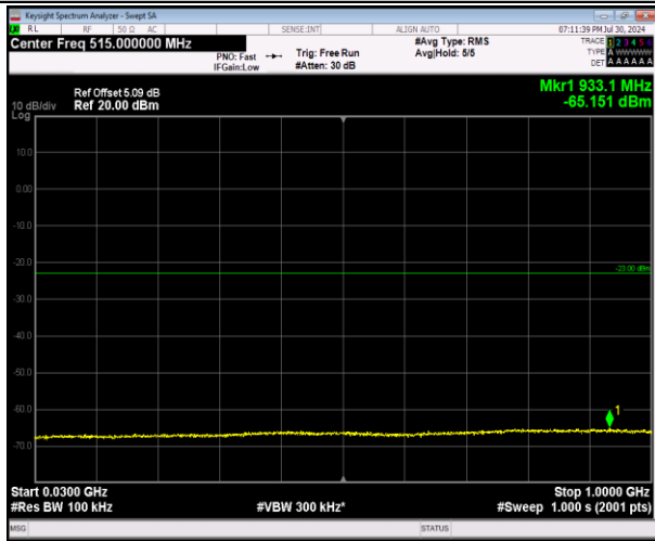
2-2-5MHz-20MHz-64QAM-64QAM-18983-19100-1RB#0- 0RB#0-30~1000MHz-PASS
