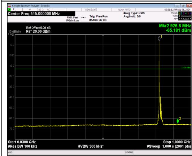
5-5-3MHz-5MHz-16QAM-16QAM-20416-20455-1RB#0-0 RB#0-30~1000MHz-PASS
