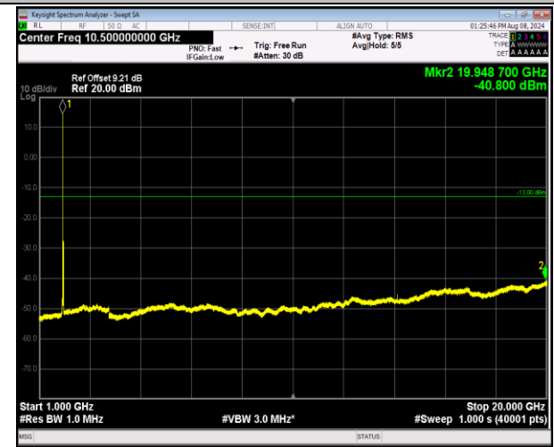
2-2-20MHz-20MHz-16QAM-16QAM-18902-19100-1RB#0 -1RB#99-1000~20000MHz-PASS
