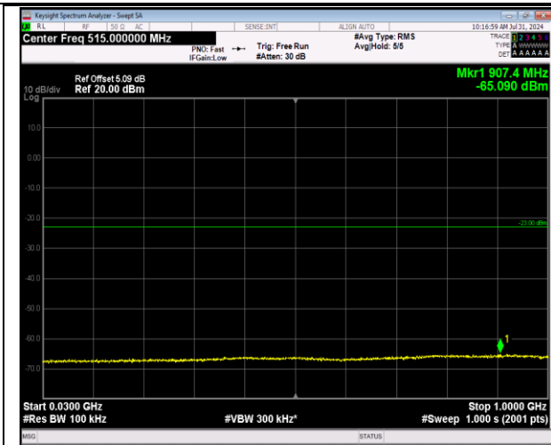
2-2-20MHz-20MHz-64QAM-64QAM-18801-18999-1RB#0 0-1RB#99-30~1000MHz-PASS
