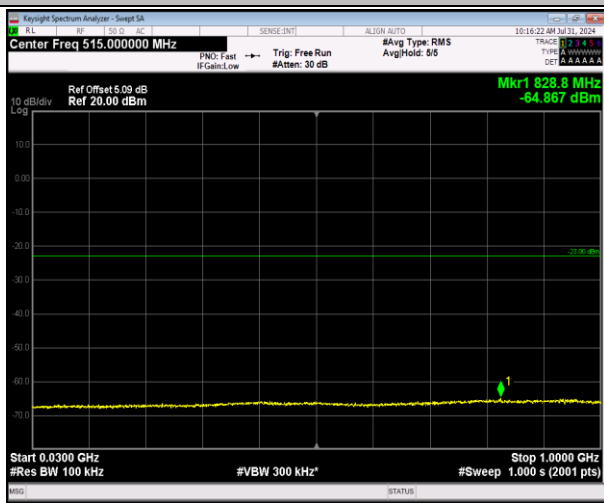
2-2-20MHz-20MHz-64QAM-64QAM-18801-18999-1RB#0 99-0RB#0-30~1000MHz-PASS
