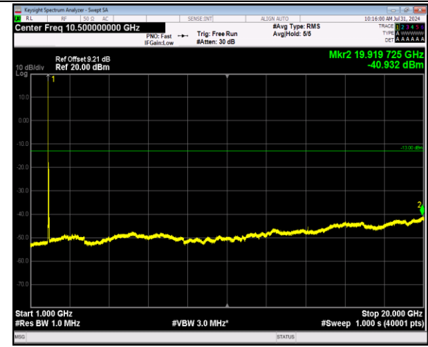
2-2-20MHz-20MHz-64QAM-64QAM-18801-18999-1RB#0-0RB#0-1000~20000MHz-PASS
