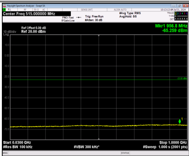
2-2-20MHz-20MHz-64QAM-64QAM-18700-18898-1RB# 0-0RB#0-30~1000MHz-PASS
