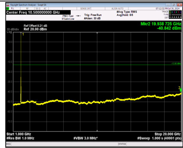
2-2-5MHz-20MHz-64QAM-64QAM-18983-19100-1RB#24-0RB#0-1000~20000MHz-PASS
