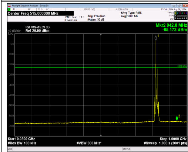
5-5-3MHz-5MHz-16QAM-16QAM-20416-20455-1RB#0-1 RB#24-30~1000MHz-PASS
