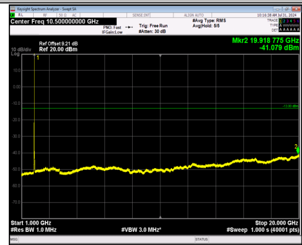
2-2-20MHz-20MHz-64QAM-64QAM-18801-18999-1RB#0 9-0RB#0-1000~20000MHz-PASS
