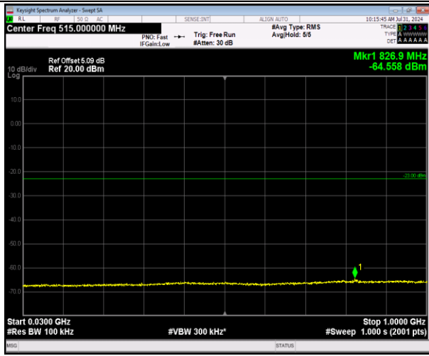
2-2-20MHz-20MHz-64QAM-64QAM-18801-18999-1RB#0-0RB#0-30~1000MHz-PASS
