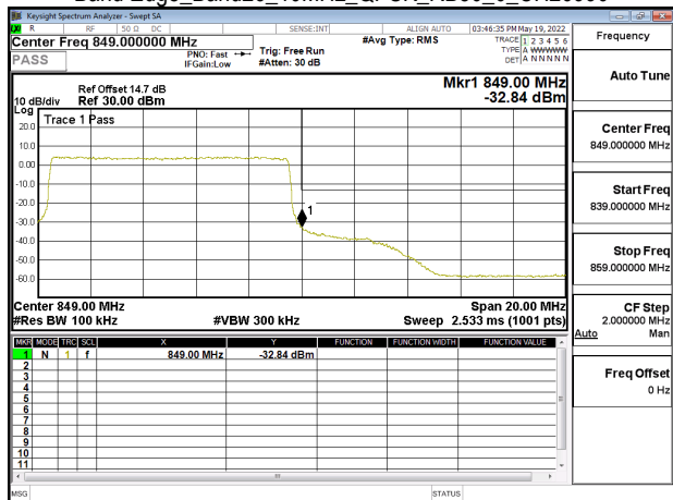
Band Edge_Band26_15MHz_QPSK_RB1_0_CH26865
