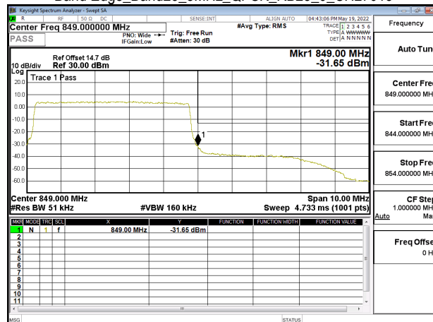
Band Edge_Band26_10MHz_QPSK_RB1_0_CH26840
