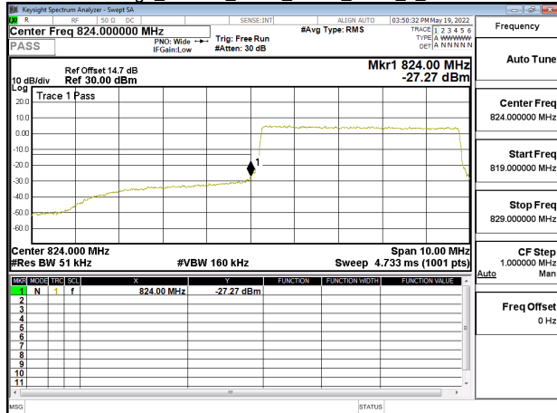
Band Edge_Band26_5MHz_QPSK_RB25_0_CH26815
