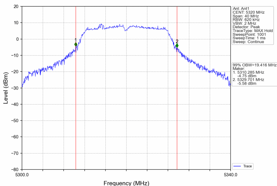
802.11a_HCH_5320MHz_Ant1_NTNV
