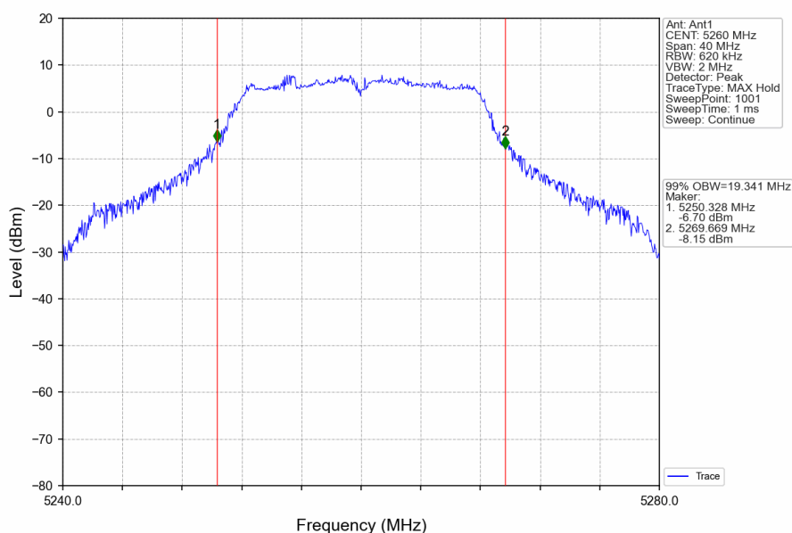
802.11a_LCH_5260MHz_Ant1_NTNV
