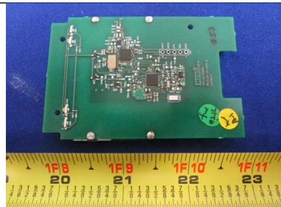
EUT Main PCB - Top View
