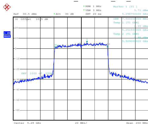
802.11ax80_5290MHz_RU_Full
