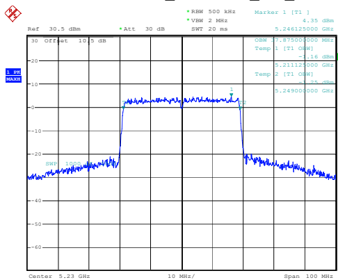
802.11ax40_5230MHz_RU_Full
