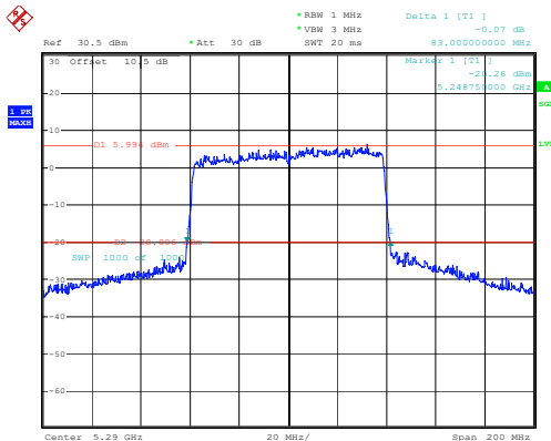
802.11ax80_5290MHz_RU_Full
