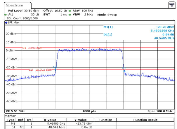
802.11ax40_5510MHz_RU_Full
