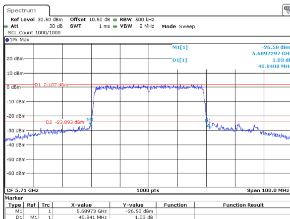
802.11ax40_5710MHz_RU_Full
