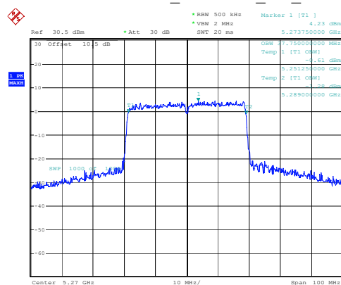
802.11ax40_5270MHz_RU_Full
