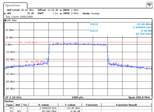
802.11ax80_5530MHz_RU_Full
