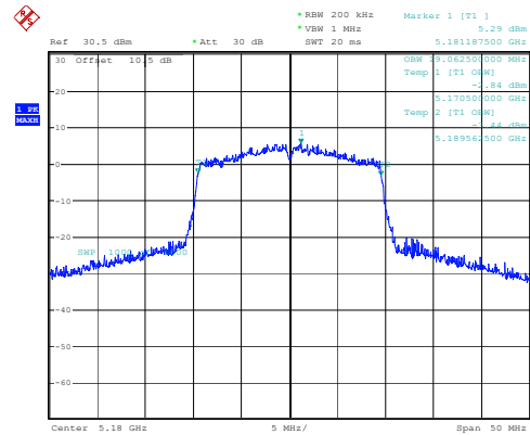
802.11ax20_5180MHz_RU_Full
