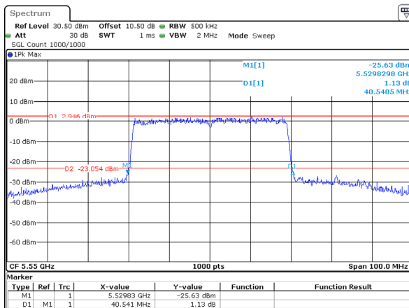
802.11ax40_5550MHz_RU_Full
