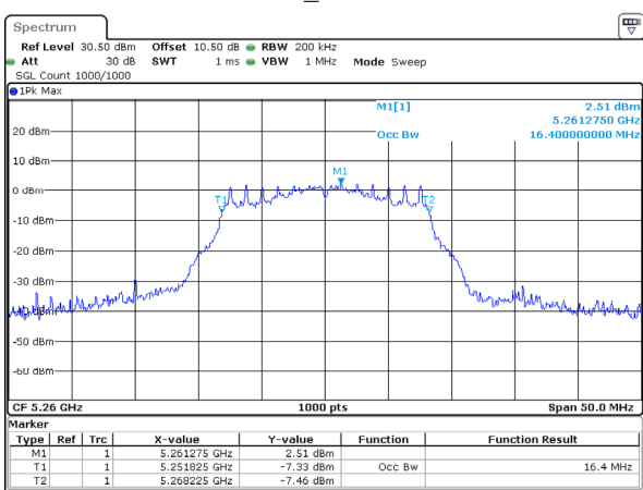
802.11a_5260MHz
