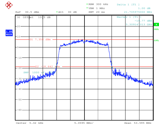
802.11ax20_5320MHz_RU_Full
