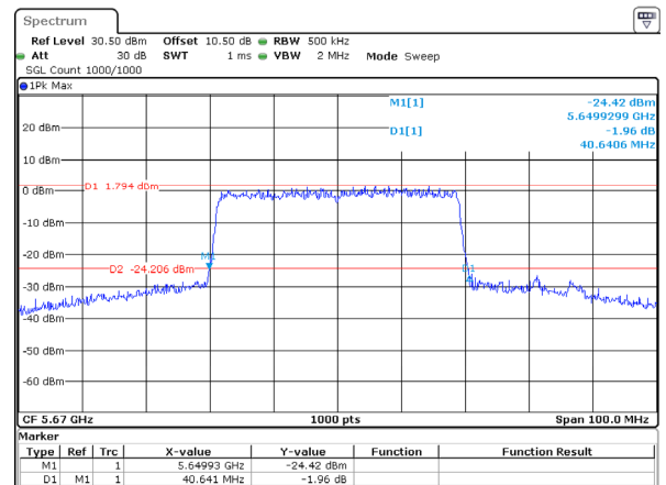
802.11ax40_5670MHz_RU_Full
