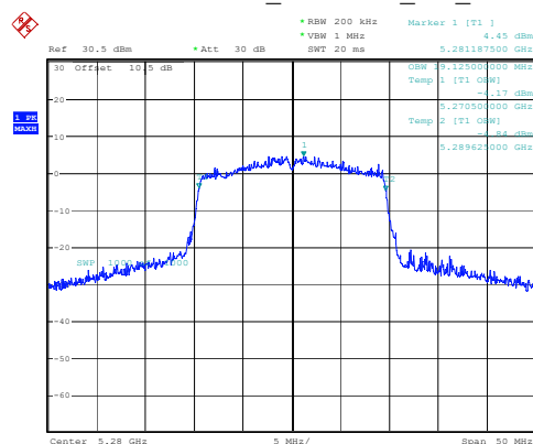
802.11ax20_5280MHz_RU_Full
