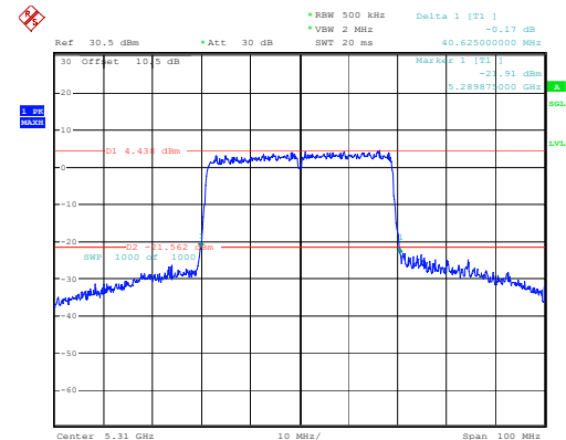
802.11ax40_5310MHz_RU_Full
