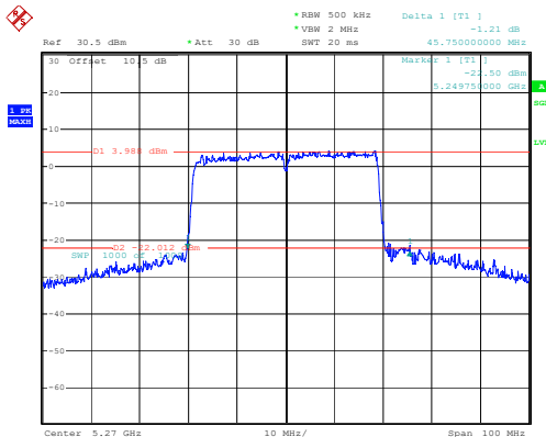
802.11ax40_5270MHz_RU_Full
