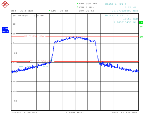
802.11ax20_5280MHz_RU_Full
