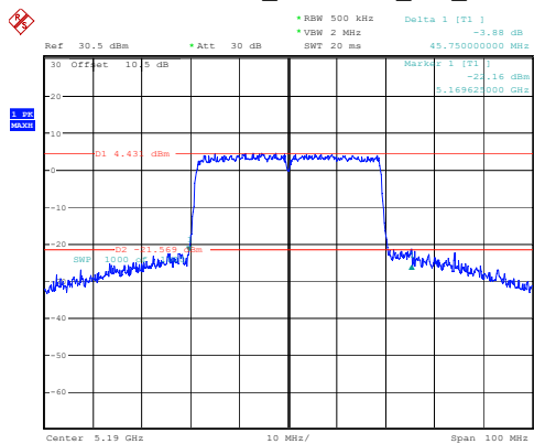
802.11ax40_5190MHz_RU_Full
