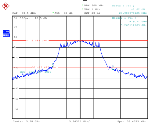
802.11a_5280MHz
