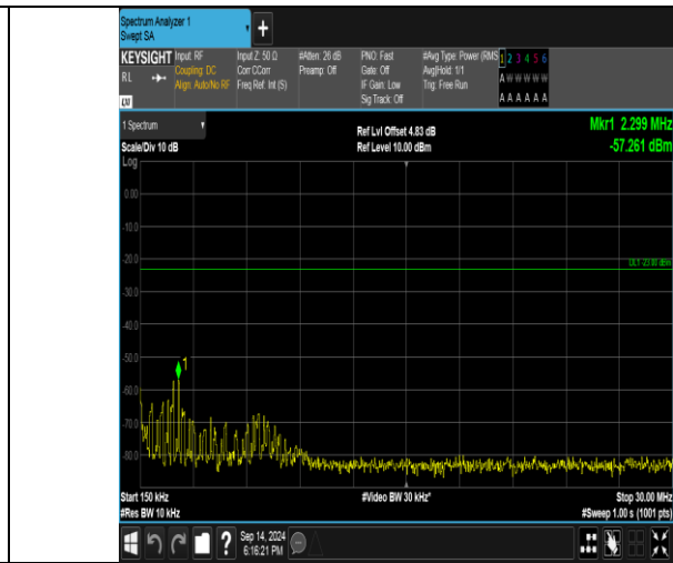
Band5-4132-0.15~30MHz-PASS
