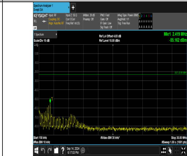
Band5-4182-0.15~30MHz-PASS
