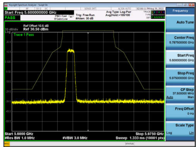
U-NII-3 ,Plot 1,Band Edge-802.11n(20M Hz),5785MHz,Ant1
