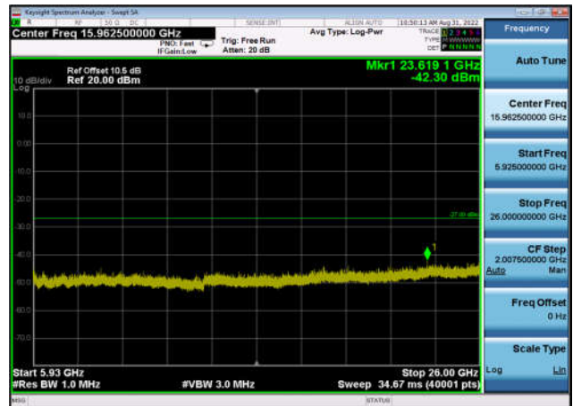
U-NII-3 ,Plot 3,5925MHz~26000MHz-802. 11ax(40MHz),5795MHz,Ant1
