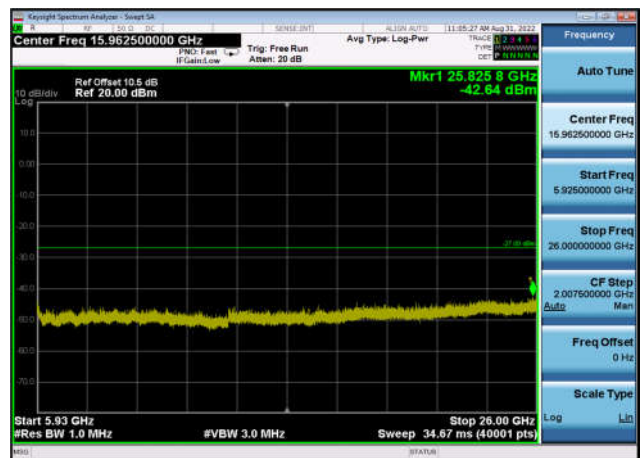
U-NII-3 ,Plot 3,5925MHz~26000MHz-802. 11ax(80MHz),5775MHz,Ant1
