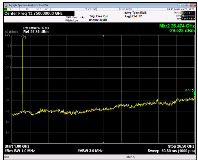
Band7-20MHz-64QAM-21350-1RB#0-Range2:1000~26500MHz
