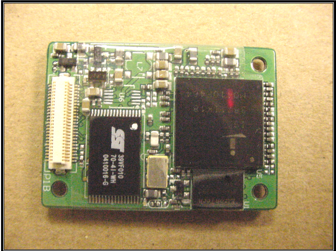
PHOTOGRAPH 16: BOTTOM OF MODULE
