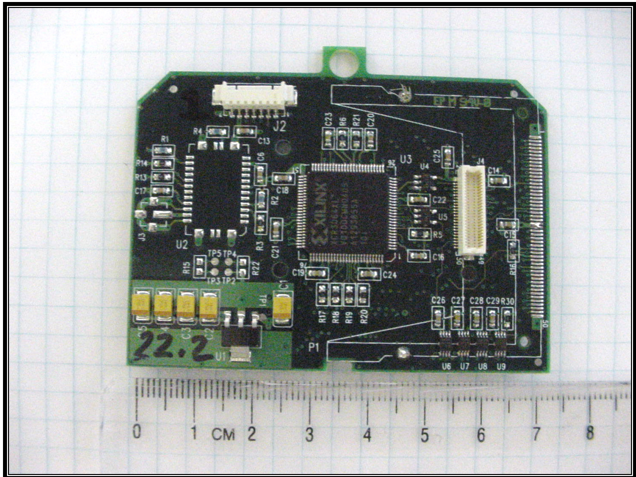
PHOTOGRAPH 17: TOP OF PCB FOR MOUNTING MODULE
