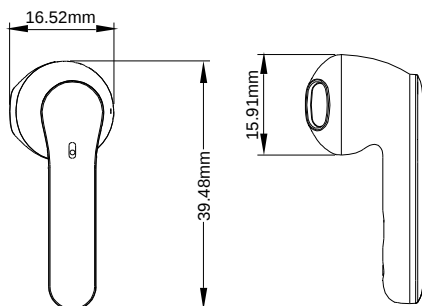
Earphone
